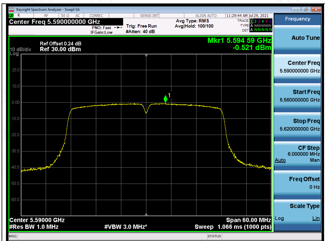
Test_Graph_802.11n40_ANT2_5590_MCS0_PSD
