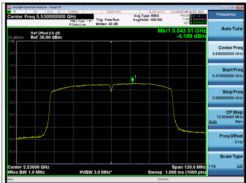
Test Graph 802.11ac80 ANT2 5530 MCS9 PSD
