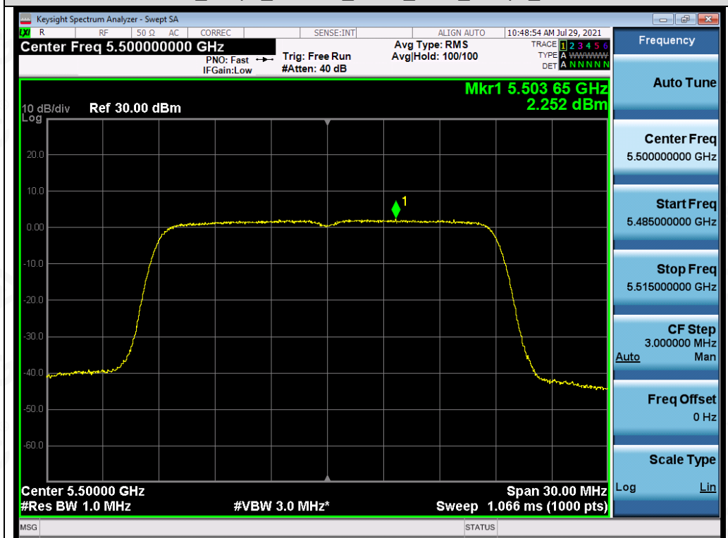
Test_Graph_802.11n20_ANT1_5500_MCS0_PSD
