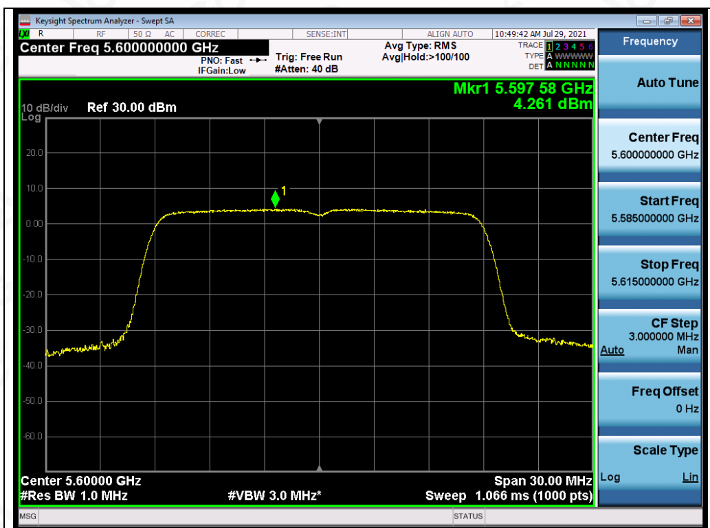
Test_Graph_802.11n20_ANT1_5600_MCS0_PSD
