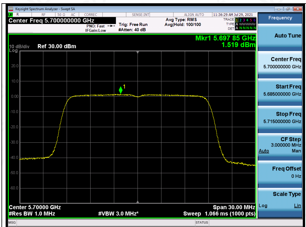
Test_Graph_802.11ac20_ANT2_5700_MCS9_PSD
