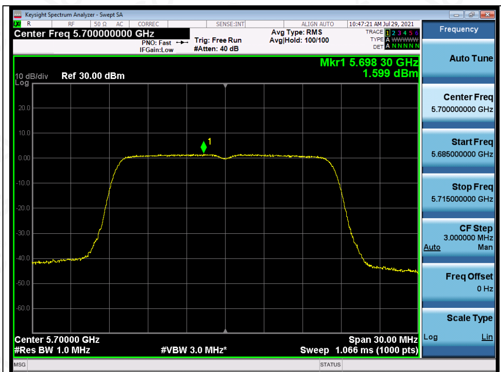
Test_Graph_802.11a_ANT1_5700_6Mbps_PSD
