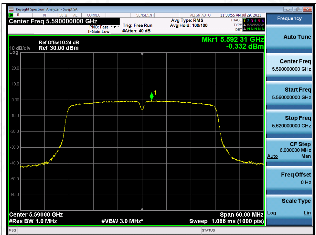
Test_Graph_802.11ac40_ANT2_5590_MCS9_PSD
