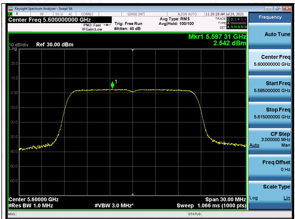
Test_Graph_802.11a_ANT2_5600_6Mbps_PSD
