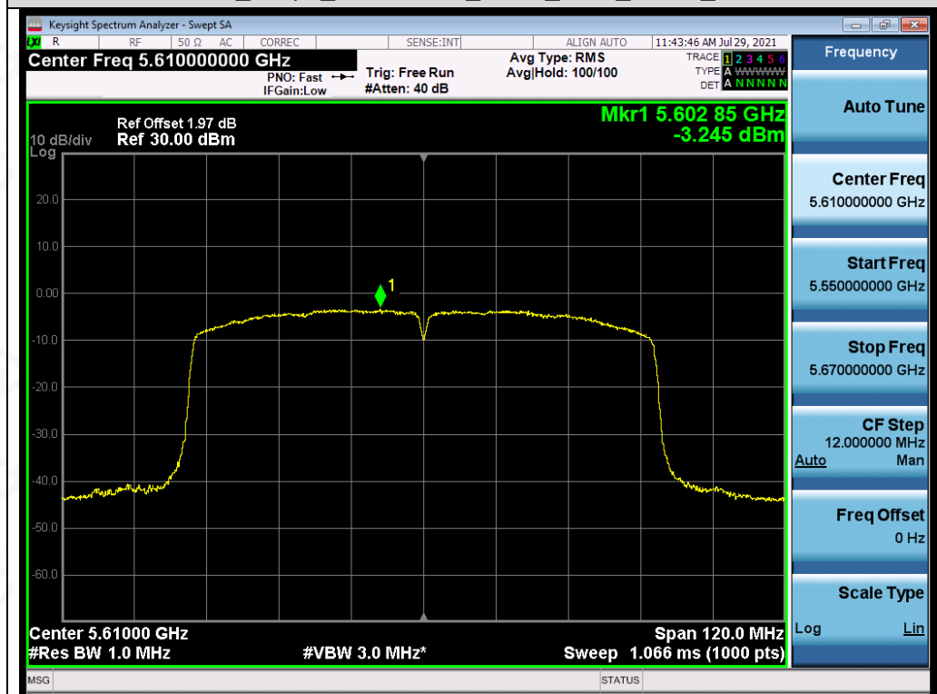
Test_Graph_802.11ac80_ANT2_5610_MCS9_PSD
