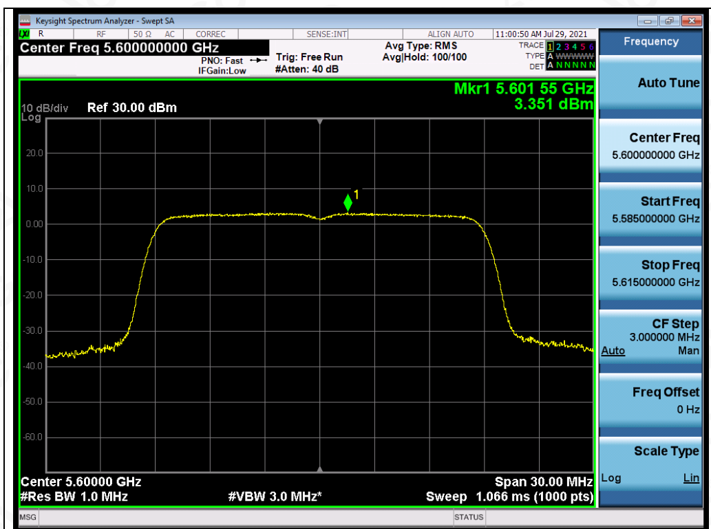
Test_Graph_802.11ac20_ANT1_5600_MCS0_PSD
