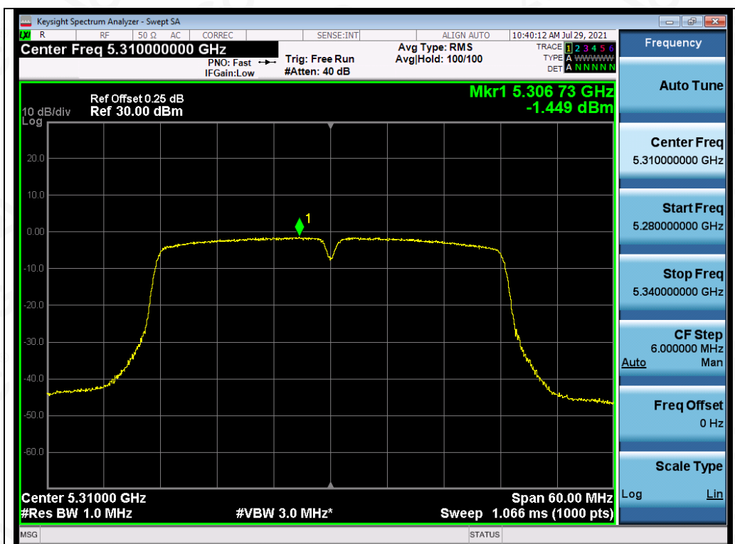
Test_Graph_802.11ac40_ANT2_5310_MCS9_PSD
