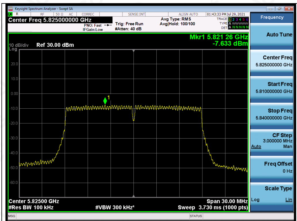
Test Graph 802.11ac20 ANT1 5825 MCS9 PSD
