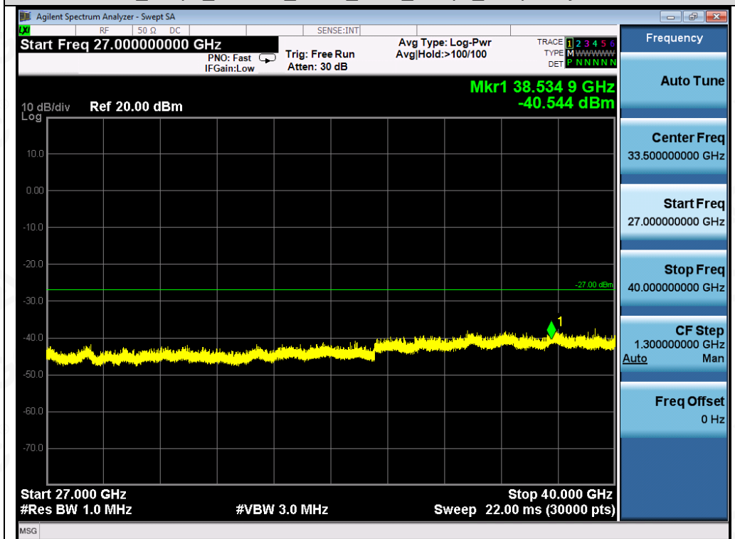
Test_Graph_802.11a_ANT1_5320_6Mbps_Frequency Band 5
