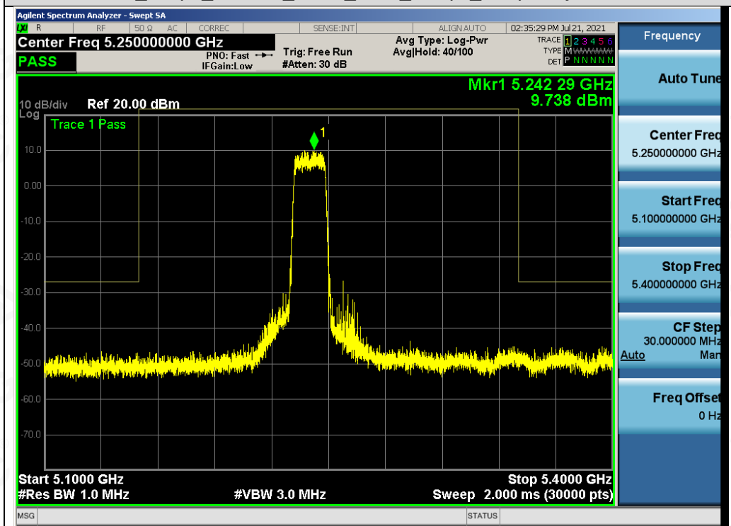
Test_Graph_802.11a_ANT1_5240_6Mbps_Frequency Band 3
