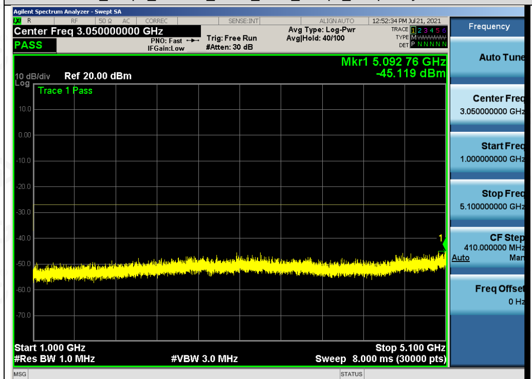
Test_Graph_802.11a_ANT1_5180_6Mbps_Frequency Band 2
