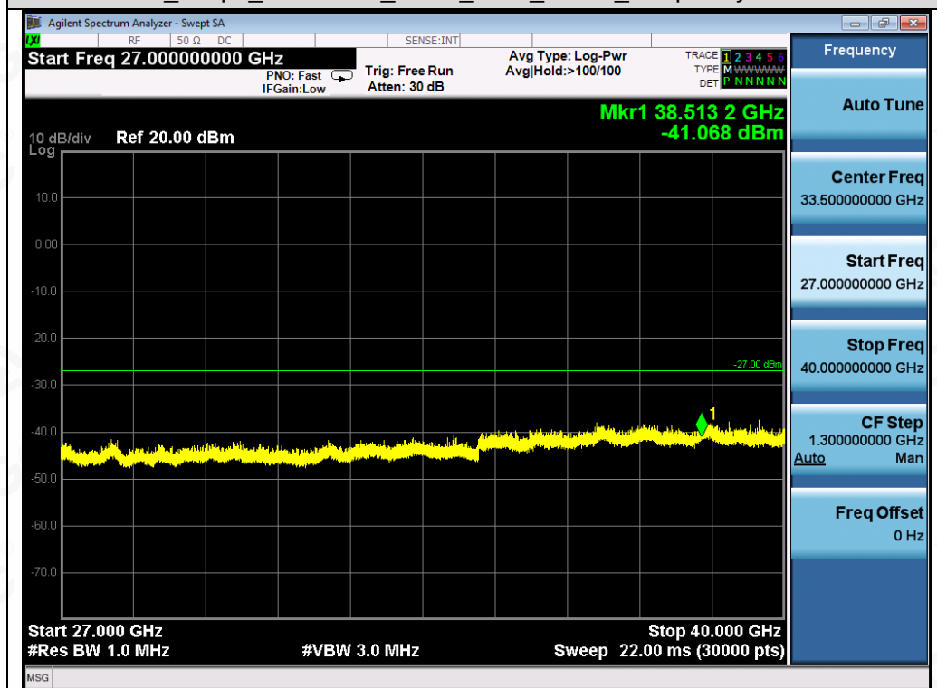
Test_Graph_802.11n40_ANT1_5310_MCS0_Frequency Band 5
