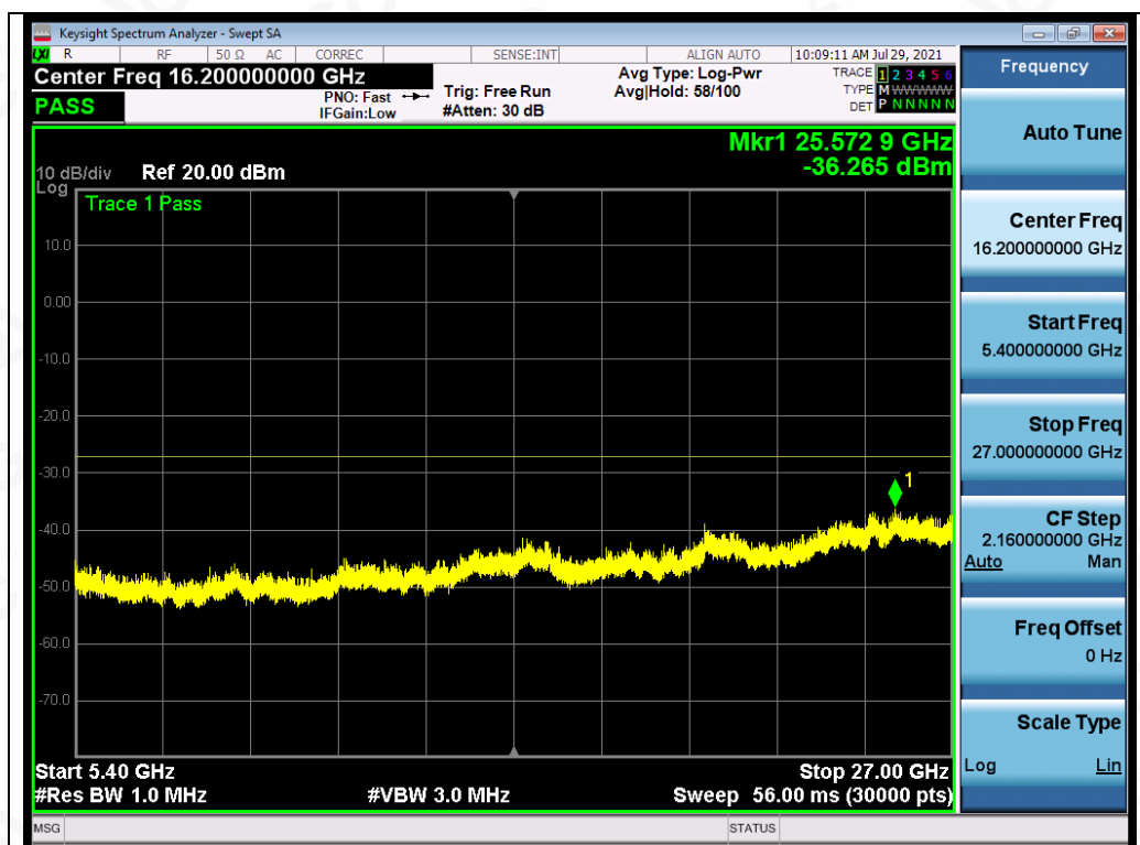
Test_Graph_802.11n40_ANT1_5310_MCS0_Frequency Band 4
