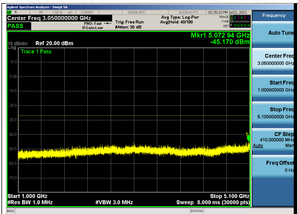
Test_Graph_802.11a_ANT1_5240_6Mbps_Frequency Band 2
