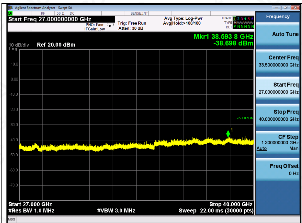
Test Graph 802.11n40 ANT1 5190 MCS0 Frequency Band 5
