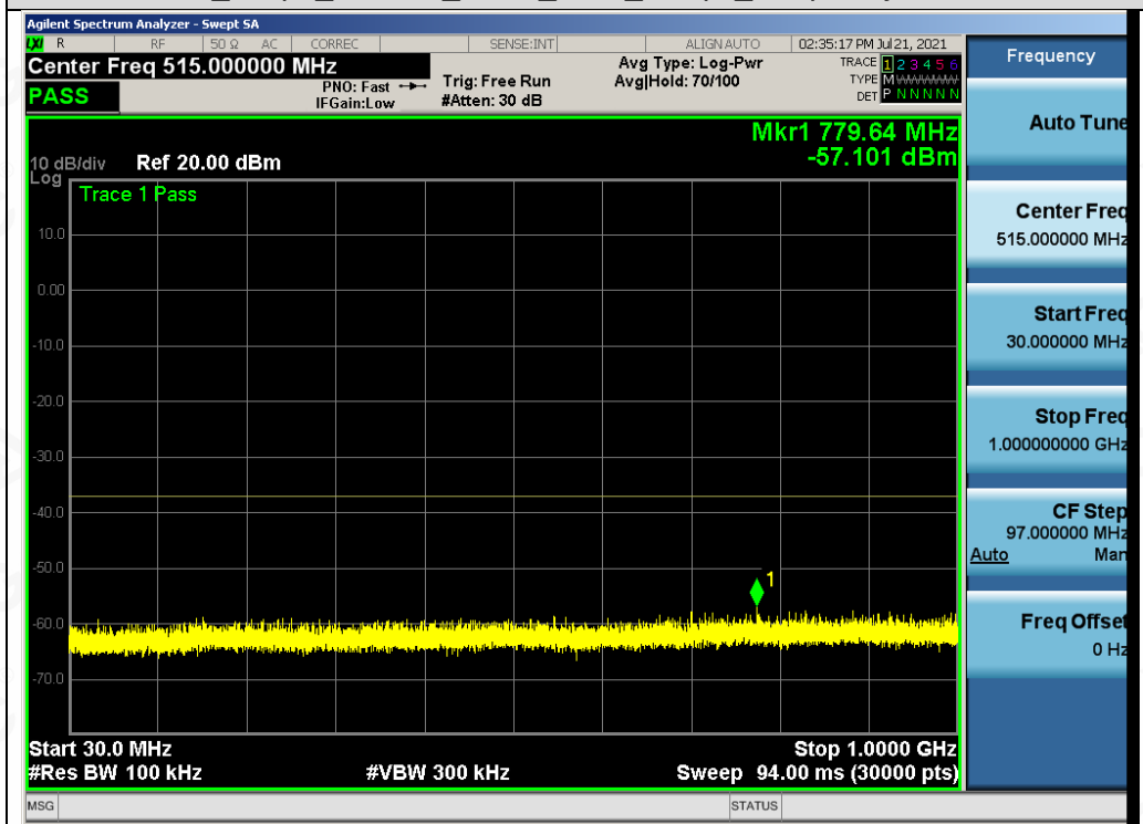
Test_Graph_802.11a_ANT1_5240_6Mbps_Frequency Band 1
