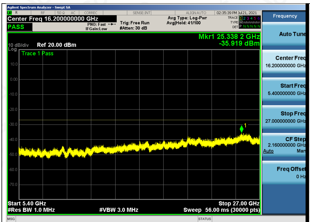
Test_Graph_802.11a_ANT1_5240_6Mbps_Frequency Band 4
