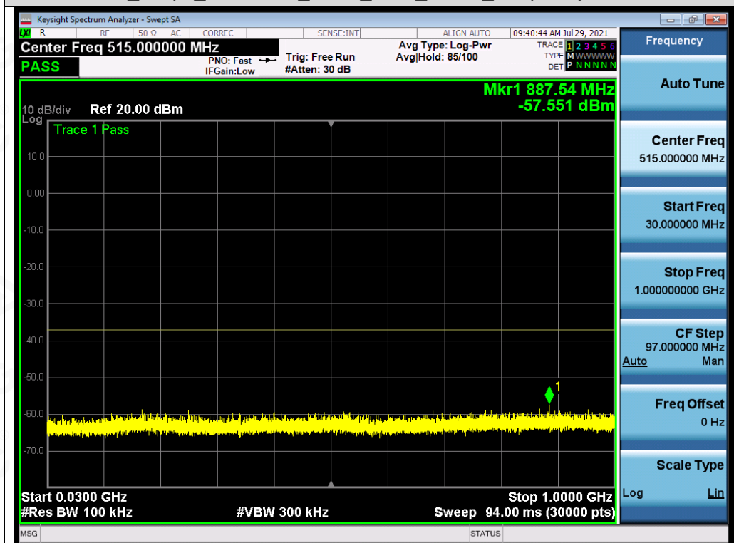
Test Graph 802.11n40 ANT1 5230 MCS0 Frequency Band 1
