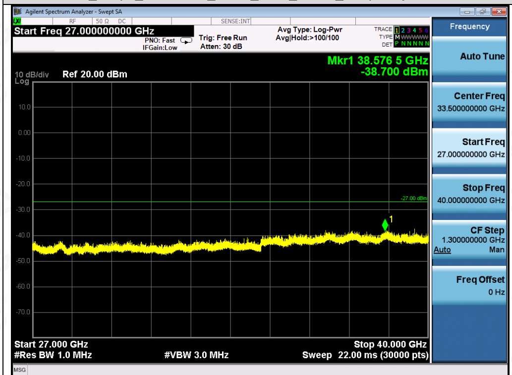
Test_Graph_802.11n40_ANT1_5230_MCS0_Frequency Band 5
