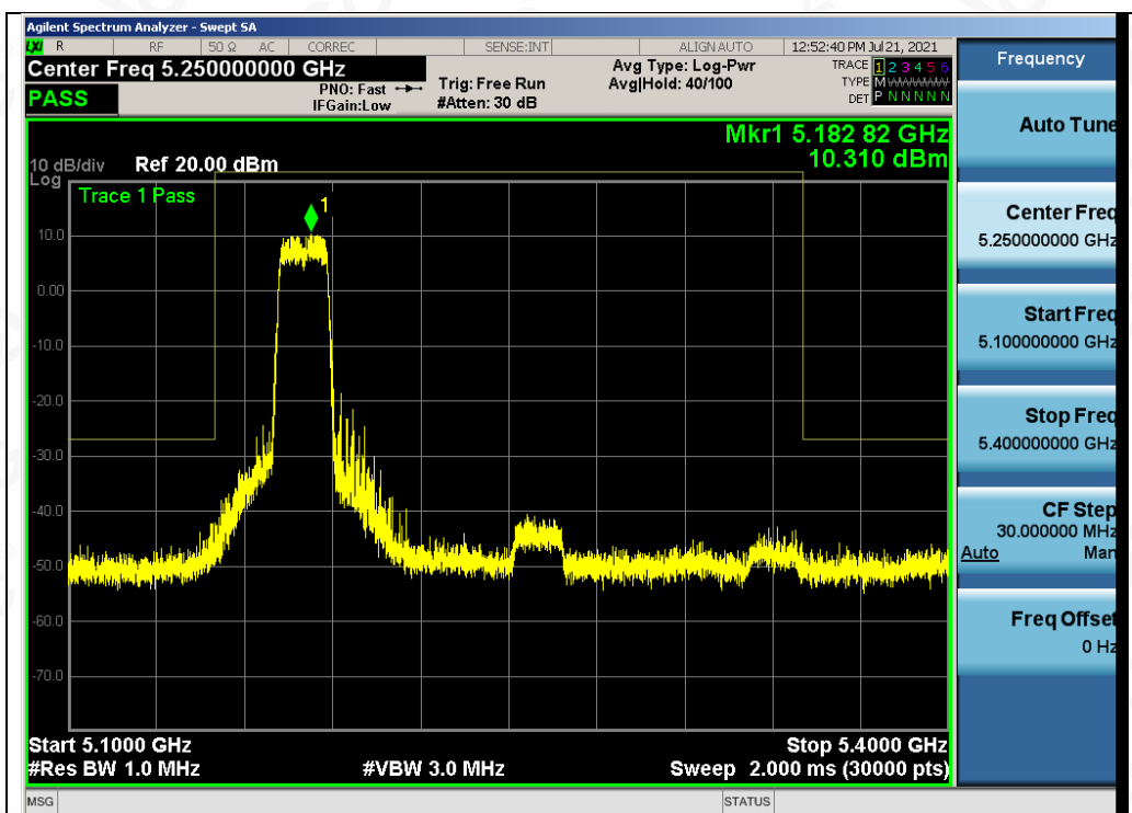
Test_Graph_802.11a_ANT1_5180_6Mbps_Frequency Band 3
