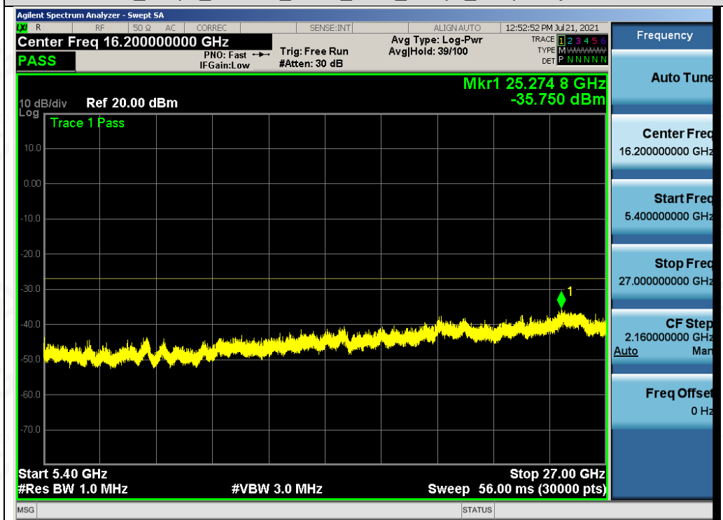
Test_Graph_802.11a_ANT1_5180_6Mbps_Frequency Band 4
