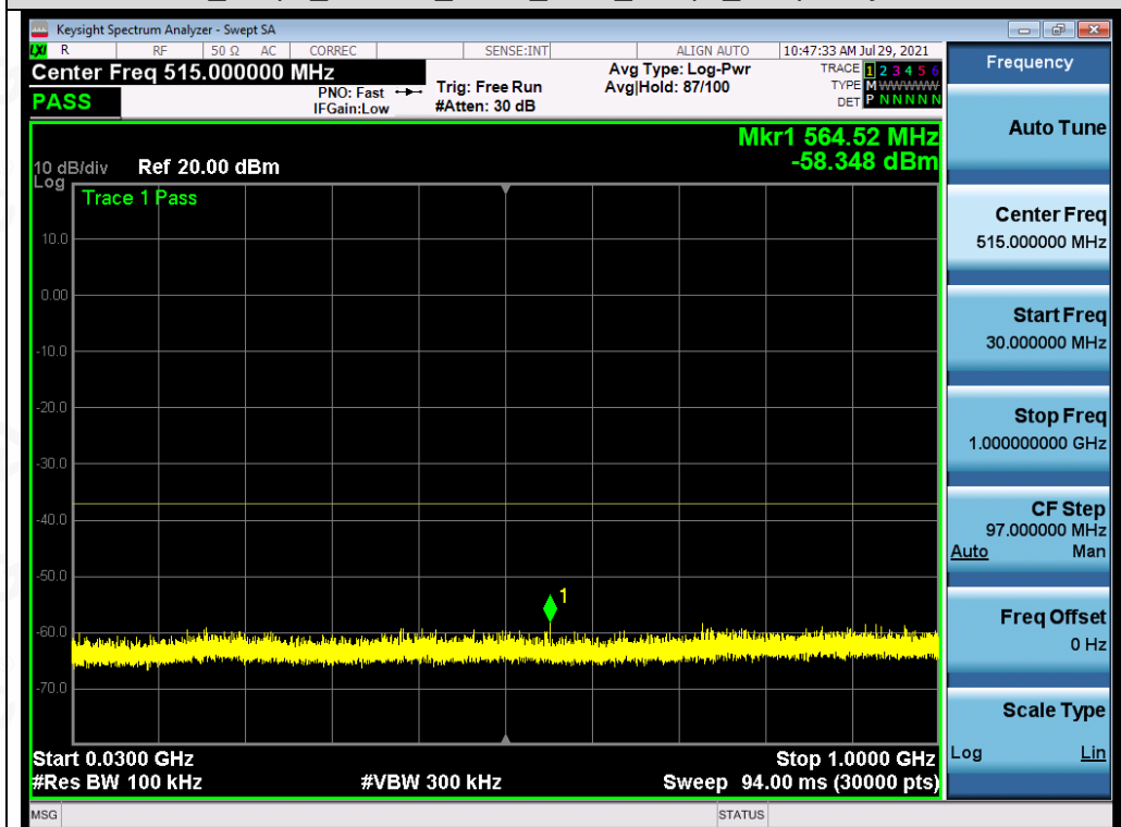
Test Graph 802.11a ANT1 5700 6Mbps Frequency Band 1
