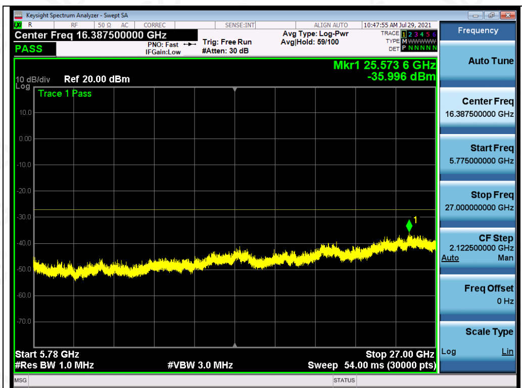
Test_Graph_802.11a_ANT1_5700_6Mbps_Frequency Band 4
