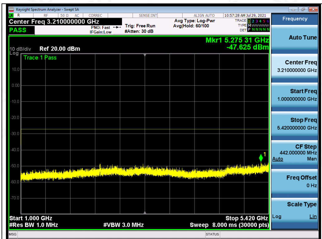
Test_Graph_802.11n40_ANT1_5590_MCS0_Frequency Band 2
