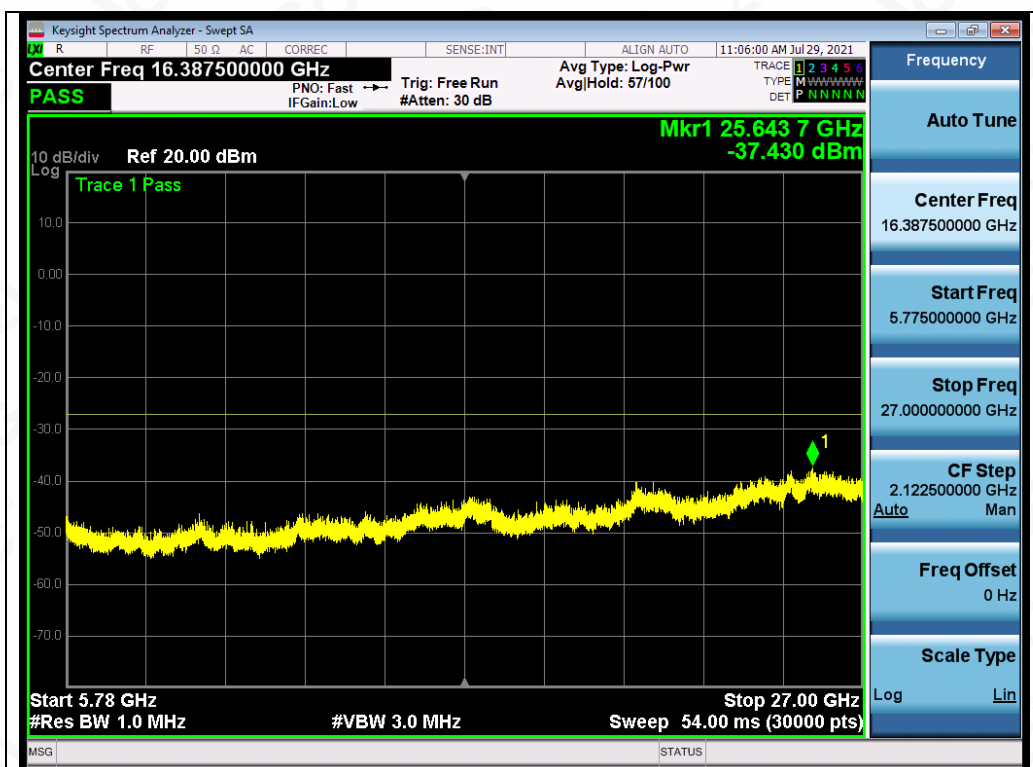
Test_Graph_802.11ac80_ANT1_5530_MCS9_Frequency Band 4
