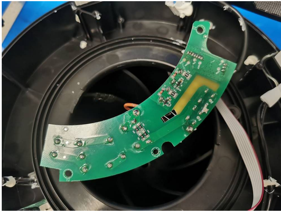
Figure 11. Overview of relay PCB
