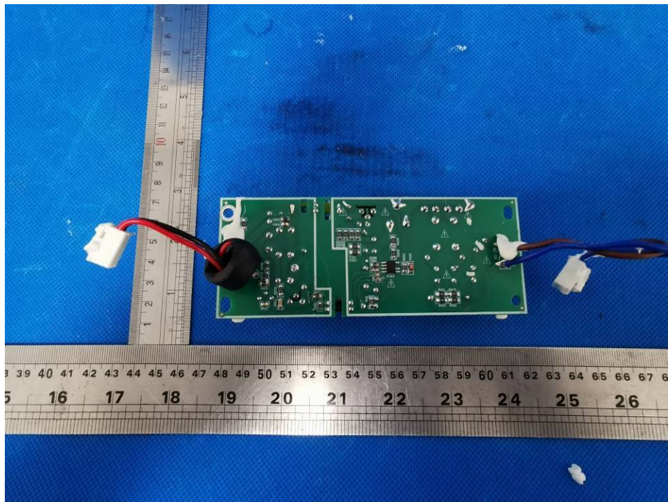
Figure 9. Power PCB
