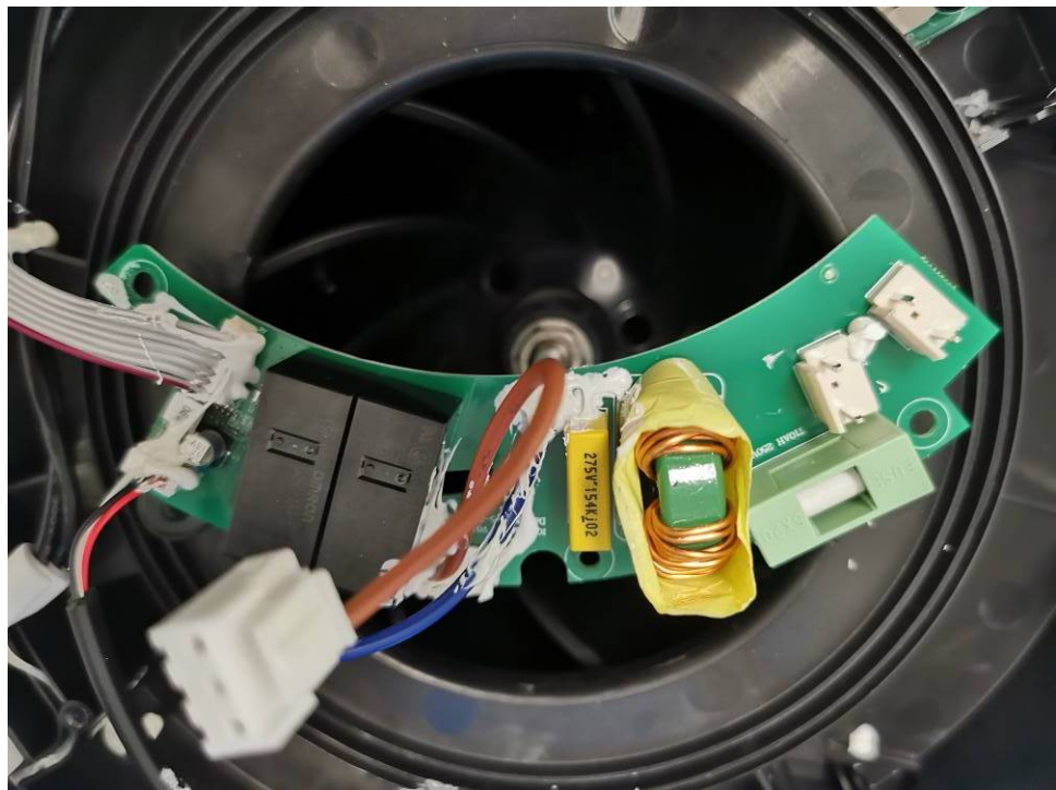
Figure 10. Overview of relay PCB
