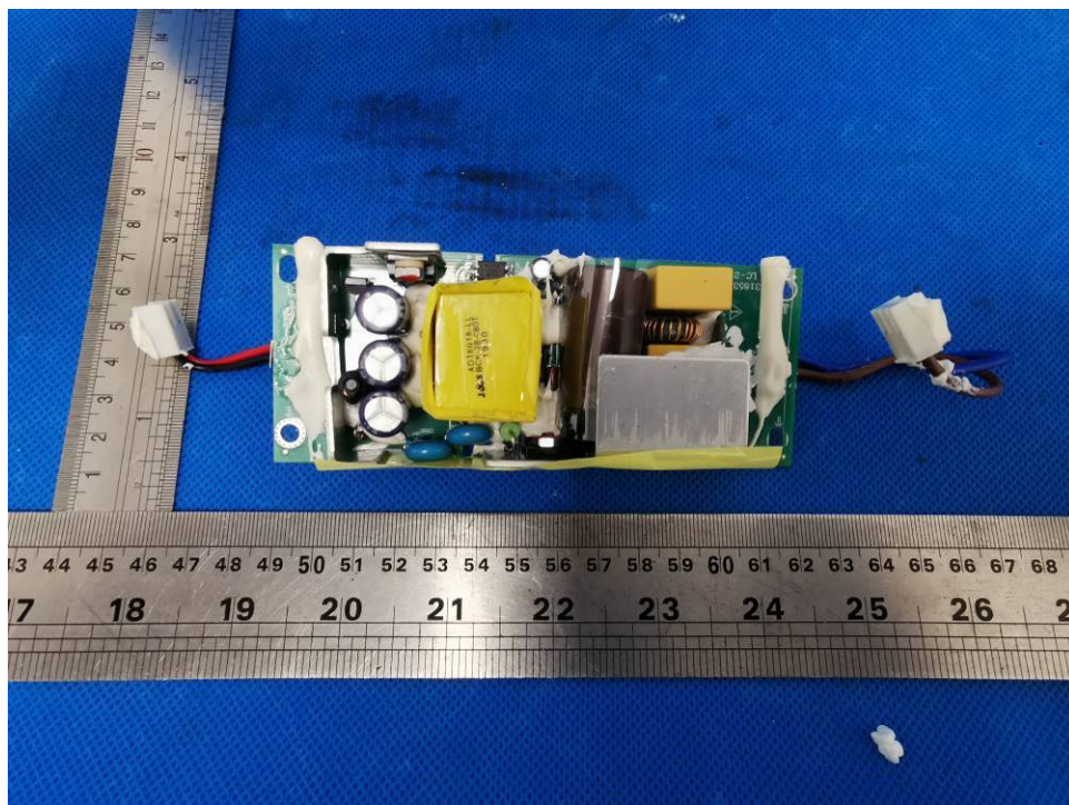
Figure 8. Power PCB
