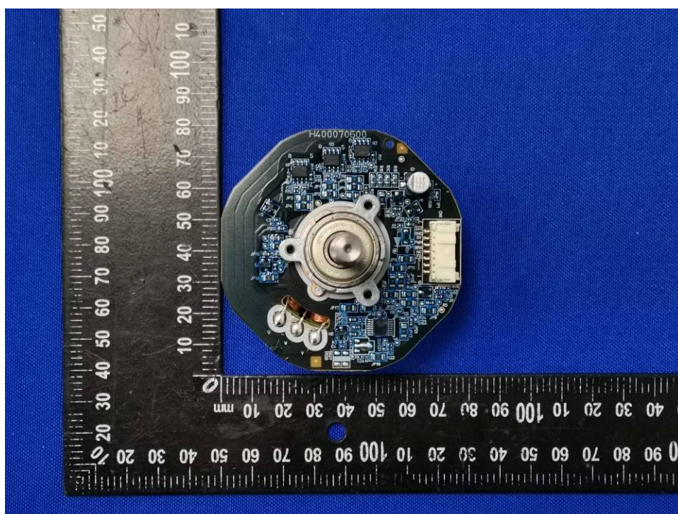
Figure 22. DC motor
