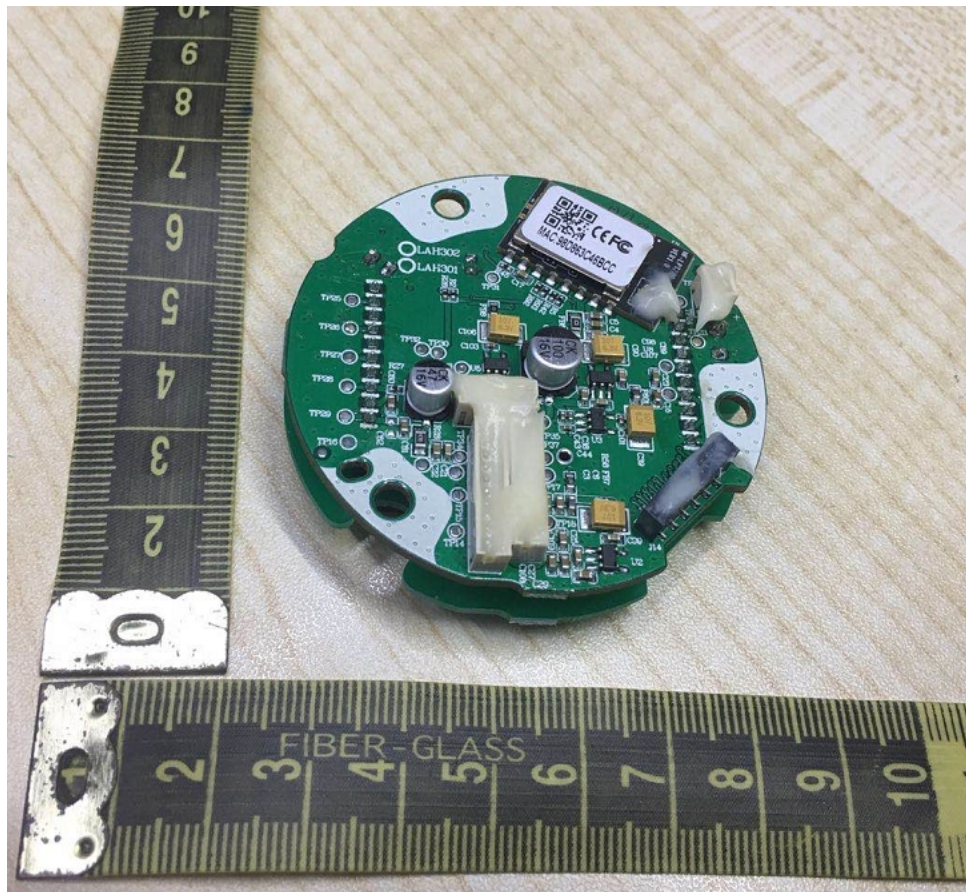
Figure 27. View of display PCB
