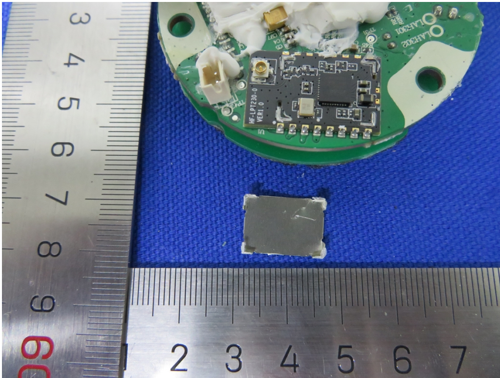
Figure 28. View of Wi-Fi module
