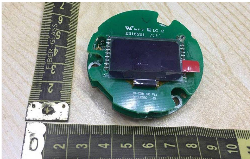
Figure 26. View of display PCB
