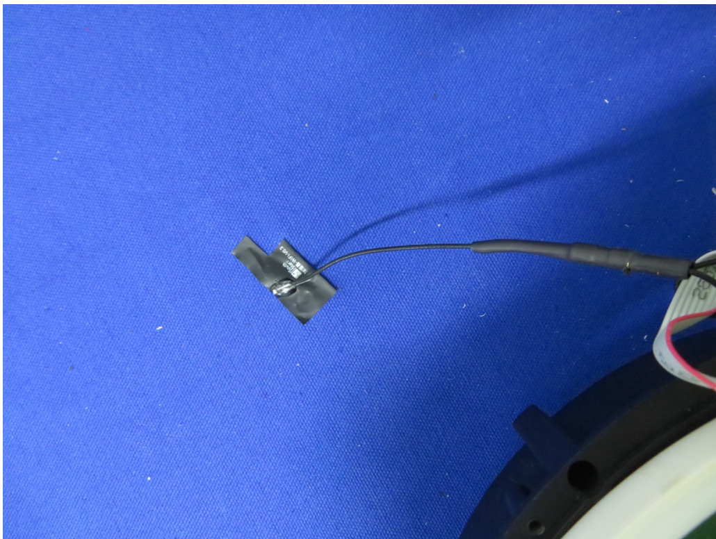
Figure 30. View of Wi-Fi antenna
