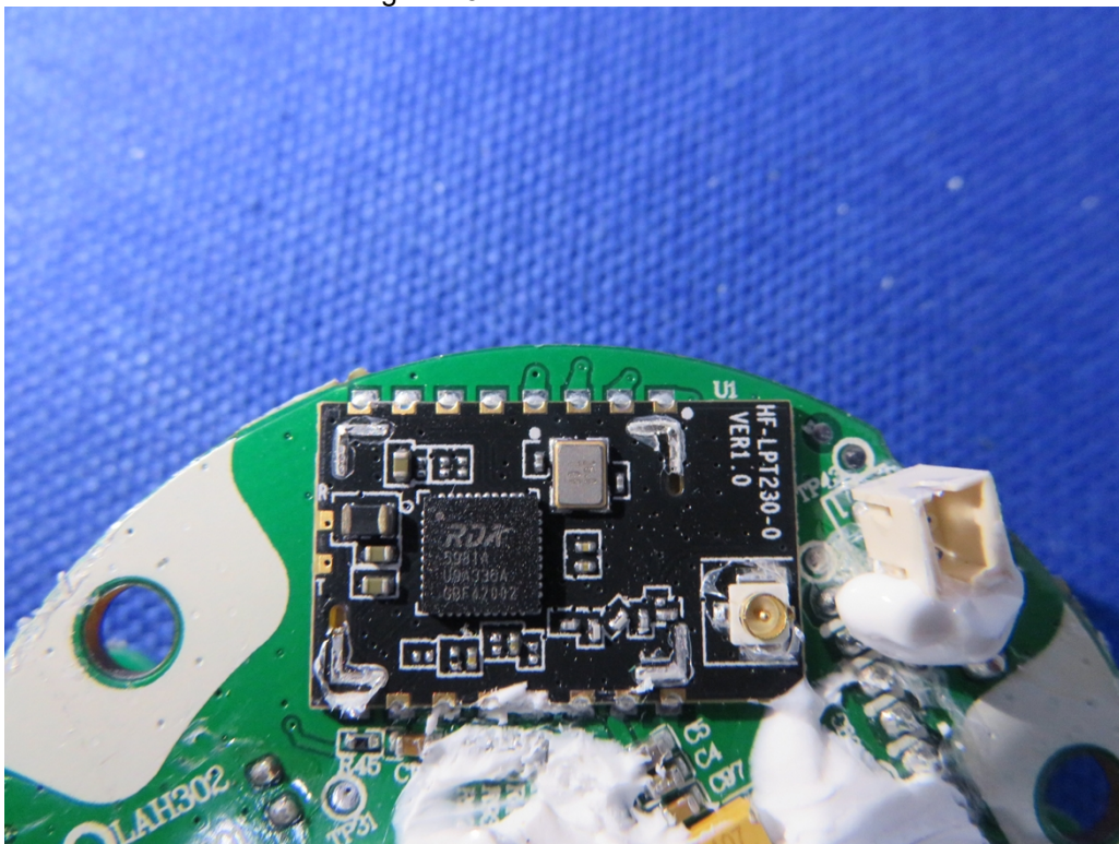
Figure 29. View of Wi-Fi module
