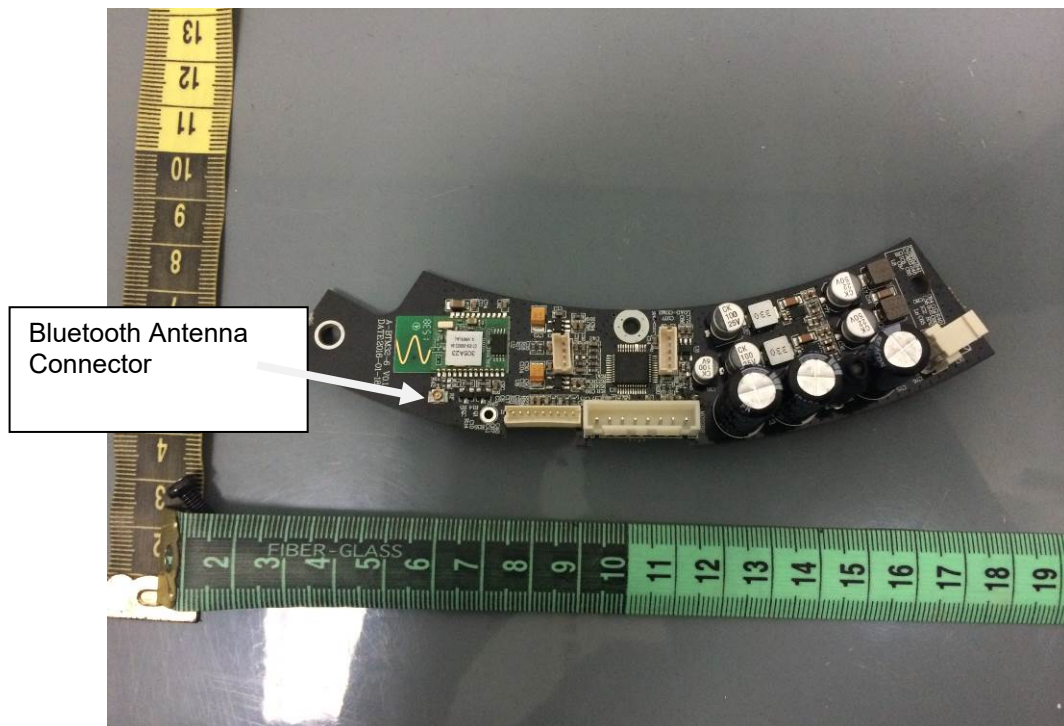
Figure 5. Main PCB of LA503
