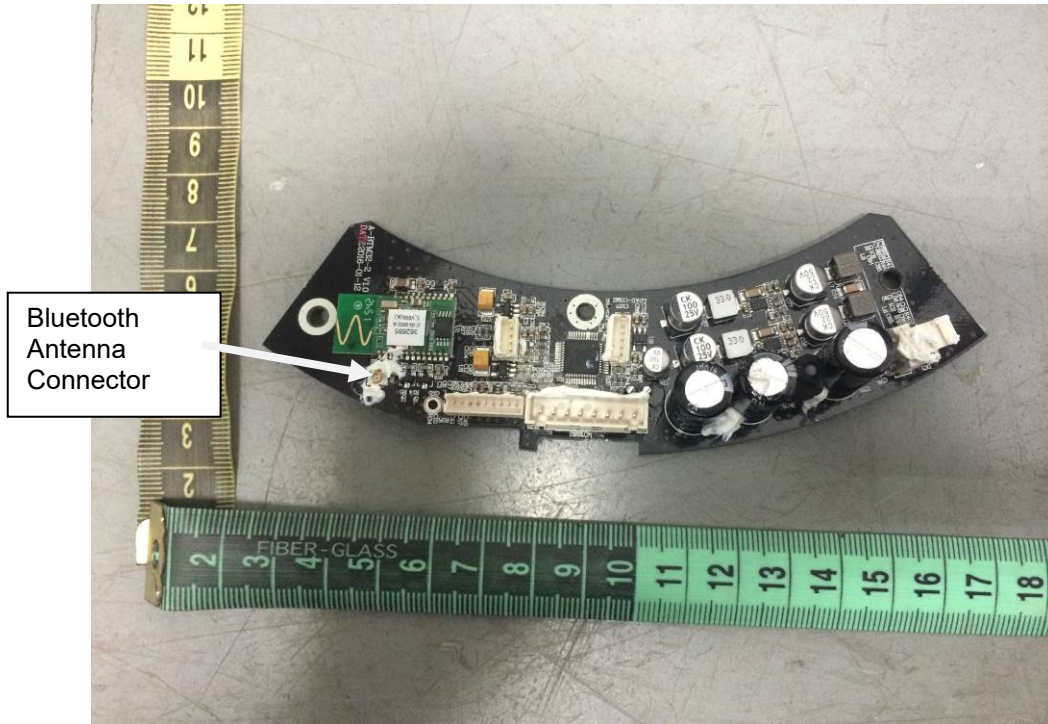
Figure 11. Main PCB of LA333
