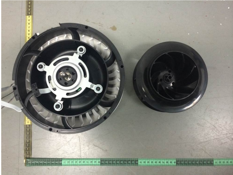
Figure 15. Motor view
