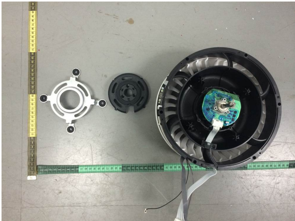
Figure 16. Motor view
