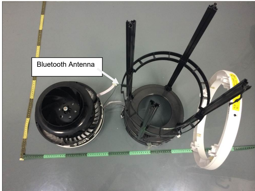
Figure 7. Internal view of LA503
