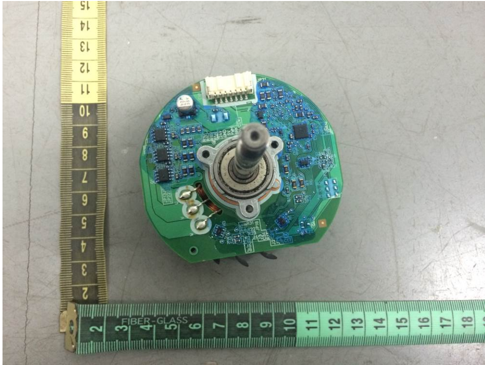
Figure 17. Motor view
