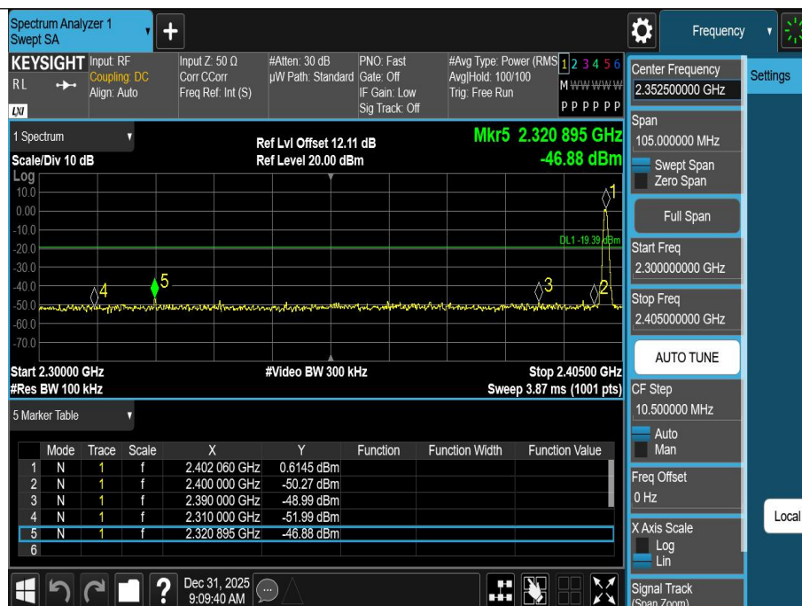
SRD-Ant1-2402-PASS
