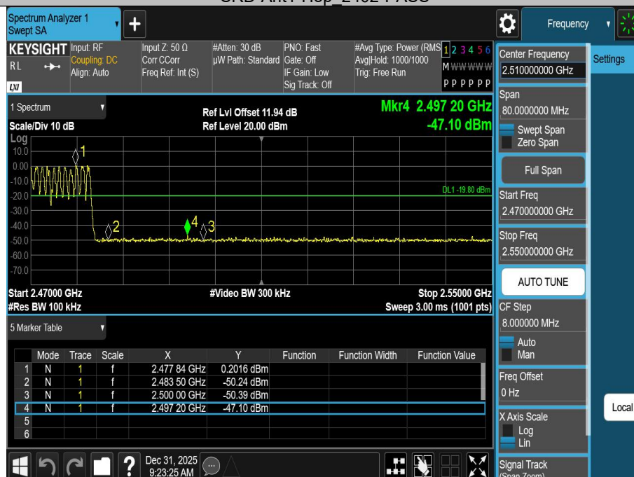
SRD-Ant1-Hop 2480-PASS
