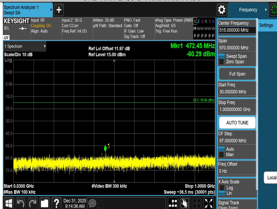
SRD-Ant1-2480-30~1000-PASS
