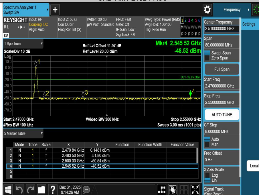
SRD-Ant1-2480-PASS
