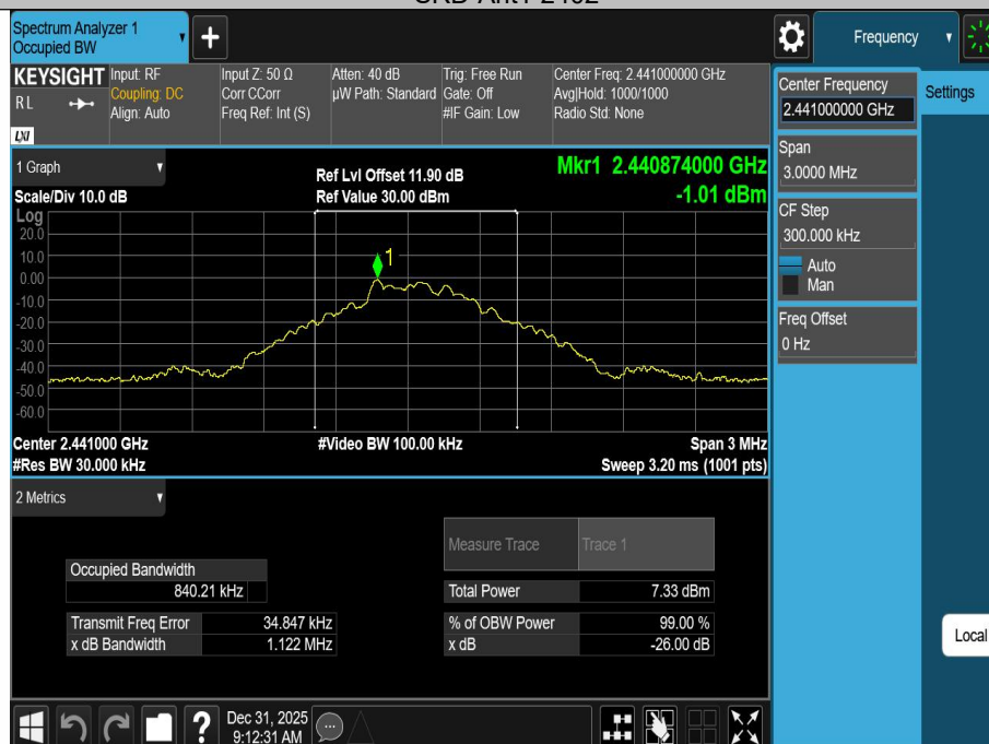
SRD-Ant1-2441
