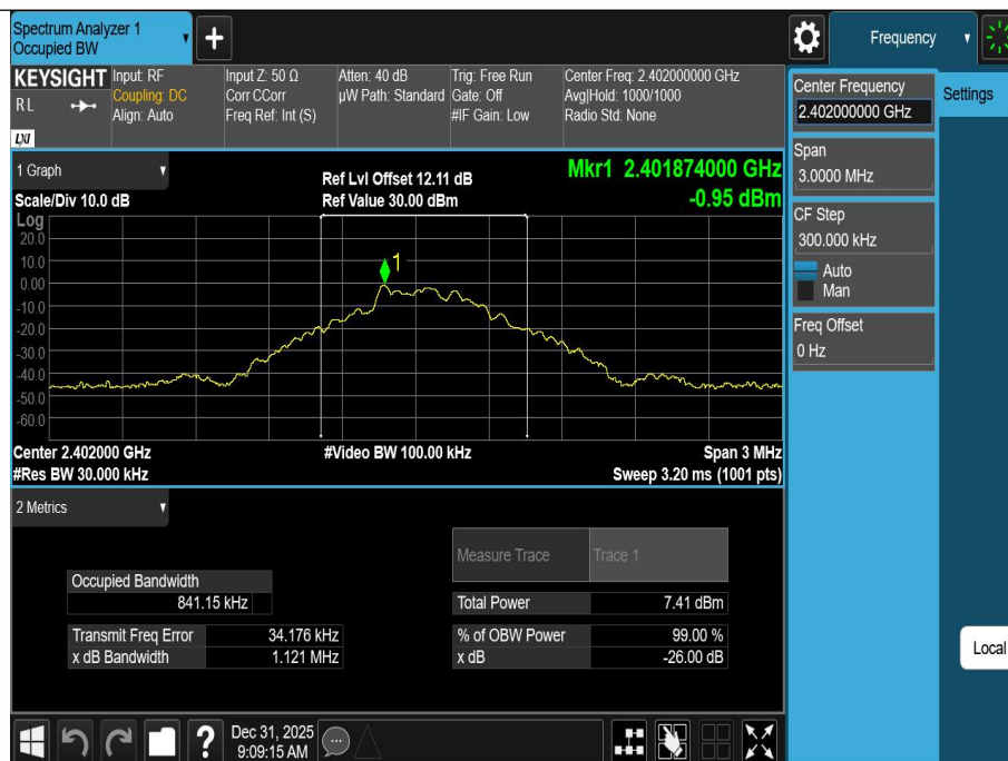
SRD-Ant1-2402
