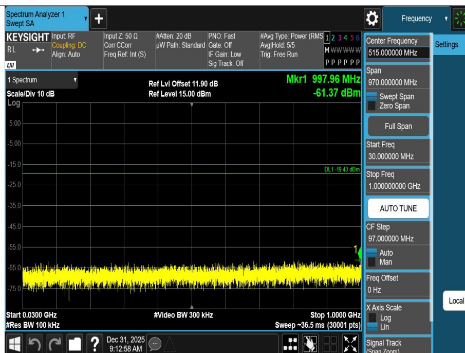
SRD-Ant1-2441-30~1000-PASS
