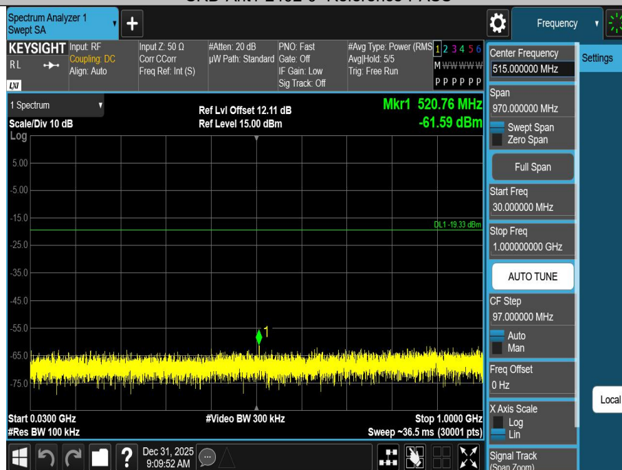
SRD-Ant1-2402-30~1000-PASS
