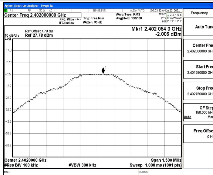
DH5_Ant1_2402_0~Reference
