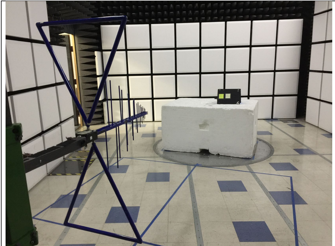
RF Radiated #1: 30-1000 MHz – Front View
