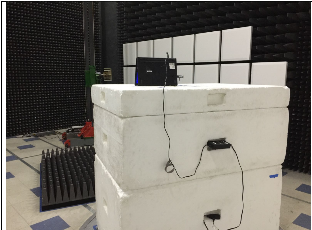
RF Radiated #4: Above 1 GHz – Back View
