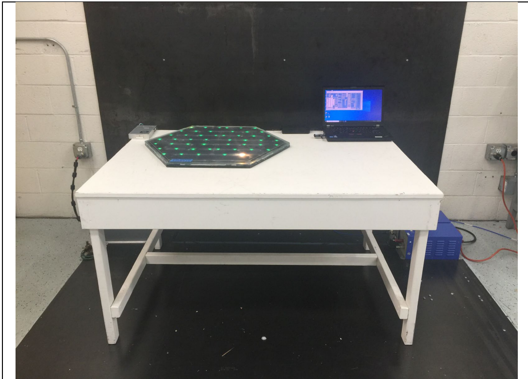
A/C Powerline Conduction #2: Side
