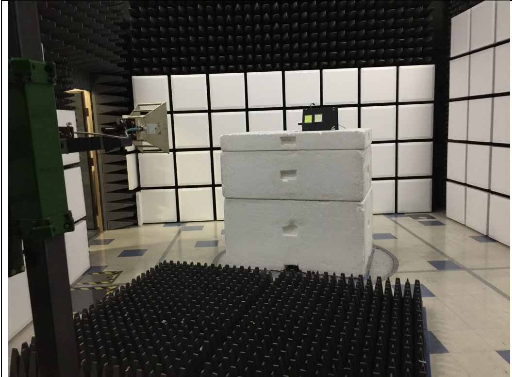
RF Radiated #3: Above 1 GHz – Front View
