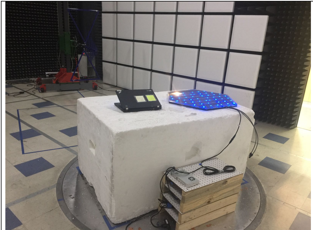
RF Radiated #2: 30-1000 MHz – Back View
