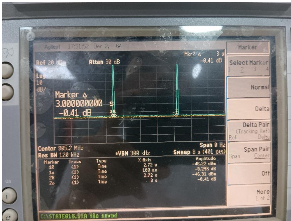
Picture 12.1 Duty factor plot
