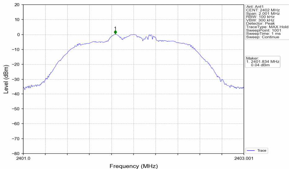
Pi/4DQPSK_2DH5_LCH_2402MHz_Ant1_NTNV
