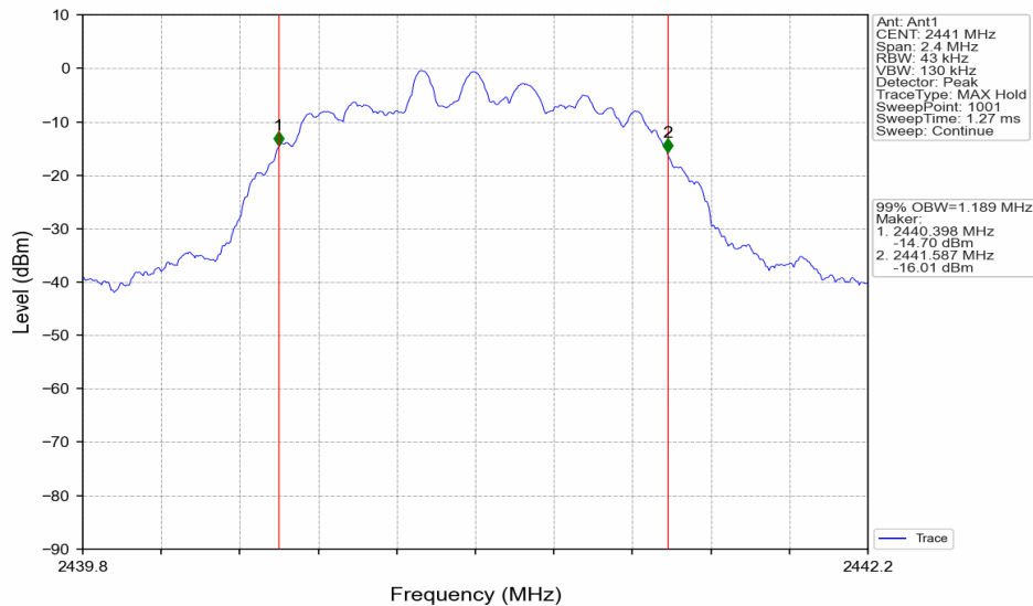
8DPSK_3DH5_MCH_2441MHz_Ant1_NTNV
