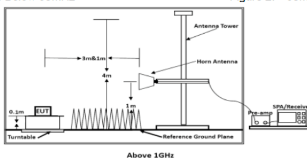
Figure 3. Above 1GHz
