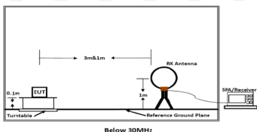
Figure 1. Below 30MHz
