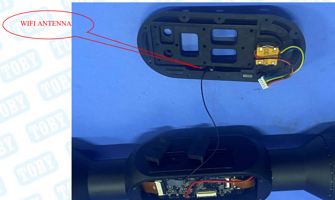
Photo 11 Appearance of PCB
