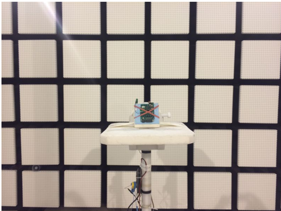
Photo 2: RSE setup < 30 MHz and > 1GHz
