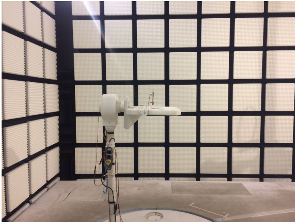
Photo 1: RSE setup < 30 MHz and > 1GHz
