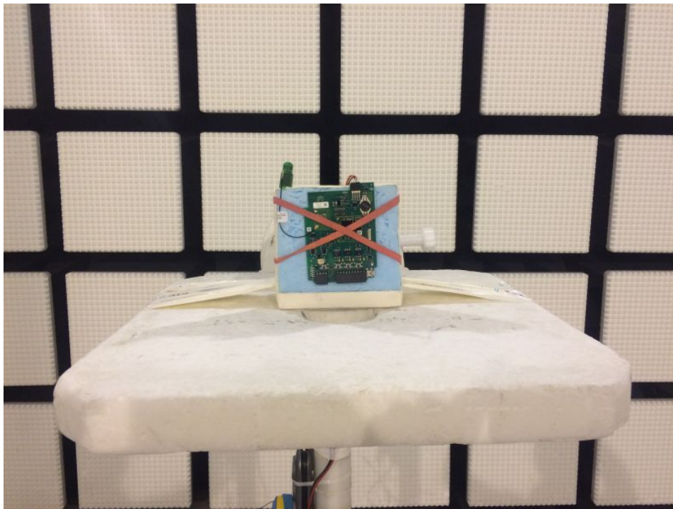
Photo 3: RSE setup < 30 MHz and > 1GHz
