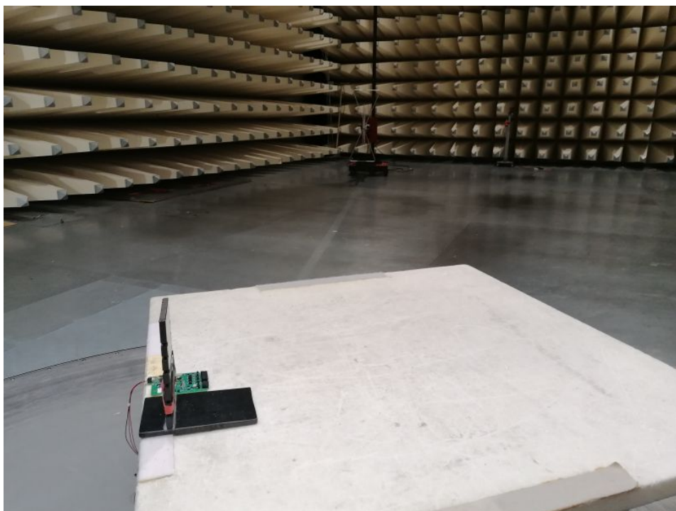
Photo 6: RSE setup 30MHz to 1GHz
