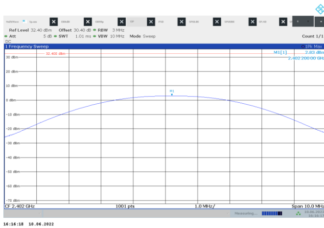
Figure 8.5-1: Output power on low channel
