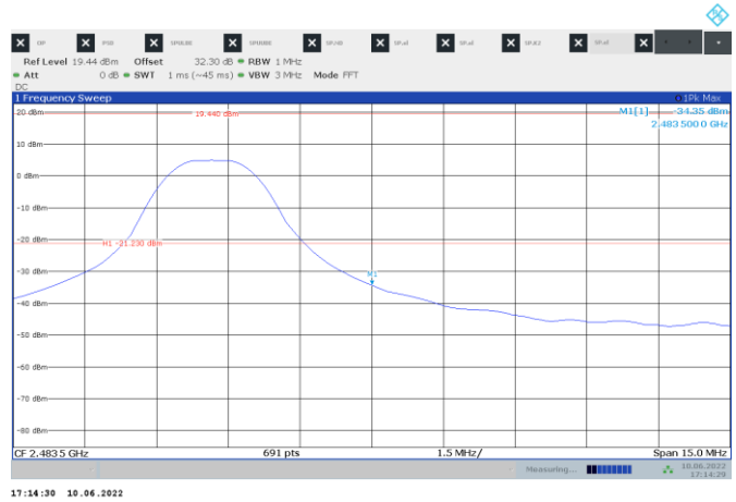
Figure 8.6-7: Conducted EIRP spurious emissions at band edge within restricted band, TX on High channel, Peak
