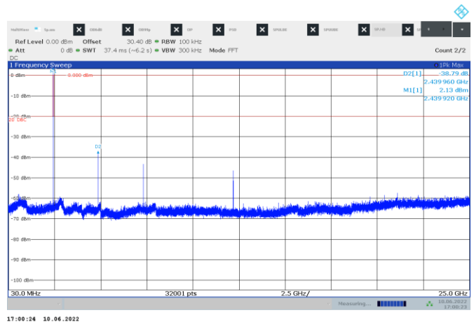
Figure 8.6-4: Conducted spurious emissions outside restricted band, TX on Mid channel
