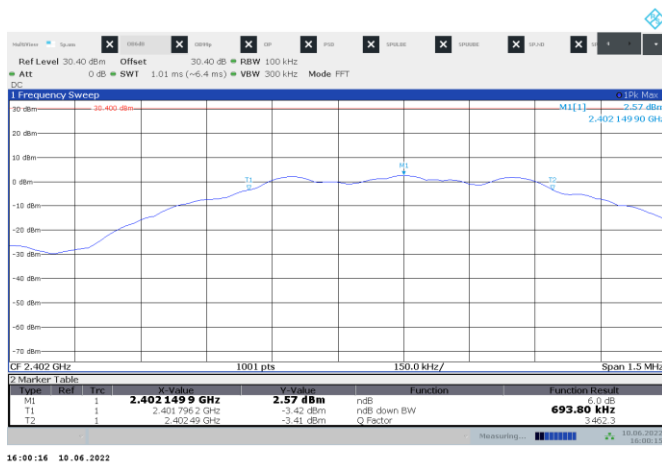
Figure 8.4-1: 6 dB bandwidth on BLE, Tx low channel
