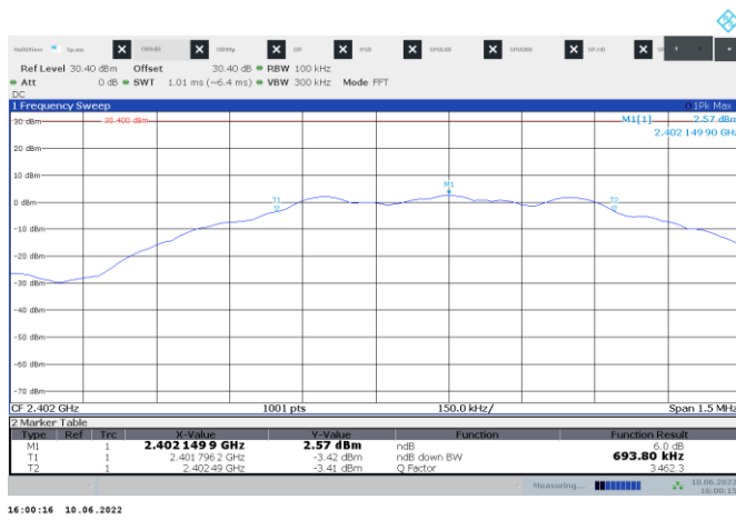
Figure 8.7-1: PSD on low channel
