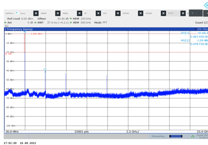
Figure 8.6-5: Conducted spurious emissions outside restricted band, TX on High channel
