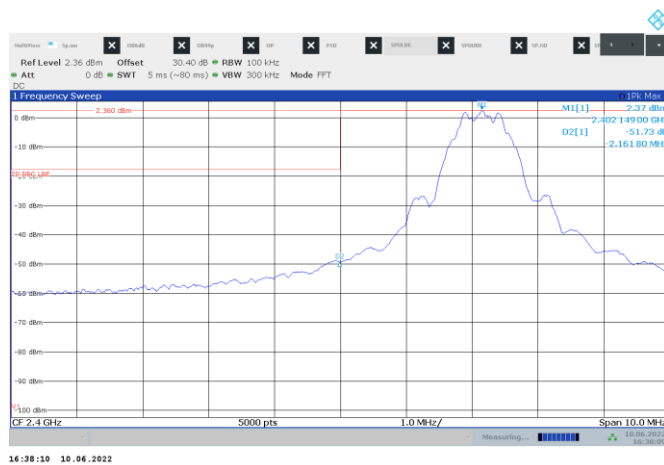
Figure 8.6-1: Conducted spurious emission at band edge outside restricted band, TX on low channel
