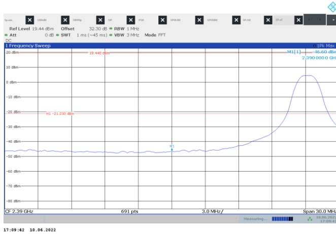
Figure 8.6-6: Conducted EIRP spurious emission at band edge within restricted band, TX on low channel, Peak
