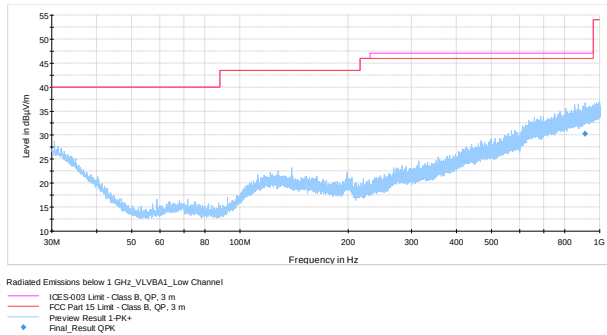
Figure 8.6-8: Radiated spurious emissions 30 MHz to 1 GHz, Low channel
