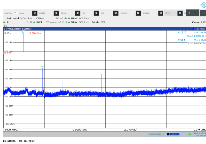
Figure 8.6-3: Conducted spurious emissions outside restricted band, TX on Low channel
