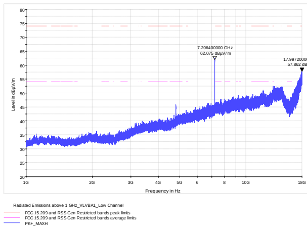
Figure 8.6-10: Radiated spurious emissions 1 GHz to 18 GHz, Low channel
