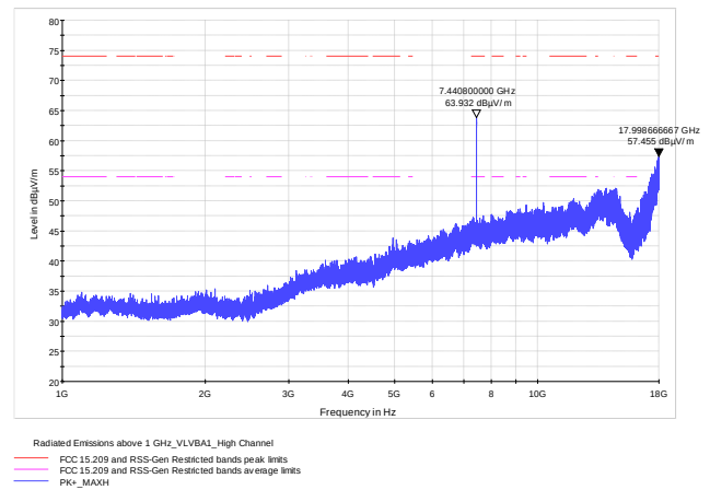
Figure 8.6-11: Radiated spurious emissions 1 GHz to 18 GHz, High channel
