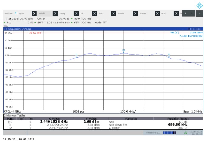
Figure 8.7-2: PSD on mid channel
