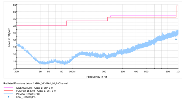
Figure 8.6-9: Radiated spurious emissions 30 MHz to 1 GHz, High channel
