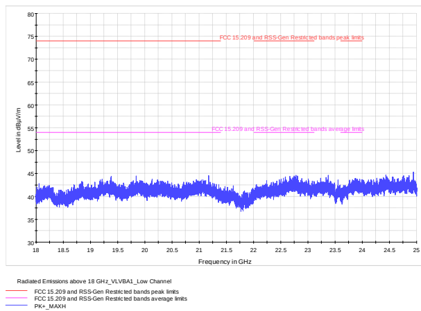
Figure 8.6-12: Radiated spurious emissions 18 GHz to 25 GHz, Low channel
