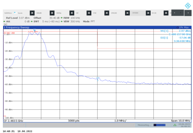
Figure 8.6-2: Conducted spurious emissions at band edge outside restricted band, TX on High channel
