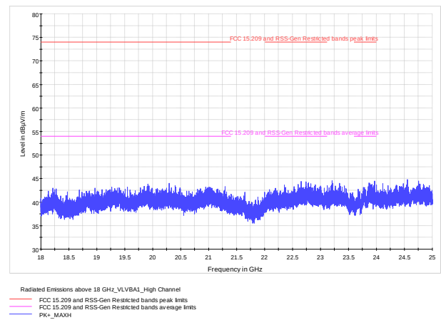
Figure 8.6-13: Radiated spurious emissions 18 GHz to 25 GHz, High channel
