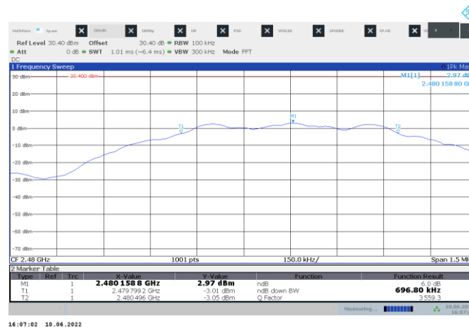
Figure 8.7-3: PSD on high channel
