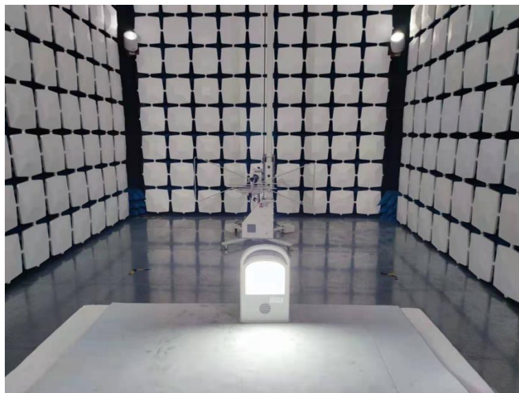
Above 1GHz for radiated emission test setup
