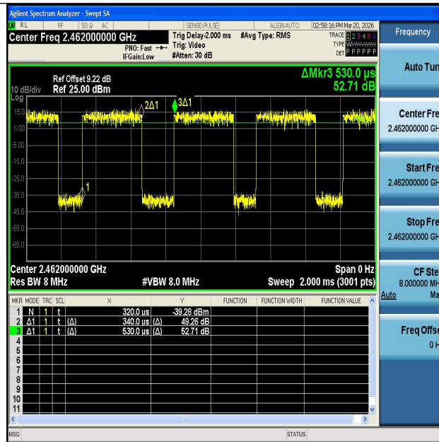
NTNV-11AX20SISO-Ant1-2462
