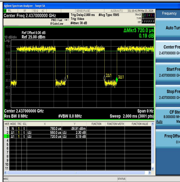
NTNV-11N20SISO-Ant1-2437
