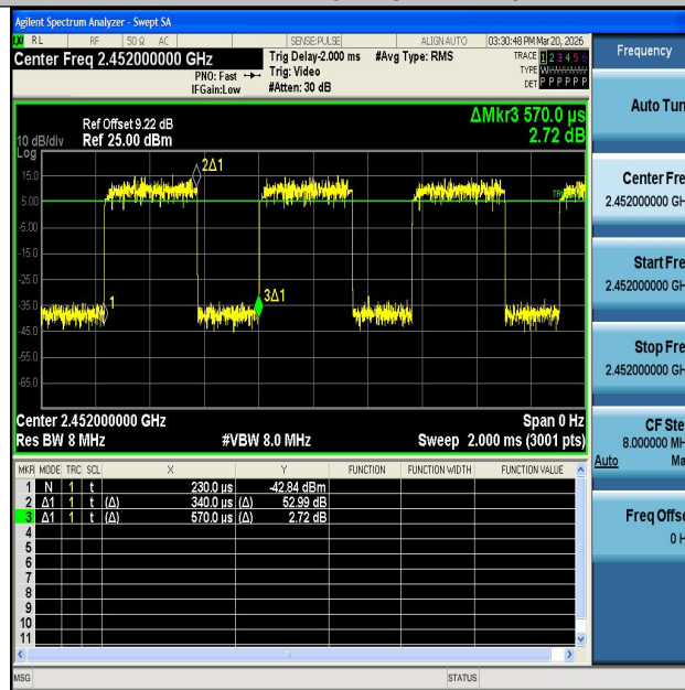
NTNV-11AX40SISO-Ant1-2452
