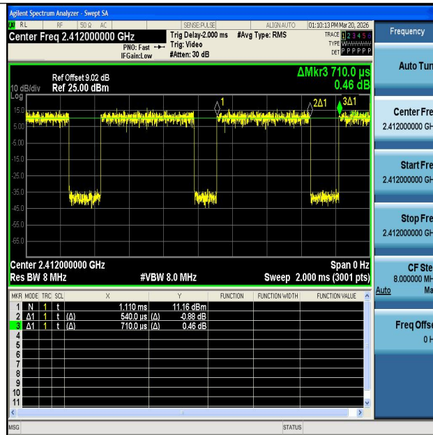
NTNV-11N20SISO-Ant1-2412
