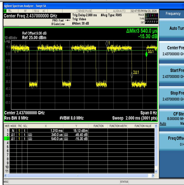
NTNV-11AX20SISO-Ant1-2437
