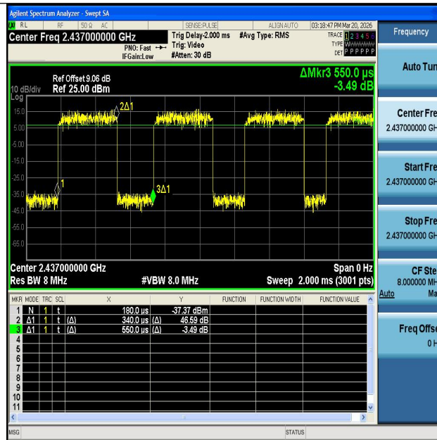
NTNV-11AX40SISO-Ant1-2437
