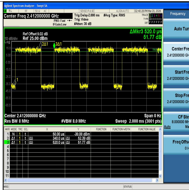
NTNV-11AX20SISO-Ant1-2412
