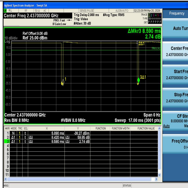
NTNV-11B-Ant1-2437
