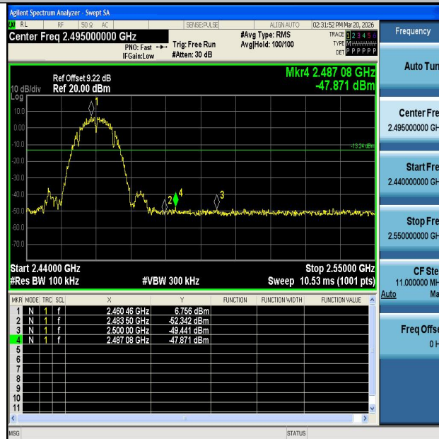
11B-Ant1-2462-PASS
