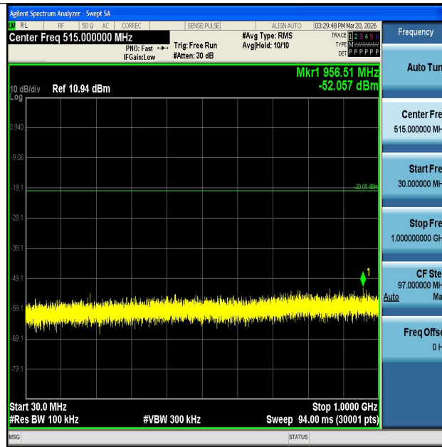
11AX40SISO-Ant1-2437-30~1000-PASS
