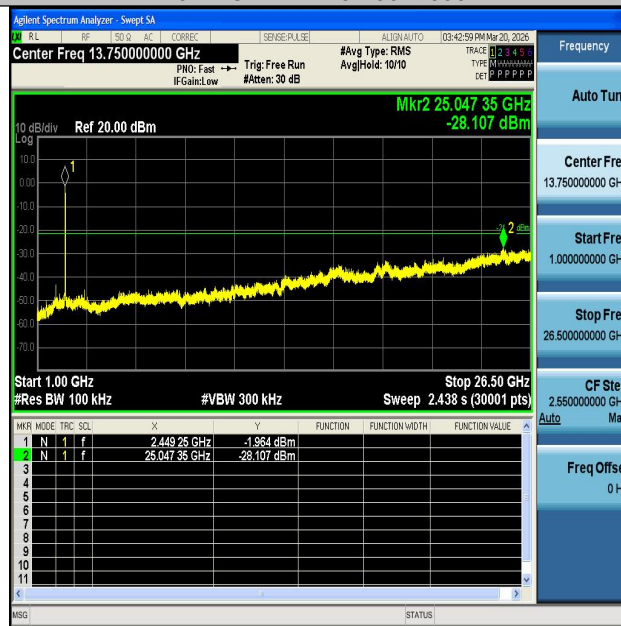
11AX40SISO-Ant1-2452-1000~26500-PASS
