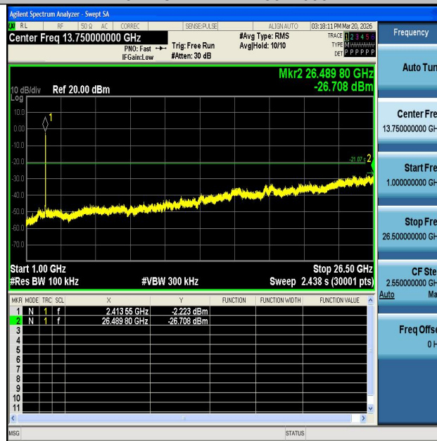
11AX40SISO-Ant1-2422-1000~26500-PASS
