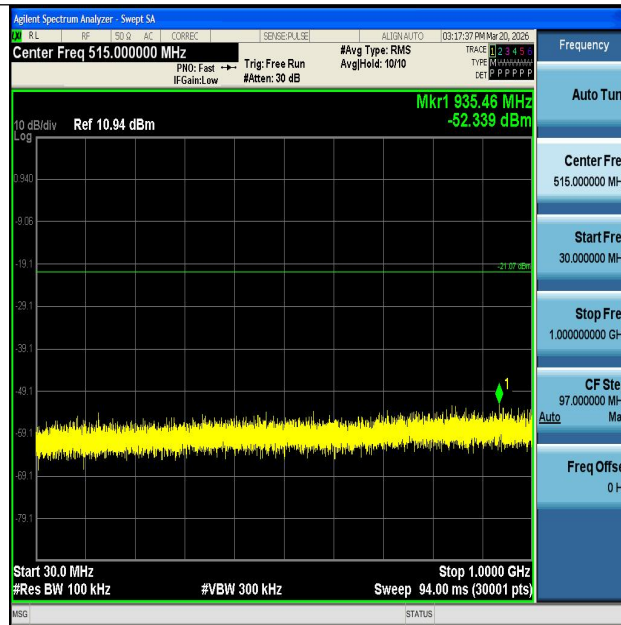
11AX40SISO-Ant1-2422-30~1000-PASS
