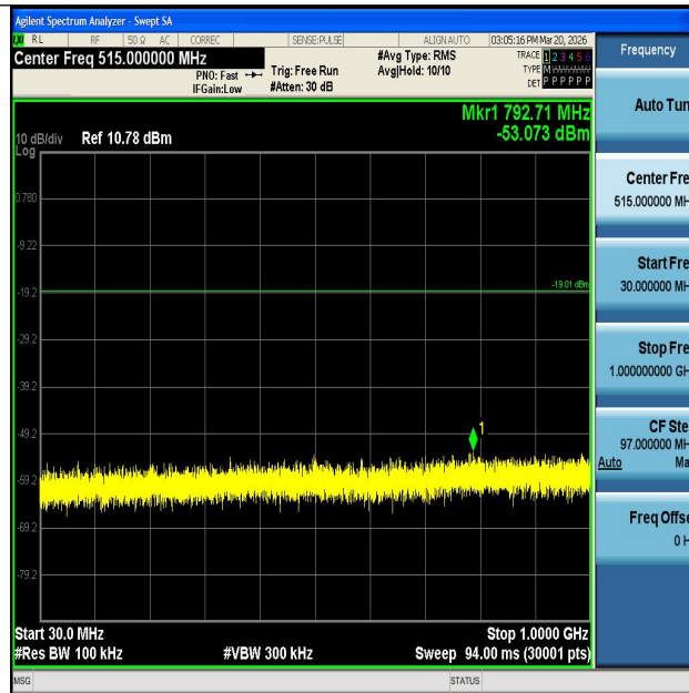
11AX20SISO-Ant1-2462-30~1000-PASS
