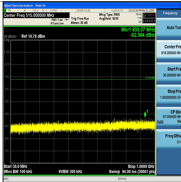
11AX40SISO-Ant1-2452-30~1000-PASS
