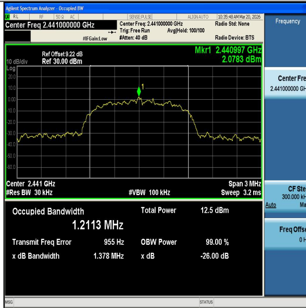
3DH5-Ant1-2441
