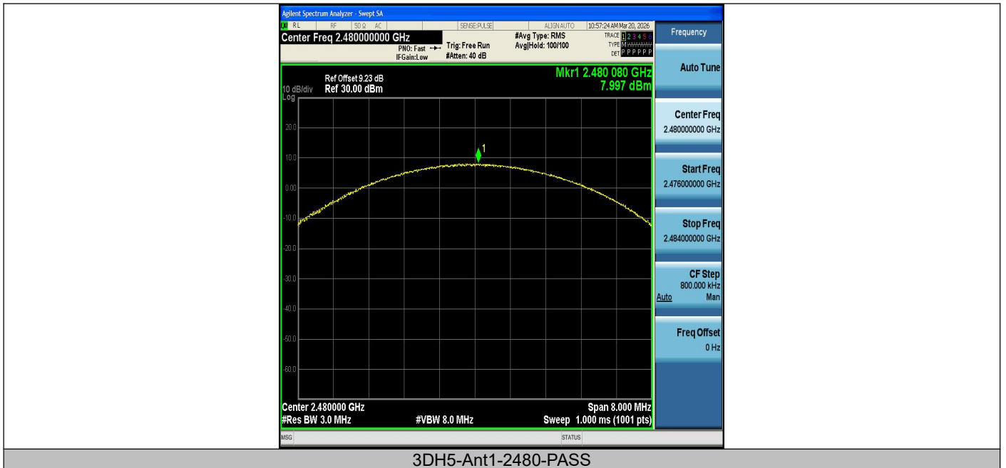
3DH5-Ant1-2480-PASS
