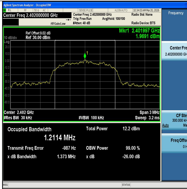
3DH5-Ant1-2402
