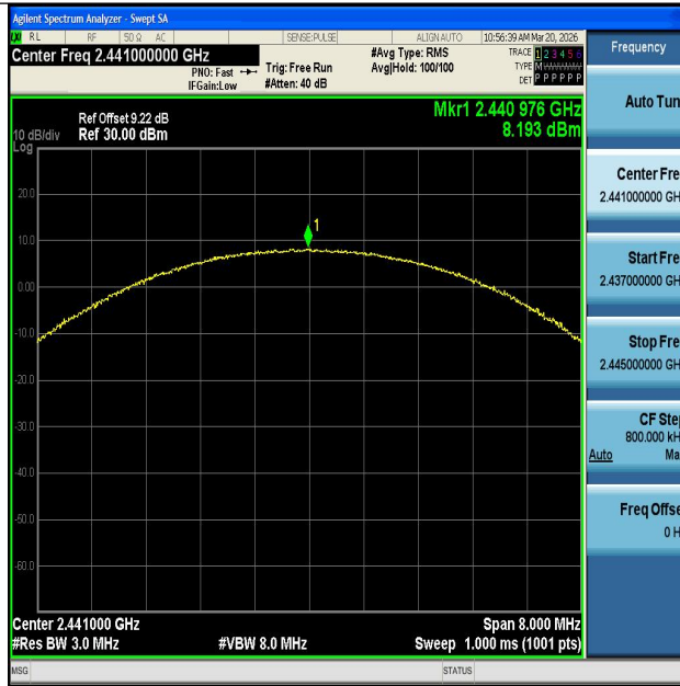
2DH5-Ant1-2441-PASS
