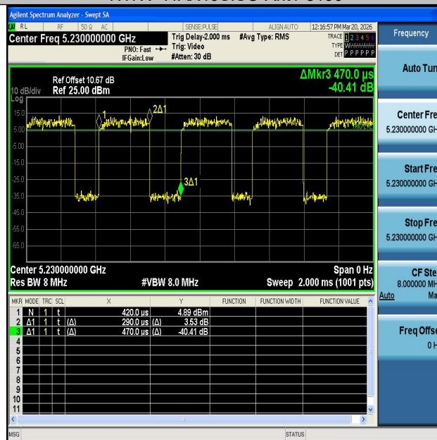
NTNV-11AX40SISO-Ant1-5230
