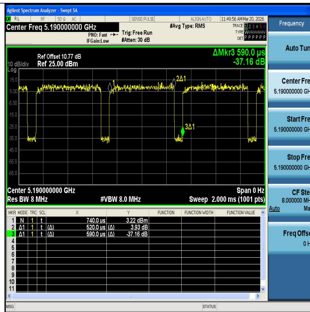
NTNV-11N40SISO-Ant1-5190
