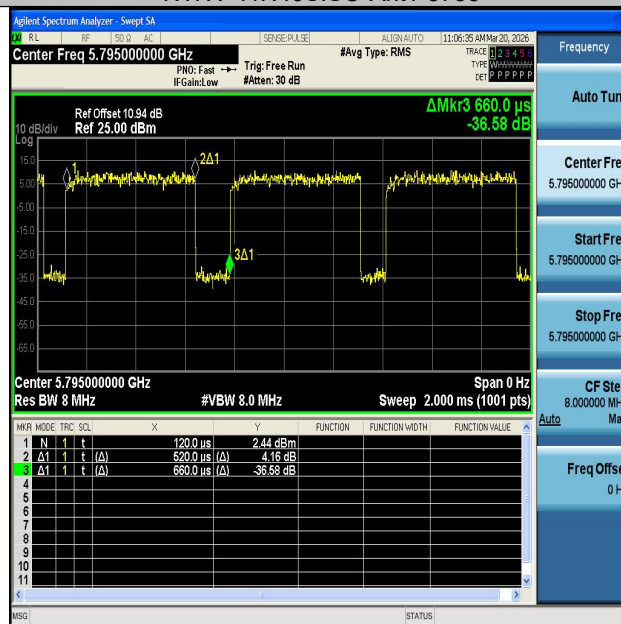
NTNV-11N40SISO-Ant1-5795
