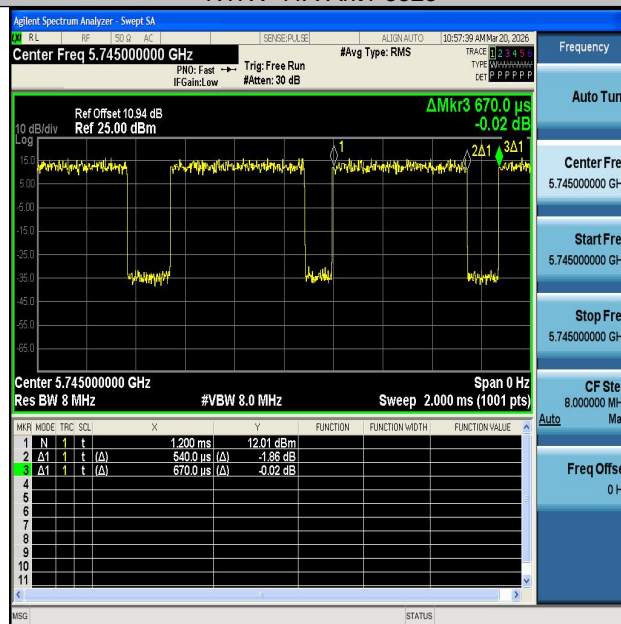
NTVN-11N20SISO-Ant1-5745
