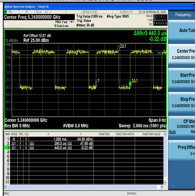
NTNV-11AX20SISO-Ant1-5240
