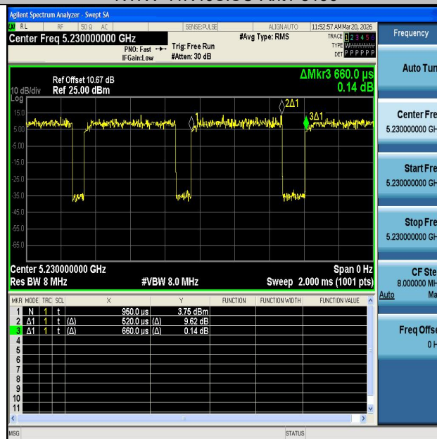
NTNV-11N40SISO-Ant1-5230
