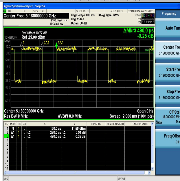
NTNV-11AX20SISO-Ant1-5180
