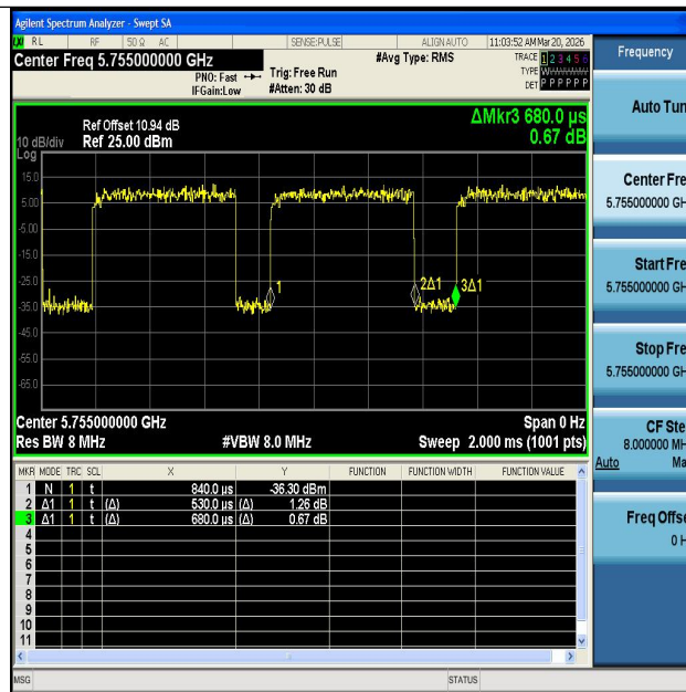
NTNV-11N40SISO-Ant1-5755
