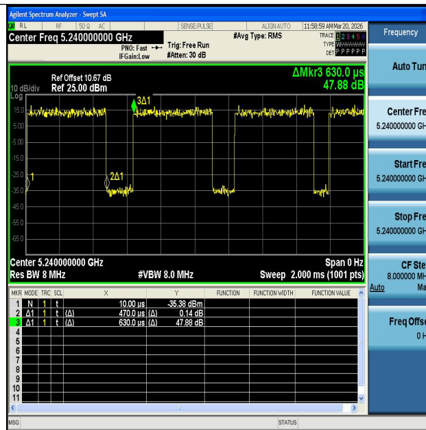
NTNV-11AC20SISO-Ant1-5240
