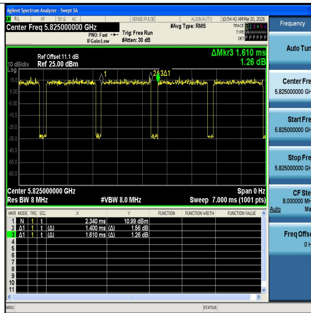
NTVN-11A-Ant1-5825
