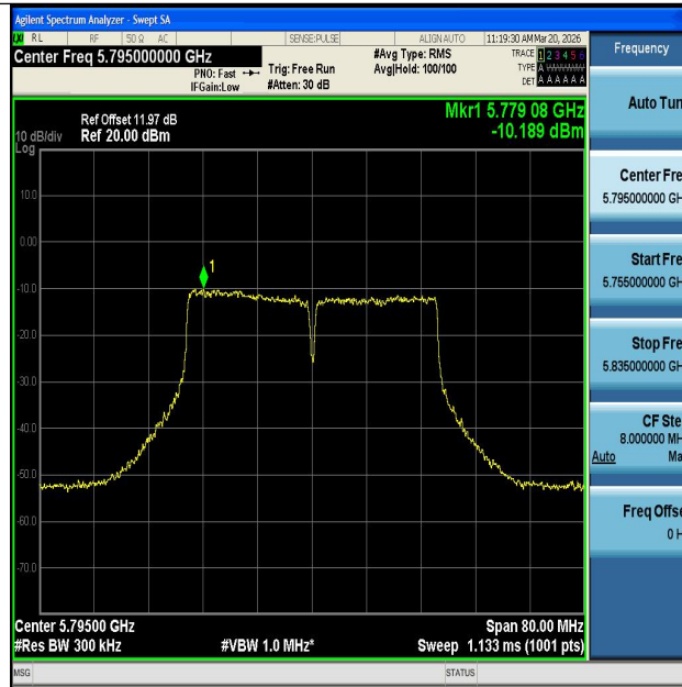
11AC40SISO-Ant1-5795-PASS
