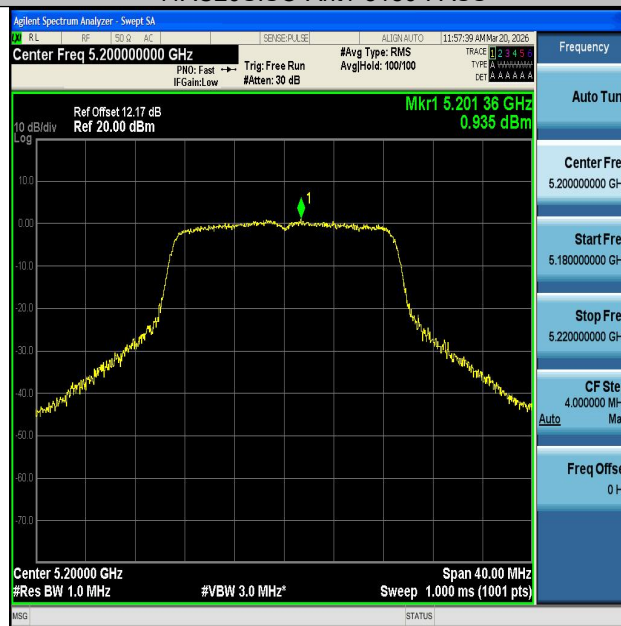
11AC20SISO-Ant1-5200-PASS
