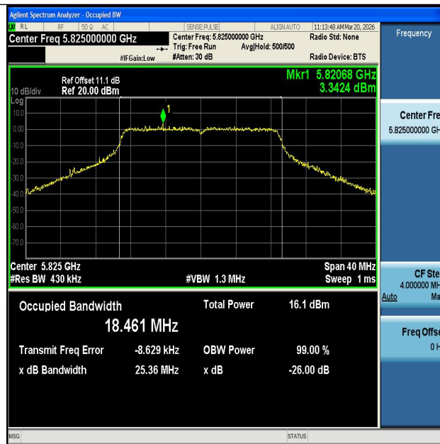
11AC20SISO-Ant1-5825
