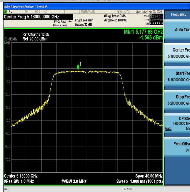
11N20SISO-Ant1-5180-PASS
