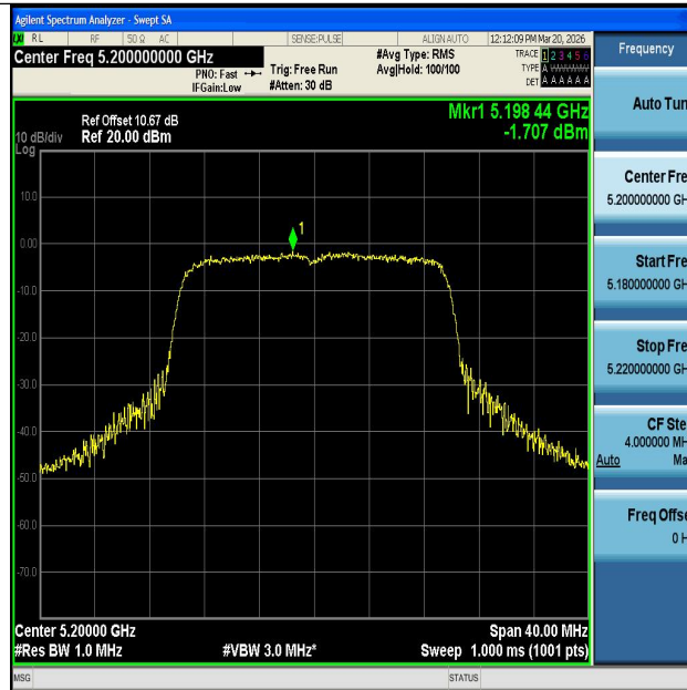
11AX20SISO-Ant1-5200-PASS
