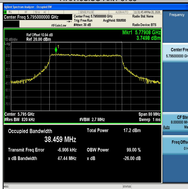
11AX40SISO-Ant1-5795
