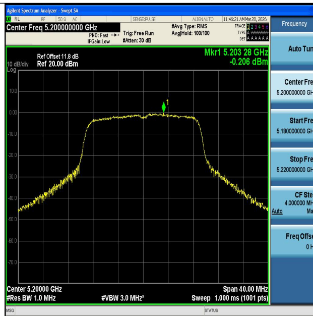
11N20SISO-Ant1-5200-PASS
