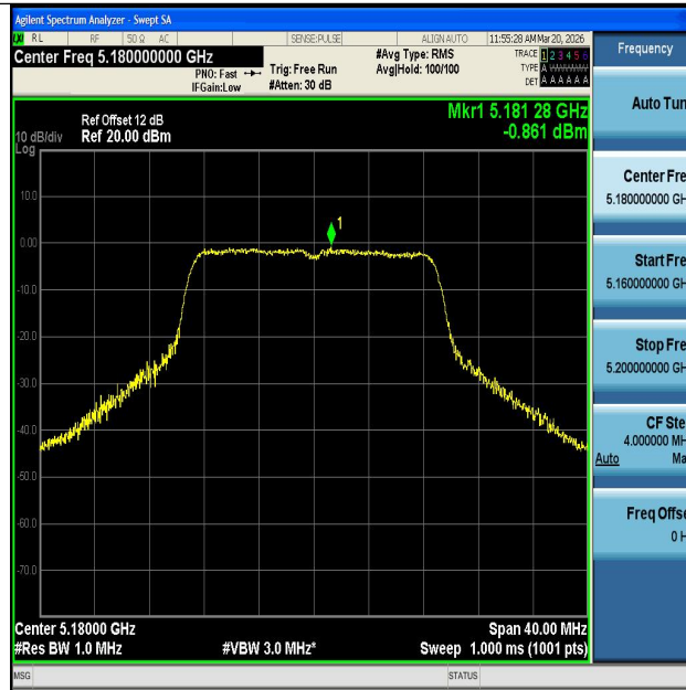
11AC20SISO-Ant1-5180-PASS
