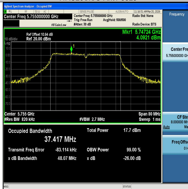
11AC40SISO-Ant1-5755
