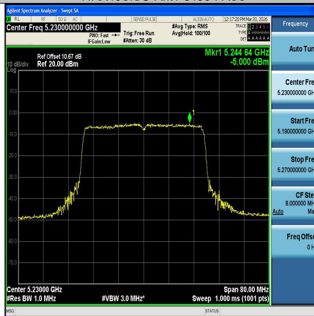
11AX40SISO-Ant1-5230-PASS
