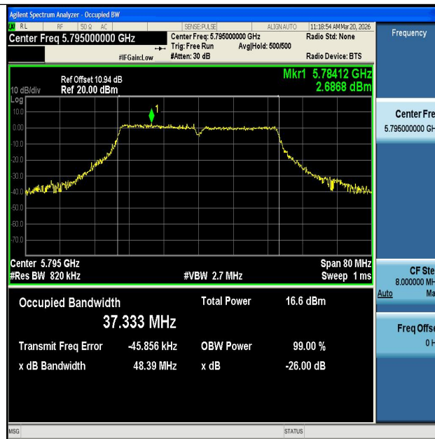
11AC40SISO-Ant1-5795
