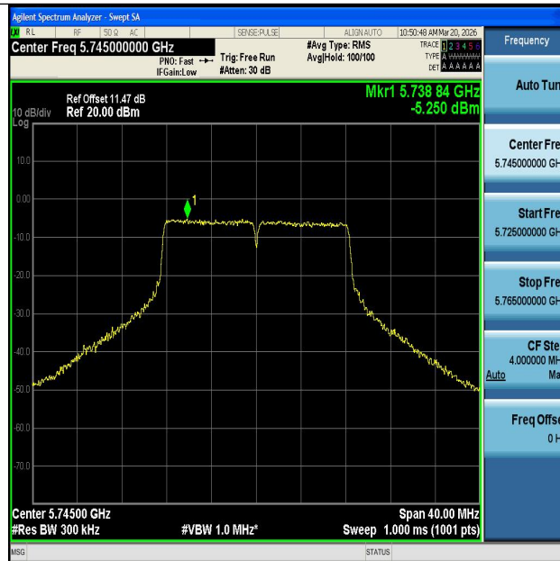
11A-Ant1-5745-PASS
