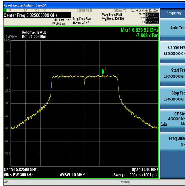
11AC20SISO-Ant1-5825-PASS
