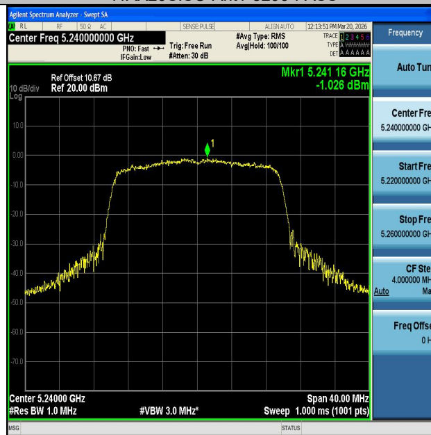
11AX20SISO-Ant1-5240-PASS
