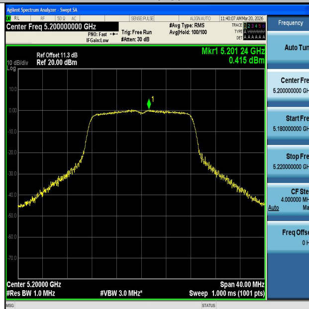
11A-Ant1-5200-PASS
