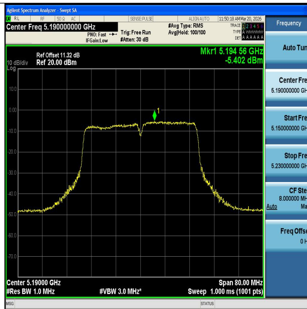
11N40SISO-Ant1-5190-PASS
