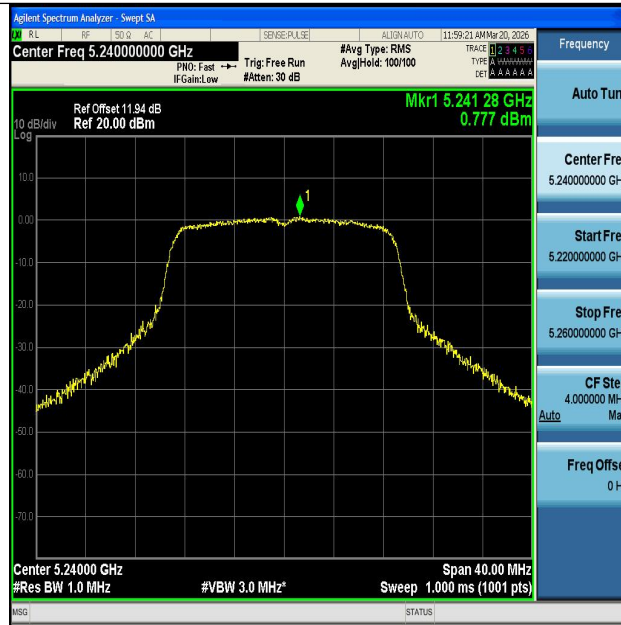
11AC20SISO-Ant1-5240-PASS
