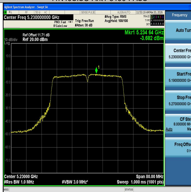
11N40SISO-Ant1-5230-PASS
