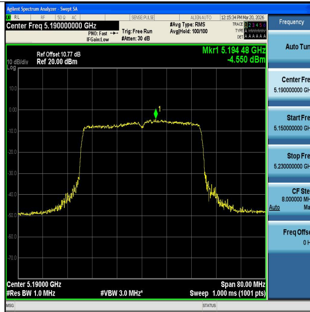
11AX40SISO-Ant1-5190-PASS
