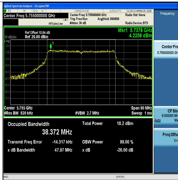
11AX40SISO-Ant1-5755
