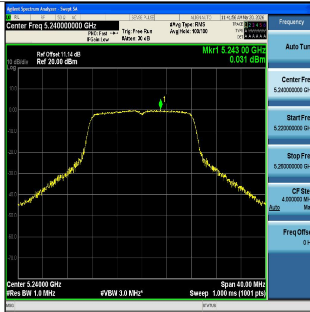
11A-Ant1-5240-PASS
