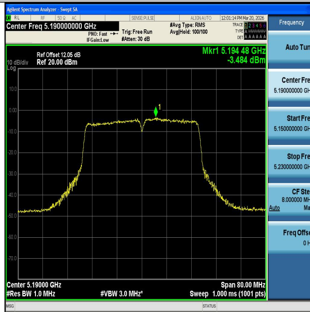
11AC40SISO-Ant1-5190-PASS
