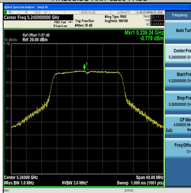
11N20SISO-Ant1-5240-PASS
