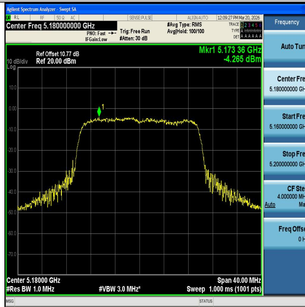
11AX20SISO-Ant1-5180-PASS
