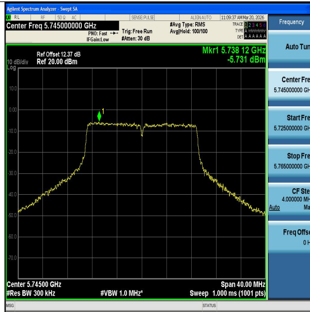
11AC20SISO-Ant1-5745-PASS
