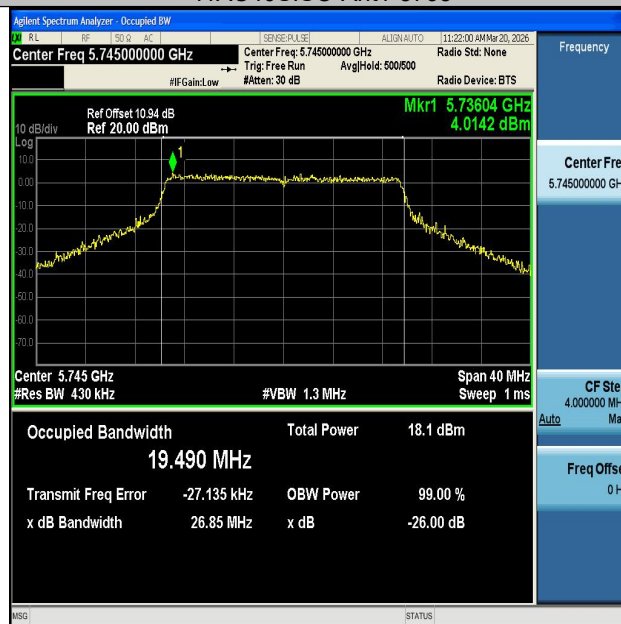
11AX20SISO-Ant1-5745
