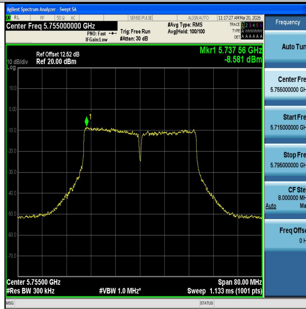
11AC40SISO-Ant1-5755-PASS
