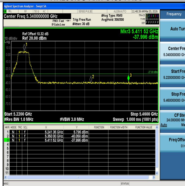
11N20SISO-Ant1-5240-PASS
