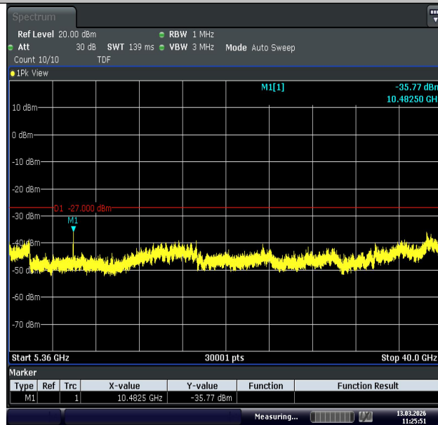
11A-Ant1-5240-5360~40000-PASS
