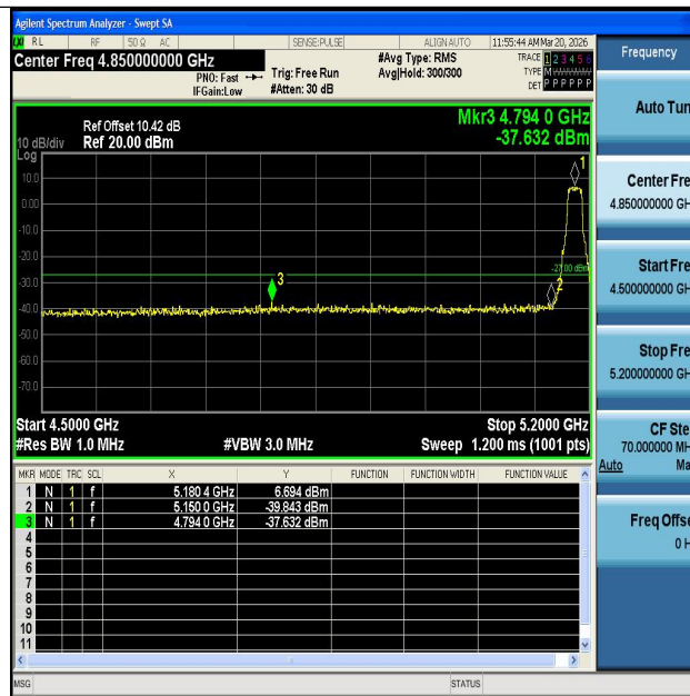
11AC20SISO-Ant1-5180-PASS
