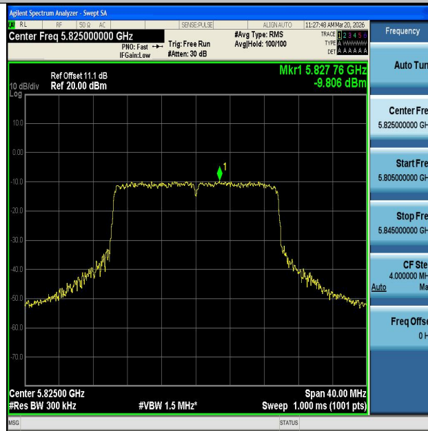
11AX20SISO-Ant1-5825-PASS
