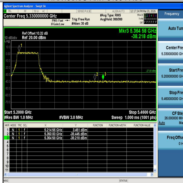
11AX40SISO-Ant1-5230-PASS
