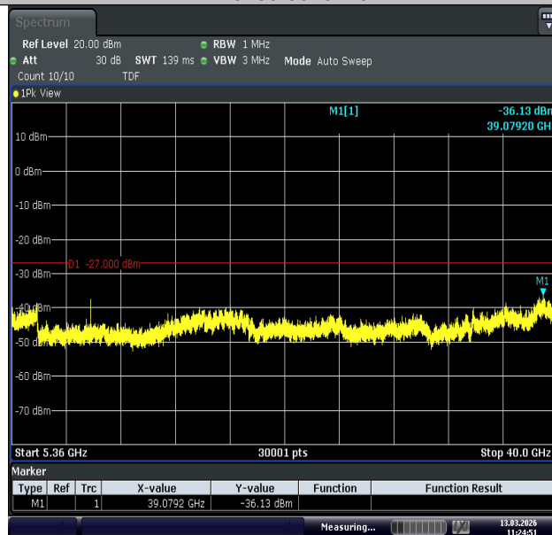
11A-Ant1-5180-5360~40000-PASS
