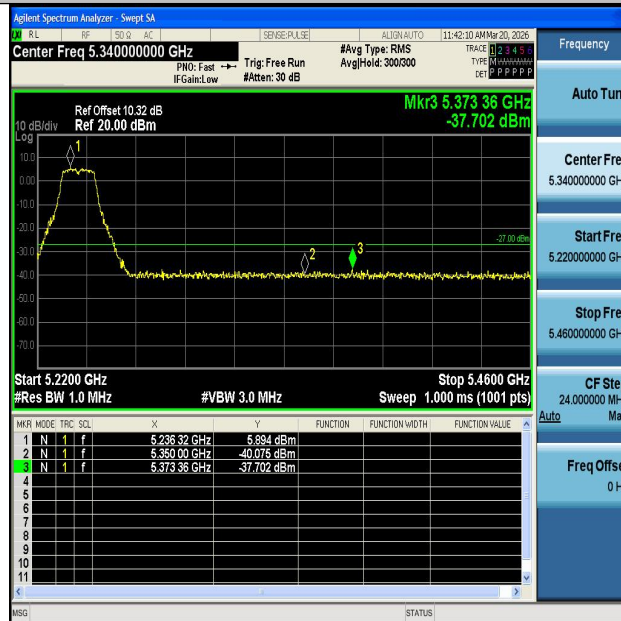
11A-Ant1-5240-PASS
