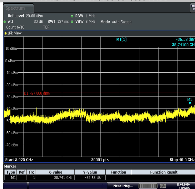
11AX40SISO-Ant1-5795-5925~40000-PASS
