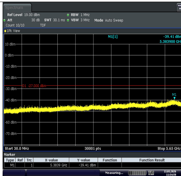
11AX40SISO-Ant1-5795-30~5650-PASS
