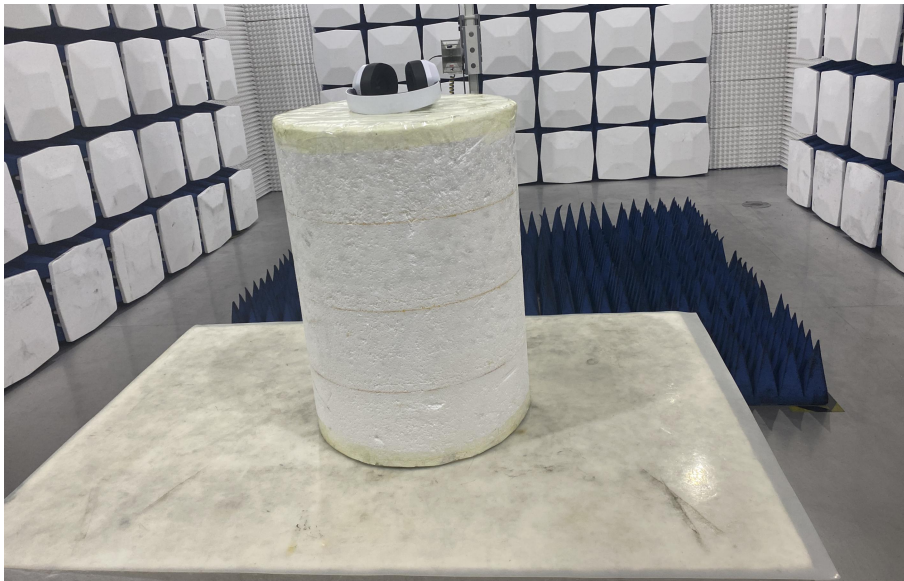
Radiated Spurious
