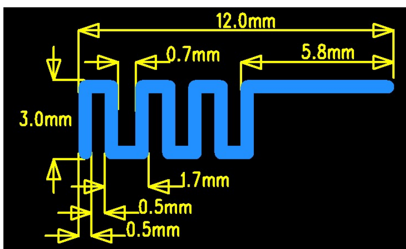
Figure 1 :keyboard Antenna size
