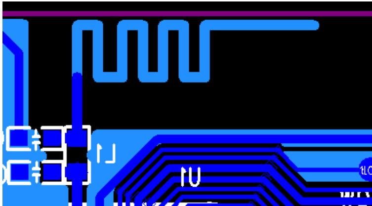
Figure 2 :keyboard Antenna
