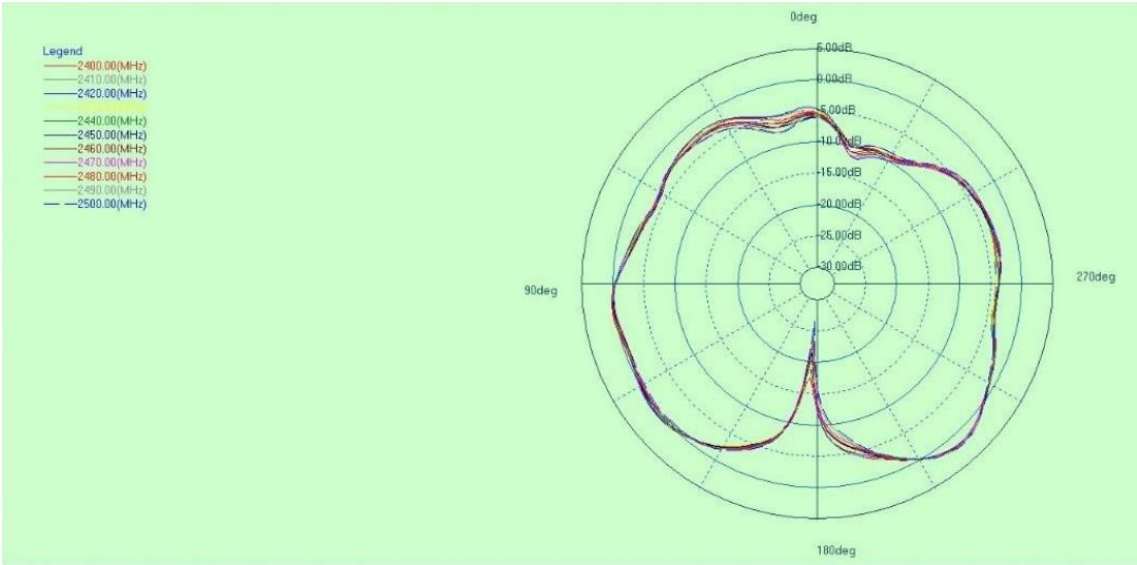
1D Radiation Pattern
