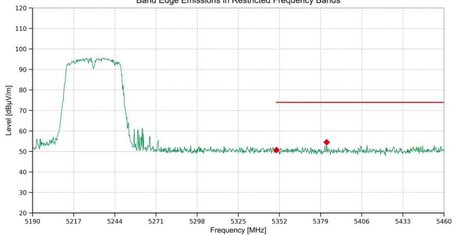
Band Edge Emissions in Restricted Frequency Bands
