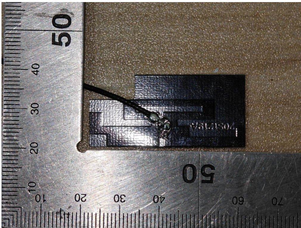
External PCB Antenna
