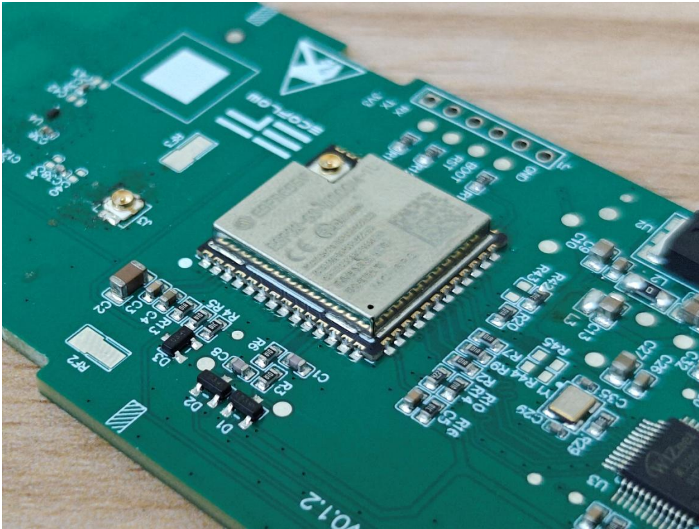
Top View of Module - module is mounted on the test board
