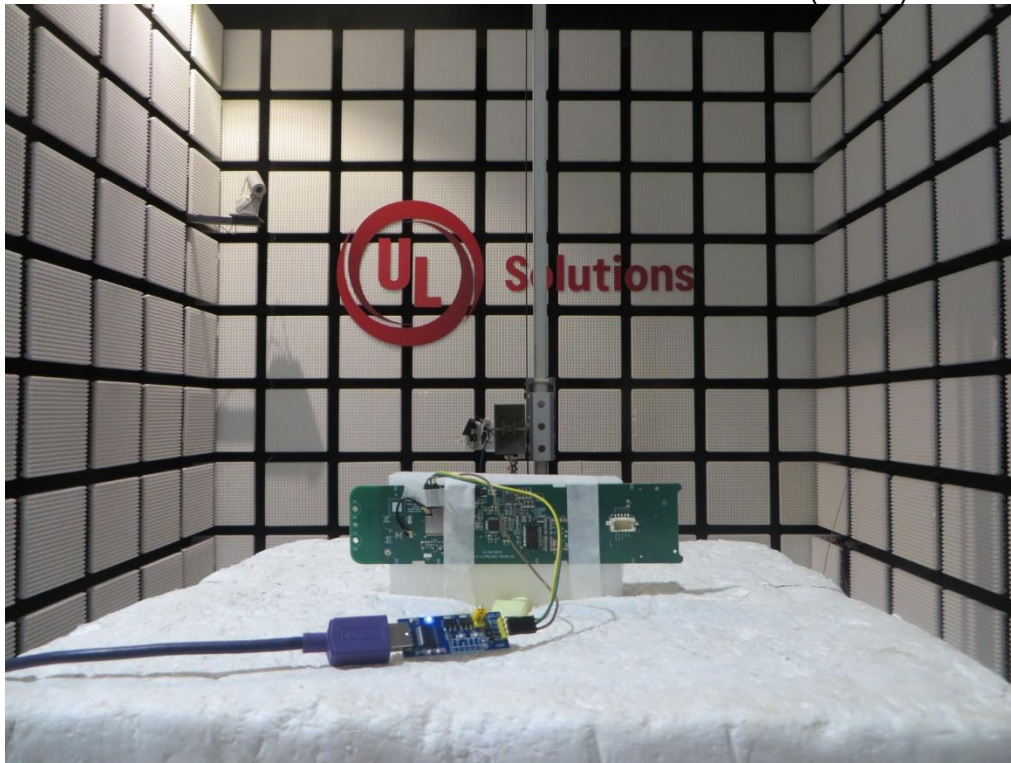
Onboard PCB Antenna MEASUREMENT POSITION (Z axis)
