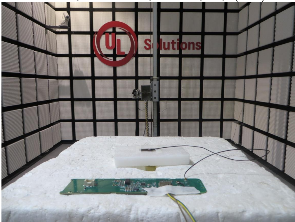
External PCB Antenna MEASUREMENT POSITION (X axis)
