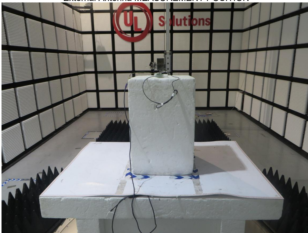
External Antenna MEASUREMENT POSITION (X axis)
