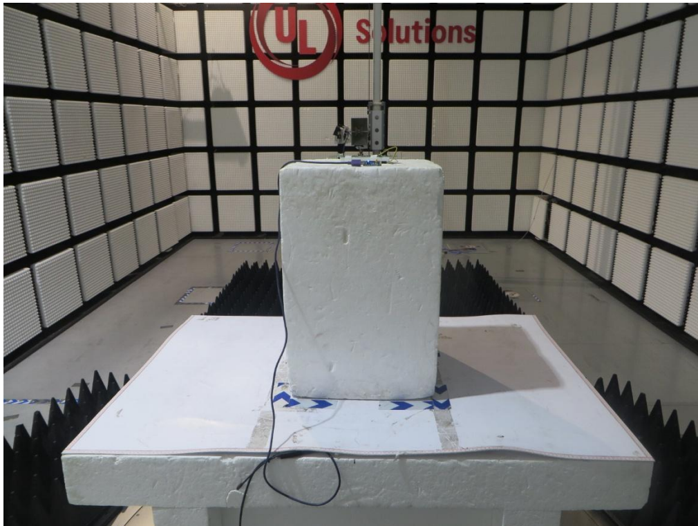
Onboard PCB Antenna MEASUREMENT POSITION (X axis)
