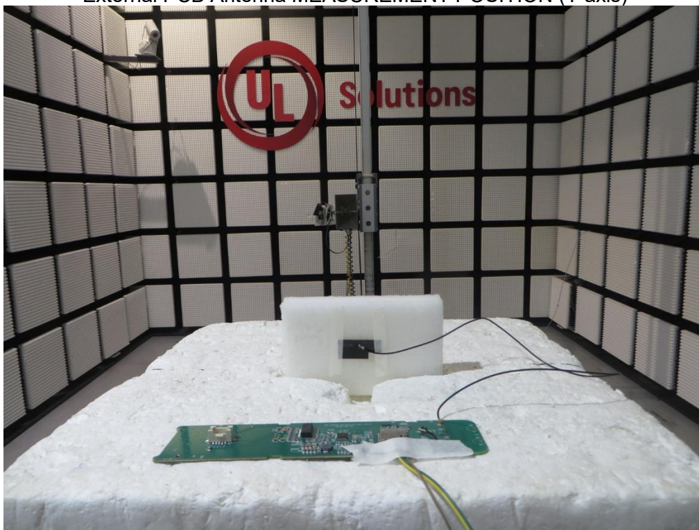
External PCB Antenna MEASUREMENT POSITION (Z axis)
