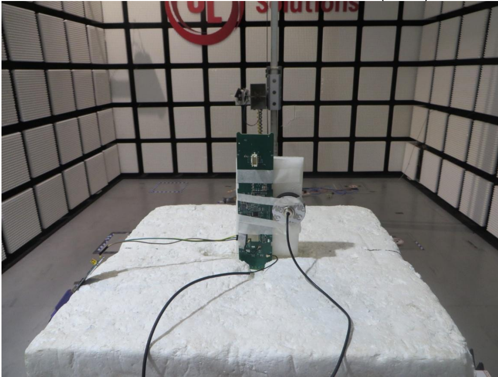
External Antenna MEASUREMENT POSITION (Z axis)
