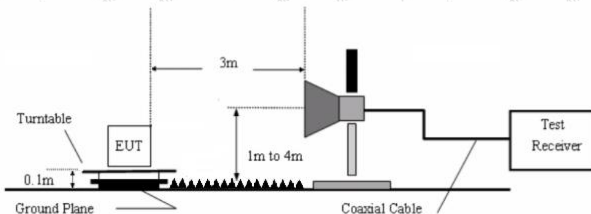
Figure 2. Above 1 GHz
