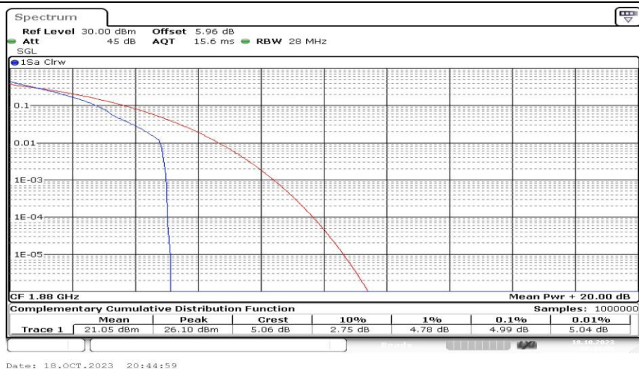
Band2-15MHz-QPSK-18900-1RB#0-PASS
