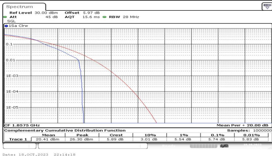
Band2-15MHz-16QAM-18675-1RB#0-PASS
