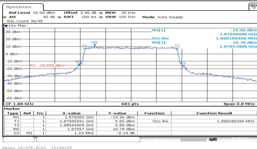
Band2-1.4MHz-QPSK-18900-6RB#0-PASS
