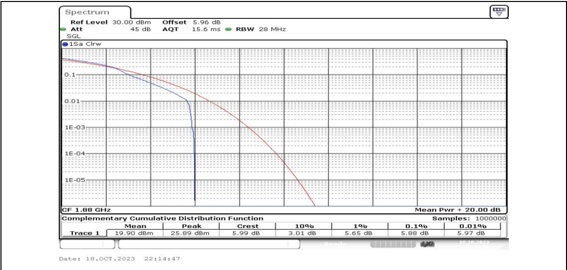
Band2-15MHz-16QAM-18900-1RB#0-PASS
