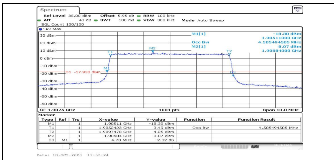
Band2-5MHz-16QAM-19175-25RB#0-PASS
