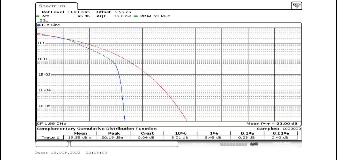
Band2-15MHz-16QAM-18900-25RB#0-PASS
