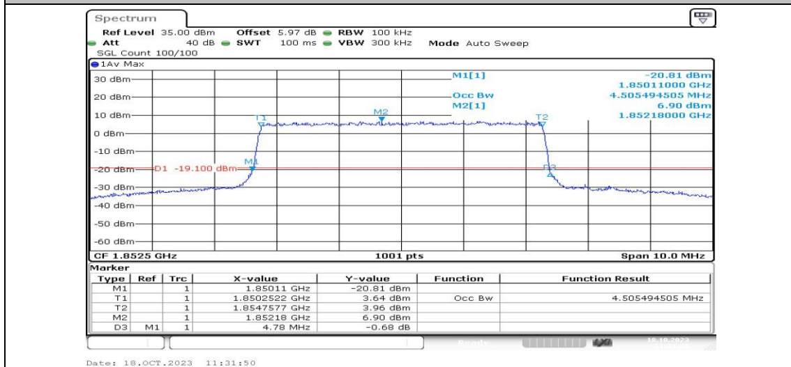
Band2-5MHz-16QAM-18625-25RB#0-PASS
