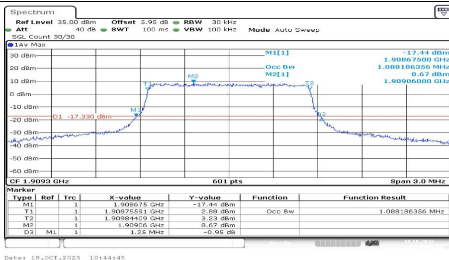
Band2-1.4MHz-16QAM-19193-6RB#0-PASS
