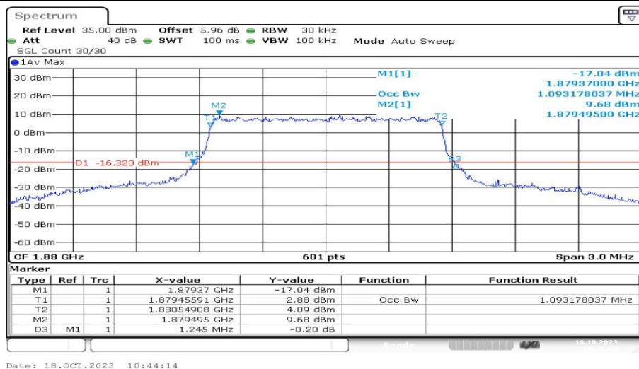
Band2-1.4MHz-16QAM-18900-6RB#0-PASS
