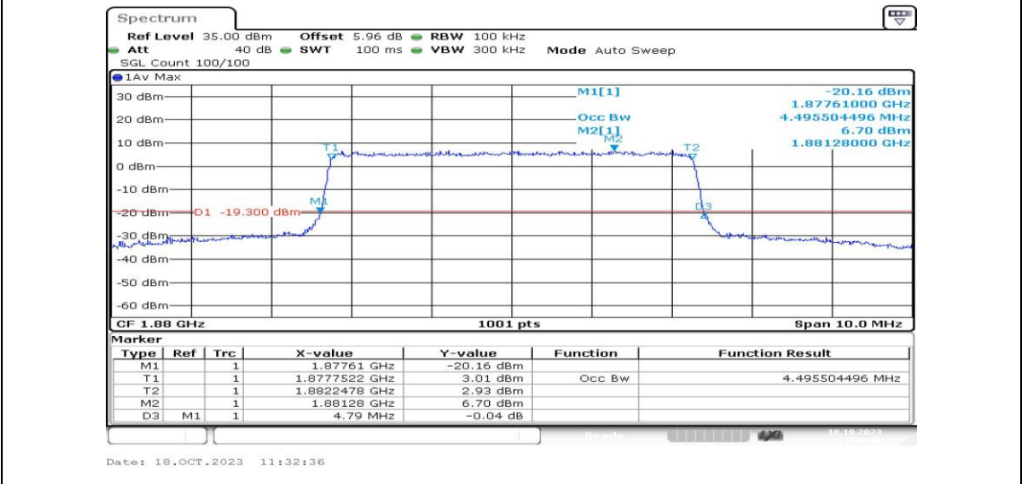
Band2-5MHz-16QAM-18900-25RB#0-PASS
