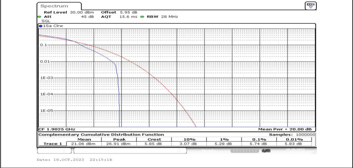
Band2-15MHz-16QAM-19125-1RB#0-PASS
