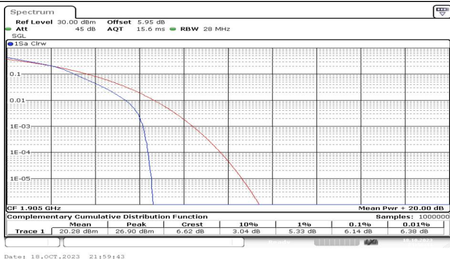
Band2-10MHz-16QAM-19150-25RB#0-PASS
