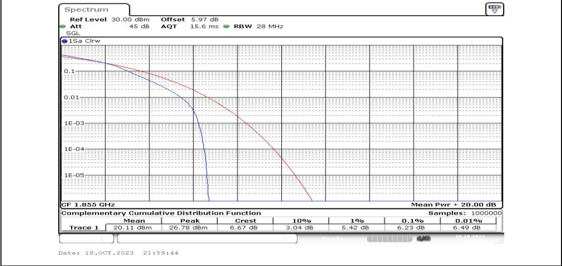
Band2-10MHz-16QAM-18650-25RB#0-PASS
