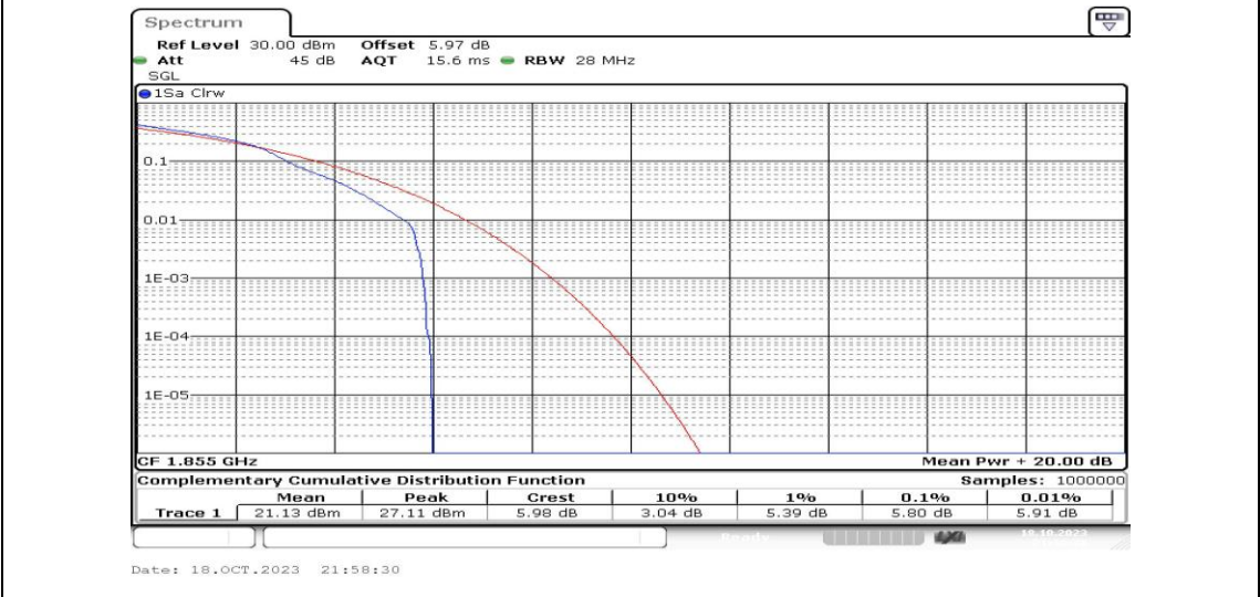
Band2-10MHz-16QAM-18650-1RB#0-PASS
