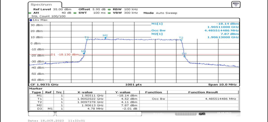
Band2-5MHz-QPSK-19175-25RB#0-PASS
