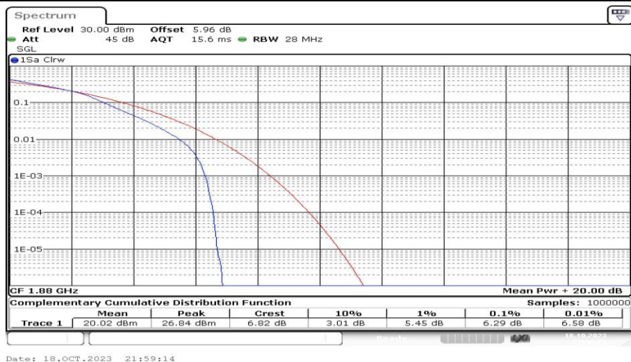
Band2-10MHz-16QAM-18900-25RB#0-PASS
