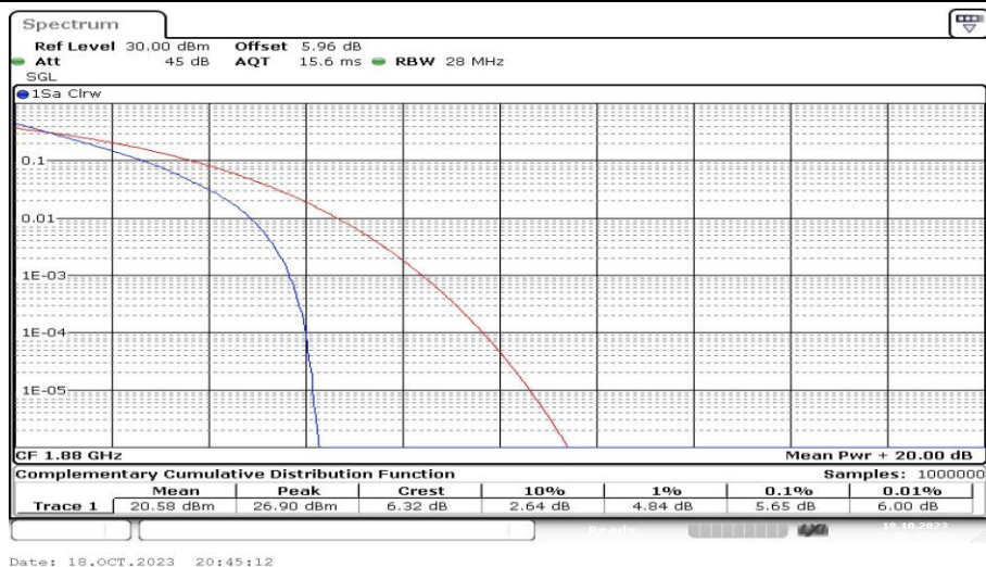
Band2-15MHz-QPSK-18900-75RB#0-PASS
