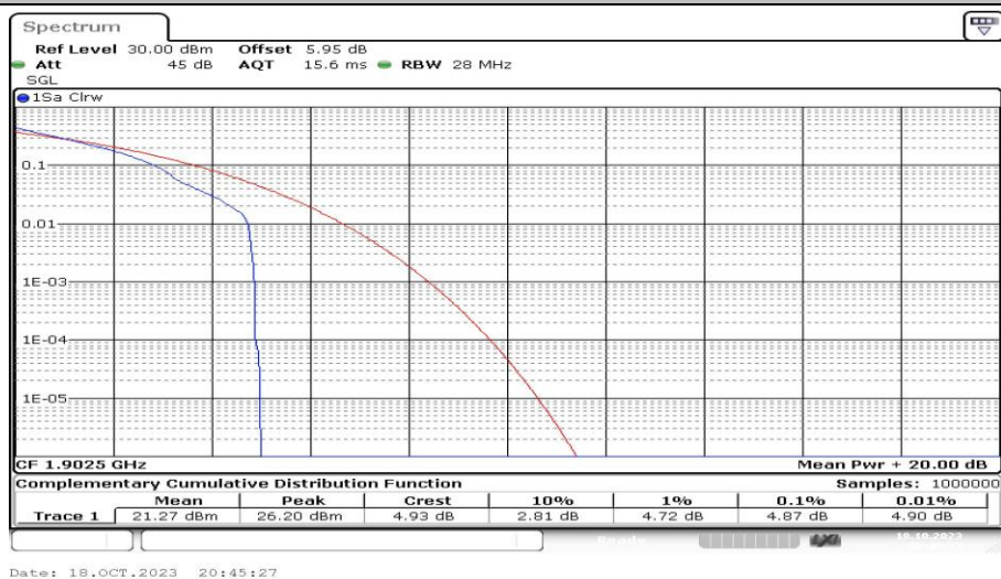
Band2-15MHz-QPSK-19125-1RB#0-PASS
