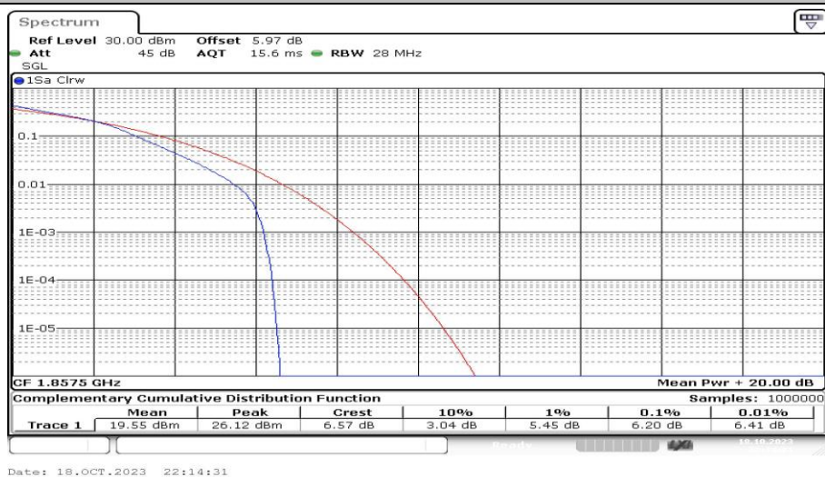
Band2-15MHz-16QAM-18675-25RB#0-PASS
