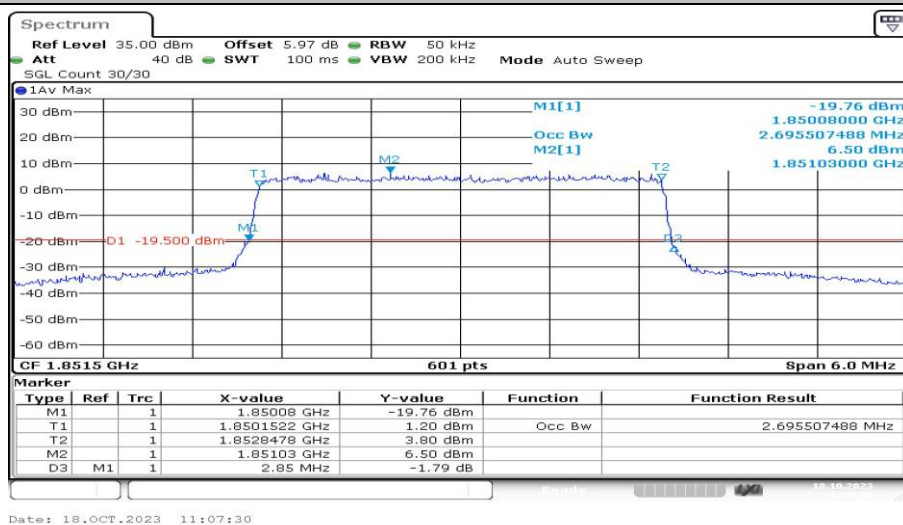
Band2-3MHz-16QAM-18615-15RB#0-PASS
