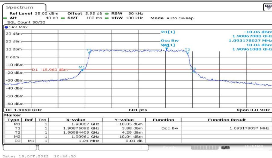
Band2-1.4MHz-QPSK-19193-6RB#0-PASS
