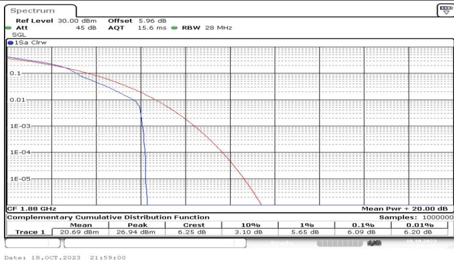
Band2-10MHz-16QAM-18900-1RB#0-PASS
