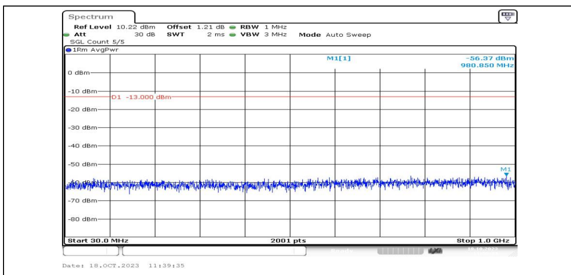
Band2-5MHz-16QAM-18900-1RB#0-Range3:30~1000MHz-PASS
