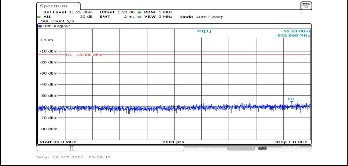
Band2-15MHz-QPSK-19125-1RB#0-Range3:30~1000MHz-PASS
