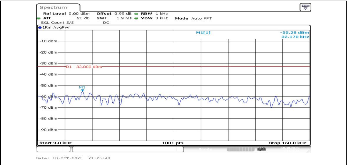
Band2-20MHz-QPSK-19100-1RB#0-Range1:0.009~0.15MHz-PASS
