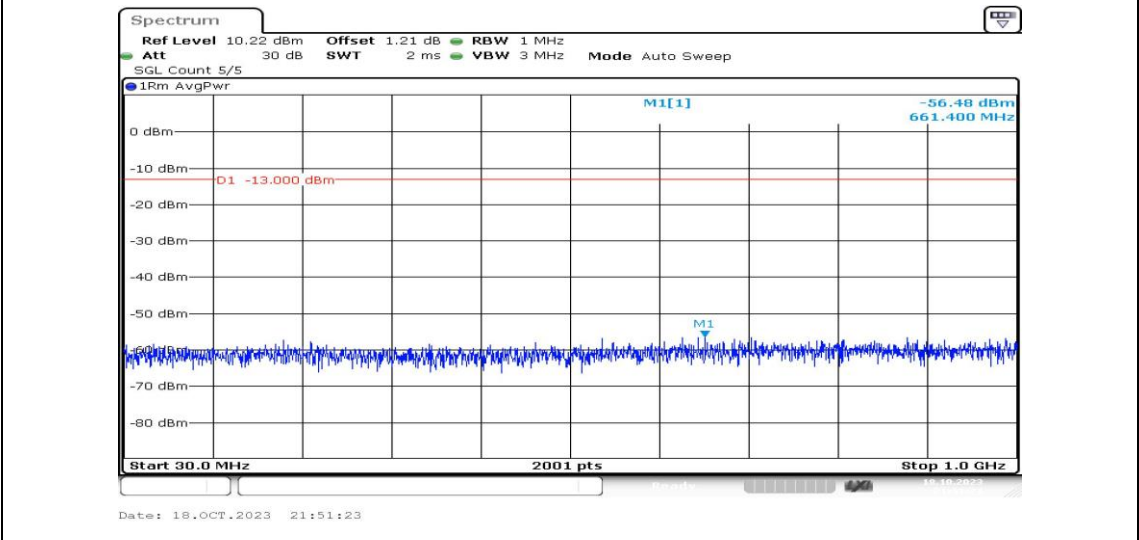
Band2-10MHz-16QAM-18900-1RB#0-Range3:30~1000MHz-PASS
