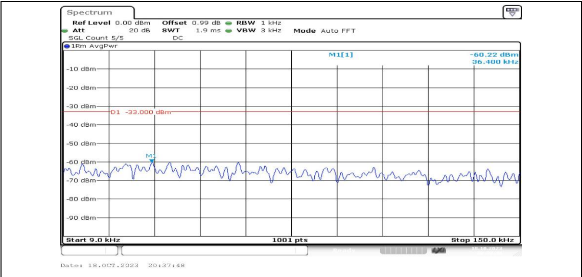
Band2-15MHz-QPSK-19125-1RB#0-Range1:0.009~0.15MHz-PASS
