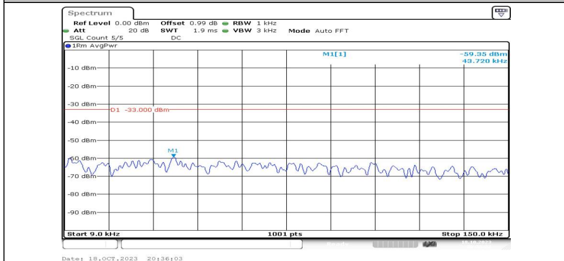
Band2-15MHz-QPSK-18675-1RB#0-Range1:0.009~0.15MHz-PASS
