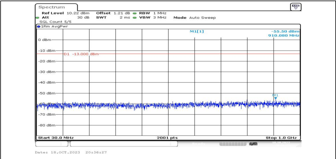
Band2-15MHz-QPSK-18675-1RB#0-Range3:30~1000MHz-PASS
