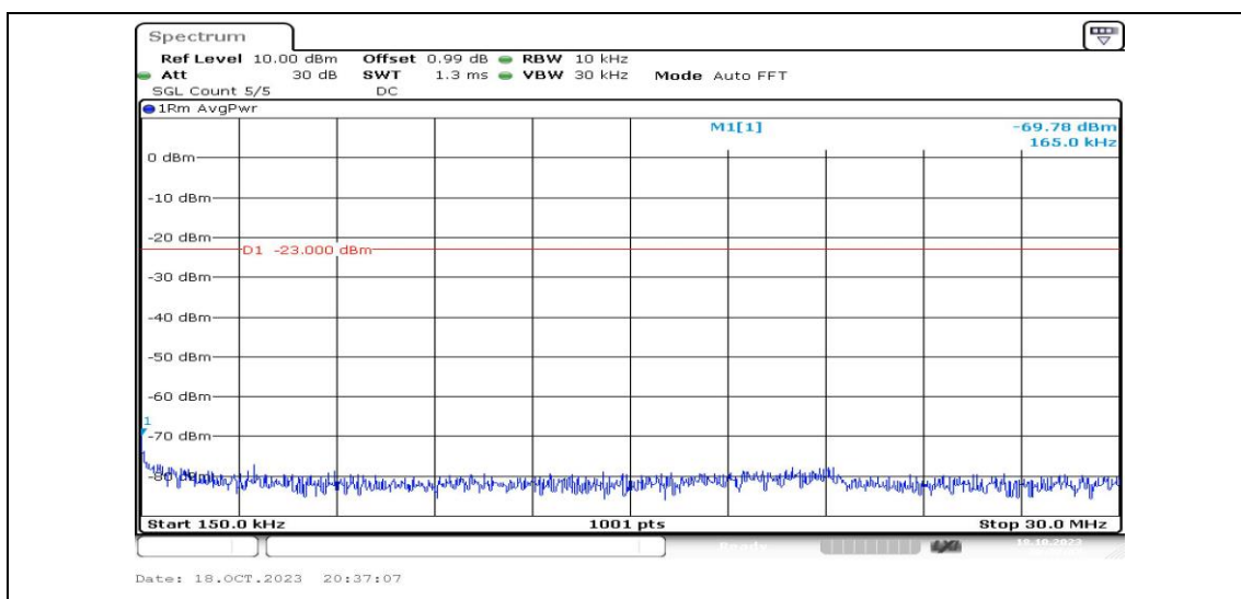
Band2-15MHz-QPSK-18900-1RB#0-Range2:0.15~30MHz-PASS
