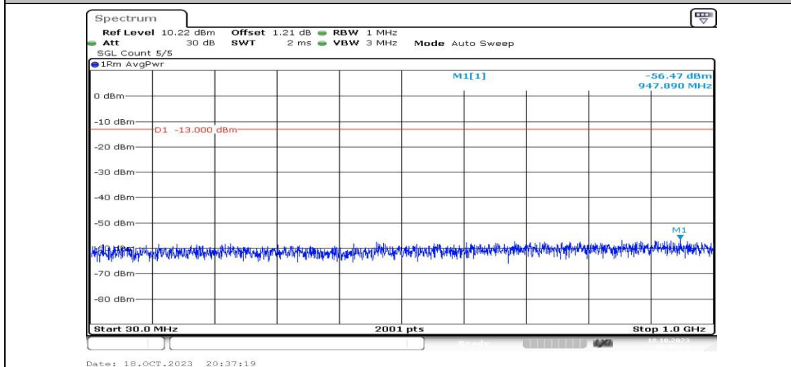
Band2-15MHz-QPSK-18900-1RB#0-Range3:30~1000MHz-PASS
