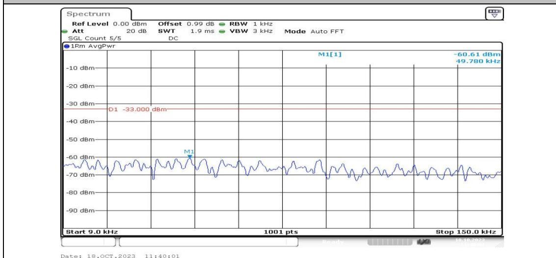
Band2-5MHz-QPSK-19175-1RB#0-Range1:0.009~0.15MHz-PASS
