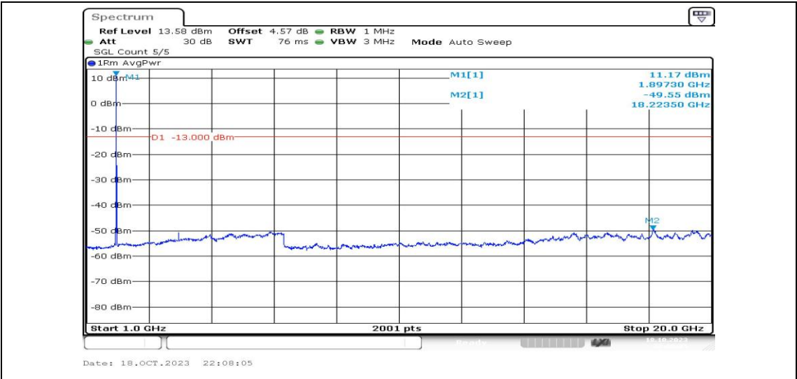
Band2-15MHz-16QAM-19125-1RB#0-Range4:1000~20000MHz-PASS
