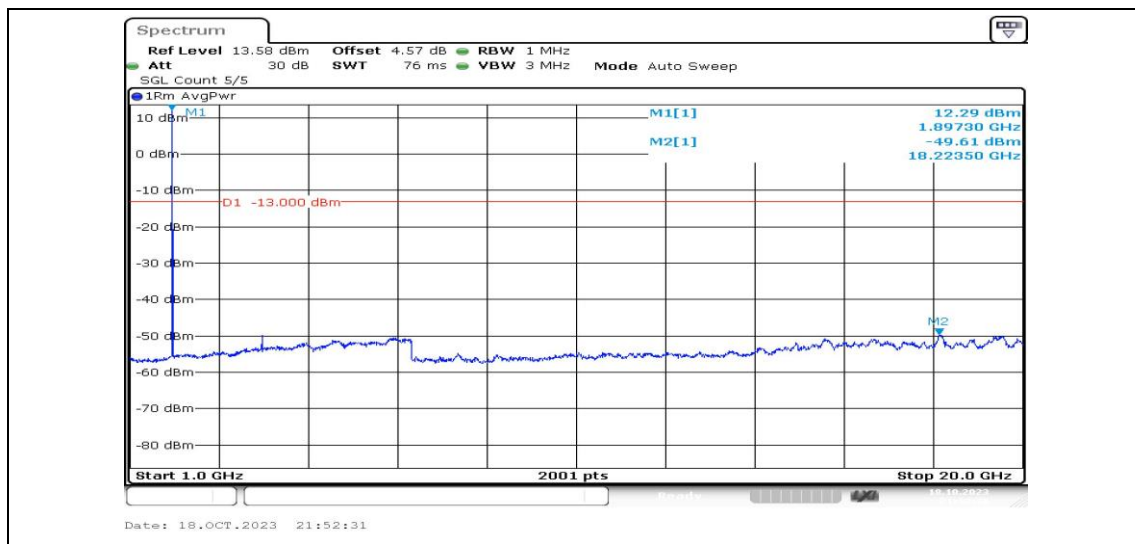
Band2-10MHz-16QAM-19150-1RB#0-Range4:1000~20000MHz-PASS
