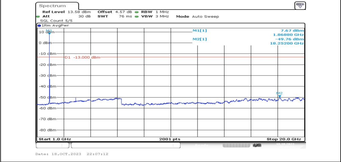
Band2-15MHz-16QAM-18900-1RB#0-Range4:1000~20000MHz-PASS
