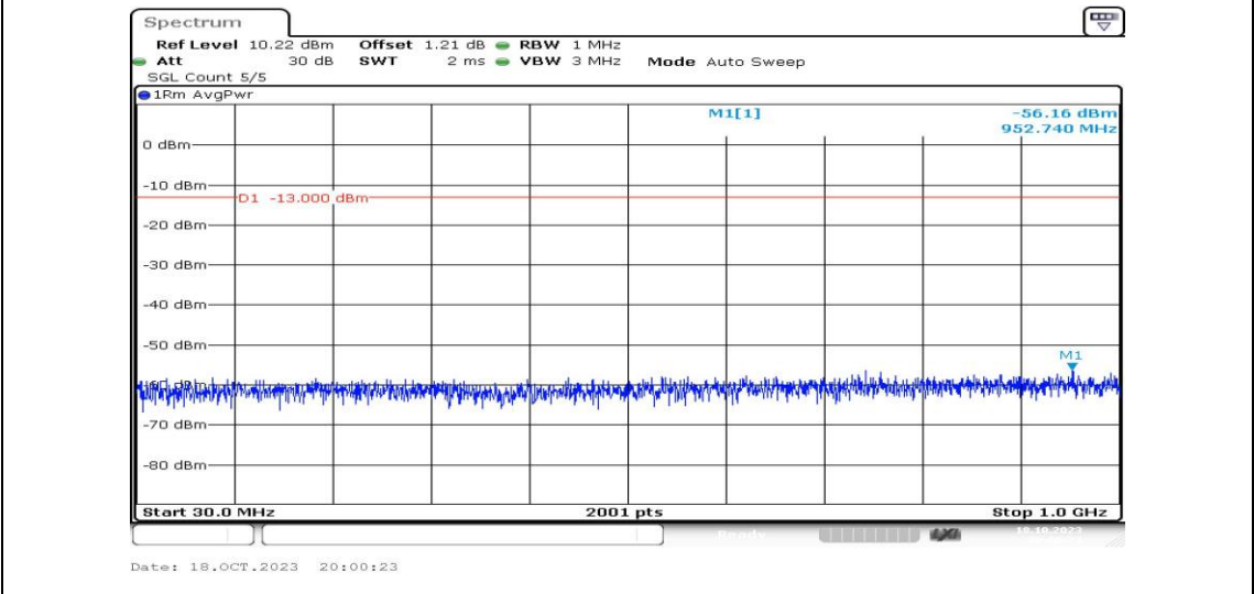
Band2-10MHz-QPSK-18900-1RB#0-Range3:30~1000MHz-PASS
