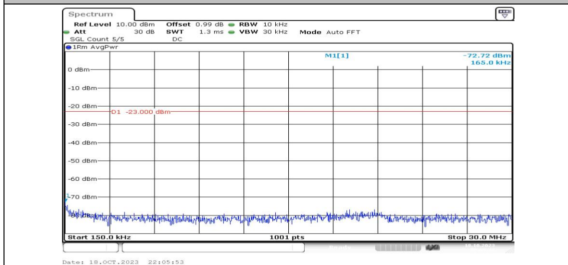
Band2-15MHz-16QAM-18675-1RB#0-Range2:0.15~30MHz-PASS
