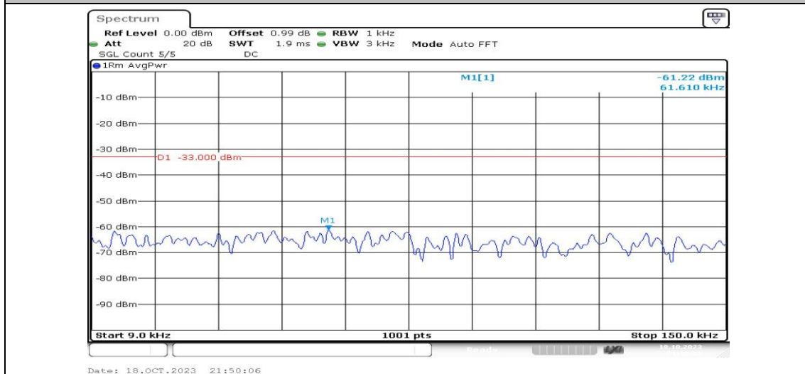
Band2-10MHz-16QAM-18650-1RB#0-Range1:0.009~0.15MHz-PASS
