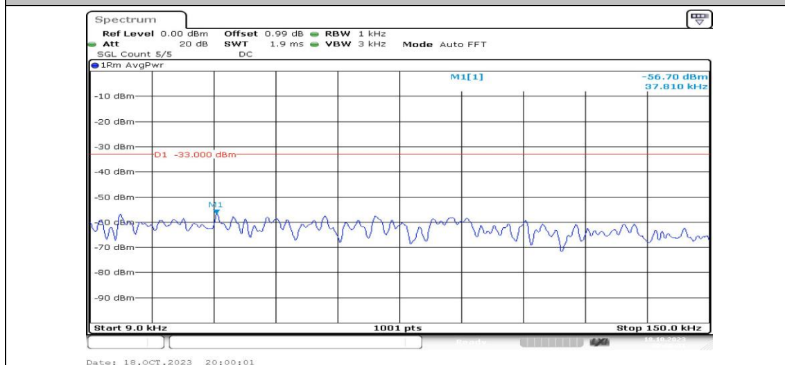
Band2-10MHz-QPSK-18900-1RB#0-Range1:0.009~0.15MHz-PASS
