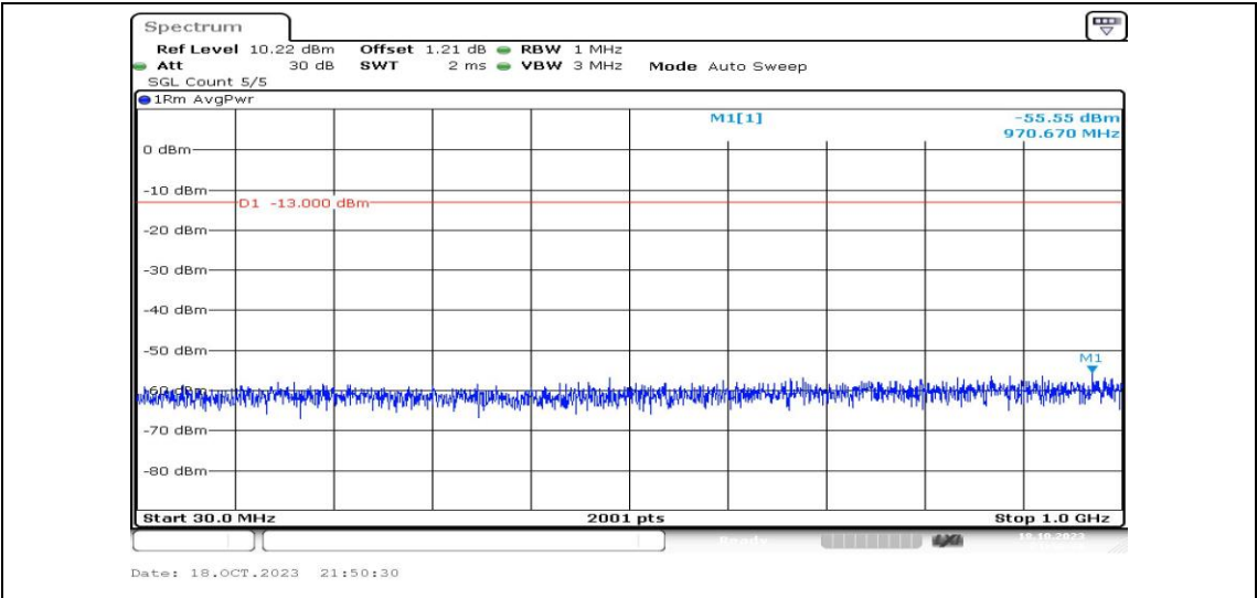
Band2-10MHz-16QAM-18650-1RB#0-Range3:30~1000MHz-PASS
