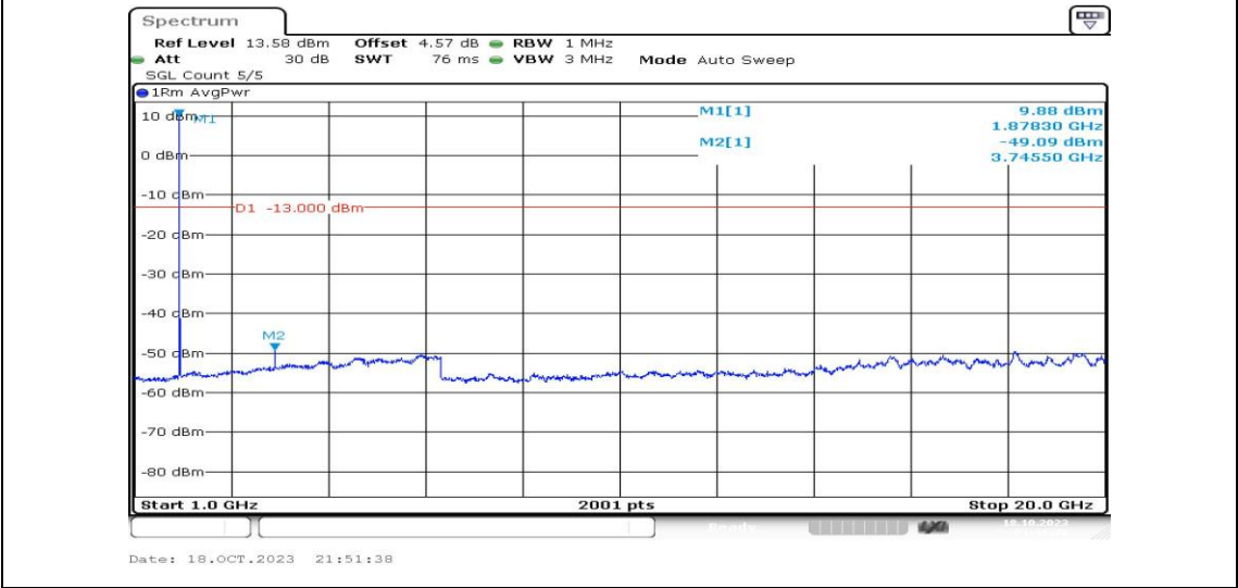
Band2-10MHz-16QAM-18900-1RB#0-Range4:1000~20000MHz-PASS
