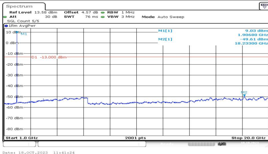
Band2-5MHz-16QAM-19175-1RB#0-Range4:1000~20000MHz-PASS
