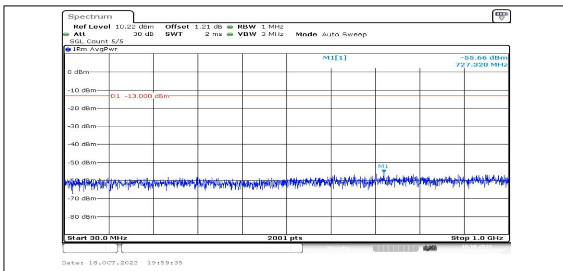
Band2-10MHz-QPSK-18650-1RB#0-Range3:30~1000MHz-PASS
