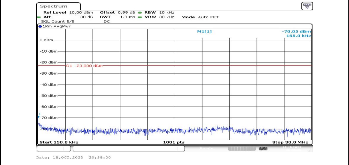
Band2-15MHz-QPSK-19125-1RB#0-Range2:0.15~30MHz-PASS
