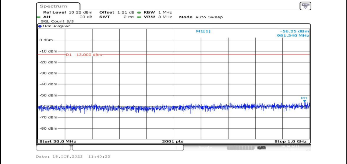
Band2-5MHz-QPSK-19175-1RB#0-Range3:30~1000MHz-PASS
