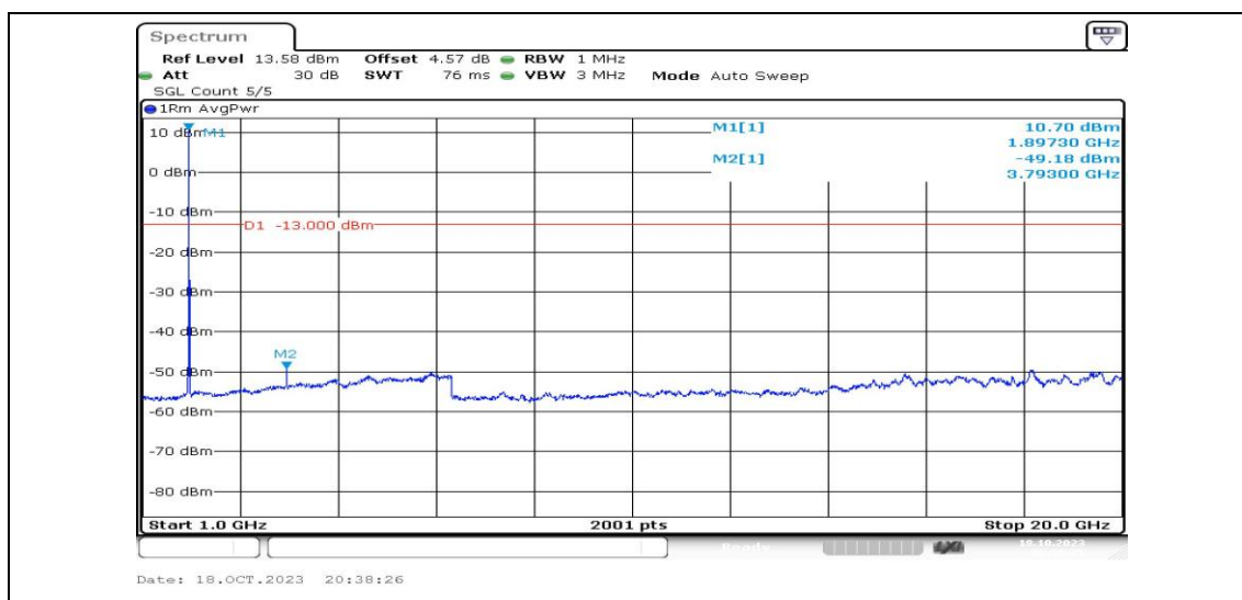
Band2-15MHz-QPSK-19125-1RB#0-Range4:1000~20000MHz-PASS
