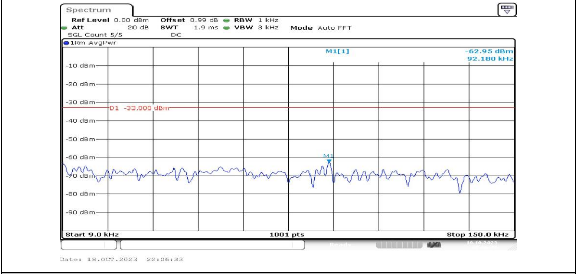
Band2-15MHz-16QAM-18900-1RB#0-Range1:0.009~0.15MHz-PASS
