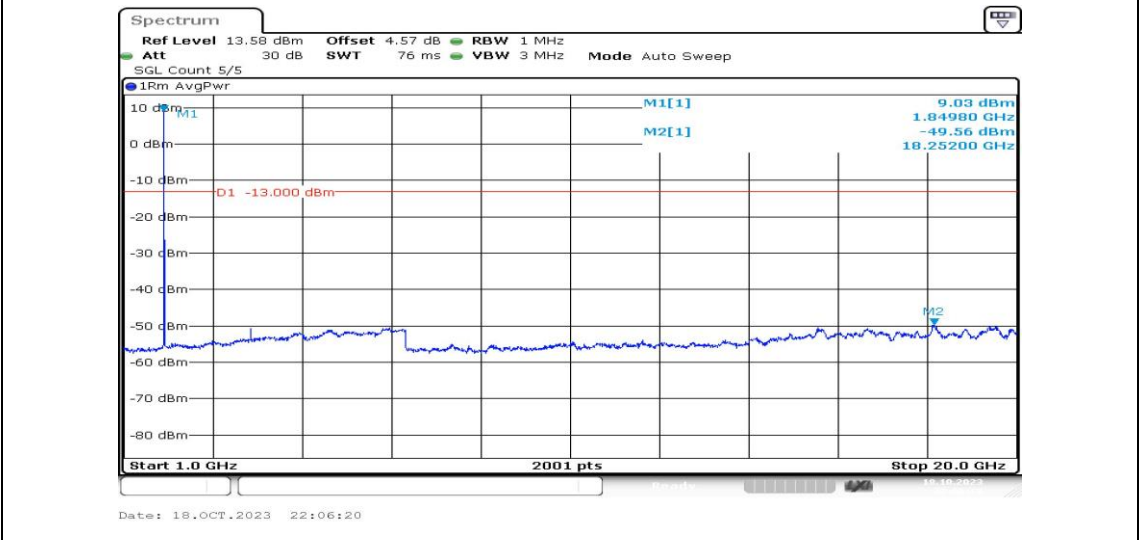
Band2-15MHz-16QAM-18675-1RB#0-Range4:1000~20000MHz-PASS
