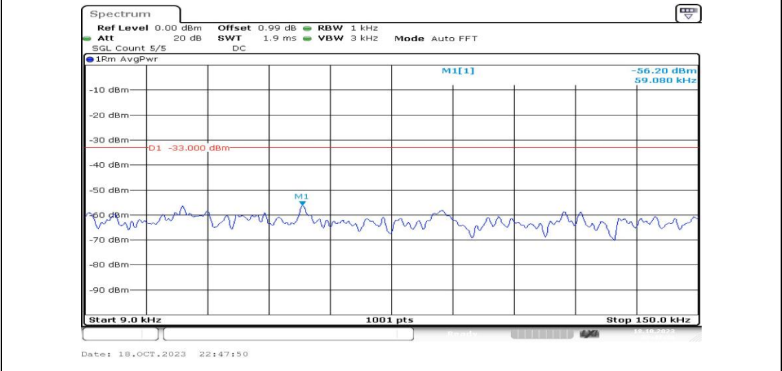
Band2-20MHz-16QAM-18700-1RB#0-Range1:0.009~0.15MHz-PASS
