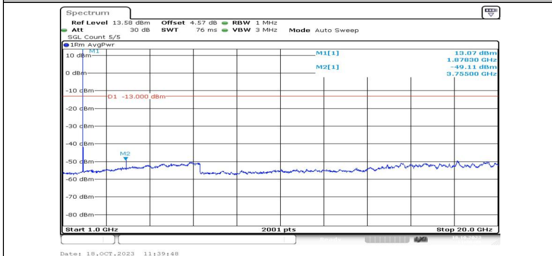
Band2-5MHz-16QAM-18900-1RB#0-Range4:1000~20000MHz-PASS
