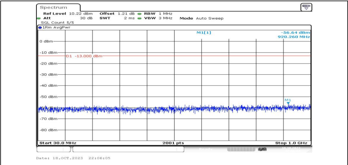
Band2-15MHz-16QAM-18675-1RB#0-Range3:30~1000MHz-PASS
