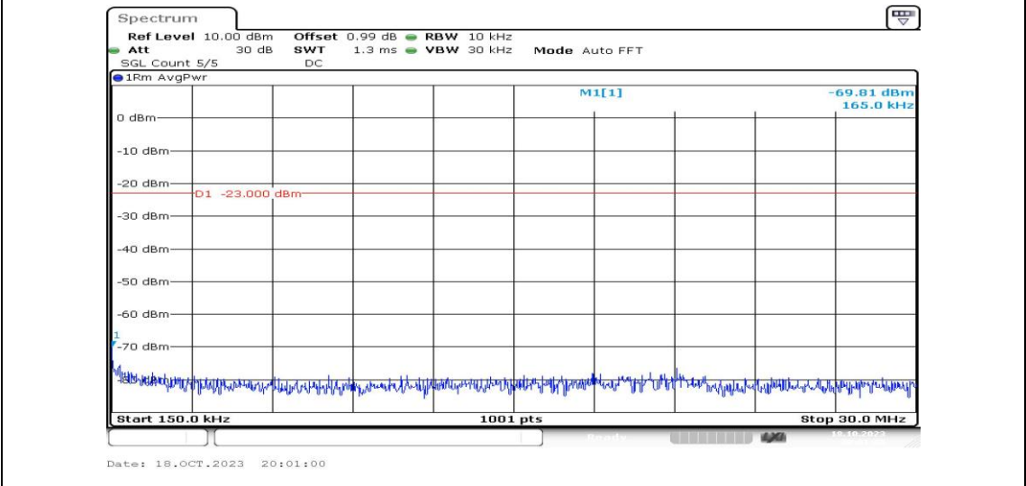
Band2-10MHz-QPSK-19150-1RB#0-Range2:0.15~30MHz-PASS
