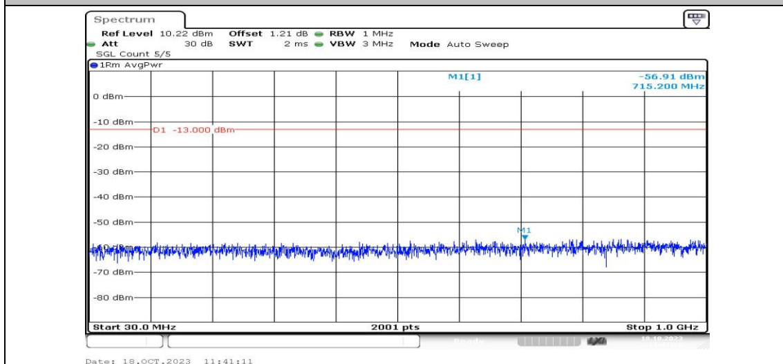
Band2-5MHz-16QAM-19175-1RB#0-Range3:30~1000MHz-PASS
