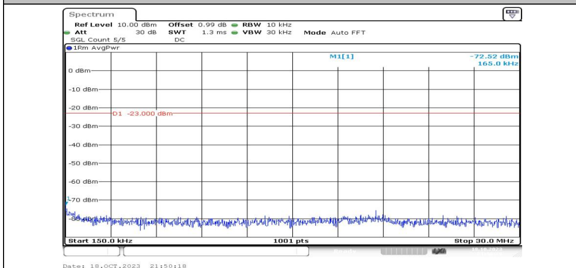
Band2-10MHz-16QAM-18650-1RB#0-Range2:0.15~30MHz-PASS
