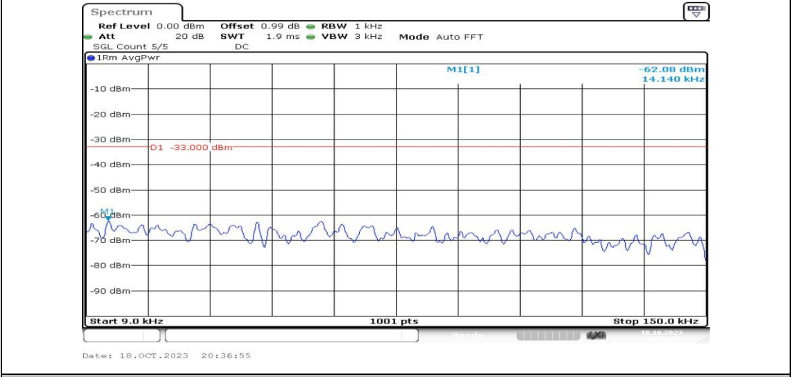
Band2-15MHz-QPSK-18900-1RB#0-Range1:0.009~0.15MHz-PASS
