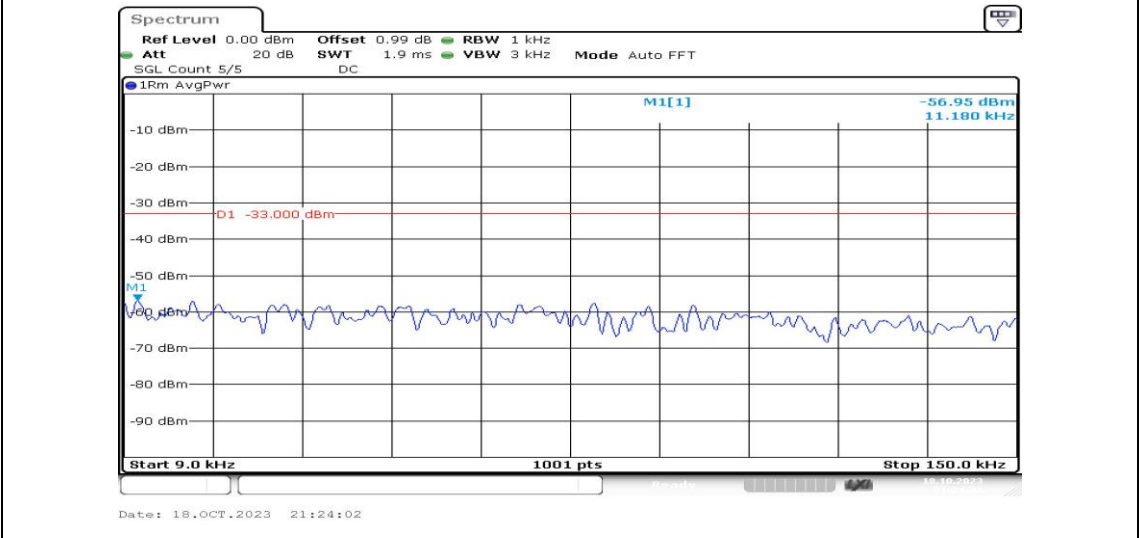
Band2-20MHz-QPSK-18900-1RB#0-Range1:0.009~0.15MHz-PASS
