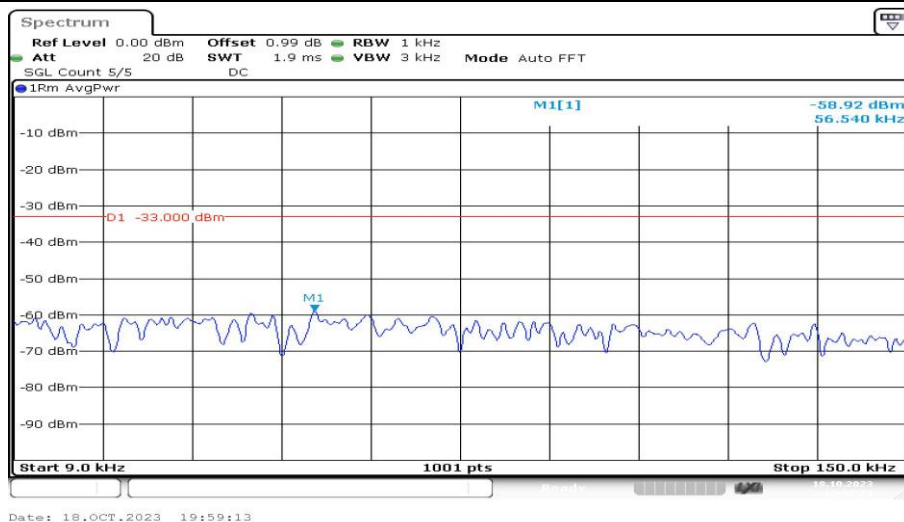
Band2-10MHz-QPSK-18650-1RB#0-Range1:0.009~0.15MHz-PASS
