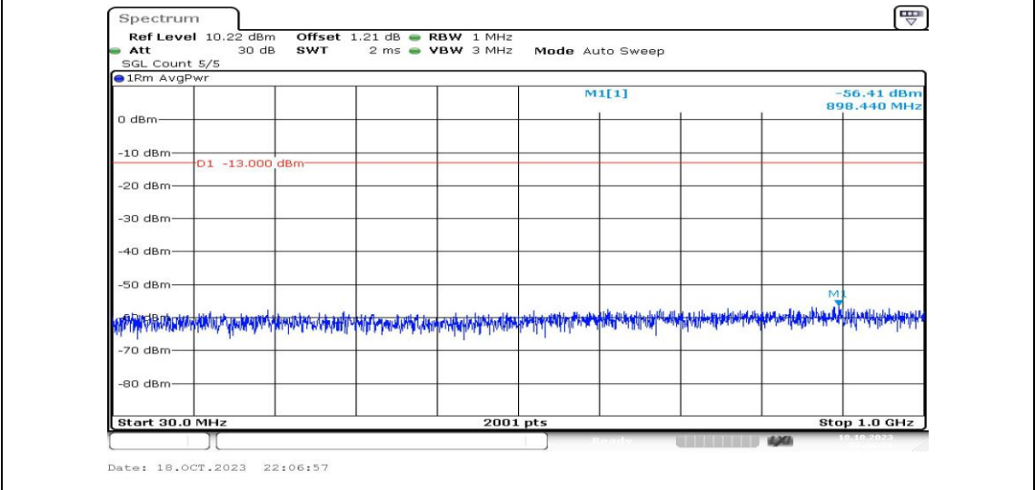
Band2-15MHz-16QAM-18900-1RB#0-Range3:30~1000MHz-PASS
