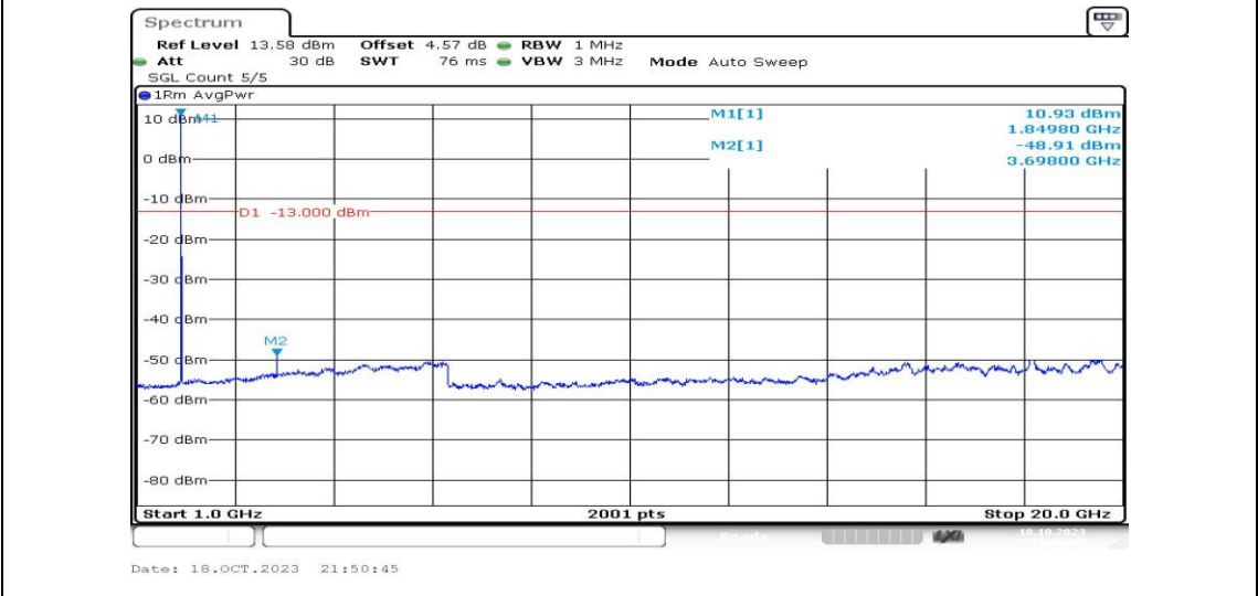
Band2-10MHz-16QAM-18650-1RB#0-Range4:1000~20000MHz-PASS
