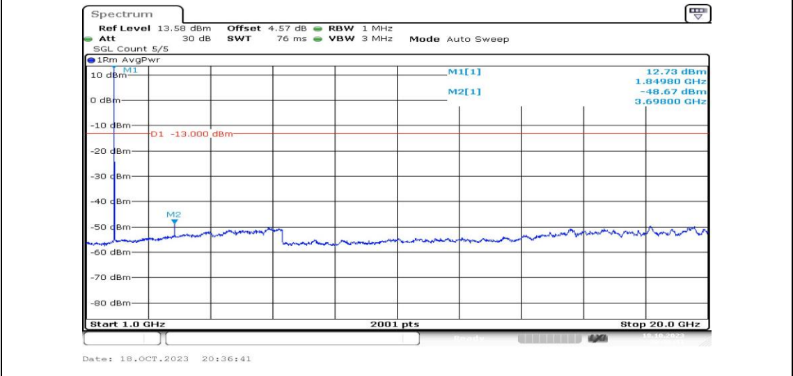
Band2-15MHz-QPSK-18675-1RB#0-Range4:1000~20000MHz-PASS
