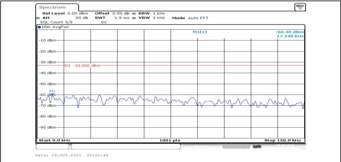
Band2-10MHz-QPSK-19150-1RB#0-Range1:0.009~0.15MHz-PASS
