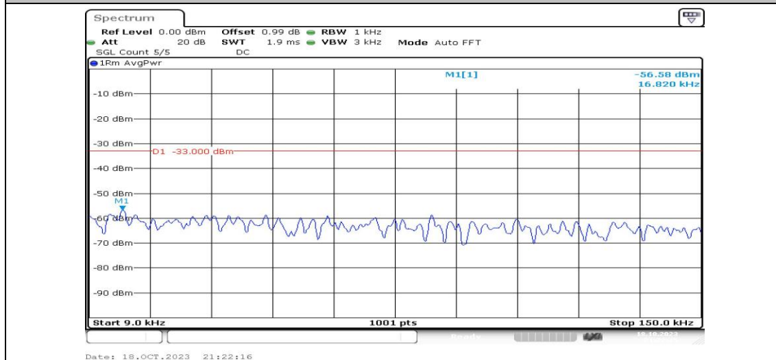
Band2-20MHz-QPSK-18700-1RB#0-Range1:0.009~0.15MHz-PASS
