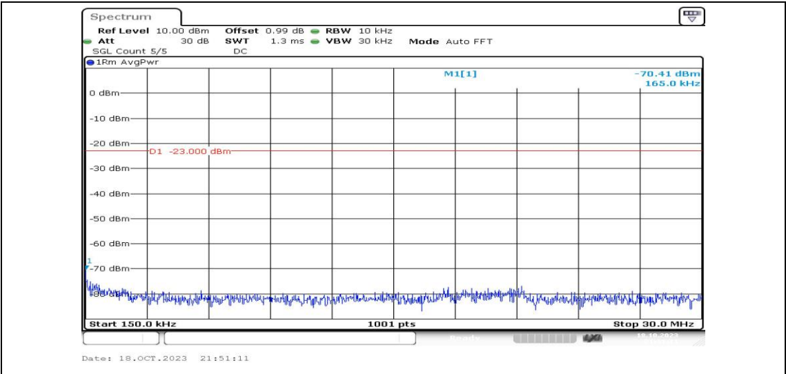
Band2-10MHz-16QAM-18900-1RB#0-Range2:0.15~30MHz-PASS
