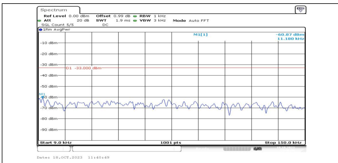
Band2-5MHz-16QAM-19175-1RB#0-Range1:0.009~0.15MHz-PASS
