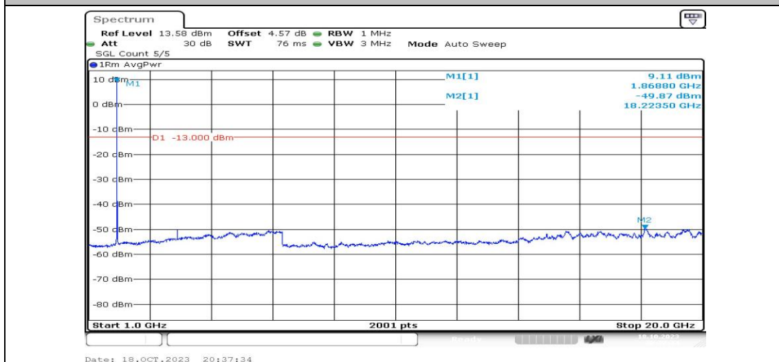
Band2-15MHz-QPSK-18900-1RB#0-Range4:1000~20000MHz-PASS
