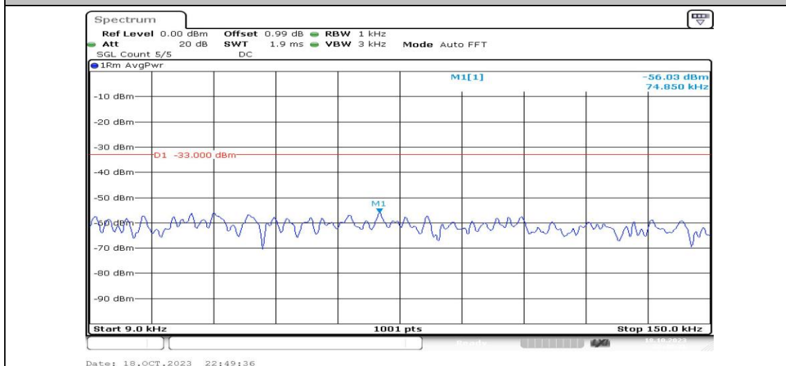
Band2-20MHz-16QAM-18900-1RB#0-Range1:0.009~0.15MHz-PASS
