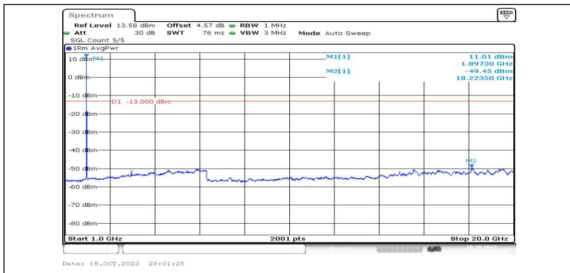
Band2-10MHz-QPSK-19150-1RB#0-Range4:1000~20000MHz-PASS
