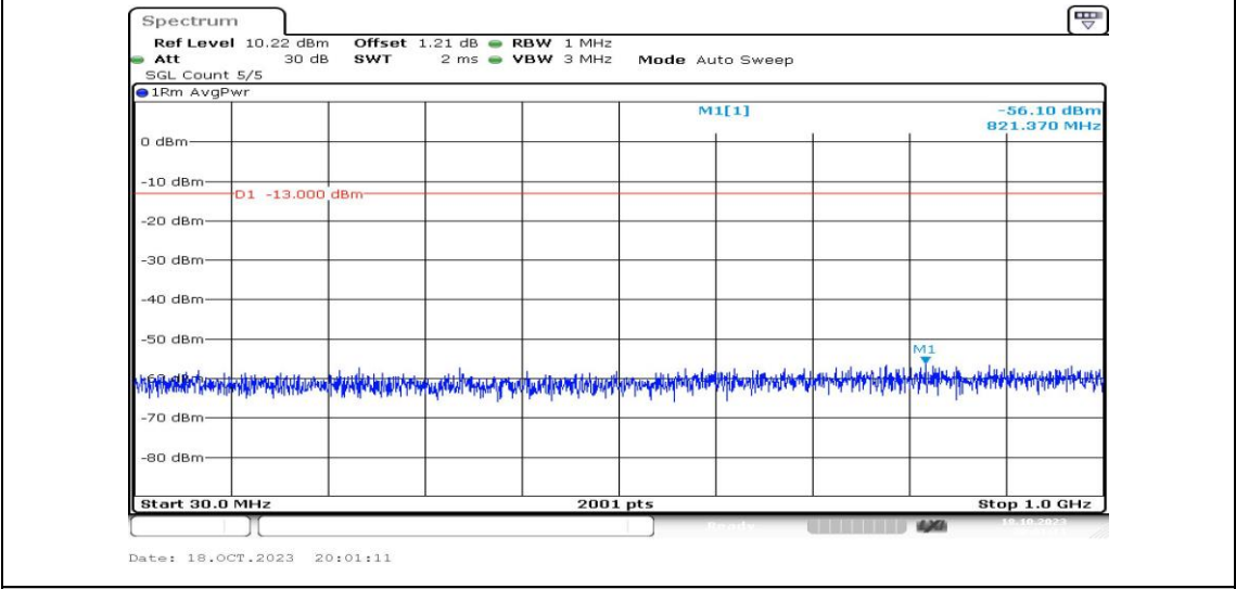
Band2-10MHz-QPSK-19150-1RB#0-Range3:30~1000MHz-PASS
