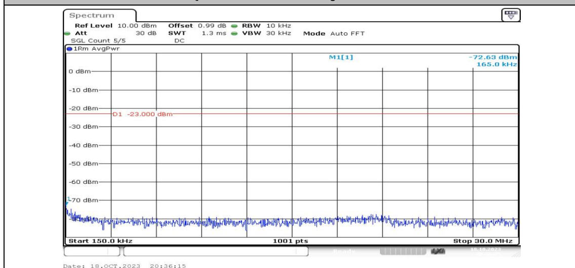
Band2-15MHz-QPSK-18675-1RB#0-Range2:0.15~30MHz-PASS
