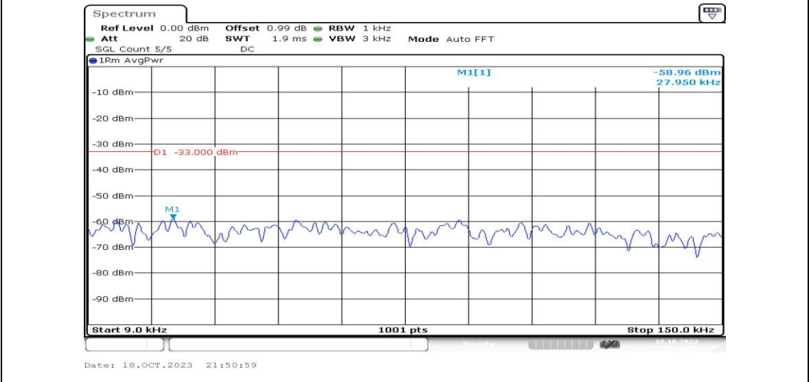
Band2-10MHz-16QAM-18900-1RB#0-Range1:0.009~0.15MHz-PASS
