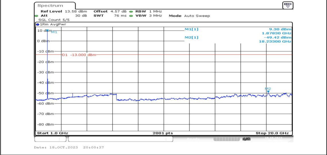
Band2-10MHz-QPSK-18900-1RB#0-Range4:1000~20000MHz-PASS
