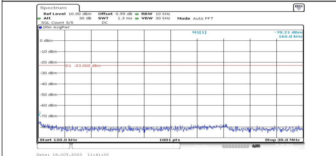
Band2-5MHz-16QAM-19175-1RB#0-Range2:0.15~30MHz-PASS
