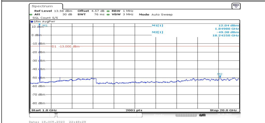
Band2-20MHz-16QAM-18700-1RB#0-Range4:1000~20000MHz-PASS
