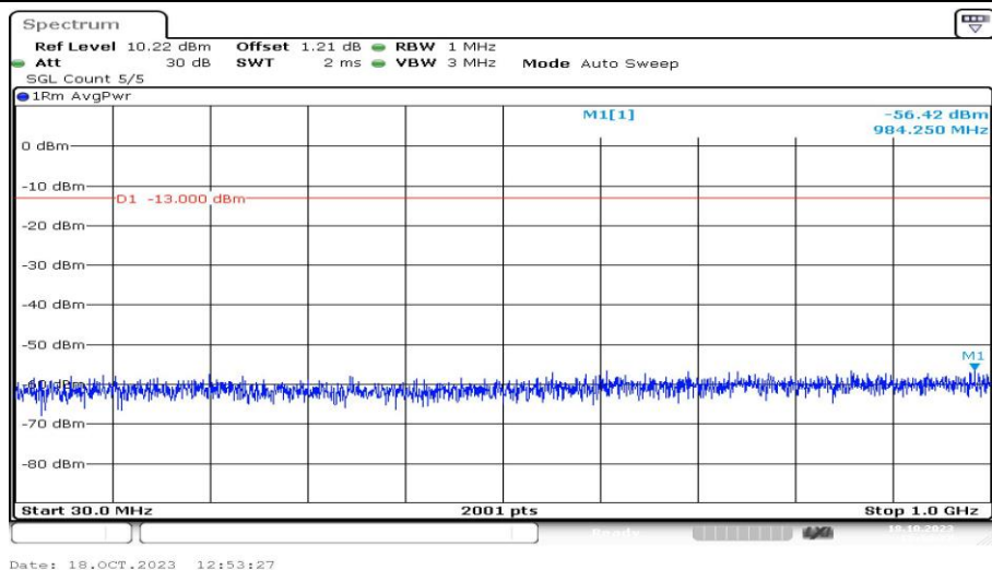
Band4-5MHz-QPSK-20375-1RB#0-Range3:30~1000MHz-PASS
