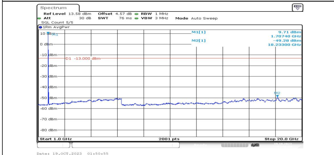
Band4-20MHz-16QAM-20050-1RB#0-Range4:1000~20000MHz-PASS
