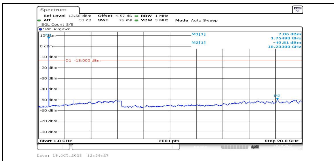
Band4-5MHz-16QAM-20375-1RB#0-Range4:1000~20000MHz-PASS
