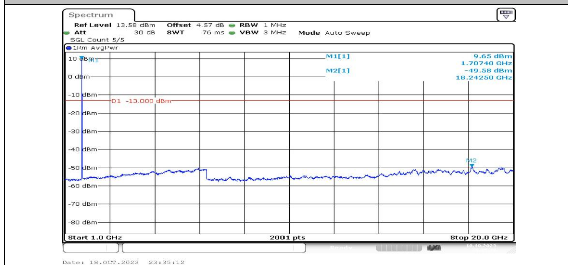
Band4-15MHz-QPSK-20025-1RB#0-Range4:1000~20000MHz-PASS
