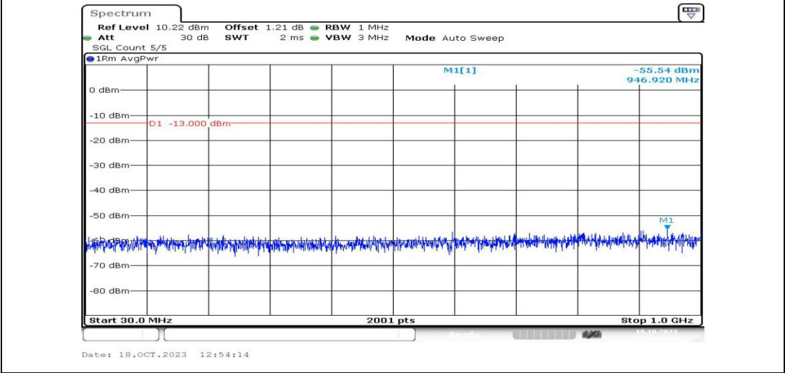
Band4-5MHz-16QAM-20375-1RB#0-Range3:30~1000MHz-PASS
