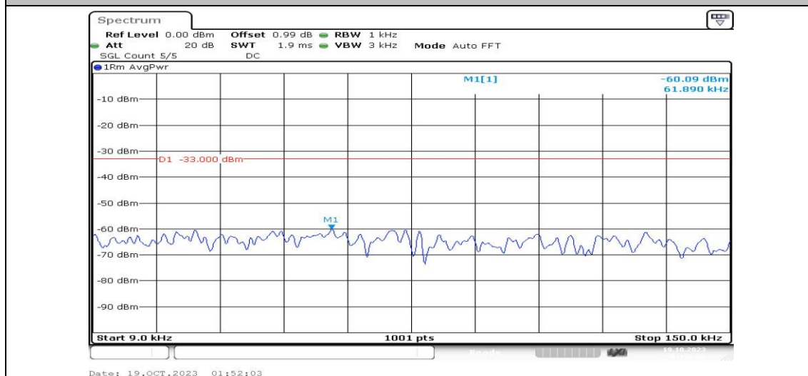
Band4-20MHz-16QAM-20175-1RB#0-Range1:0.009~0.15MHz-PASS
