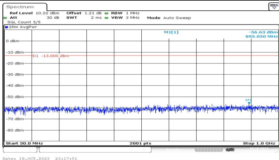
Band4-10MHz-QPSK-20175-1RB#0-Range3:30~1000MHz-PASS
