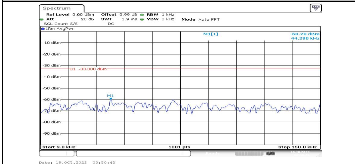
Band4-10MHz-16QAM-20000-1RB#0-Range1:0.009~0.15MHz-PASS
