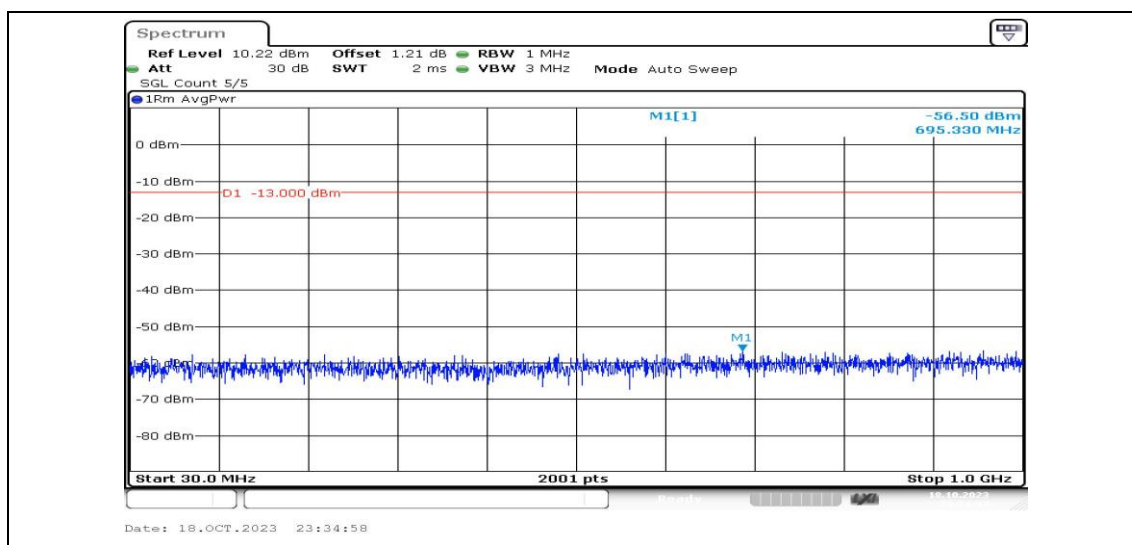
Band4-15MHz-QPSK-20025-1RB#0-Range3:30~1000MHz-PASS
