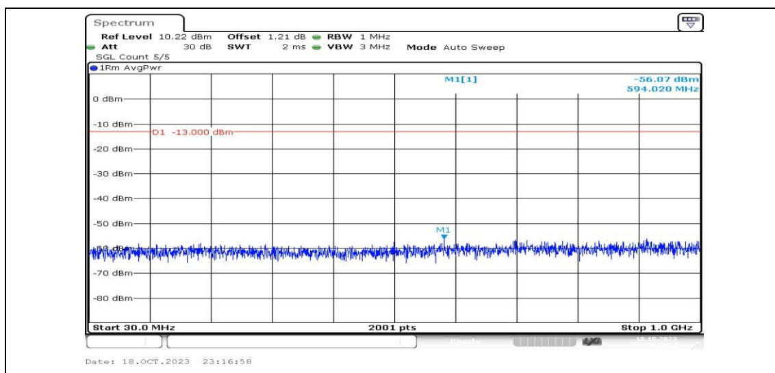
Band4-10MHz-QPSK-20000-1RB#0-Range3:30~1000MHz-PASS
