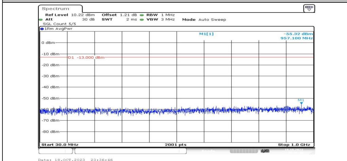
Band4-15MHz-QPSK-20325-1RB#0-Range3:30~1000MHz-PASS
