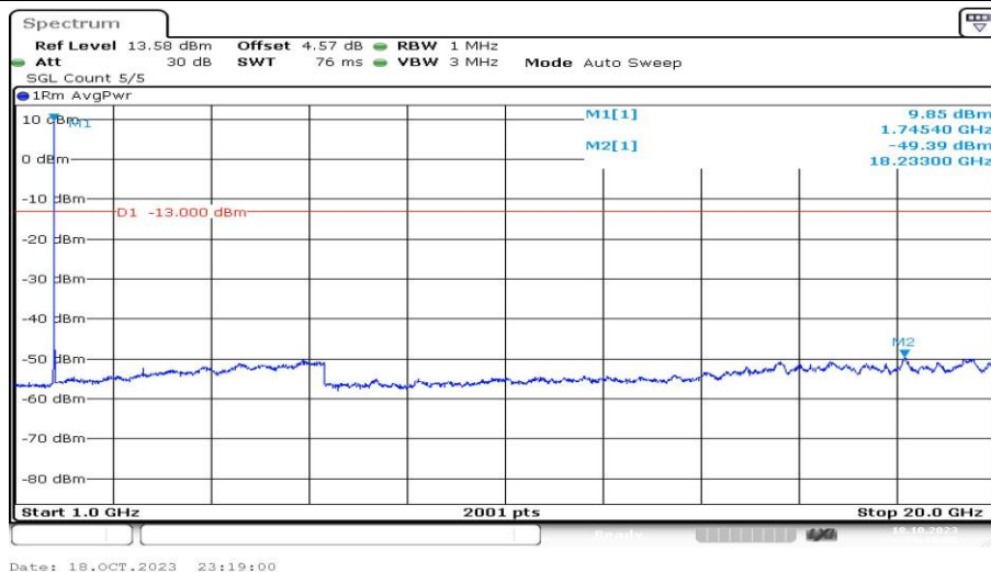
Band4-10MHz-QPSK-20350-1RB#0-Range4:1000~20000MHz-PASS
