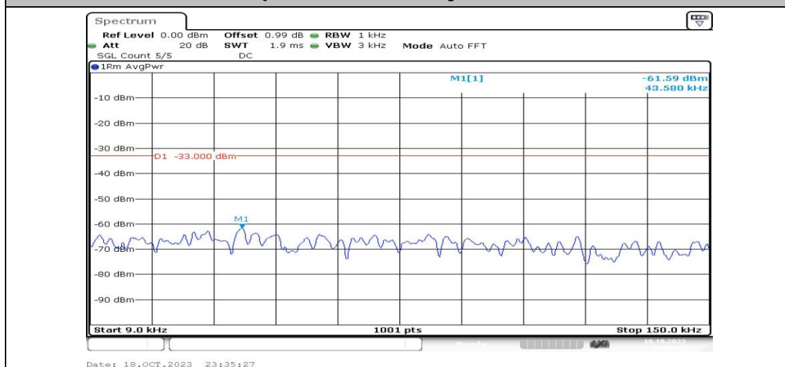
Band4-15MHz-QPSK-20175-1RB#0-Range1:0.009~0.15MHz-PASS
