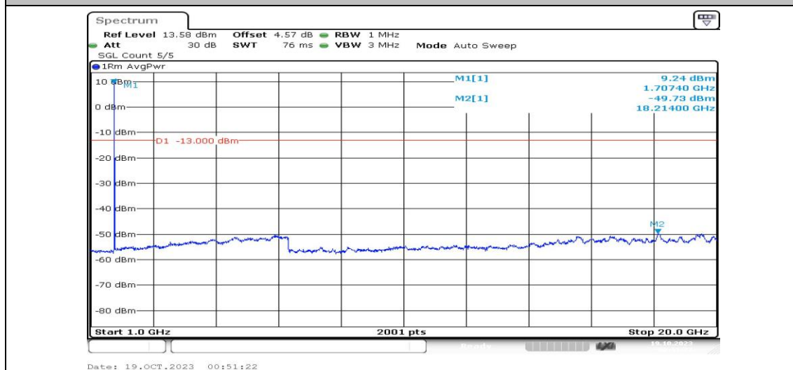
Band4-10MHz-16QAM-20000-1RB#0-Range4:1000~20000MHz-PASS
