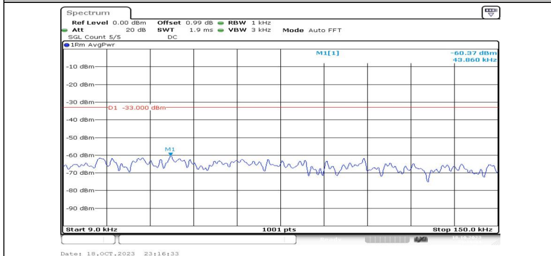
Band4-10MHz-QPSK-20000-1RB#0-Range1:0.009~0.15MHz-PASS
