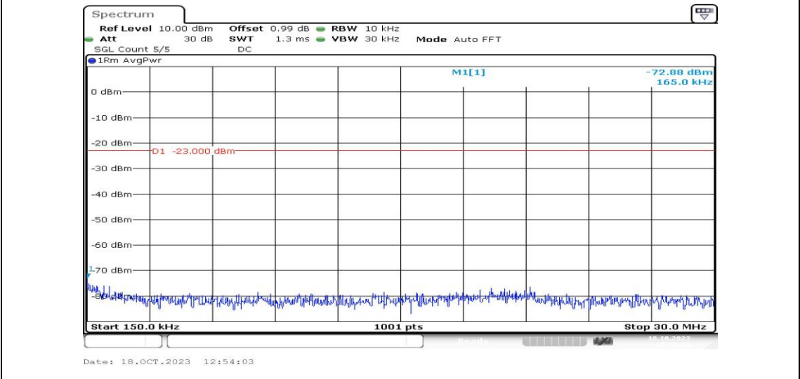
Band4-5MHz-16QAM-20375-1RB#0-Range2:0.15~30MHz-PASS
