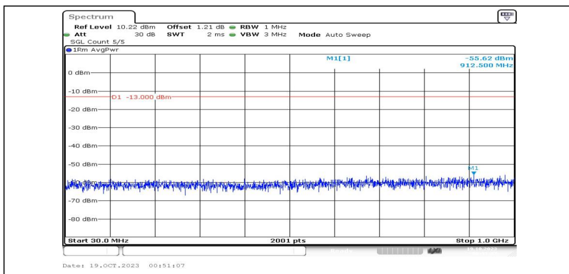
Band4-10MHz-16QAM-20000-1RB#0-Range3:30~1000MHz-PASS
