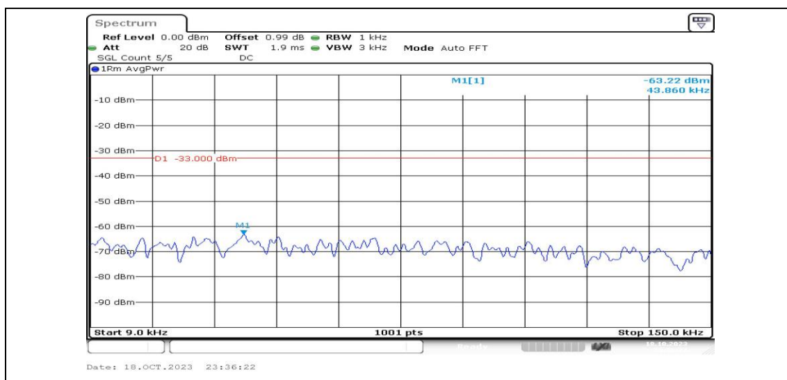
Band4-15MHz-QPSK-20325-1RB#0-Range1:0.009~0.15MHz-PASS
