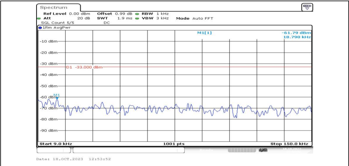
Band4-5MHz-16QAM-20375-1RB#0-Range1:0.009~0.15MHz-PASS
