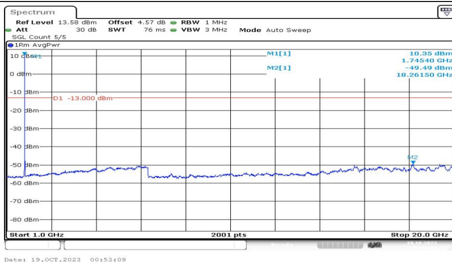
Band4-10MHz-16QAM-20350-1RB#0-Range4:1000~20000MHz-PASS
