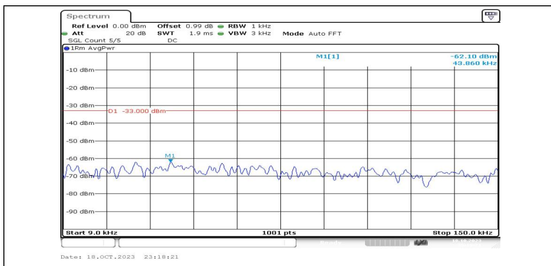
Band4-10MHz-QPSK-20350-1RB#0-Range1:0.009~0.15MHz-PASS
