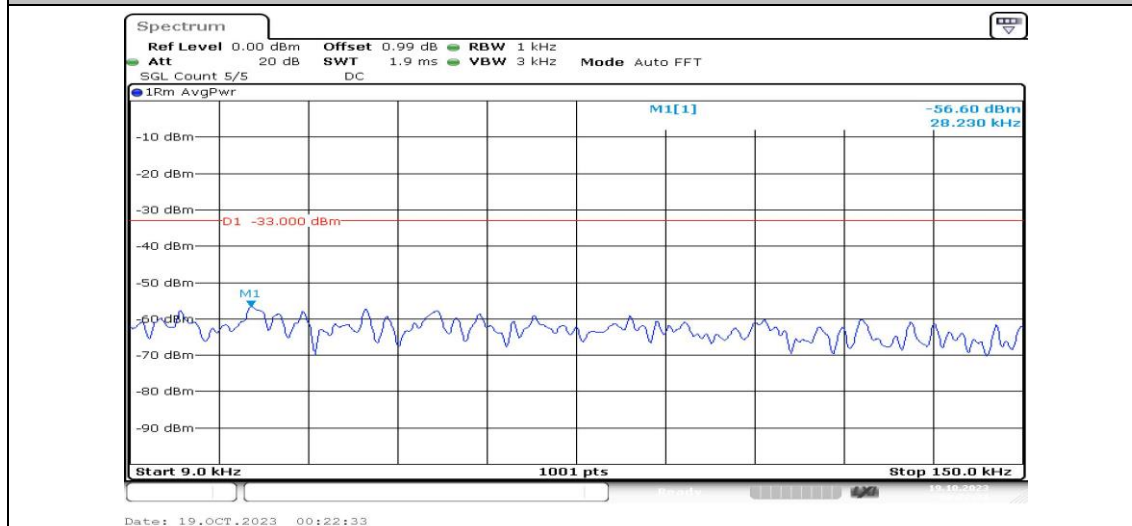
Band4-20MHz-QPSK-20050-1RB#0-Range1:0.009~0.15MHz-PASS
