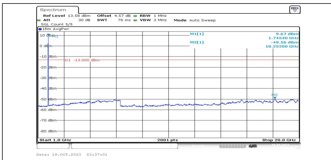
Band4-15MHz-QPSK-20325-1RB#0-Range4:1000~20000MHz-PASS
