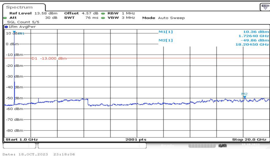
Band4-10MHz-QPSK-20175-1RB#0-Range4:1000~20000MHz-PASS
