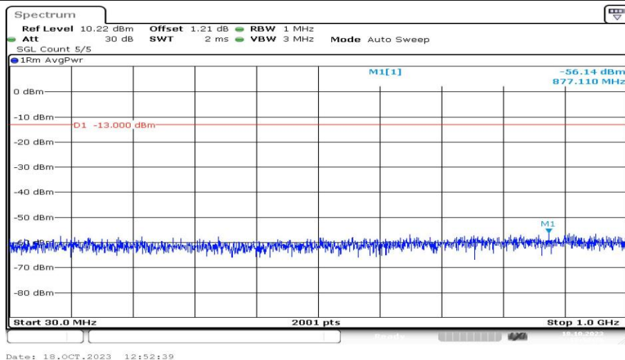
Band4-5MHz-16QAM-20175-1RB#0-Range3:30~1000MHz-PASS
