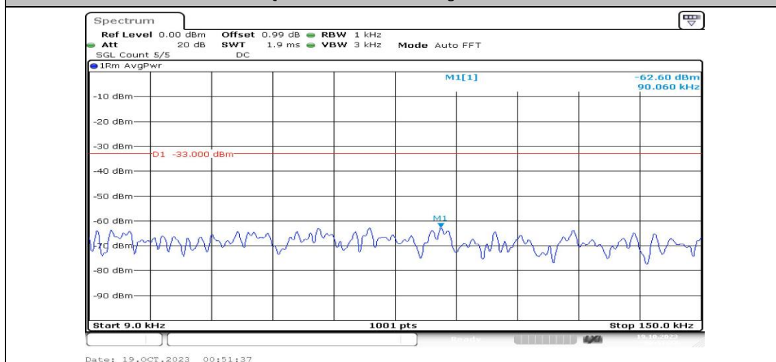
Band4-10MHz-16QAM-20175-1RB#0-Range1:0.009~0.15MHz-PASS
