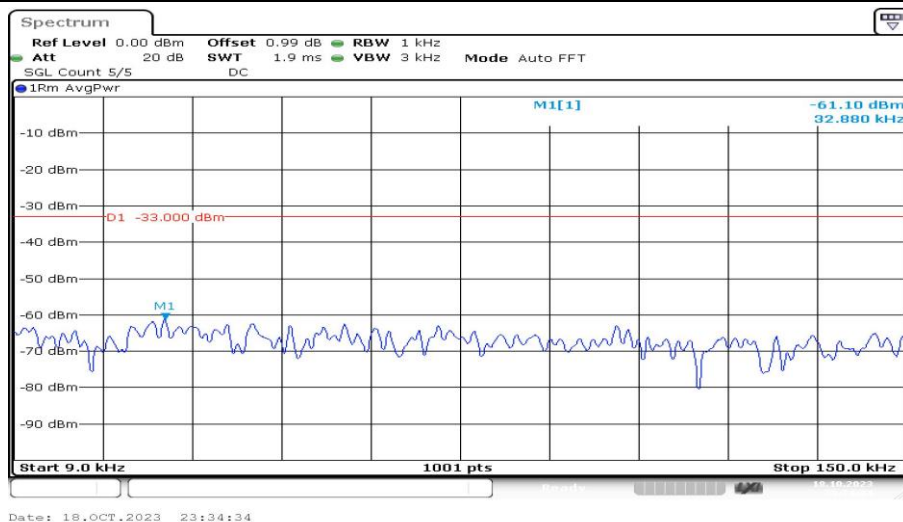
Band4-15MHz-QPSK-20025-1RB#0-Range1:0.009~0.15MHz-PASS
