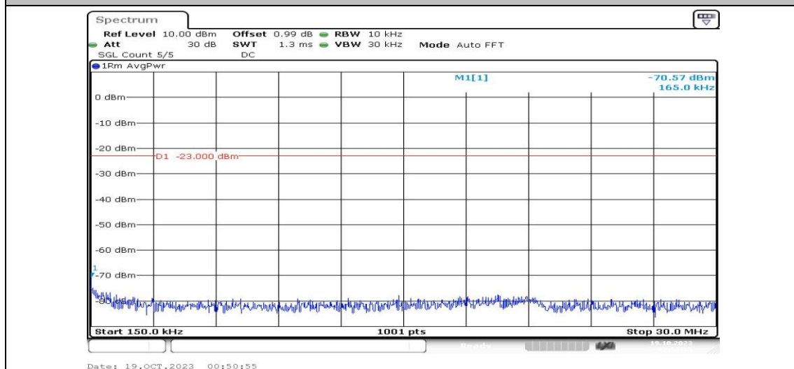
Band4-10MHz-16QAM-20000-1RB#0-Range2:0.15~30MHz-PASS
