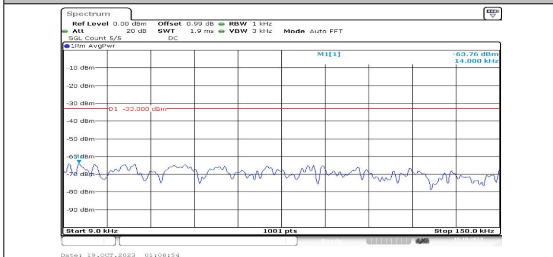
Band4-15MHz-16QAM-20175-1RB#0-Range1:0.009~0.15MHz-PASS
