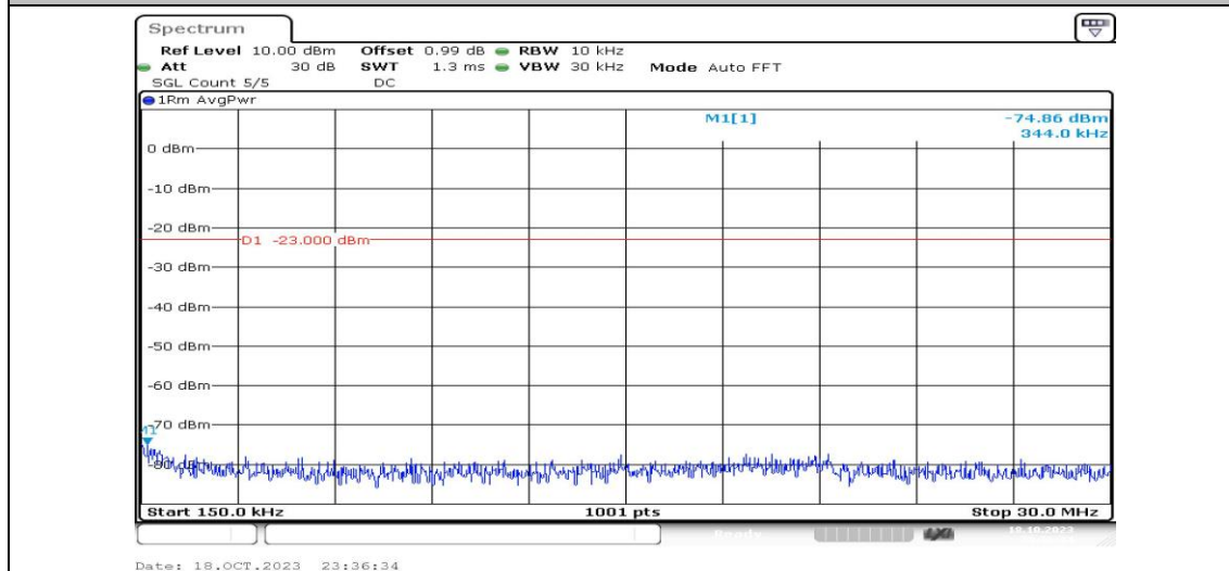
Band4-15MHz-QPSK-20325-1RB#0-Range2:0.15~30MHz-PASS
