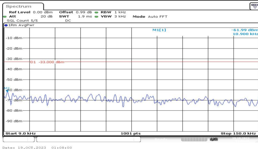
Band4-15MHz-16QAM-20025-1RB#0-Range1:0.009~0.15MHz-PASS
