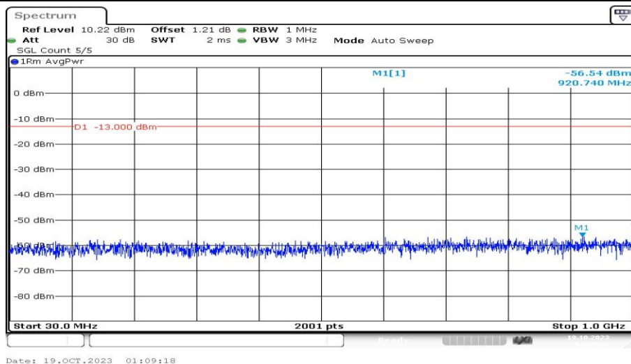
Band4-15MHz-16QAM-20175-1RB#0-Range3:30~1000MHz-PASS
