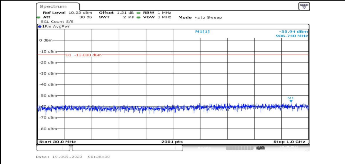
Band4-20MHz-QPSK-20300-1RB#0-Range3:30~1000MHz-PASS
