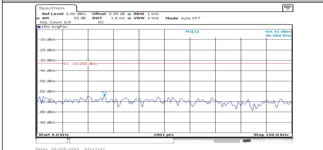
Band4-10MHz-QPSK-20175-1RB#0-Range1:0.009~0.15MHz-PASS
