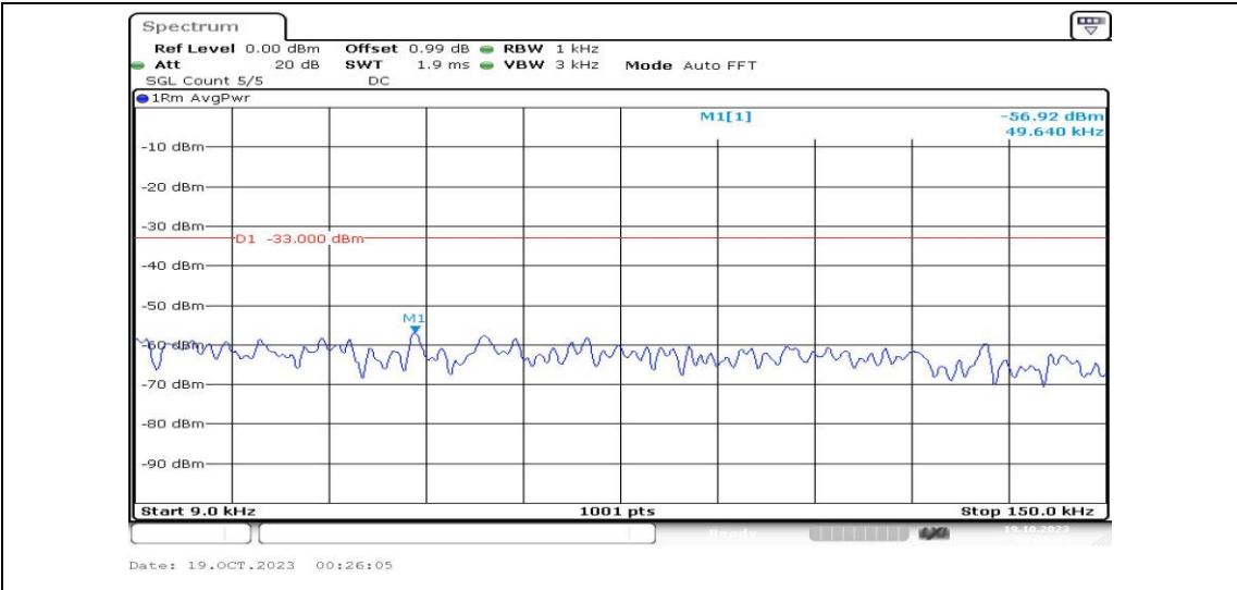
Band4-20MHz-QPSK-20300-1RB#0-Range1:0.009~0.15MHz-PASS
