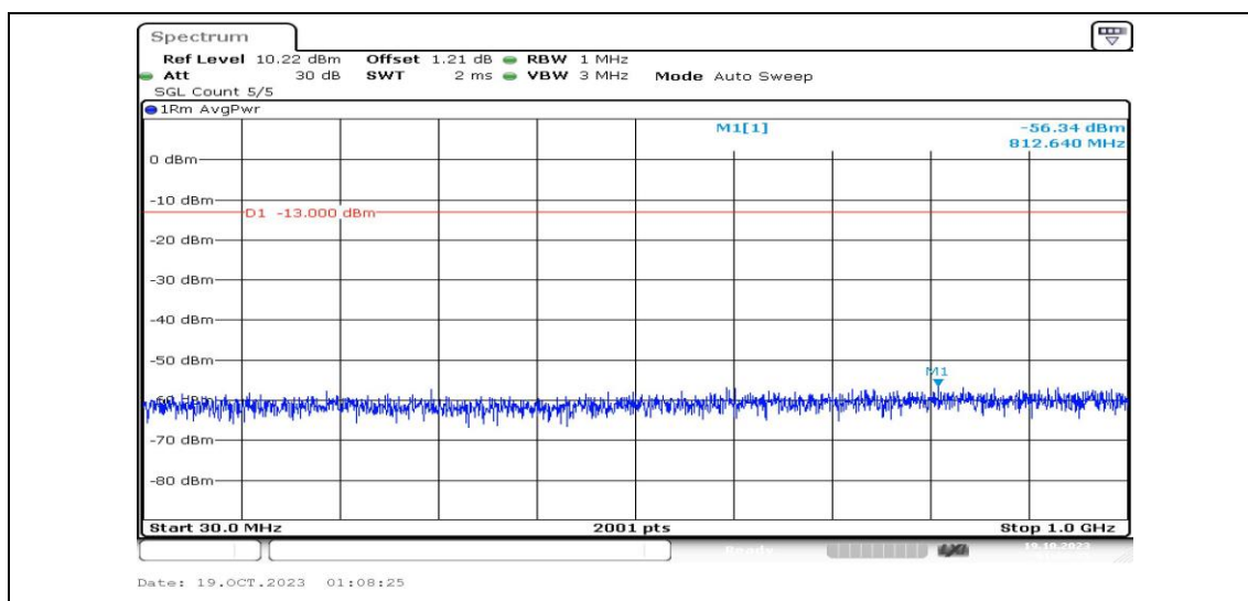
Band4-15MHz-16QAM-20025-1RB#0-Range3:30~1000MHz-PASS
