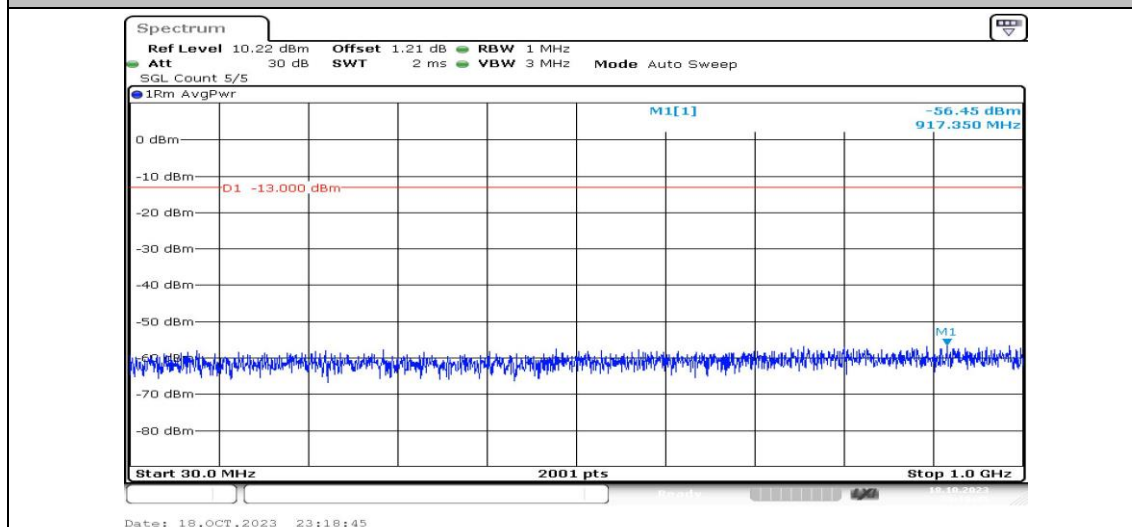
Band4-10MHz-QPSK-20350-1RB#0-Range3:30~1000MHz-PASS
