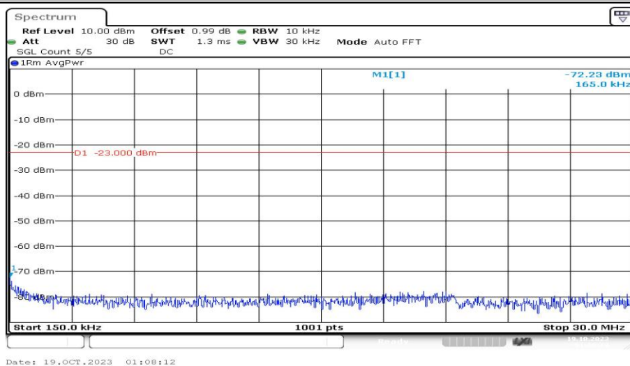
Band4-15MHz-16QAM-20025-1RB#0-Range2:0.15~30MHz-PASS
