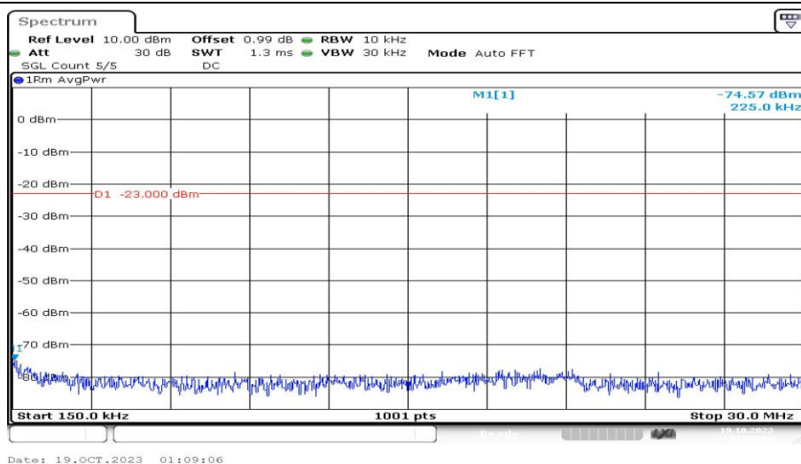
Band4-15MHz-16QAM-20175-1RB#0-Range2:0.15~30MHz-PASS
