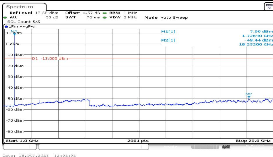
Band4-5MHz-16QAM-20175-1RB#0-Range4:1000~20000MHz-PASS
