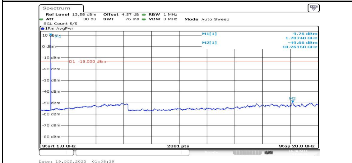
Band4-15MHz-16QAM-20025-1RB#0-Range4:1000~20000MHz-PASS
