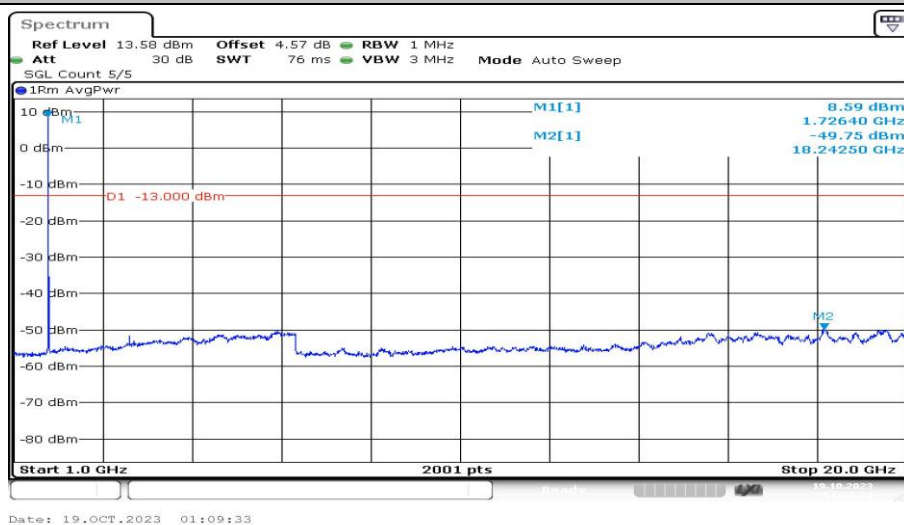
Band4-15MHz-16QAM-20175-1RB#0-Range4:1000~20000MHz-PASS
