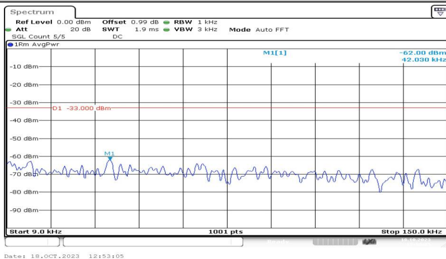
Band4-5MHz-QPSK-20375-1RB#0-Range1:0.009~0.15MHz-PASS
