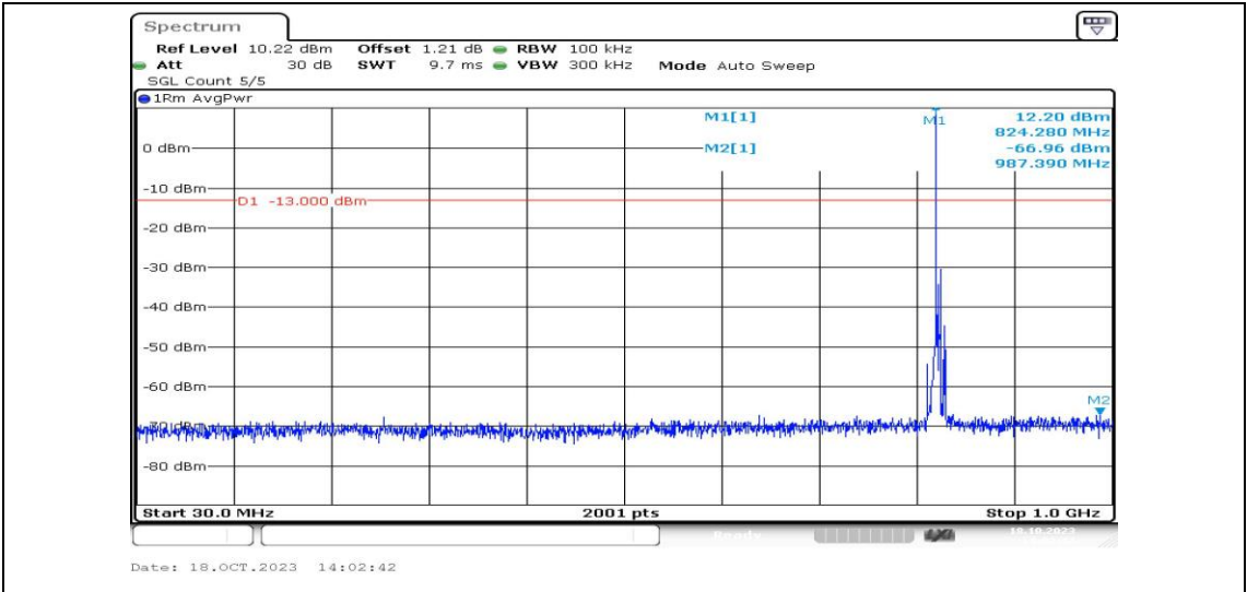
Band5-5MHz-QPSK-20425-1RB#0-Range3:30~1000MHz-PASS
