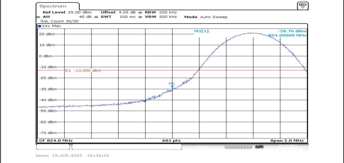
Band5-10MHz-16QAM-20450-1RB#0-PASS
