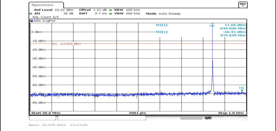
Band5-1.4MHz-QPSK-20643-1RB#0-Range3:30~1000MHz-PASS
