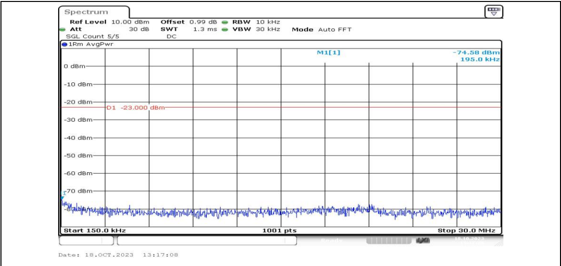
Band5-1.4MHz-QPSK-20643-1RB#0-Range2:0.15~30MHz-PASS
