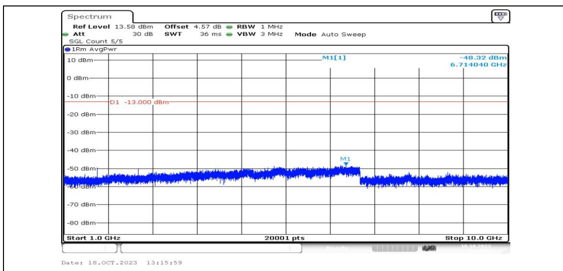
Band5-1.4MHz-QPSK-20525-1RB#0-Range4:1000~10000MHz-PASS
