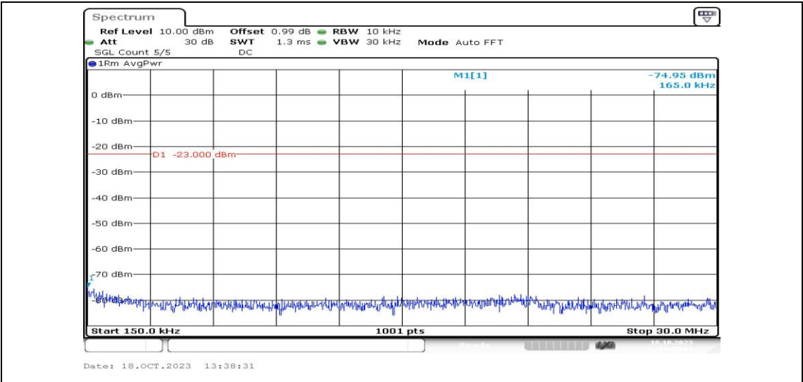
Band5-3MHz-16QAM-20415-1RB#0-Range2:0.15~30MHz-PASS
