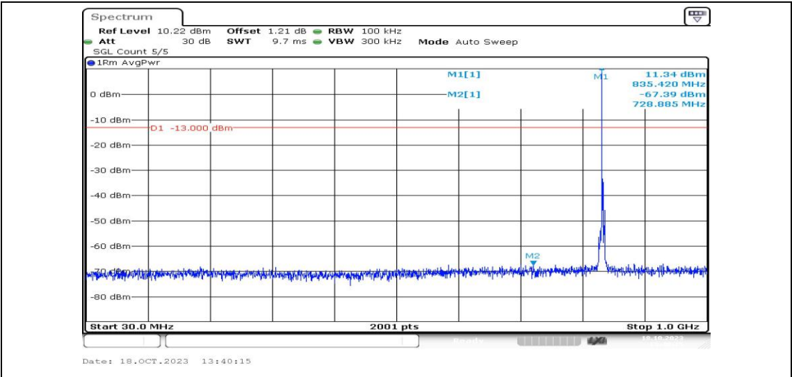
Band5-3MHz-16QAM-20525-1RB#0-Range3:30~1000MHz-PASS
