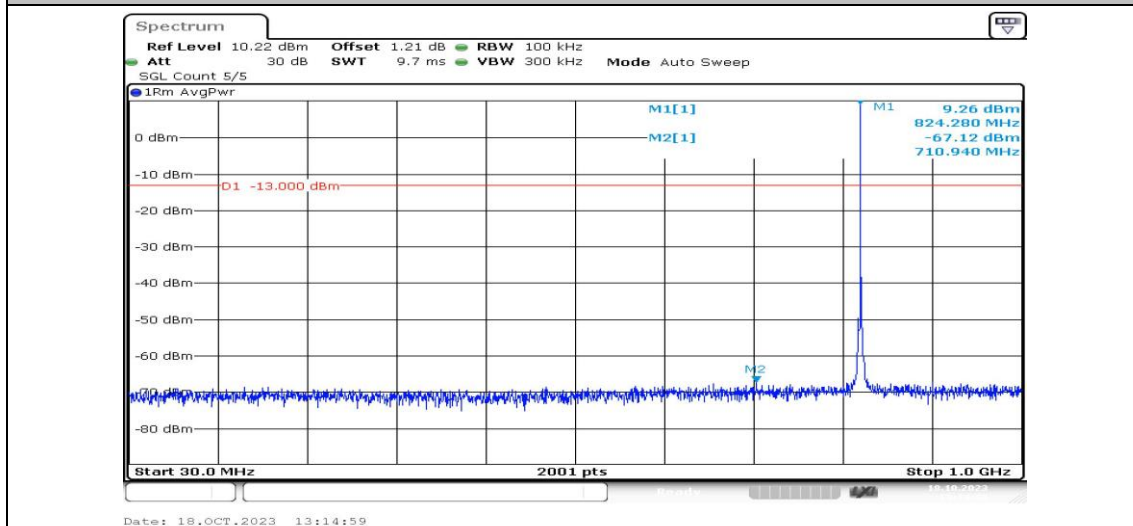
Band5-1.4MHz-16QAM-20407-1RB#0-Range3:30~1000MHz-PASS
