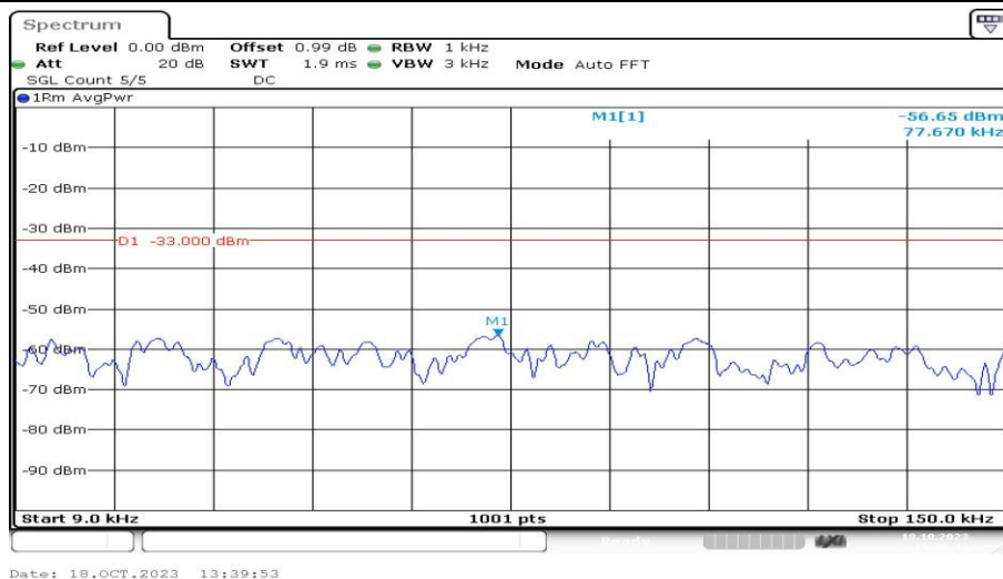
Band5-3MHz-16QAM-20525-1RB#0-Range1:0.009~0.15MHz-PASS
