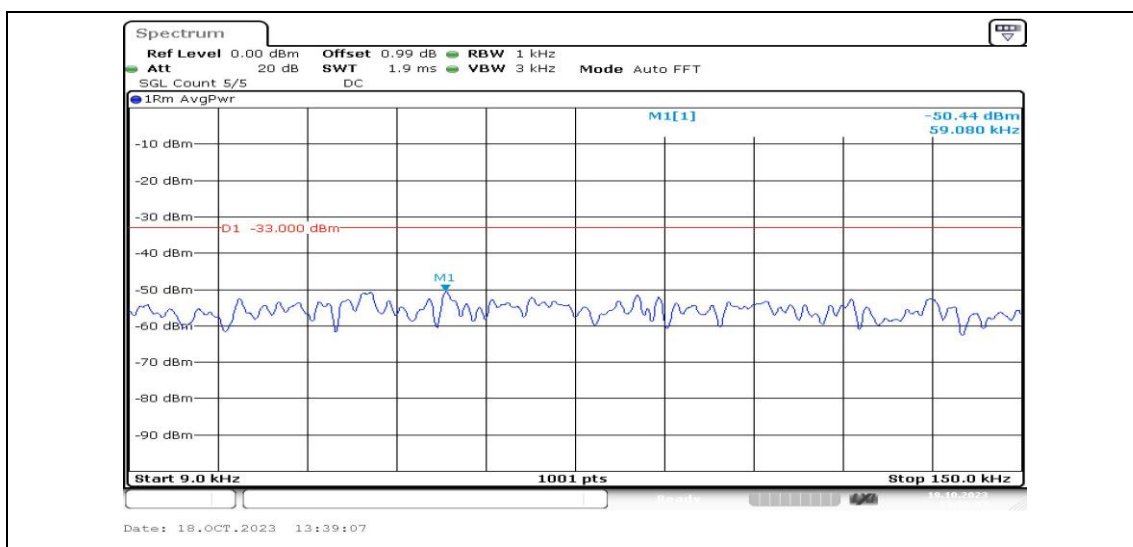
Band5-3MHz-QPSK-20525-1RB#0-Range1:0.009~0.15MHz-PASS
