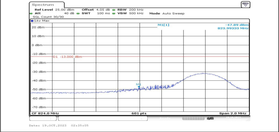
Band5-10MHz-16QAM-20450-1RB#49-PASS
