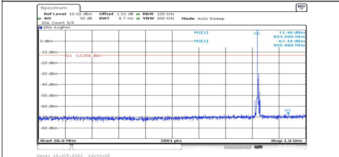
Band5-5MHz-16QAM-20425-1RB#0-Range3:30~1000MHz-PASS
