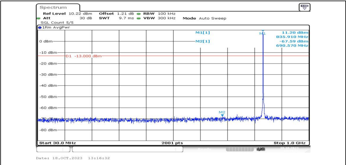
Band5-1.4MHz-16QAM-20525-1RB#0-Range3:30~1000MHz-PASS
