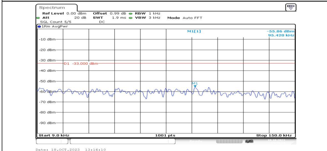
Band5-1.4MHz-16QAM-20525-1RB#0-Range1:0.009~0.15MHz-PASS
