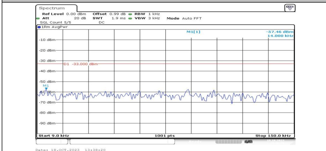
Band5-3MHz-16QAM-20415-1RB#0-Range1:0.009~0.15MHz-PASS
