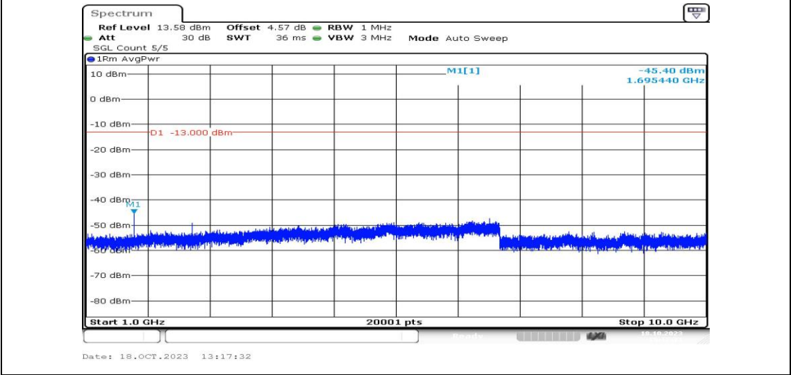
Band5-1.4MHz-QPSK-20643-1RB#0-Range4:1000~10000MHz-PASS
