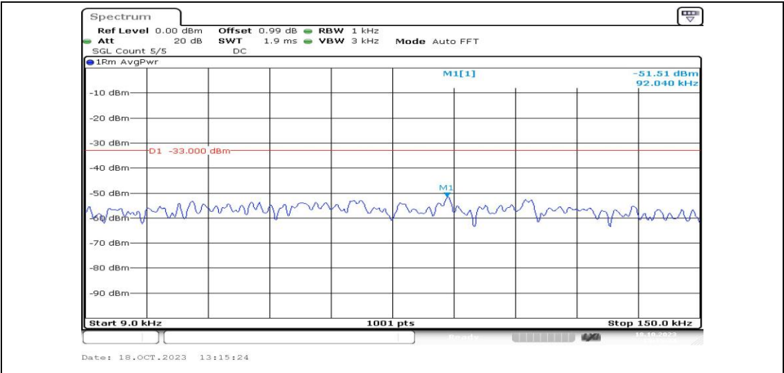
Band5-1.4MHz-QPSK-20525-1RB#0-Range1:0.009~0.15MHz-PASS
