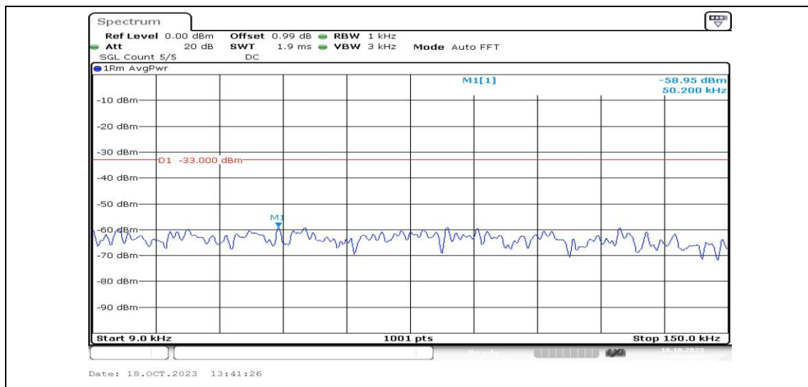
Band5-3MHz-16QAM-20635-1RB#0-Range1:0.009~0.15MHz-PASS
