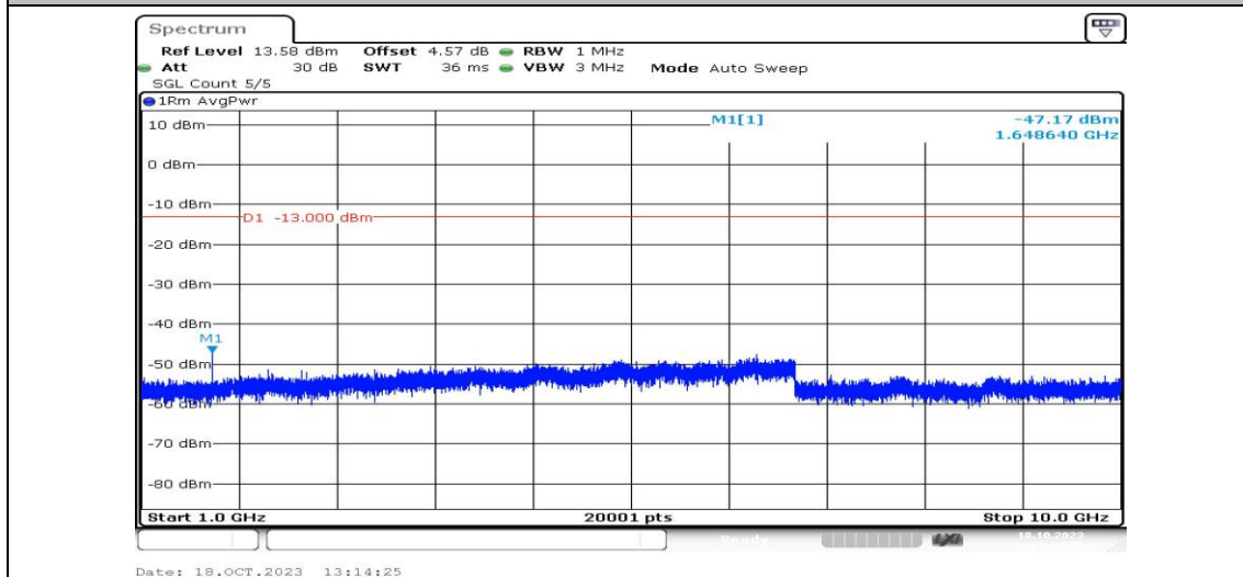
Band5-1.4MHz-QPSK-20407-1RB#0-Range4:1000~10000MHz-PASS
