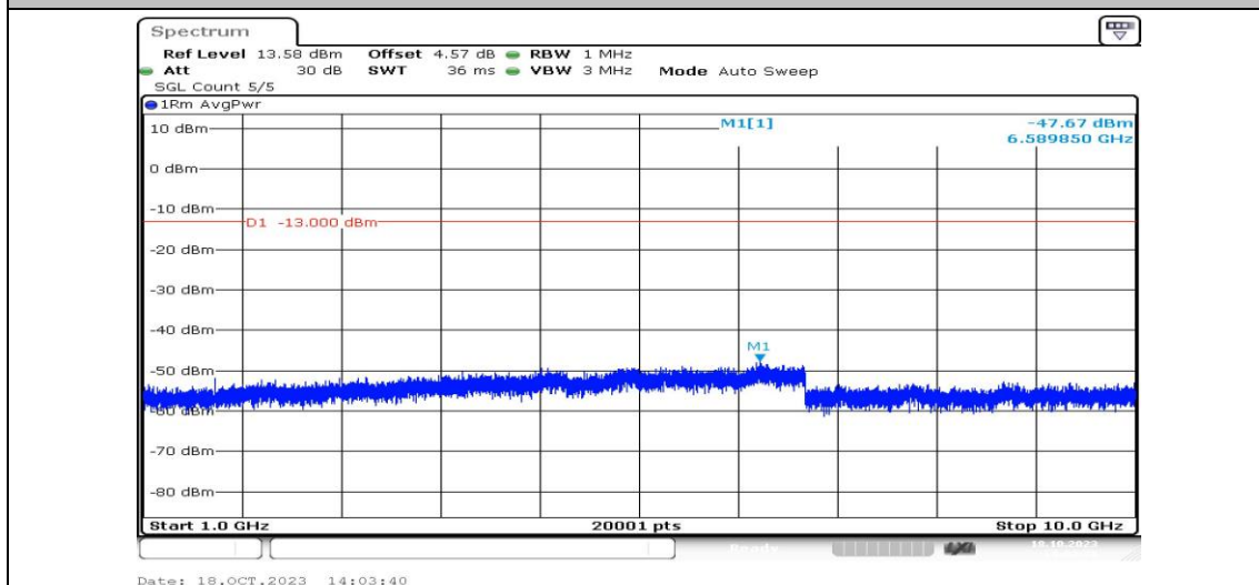
Band5-5MHz-16QAM-20425-1RB#0-Range4:1000~10000MHz-PASS
