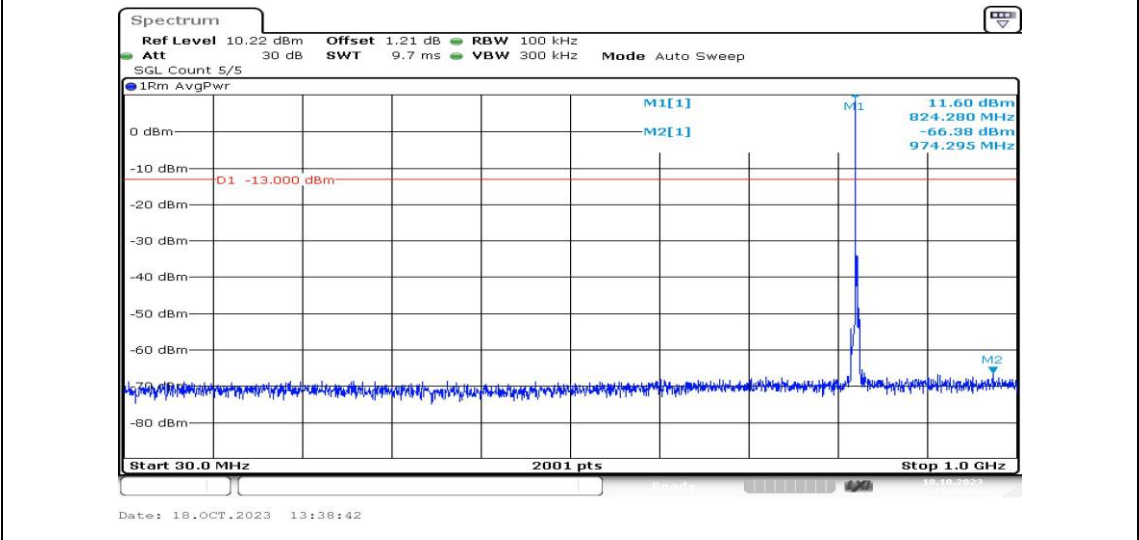
Band5-3MHz-16QAM-20415-1RB#0-Range3:30~1000MHz-PASS
