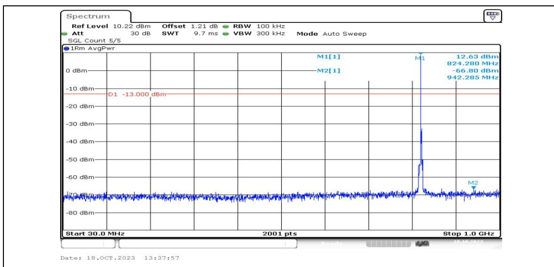
Band5-3MHz-QPSK-20415-1RB#0-Range3:30~1000MHz-PASS
