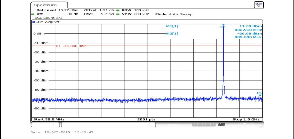
Band5-1.4MHz-QPSK-20525-1RB#0-Range3:30~1000MHz-PASS
