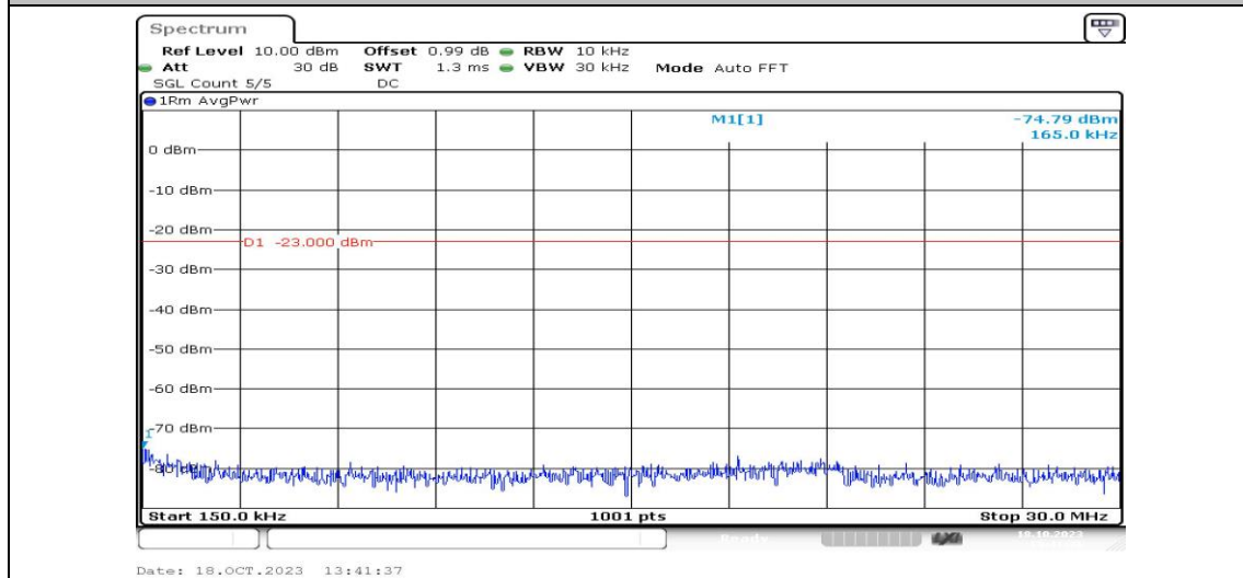
Band5-3MHz-16QAM-20635-1RB#0-Range2:0.15~30MHz-PASS
