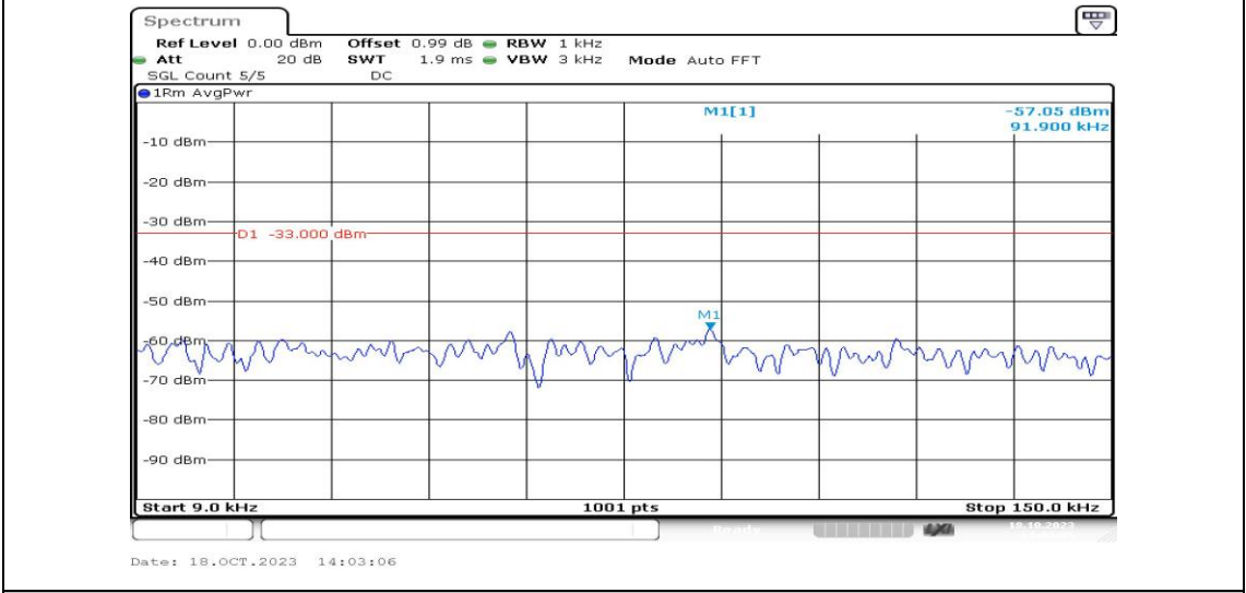
Band5-5MHz-16QAM-20425-1RB#0-Range1:0.009~0.15MHz-PASS
