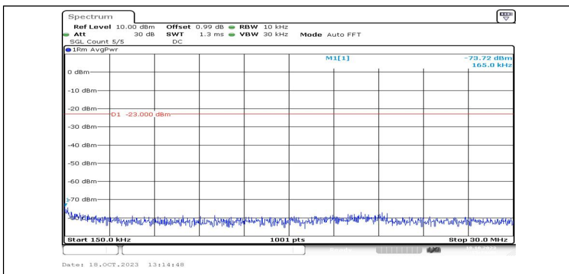
Band5-1.4MHz-16QAM-20407-1RB#0-Range2:0.15~30MHz-PASS
