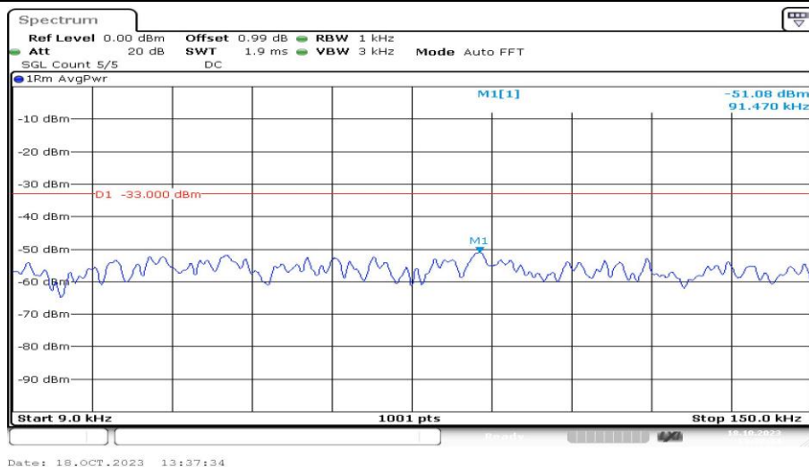
Band5-3MHz-QPSK-20415-1RB#0-Range1:0.009~0.15MHz-PASS
