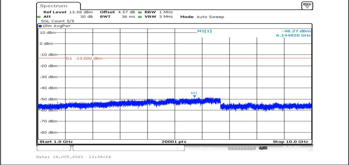
Band5-3MHz-16QAM-20415-1RB#0-Range4:1000~10000MHz-PASS
