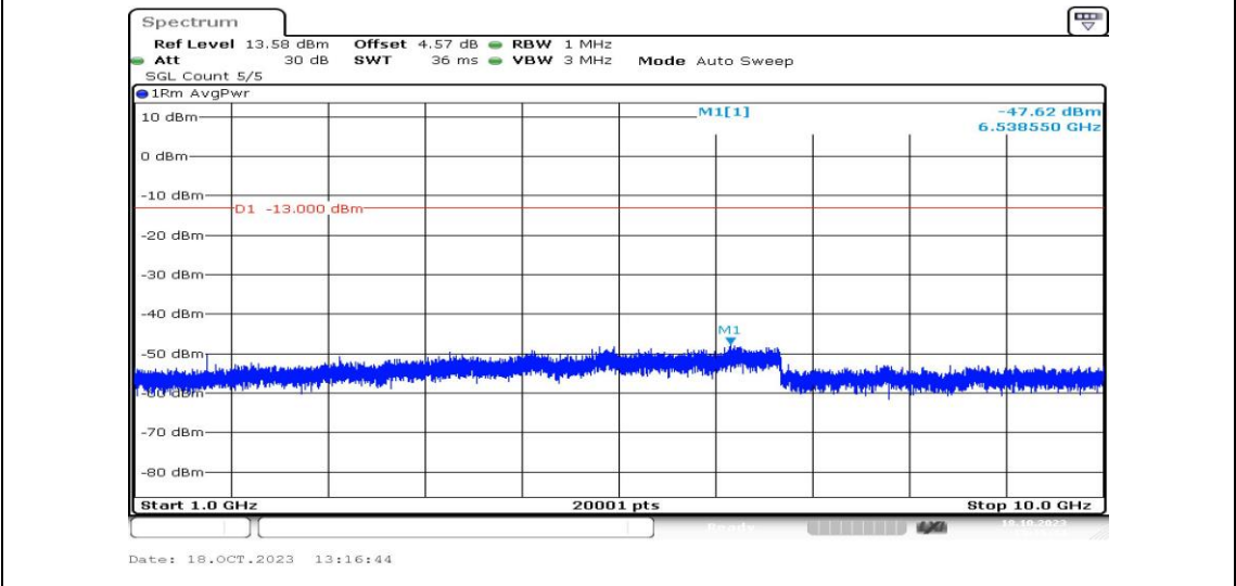
Band5-1.4MHz-16QAM-20525-1RB#0-Range4:1000~10000MHz-PASS
