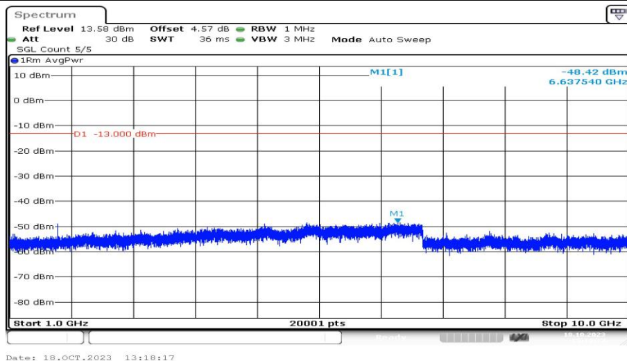
Band5-1.4MHz-16QAM-20643-1RB#0-Range4:1000~10000MHz-PASS
