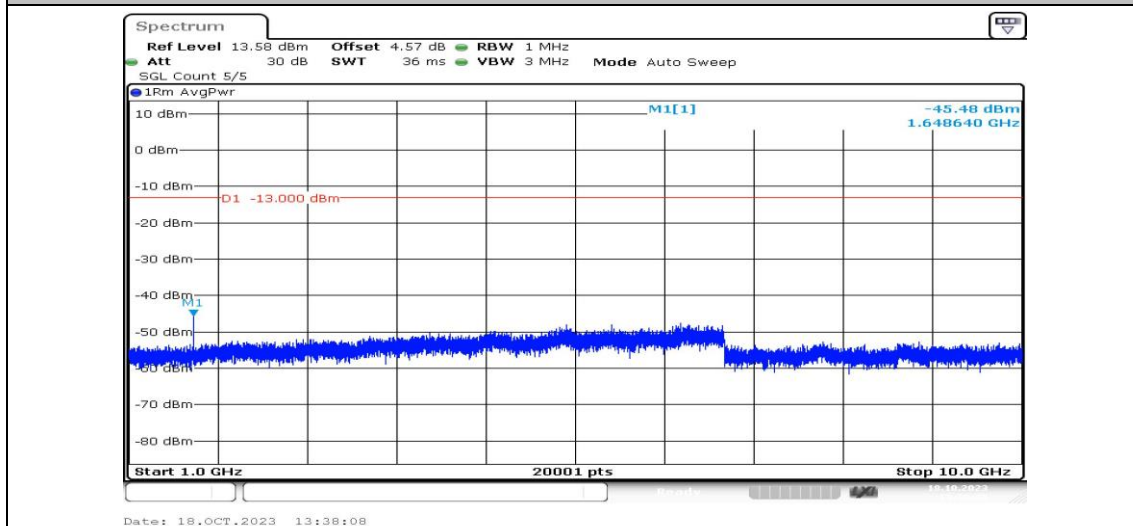
Band5-3MHz-QPSK-20415-1RB#0-Range4:1000~10000MHz-PASS
