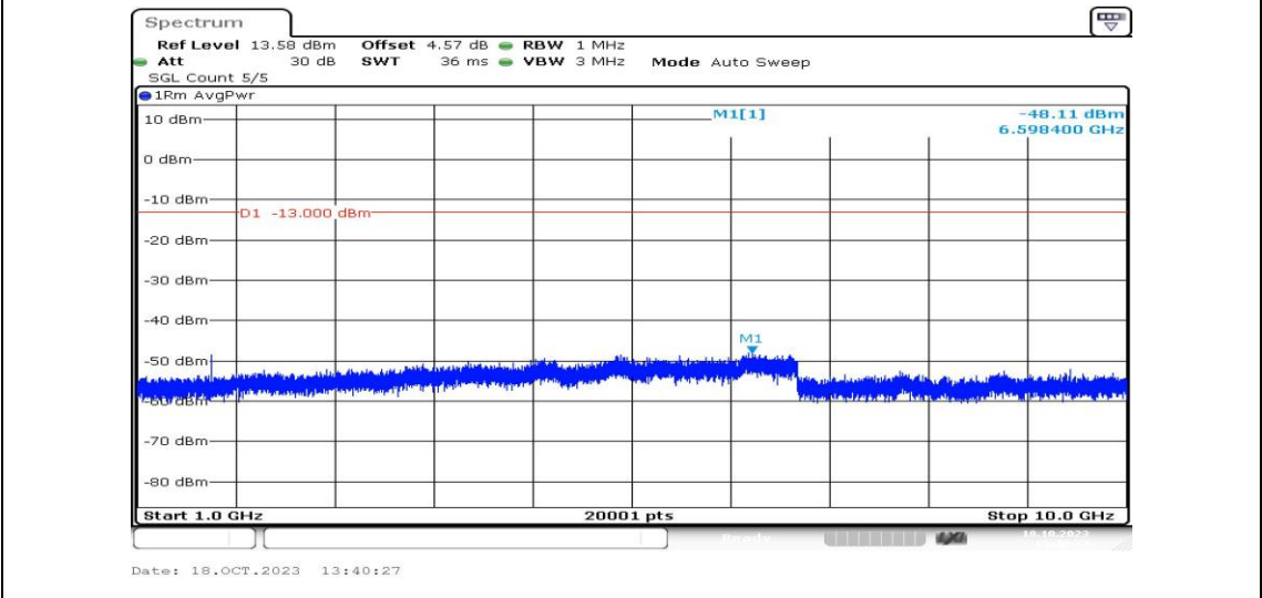
Band5-3MHz-16QAM-20525-1RB#0-Range4:1000~10000MHz-PASS
