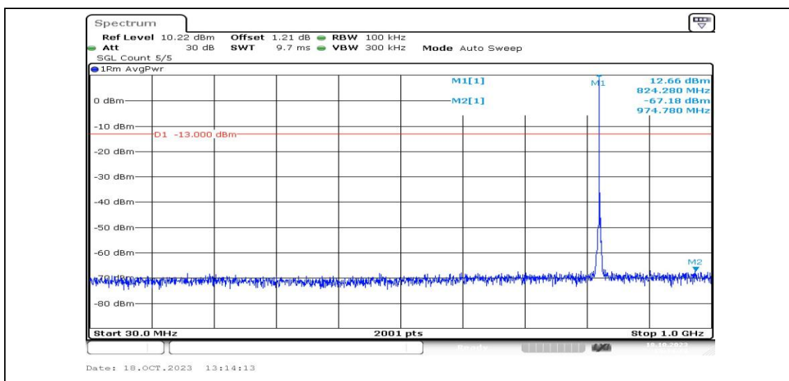
Band5-1.4MHz-QPSK-20407-1RB#0-Range3:30~1000MHz-PASS
