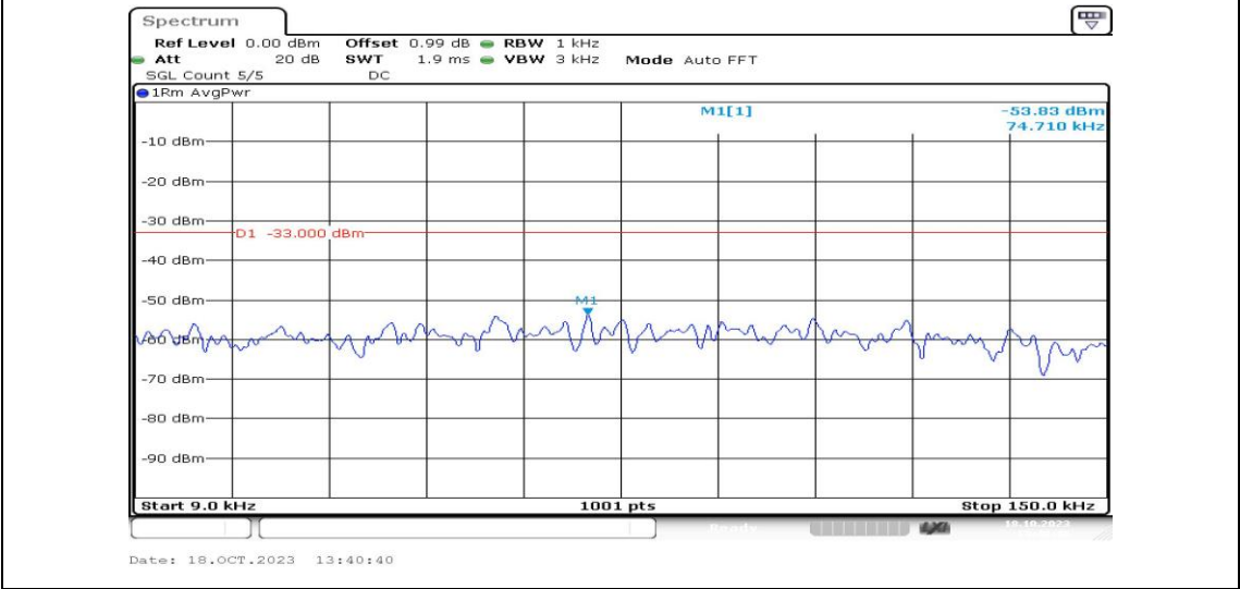
Band5-3MHz-QPSK-20635-1RB#0-Range1:0.009~0.15MHz-PASS
