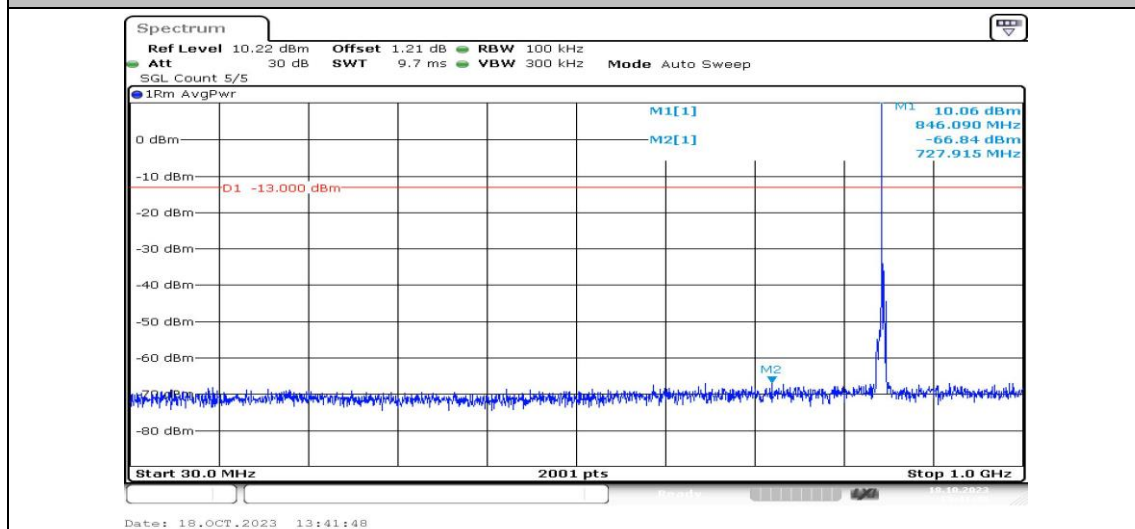
Band5-3MHz-16QAM-20635-1RB#0-Range3:30~1000MHz-PASS
