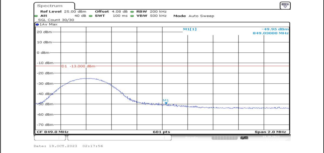
Band5-10MHz-QPSK-20600-1RB#0-PASS
