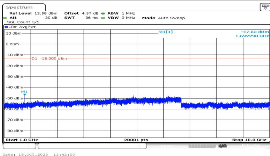
Band5-3MHz-16QAM-20635-1RB#0-Range4:1000~10000MHz-PASS
