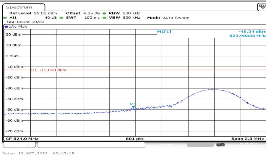
Band5-10MHz-QPSK-20450-1RB#49-PASS
