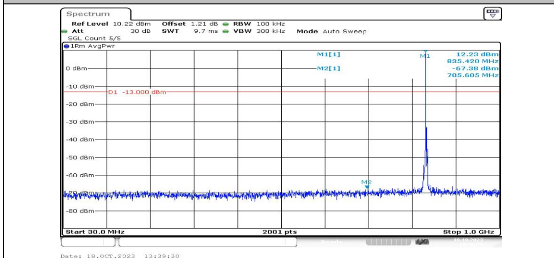
Band5-3MHz-QPSK-20525-1RB#0-Range3:30~1000MHz-PASS
