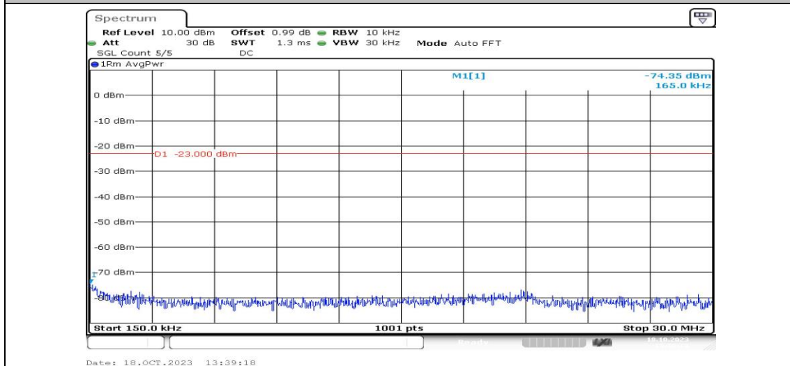
Band5-3MHz-QPSK-20525-1RB#0-Range2:0.15~30MHz-PASS
