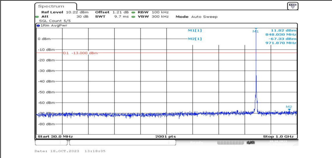
Band5-1.4MHz-16QAM-20643-1RB#0-Range3:30~1000MHz-PASS
