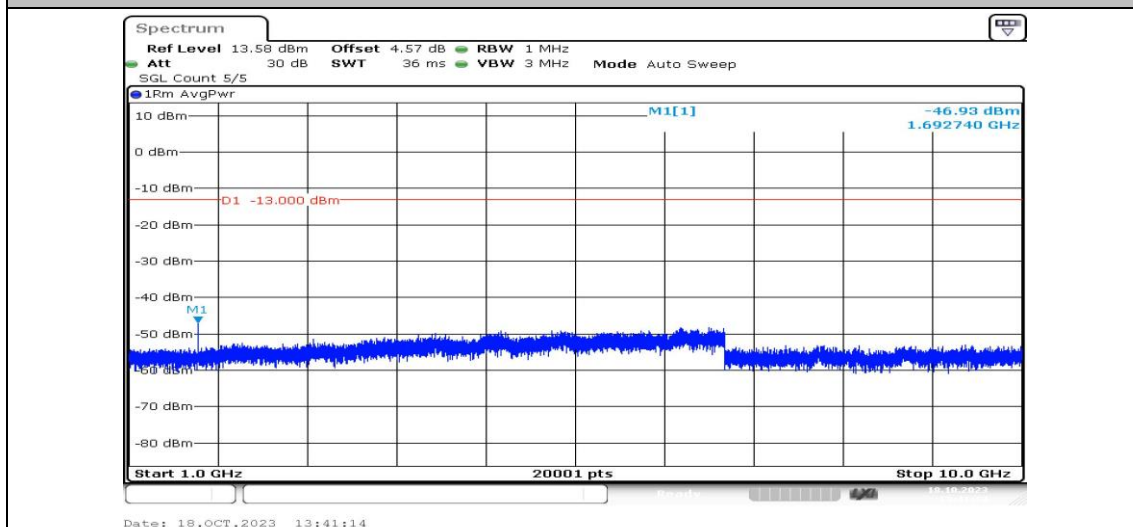
Band5-3MHz-QPSK-20635-1RB#0-Range4:1000~10000MHz-PASS
