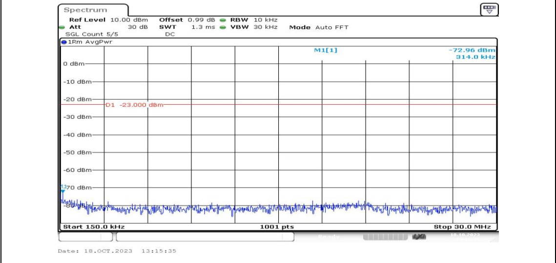
Band5-1.4MHz-QPSK-20525-1RB#0-Range2:0.15~30MHz-PASS
