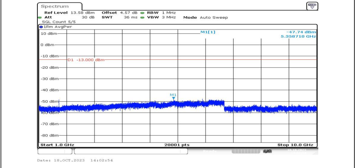
Band5-5MHz-QPSK-20425-1RB#0-Range4:1000~10000MHz-PASS
