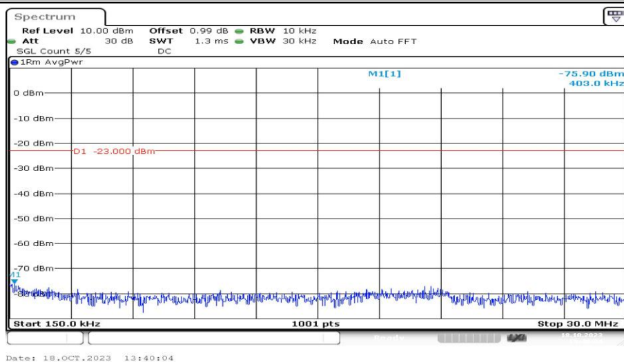
Band5-3MHz-16QAM-20525-1RB#0-Range2:0.15~30MHz-PASS
