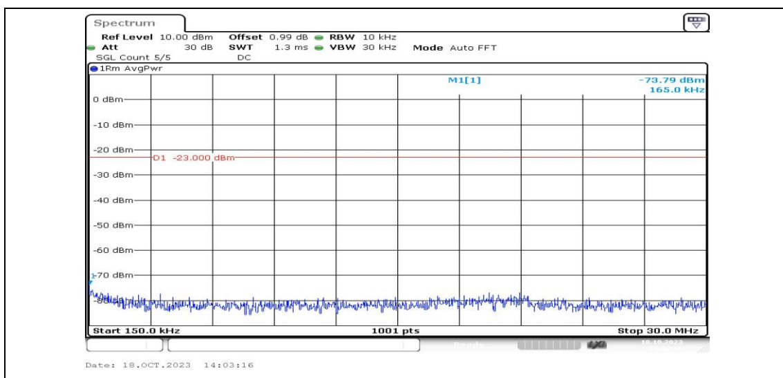
Band5-5MHz-16QAM-20425-1RB#0-Range2:0.15~30MHz-PASS
