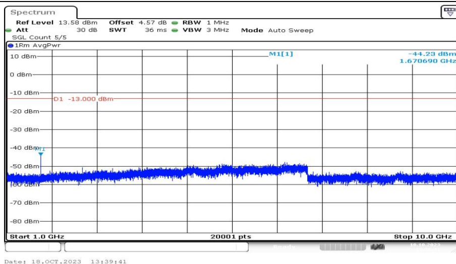
Band5-3MHz-QPSK-20525-1RB#0-Range4:1000~10000MHz-PASS
