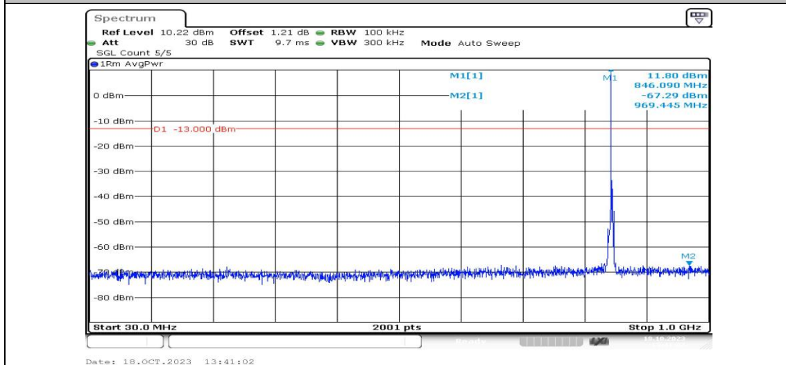
Band5-3MHz-QPSK-20635-1RB#0-Range3:30~1000MHz-PASS
