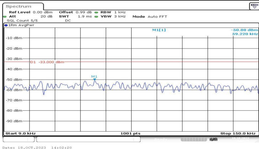
Band5-5MHz-QPSK-20425-1RB#0-Range1:0.009~0.15MHz-PASS
