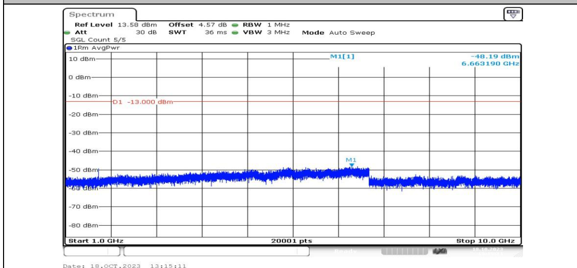
Band5-1.4MHz-16QAM-20407-1RB#0-Range4:1000~10000MHz-PASS
