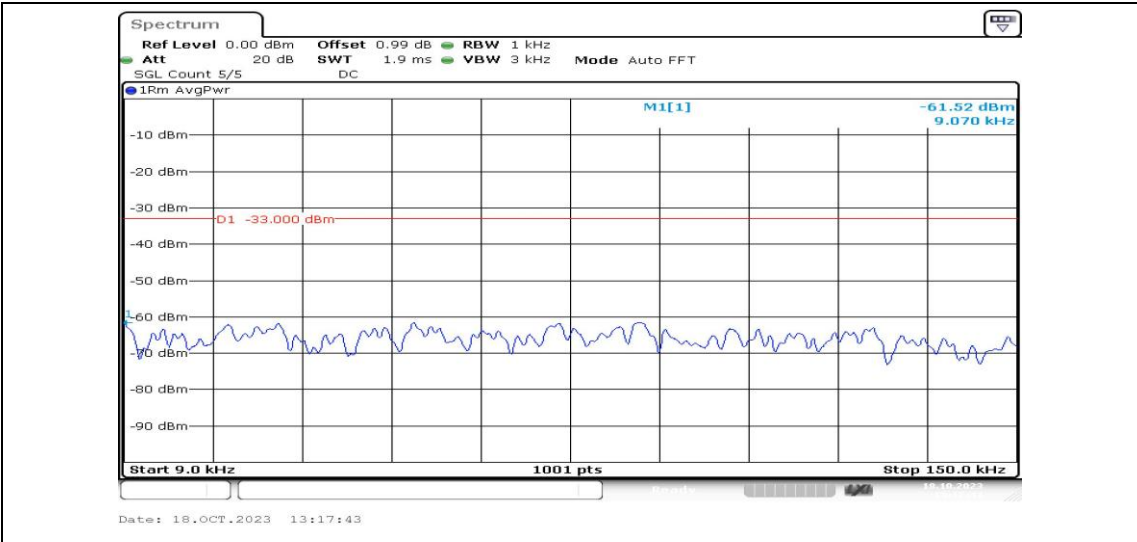
Band5-1.4MHz-16QAM-20643-1RB#0-Range1:0.009~0.15MHz-PASS
