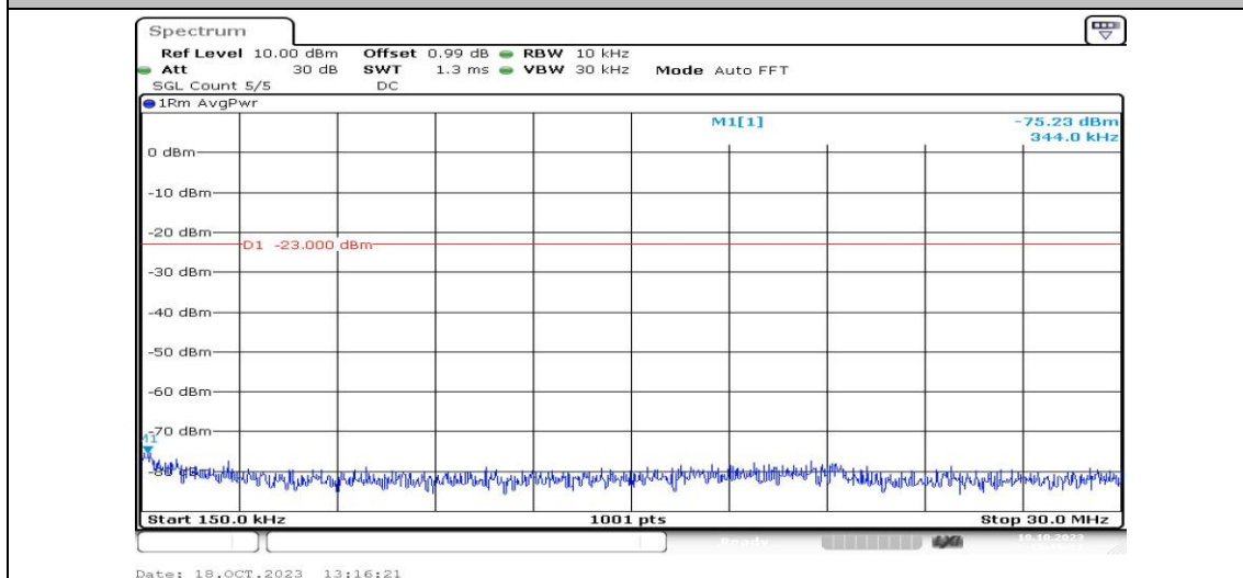
Band5-1.4MHz-16QAM-20525-1RB#0-Range2:0.15~30MHz-PASS
