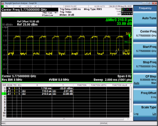
NTNV-11AC80MIMO-Ant2-5775
