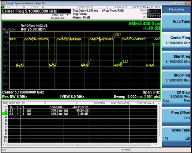
NTNV-11AX20MIMO-Ant1-5180
