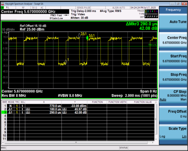
NTNV-11AC40MIMO-Ant1-5670
