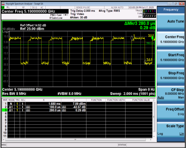
NTNV-11AC40MIMO-Ant1-5190
