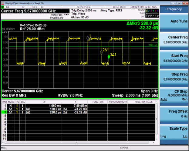
NTNV-11AC40MIMO-Ant2-5670
