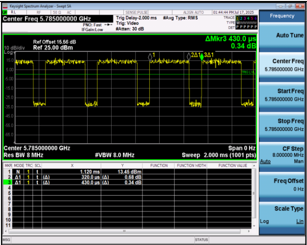
NTNV-11AC20MIMO-Ant2-5785
