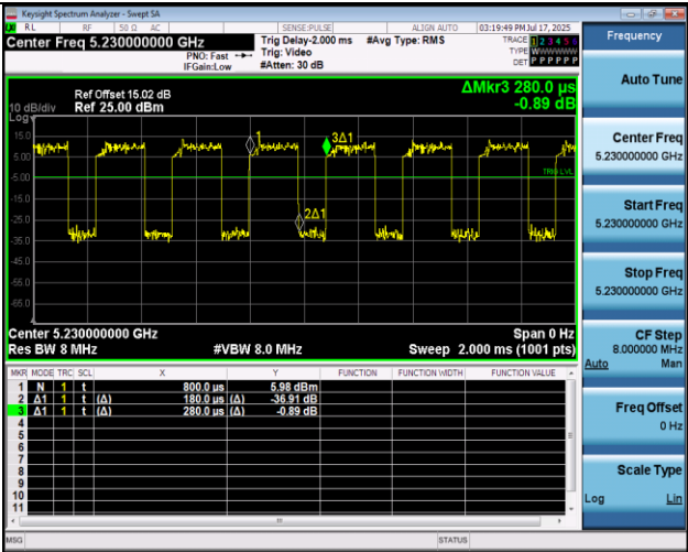
NTNV-11AC40MIMO-Ant2-5230
