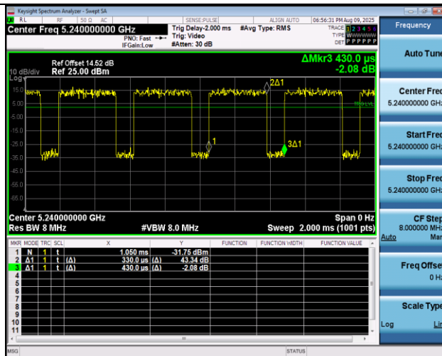
NTNV-11AX20MIMO-Ant2-5240
