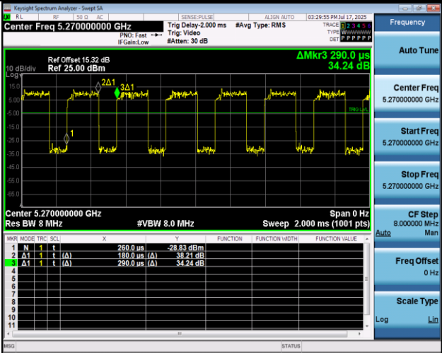
NTNV-11AC40MIMO-Ant2-5270
