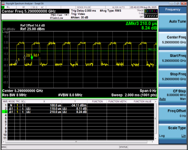
NTNV-11AC80MIMO-Ant1-5290
