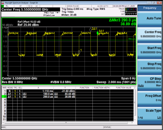
NTNV-11AC40MIMO-Ant1-5550
