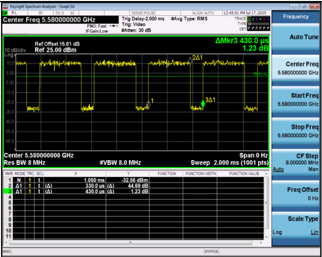
NTNV-11AC20MIMO-Ant2-5580
