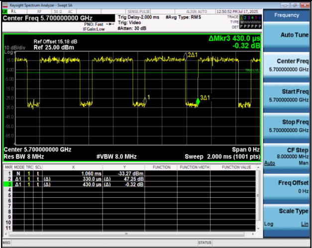
NTNV-11AC20MIMO-Ant1-5700
