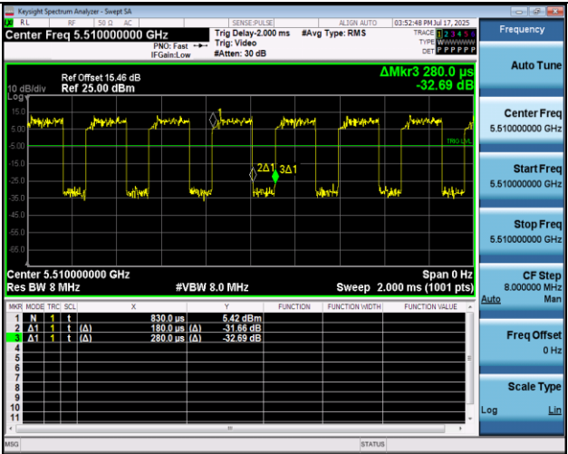
NTNV-11AC40MIMO-Ant2-5510
