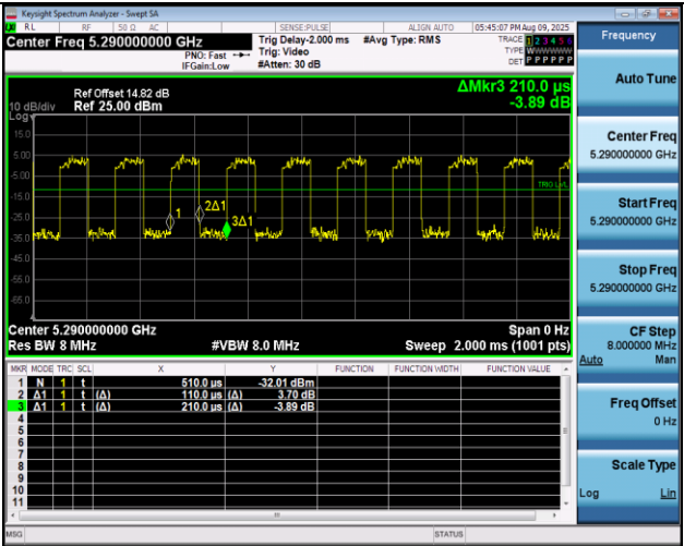
NTNV-11AC80MIMO-Ant2-5290
