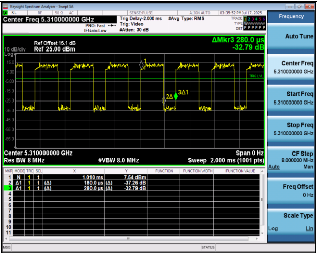
NTNV-11AC40MIMO-Ant1-5310
