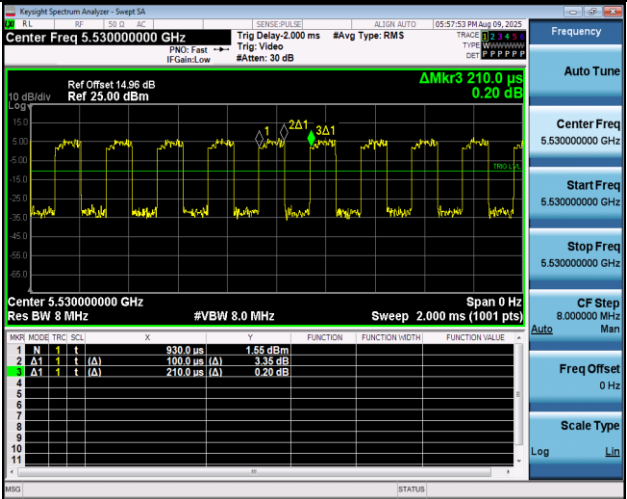
NTNV-11AC80MIMO-Ant2-5530
