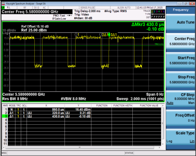
NTNV-11AC20MIMO-Ant1-5580
