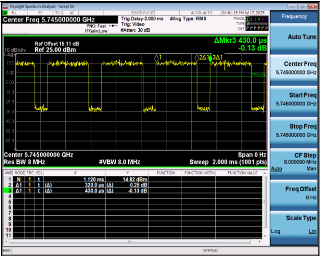
NTNV-11AC20MIMO-Ant1-5745
