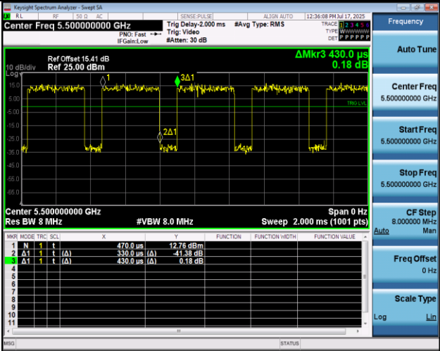
NTNV-11AC20MIMO-Ant2-5500
