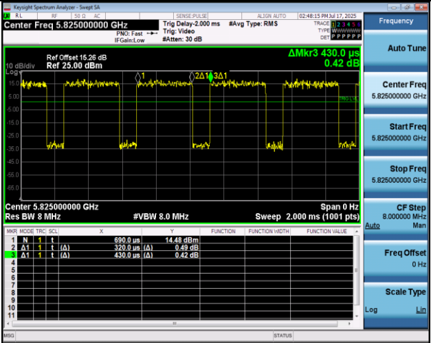
NTNV-11AC20MIMO-Ant1-5825
