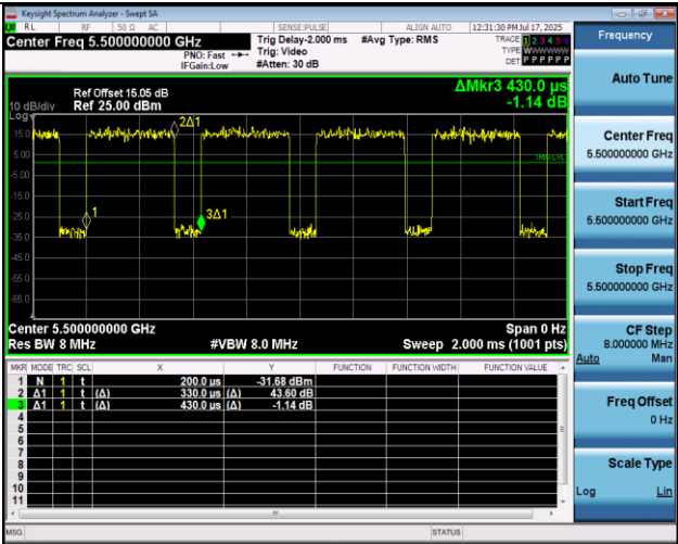
NTNV-11AC20MIMO-Ant1-5500
