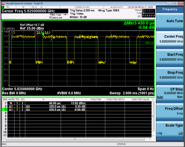
NTNV-11AC20MIMO-Ant2-5825
