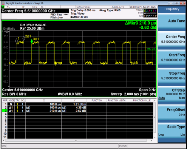
NTNV-11AC80MIMO-Ant2-5610
