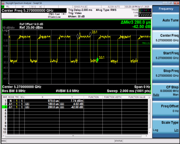
NTNV-11AC40MIMO-Ant1-5270
