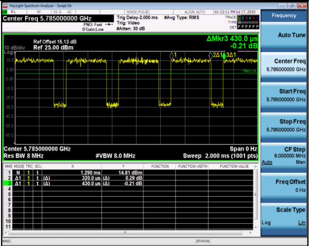
NTNV-11AC20MIMO-Ant1-5785
