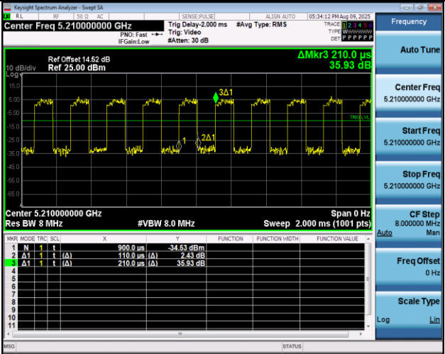
NTNV-11AC80MIMO-Ant2-5210
