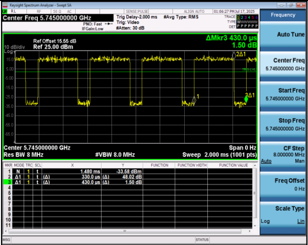
NTNV-11AC20MIMO-Ant2-5745
