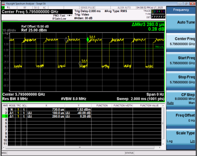
NTNV-11AC40MIMO-Ant2-5795
