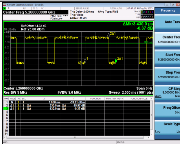
NTNV-11AX20MIMO-Ant2-5260
