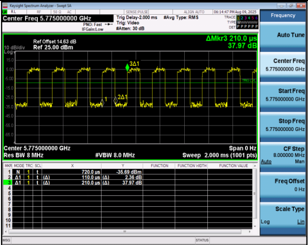
NTNV-11AC80MIMO-Ant1-5775
