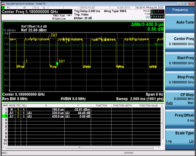
NTNV-11AX20MIMO-Ant2-5180
