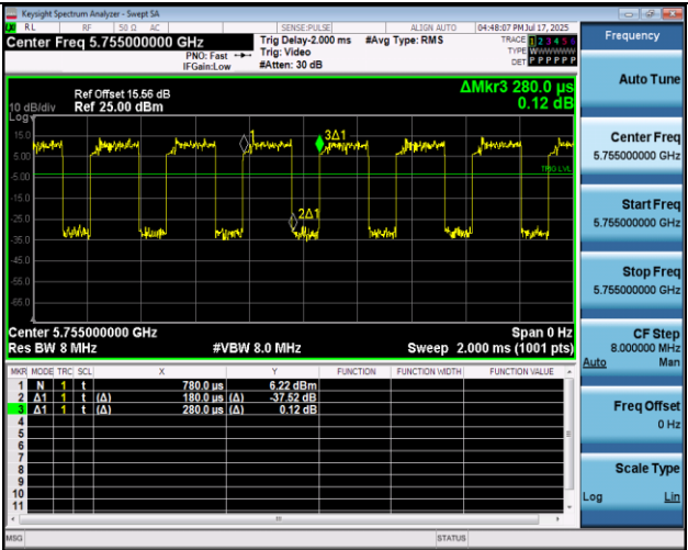
NTNV-11AC40MIMO-Ant2-5755
