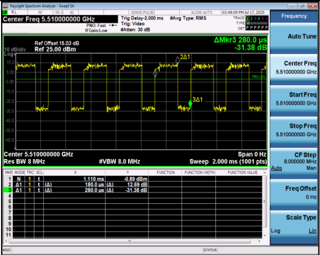
NTNV-11AC40MIMO-Ant1-5510
