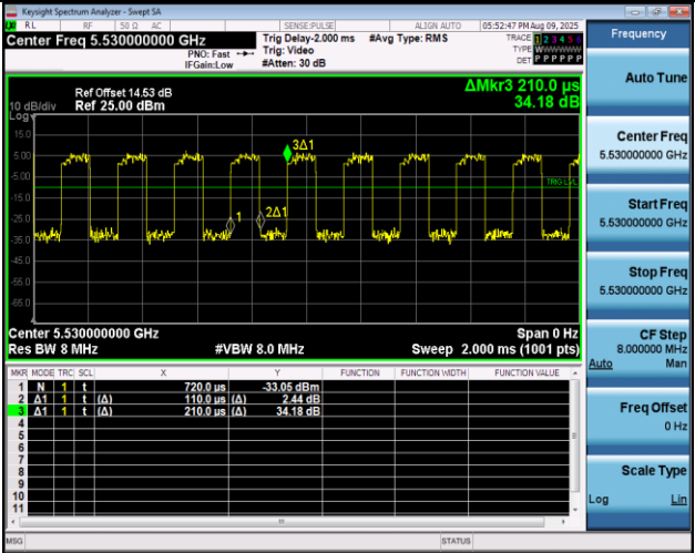
NTNV-11AC80MIMO-Ant1-5530
