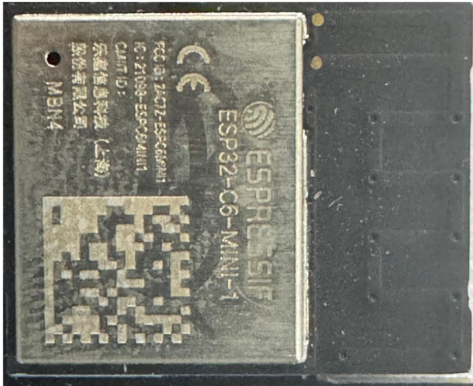
Internal Photo
