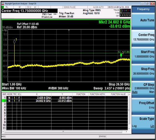
11N40SISO-Ant1-2422-1000~26500-PASS
