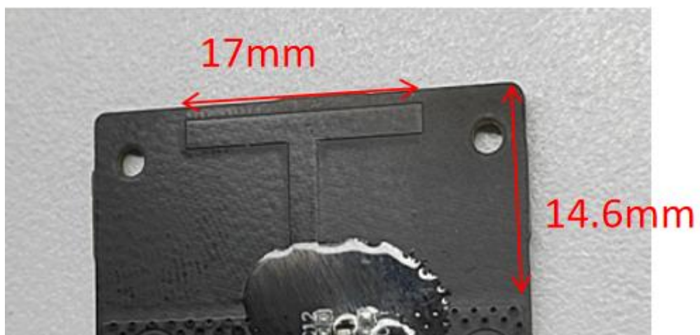
Onboard Antenna Physical Size (unit: mm)
