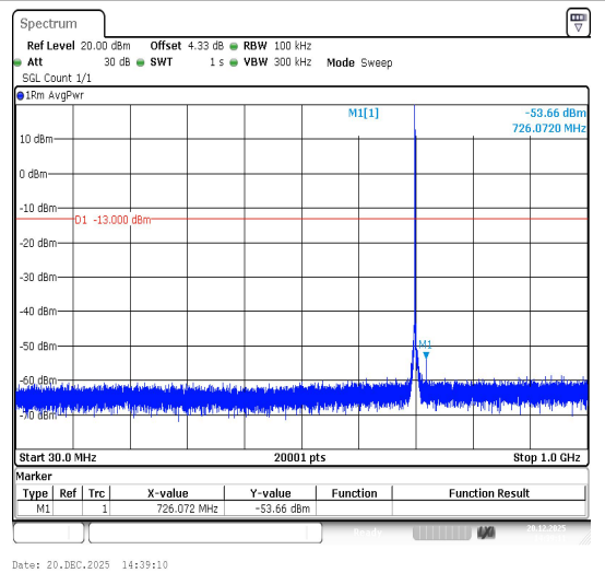
Band12-1.4MHz-16QAM-23095-1RB#0-30~1000-P ASS
