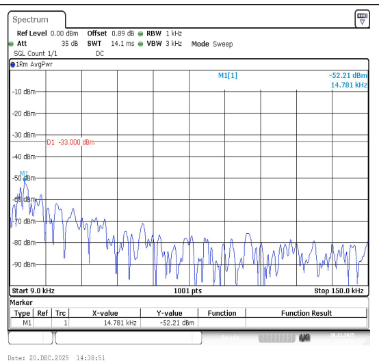
Band12-1.4MHz-16QAM-23095-1RB#0-0.009~0.1 5-PASS
