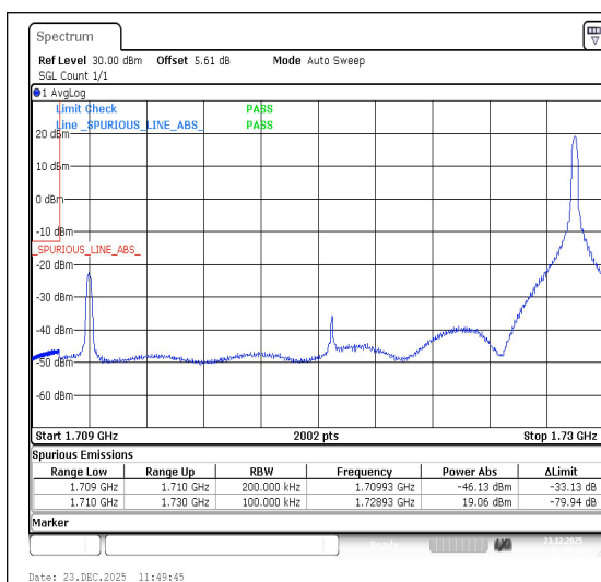
Band66-20MHz-16QAM-132072-1RB#99-PASS
