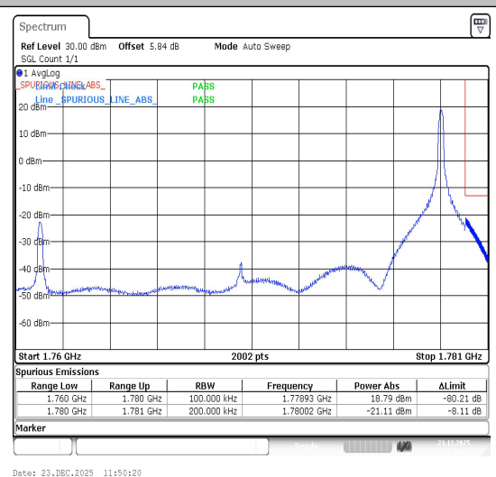
Band66-20MHz-16QAM-132572-1RB#99-PASS
