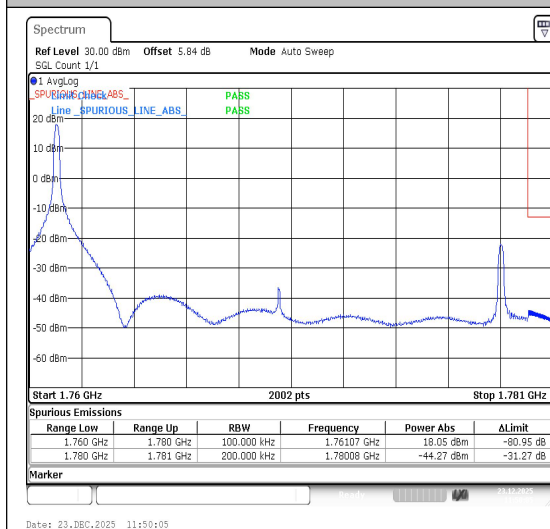
Band66-20MHz-16QAM-132572-1RB#0-PASS
