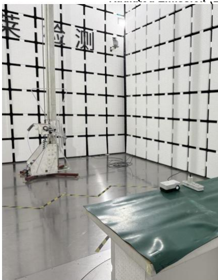
Radiated Emission (Below 1G)
