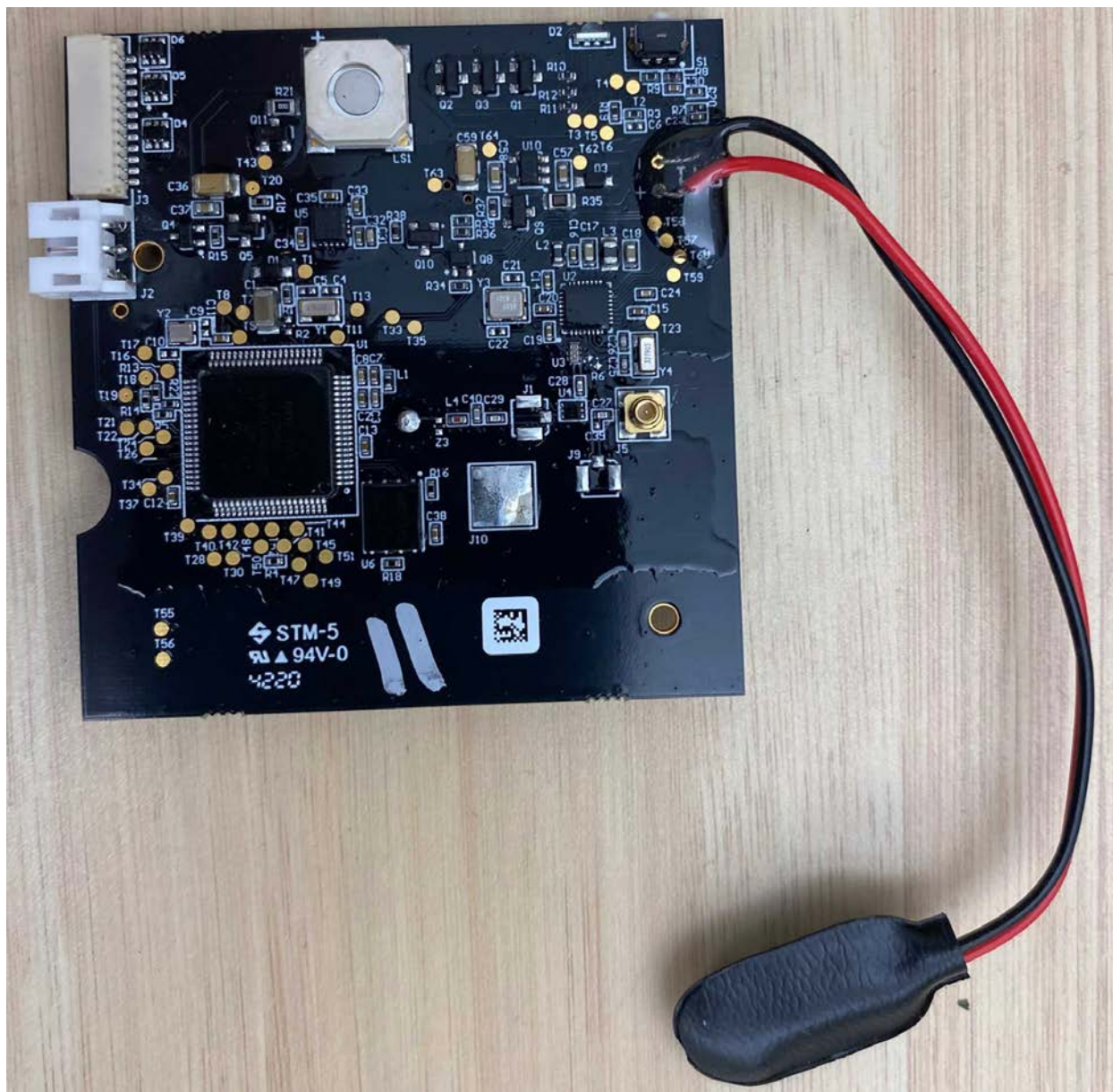
Figure 2: EMB Board - Back.
