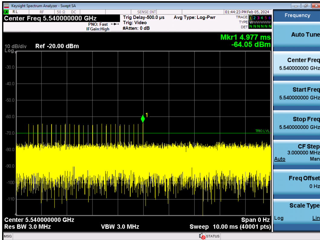
Radar Signal 3
