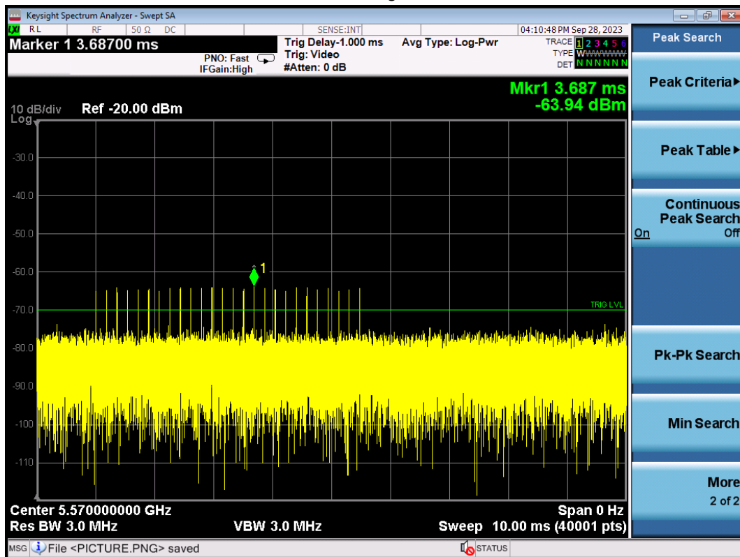
Radar Signal 3
