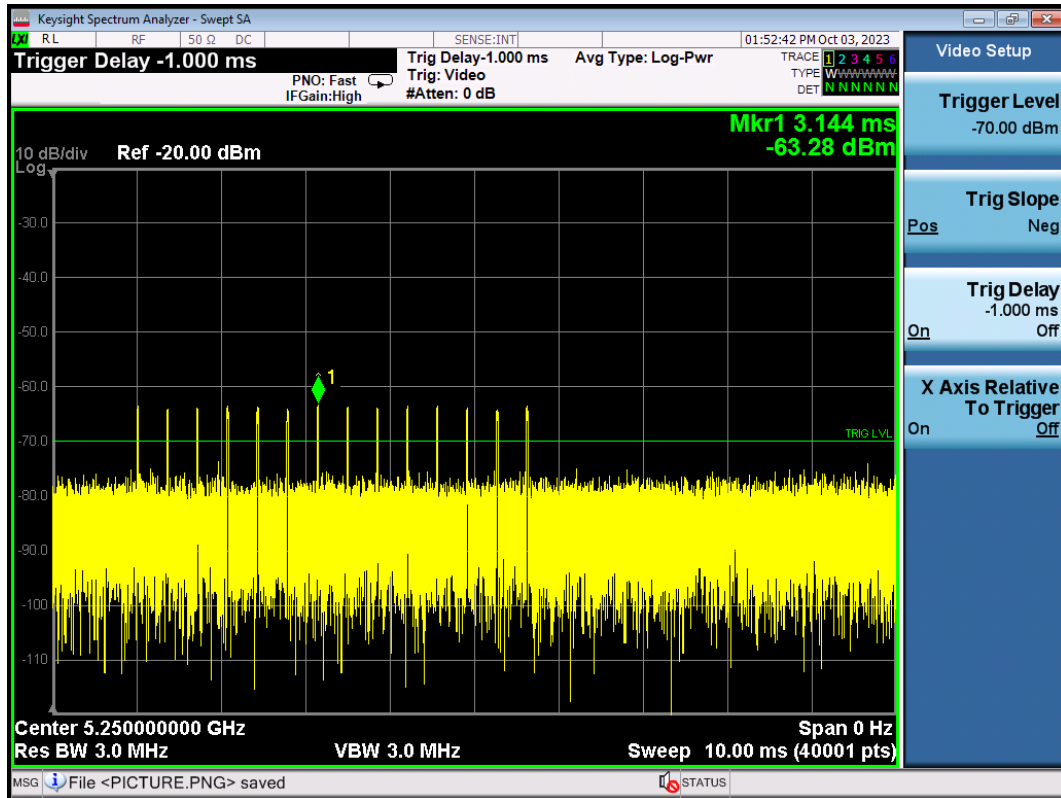
Radar Signal 5
