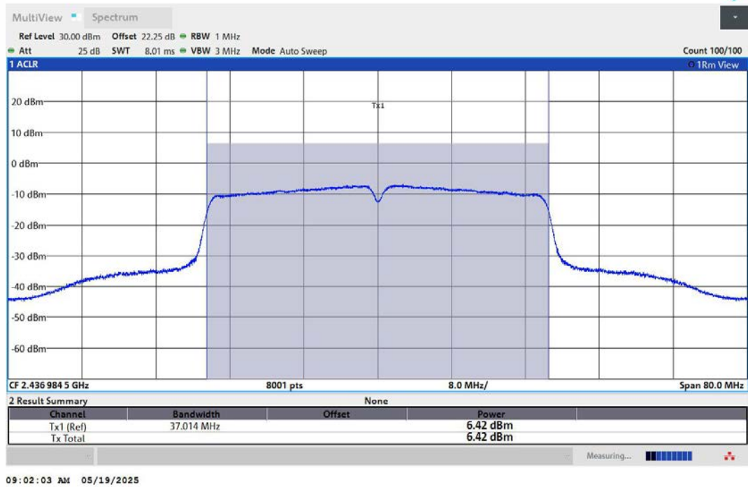
11N40MIMO-Ant1-2437-PASS
