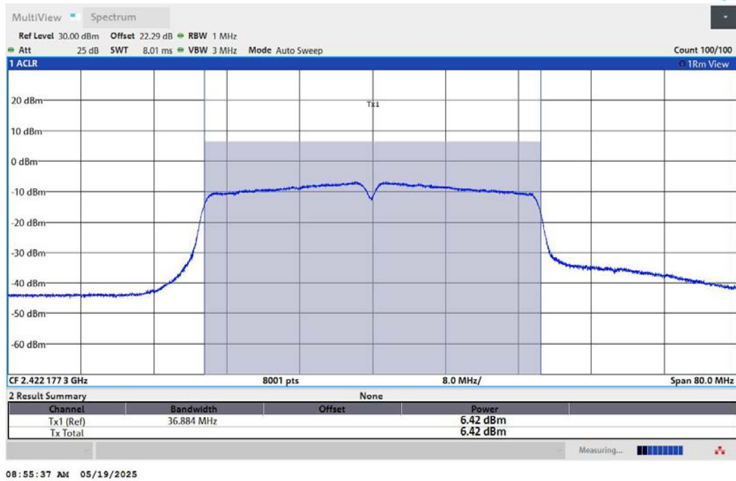
11N40MIMO-Ant1-2422-PASS
