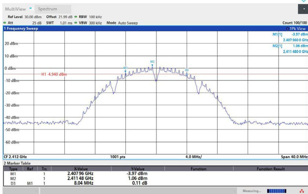
11B-Ant2-2412-PASS
