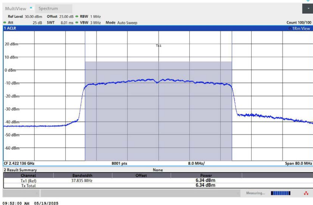
11AX40MIMO-Ant2-2422-PASS
