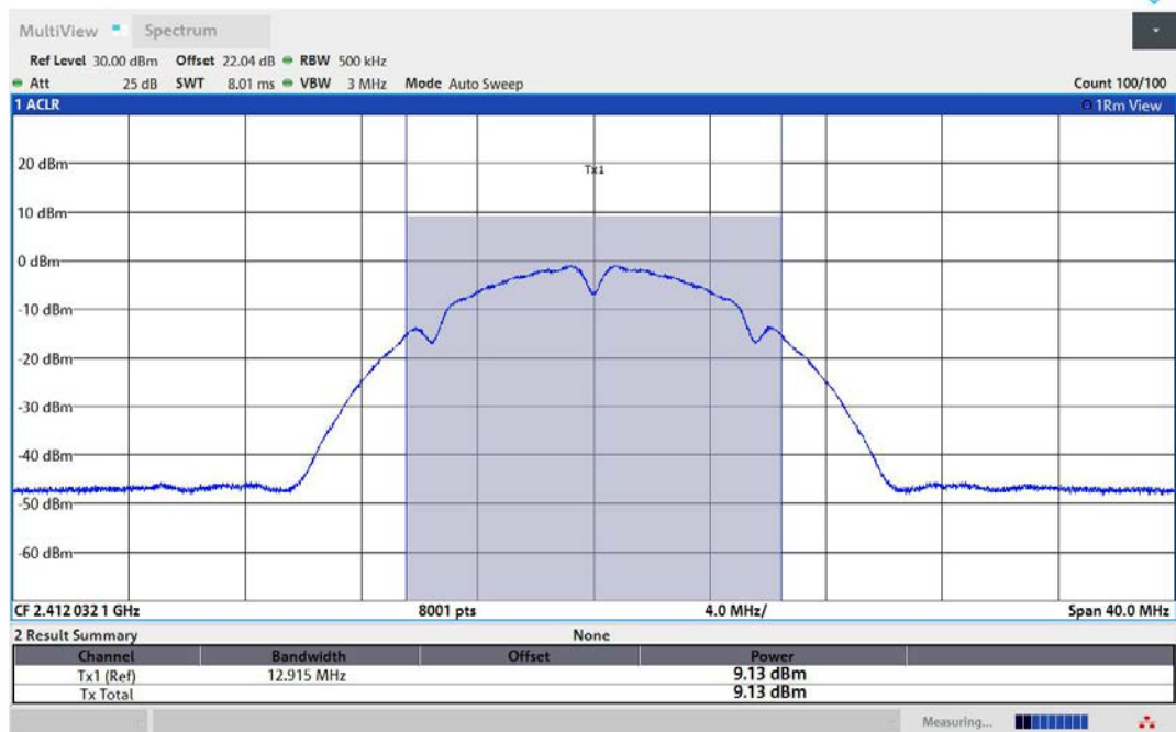
11B-Ant1-2412-PASS
