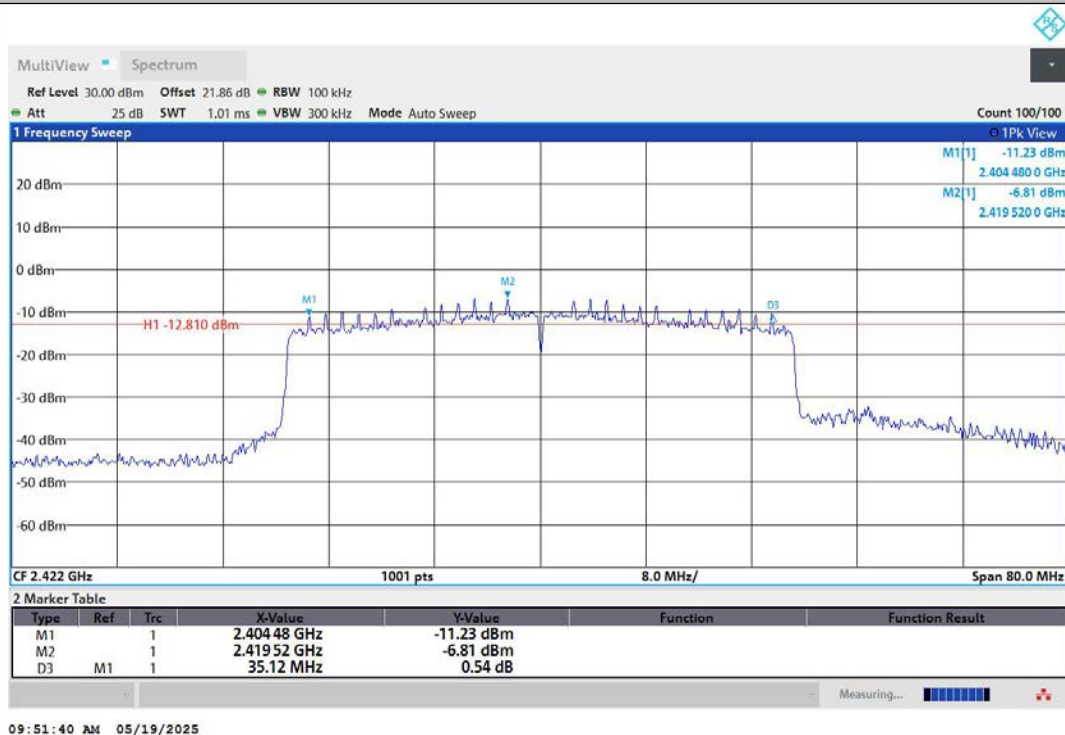
11AX40MIMO-Ant2-2422-PASS
