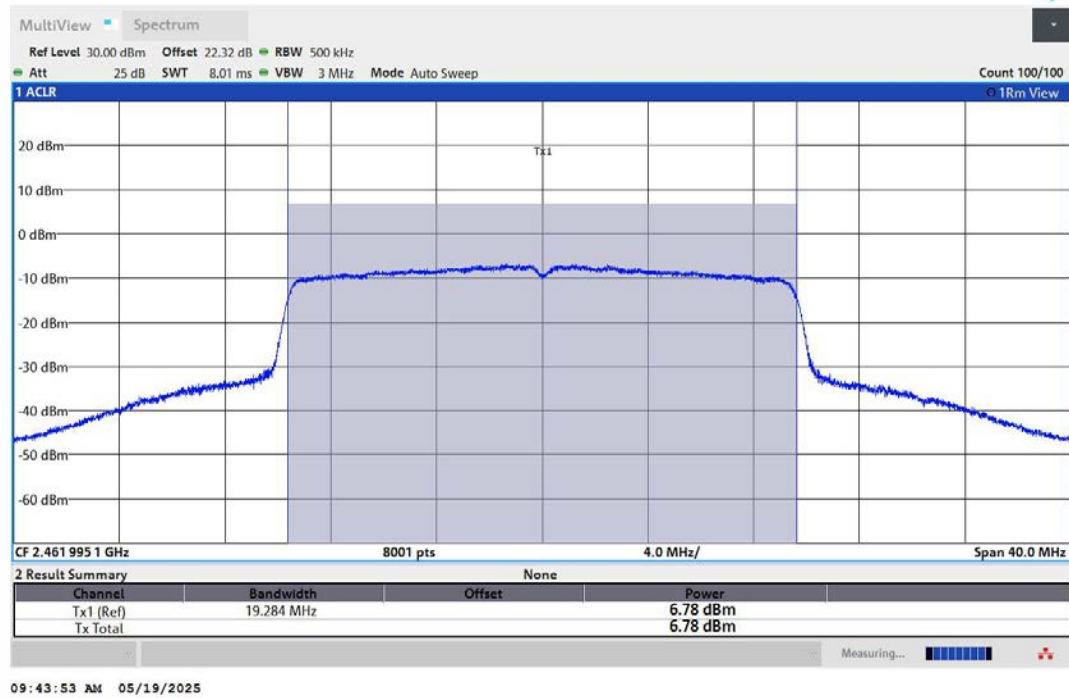
11AX20MIMO-Ant1-2462-PASS
