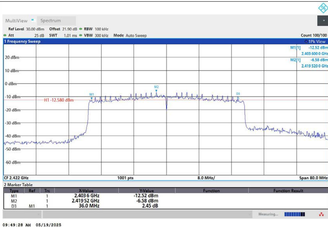
11AX40MIMO-Ant1-2422-PASS
