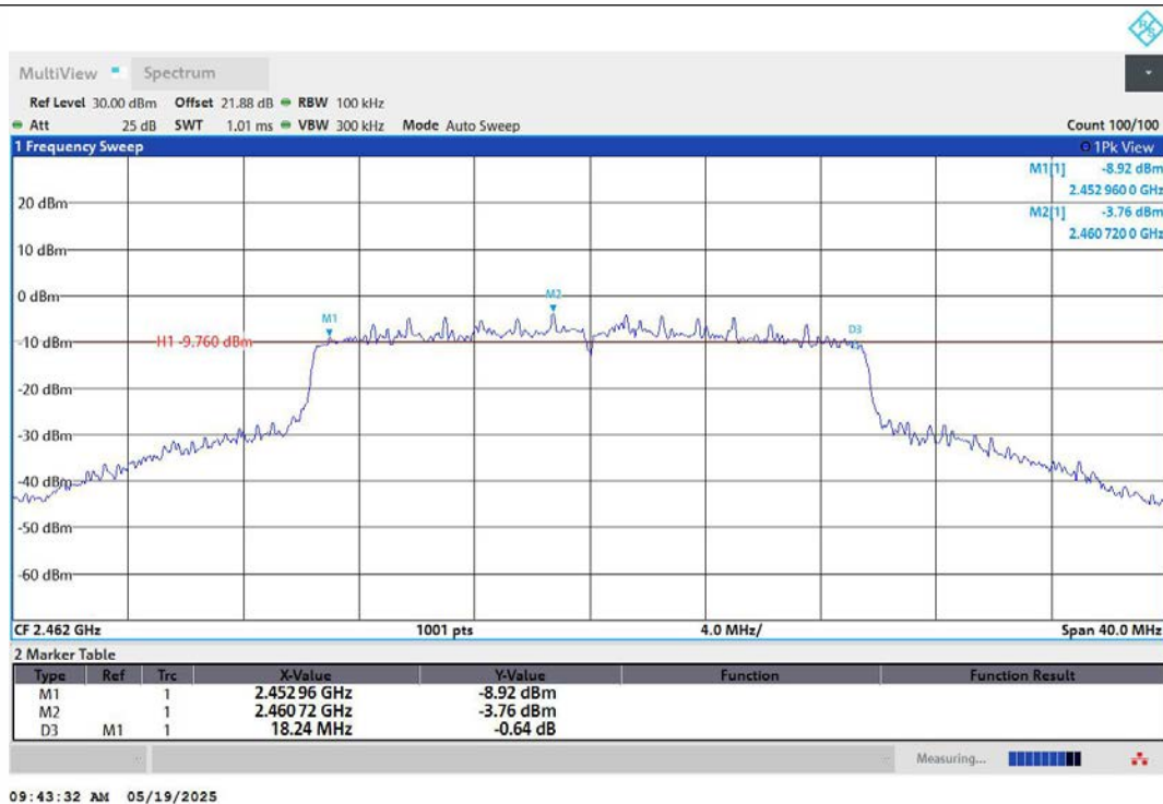
11AX20MIMO-Ant1-2462-PASS
