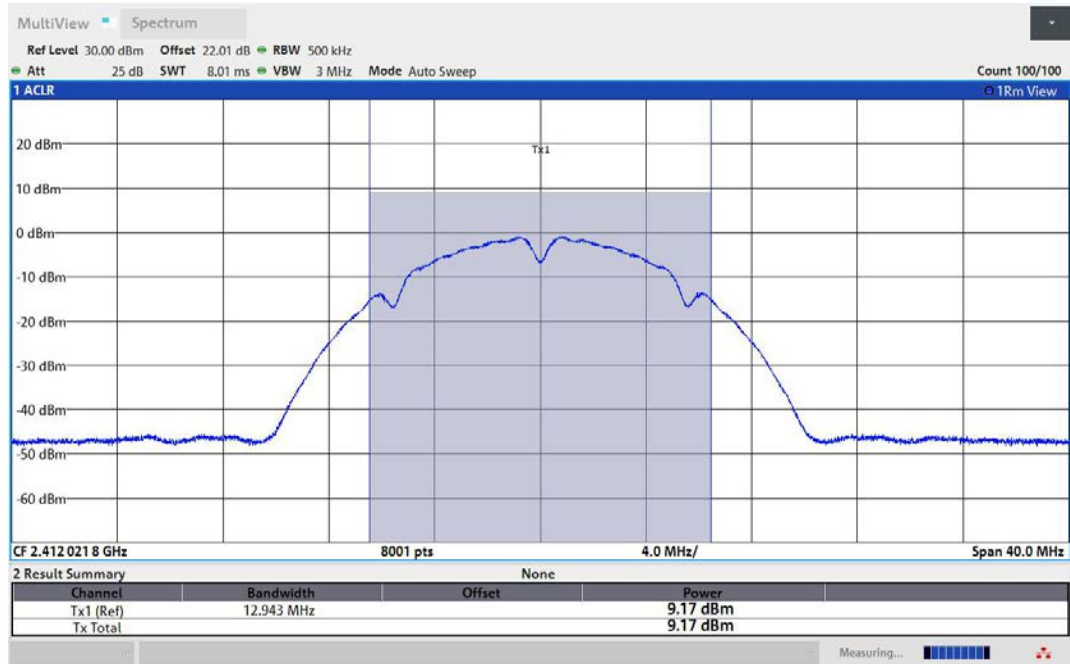
11B-Ant2-2412-PASS
