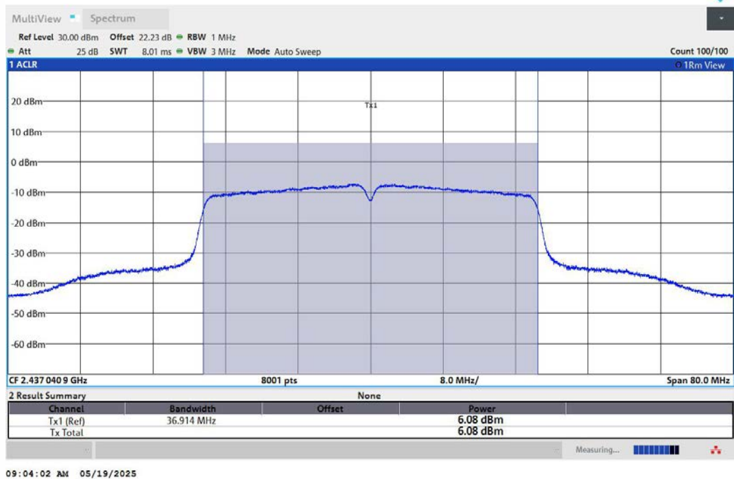
11N40MIMO-Ant2-2437-PASS
