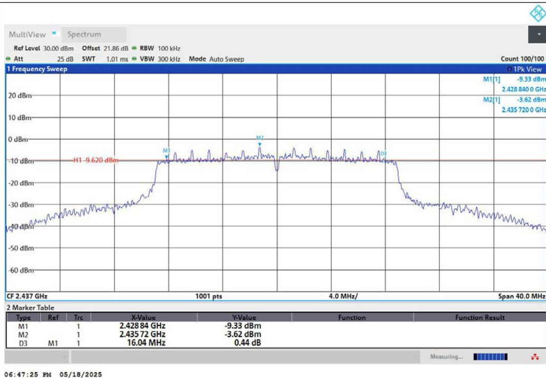
11N20MIMO-Ant1-2437-PASS
