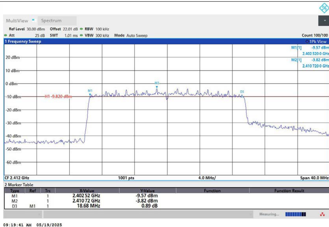
11AX20MIMO-Ant1-2412-PASS
