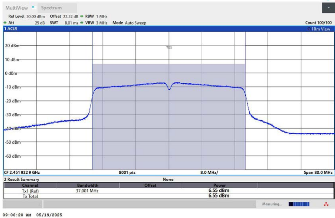
11N40MIMO-Ant1-2452-PASS
