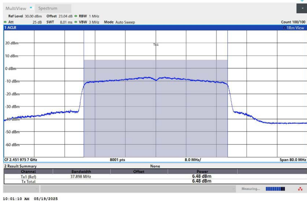
11AX40MIMO-Ant2-2452-PASS
