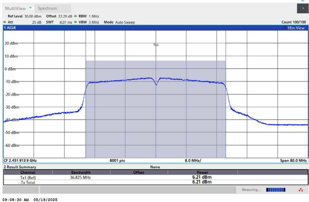
11N40MIMO-Ant2-2452-PASS
