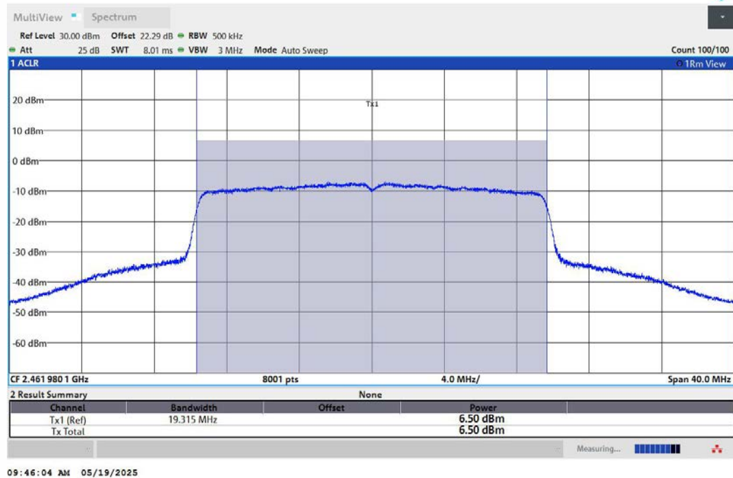
11AX20MIMO-Ant2-2462-PASS
