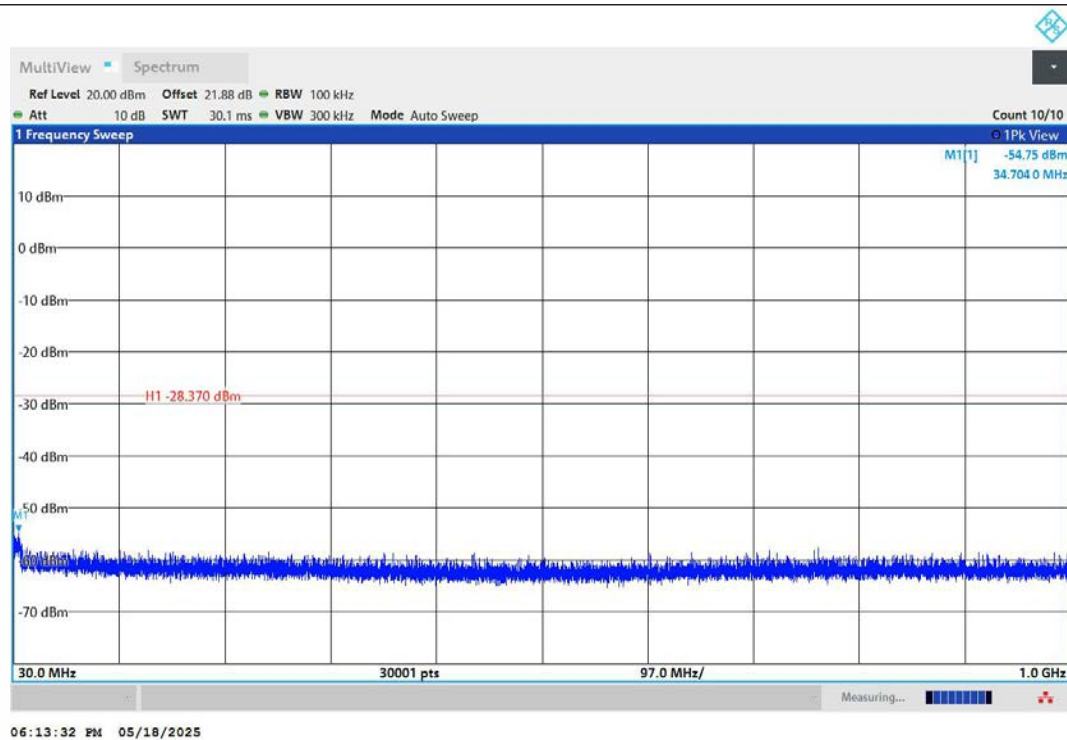
11B-Ant1-2462-30~1000-PASS
