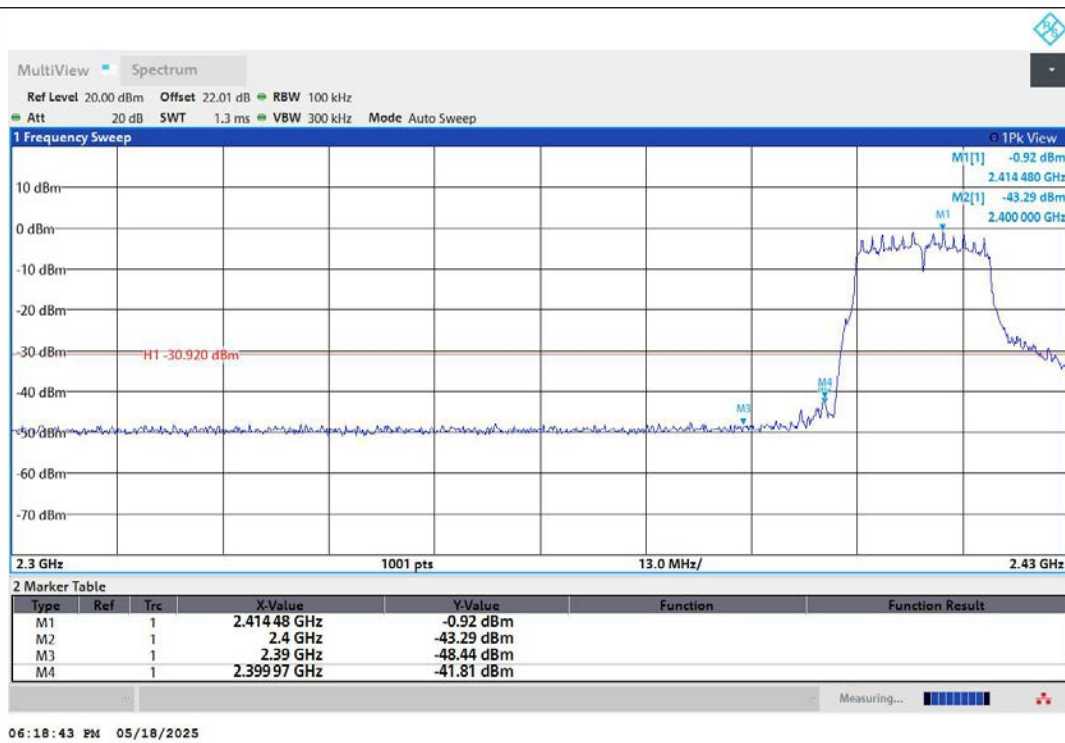
11G-Ant1-2412-PASS
