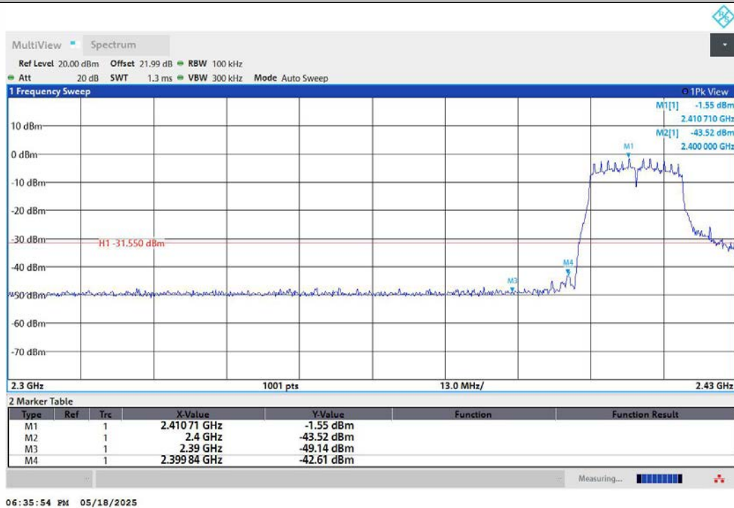
11G-Ant2-2412-PASS
