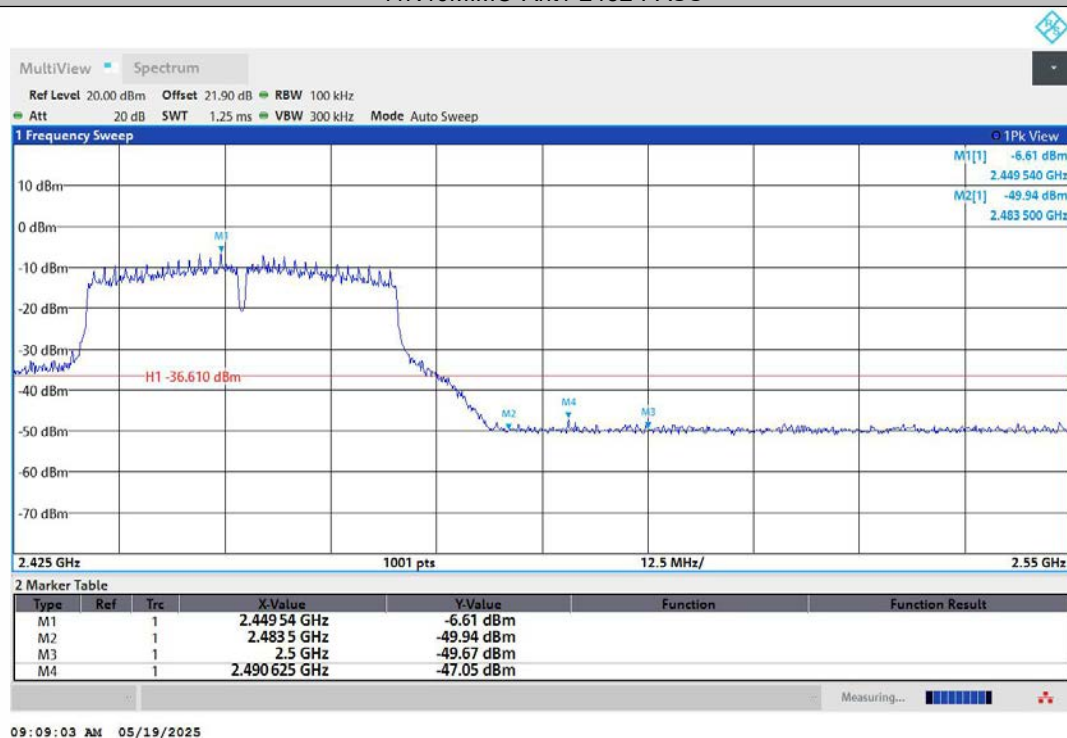
11N40MIMO-Ant2-2452-PASS
