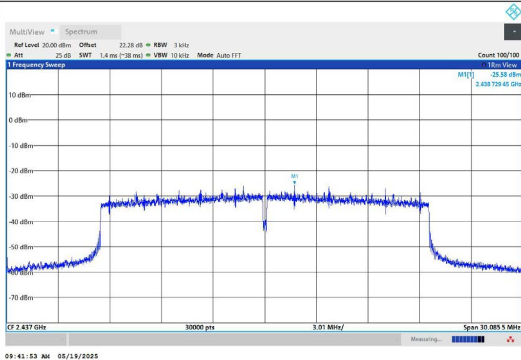
11AX20MIMO-Ant2-2437-PASS
