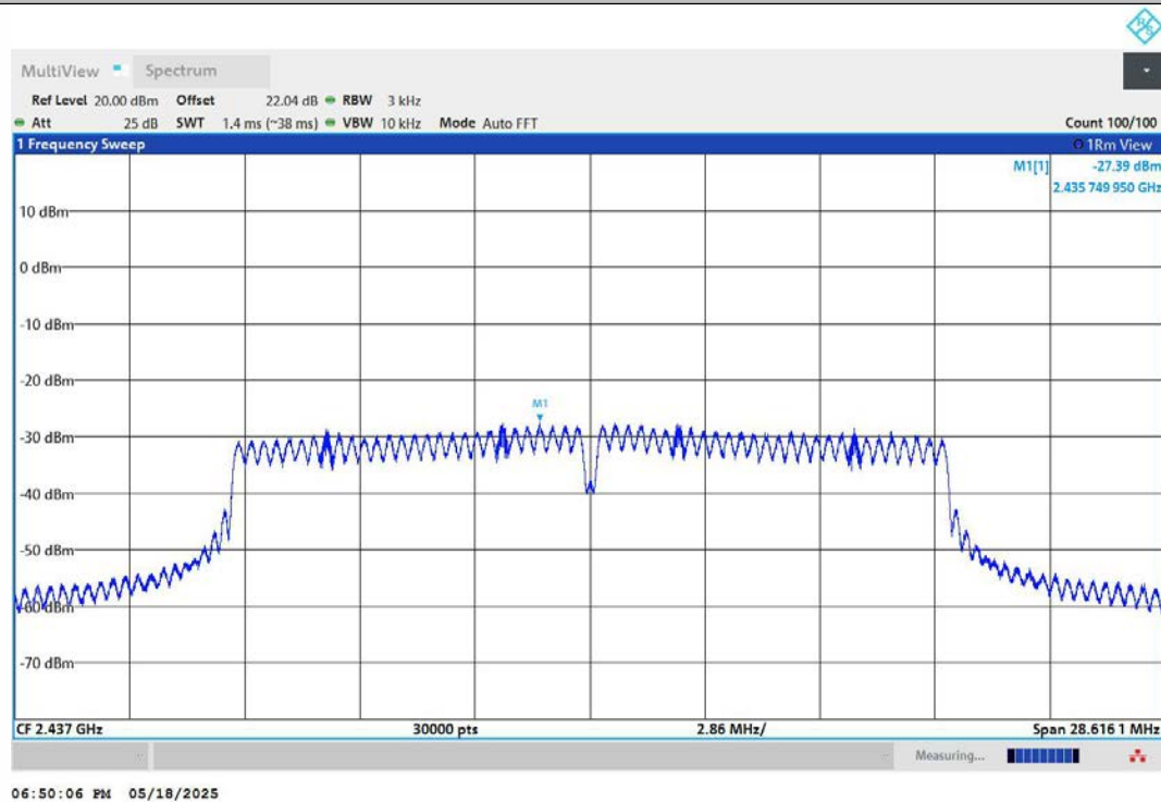
11N20MIMO-Ant2-2437-PASS
