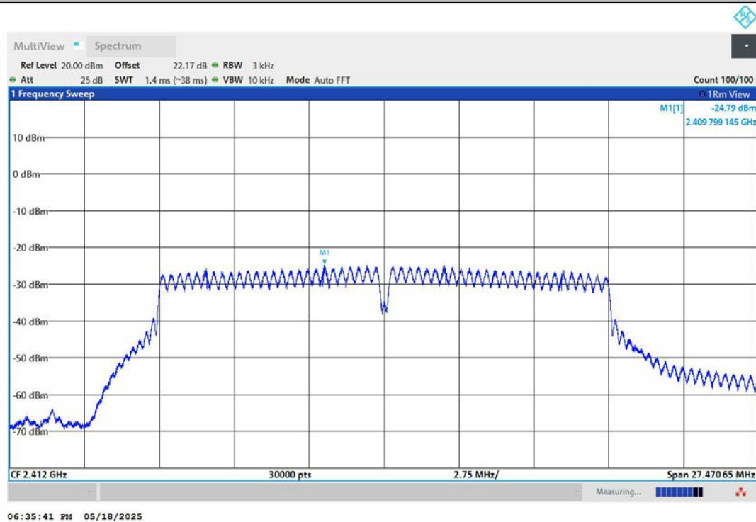
11G-Ant2-2412-PASS
