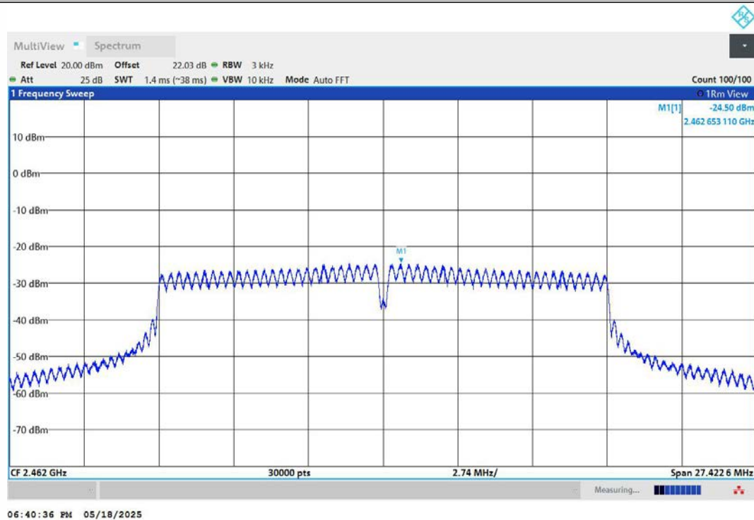
11G-Ant2-2462-PASS
