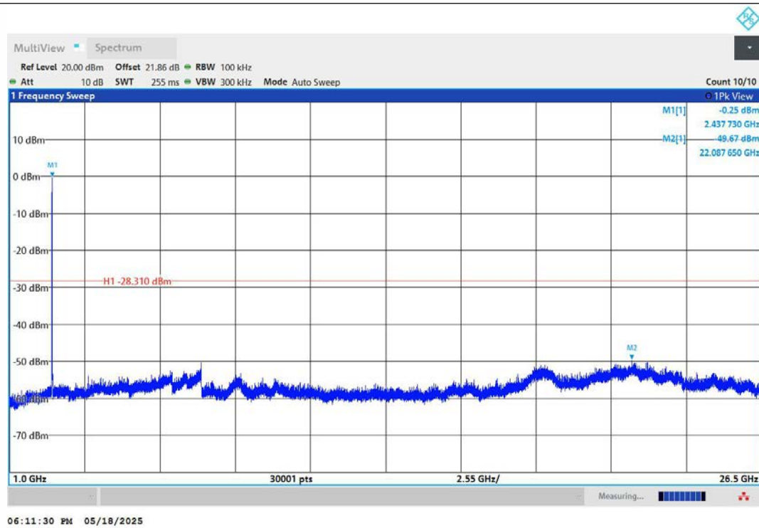
11B-Ant1-2437-1000~26500-PASS
