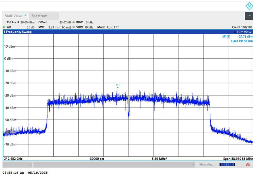
11AX40MIMO-Ant1-2452-PASS
