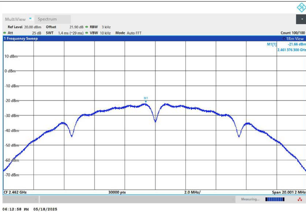
11B-Ant1-2462-PASS
