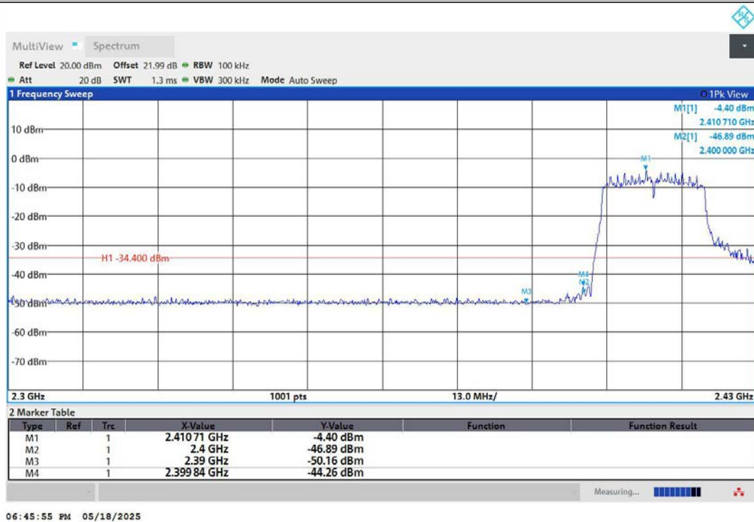
11N20MIMO-Ant2-2412-PASS
