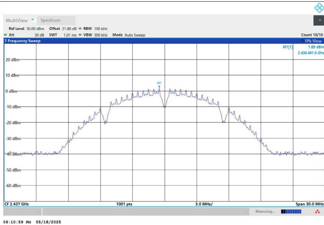
11B-Ant1-2437-0~Reference-PASS
