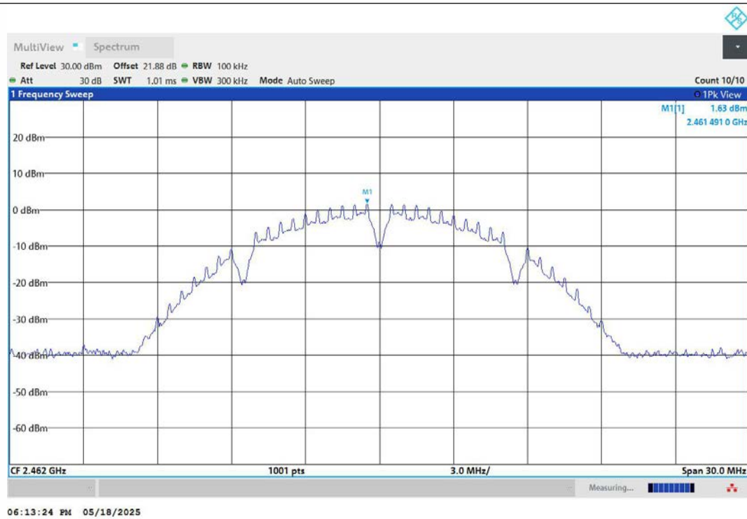
11B-Ant1-2462-0~Reference-PASS
