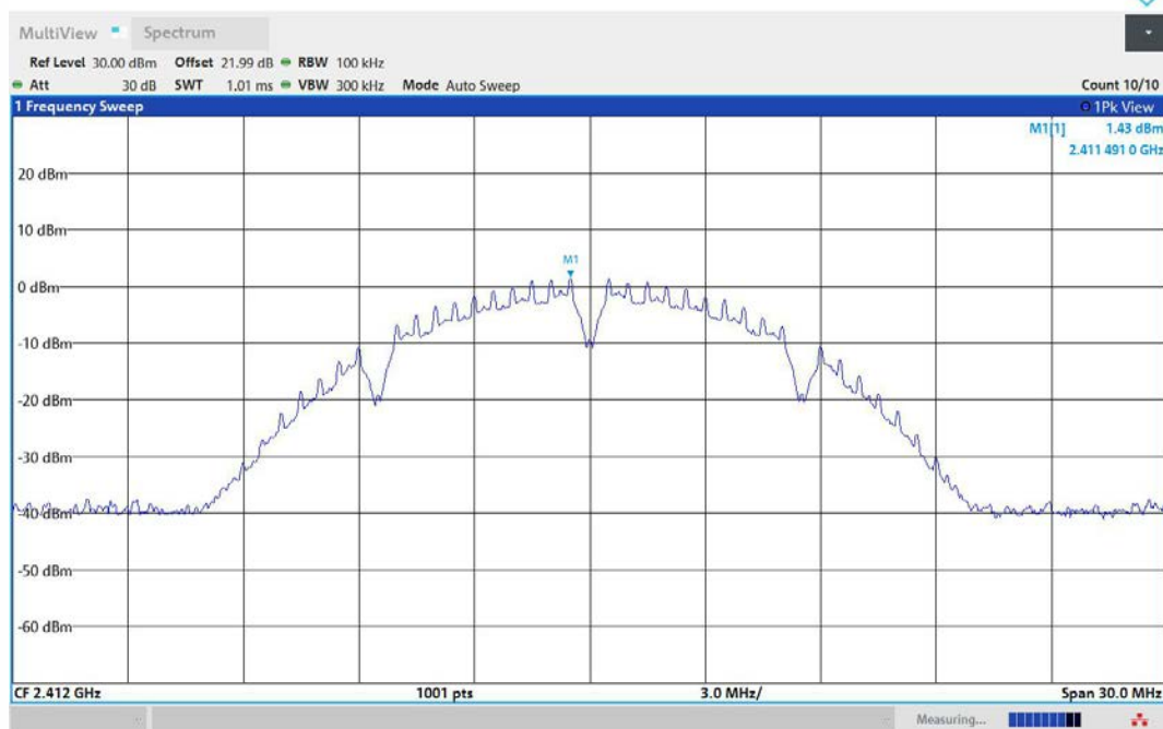
11B-Ant2-2412-0~Reference-PASS
