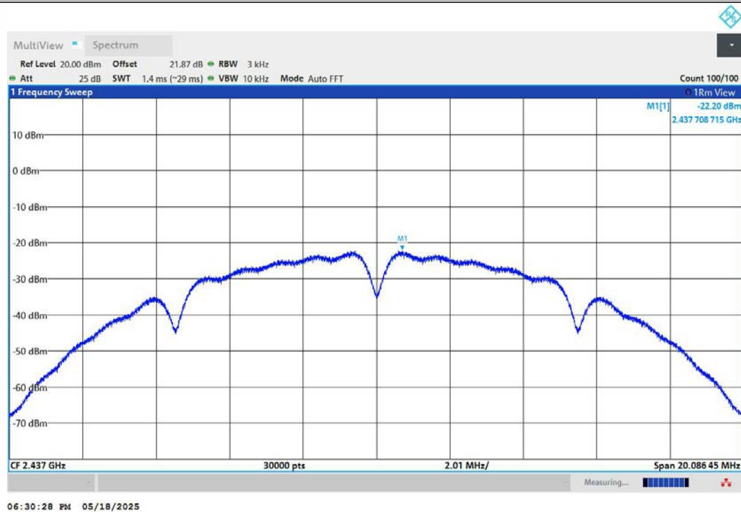
11B-Ant2-2437-PASS
