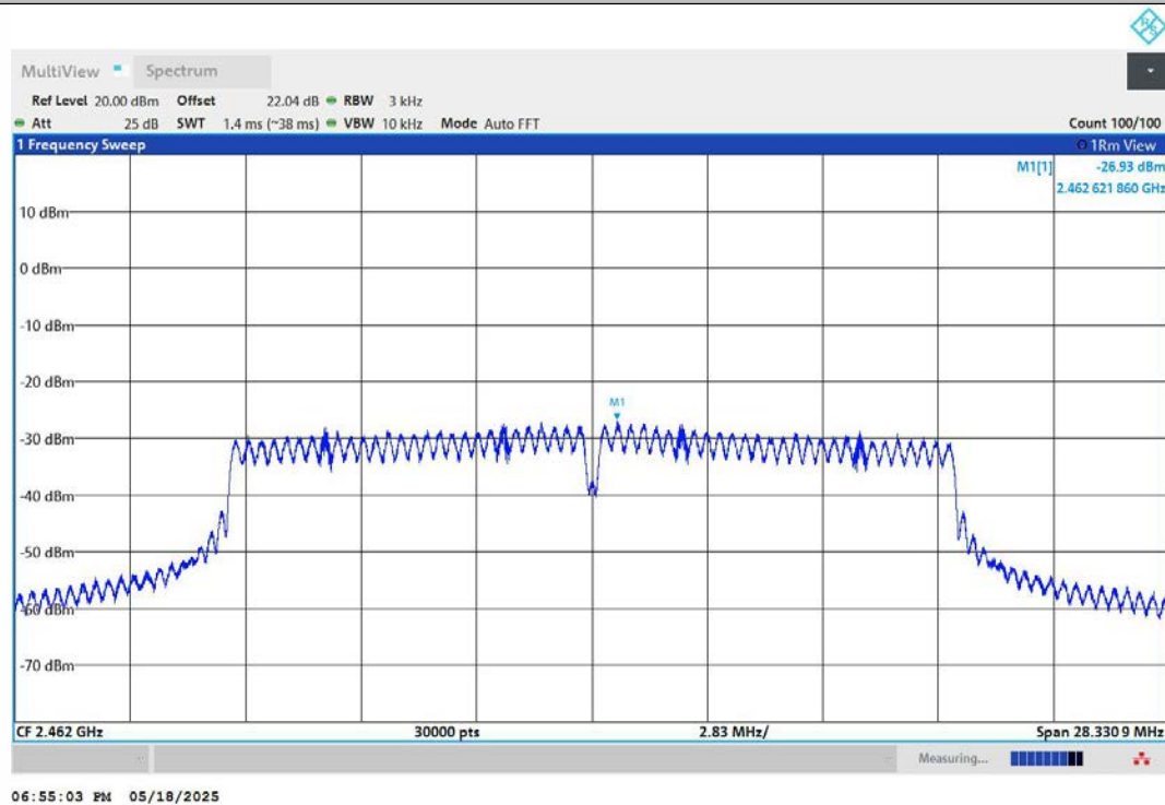
11N20MIMO-Ant2-2462-PASS
