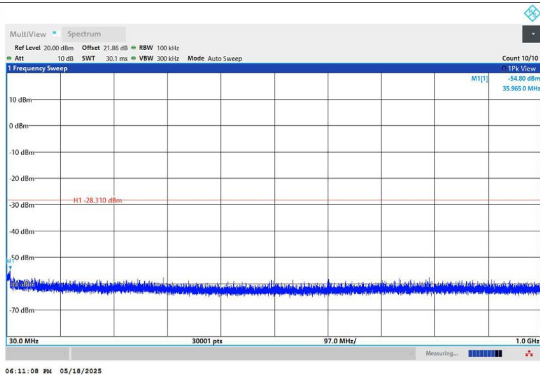
11B-Ant1-2437-30~1000-PASS
