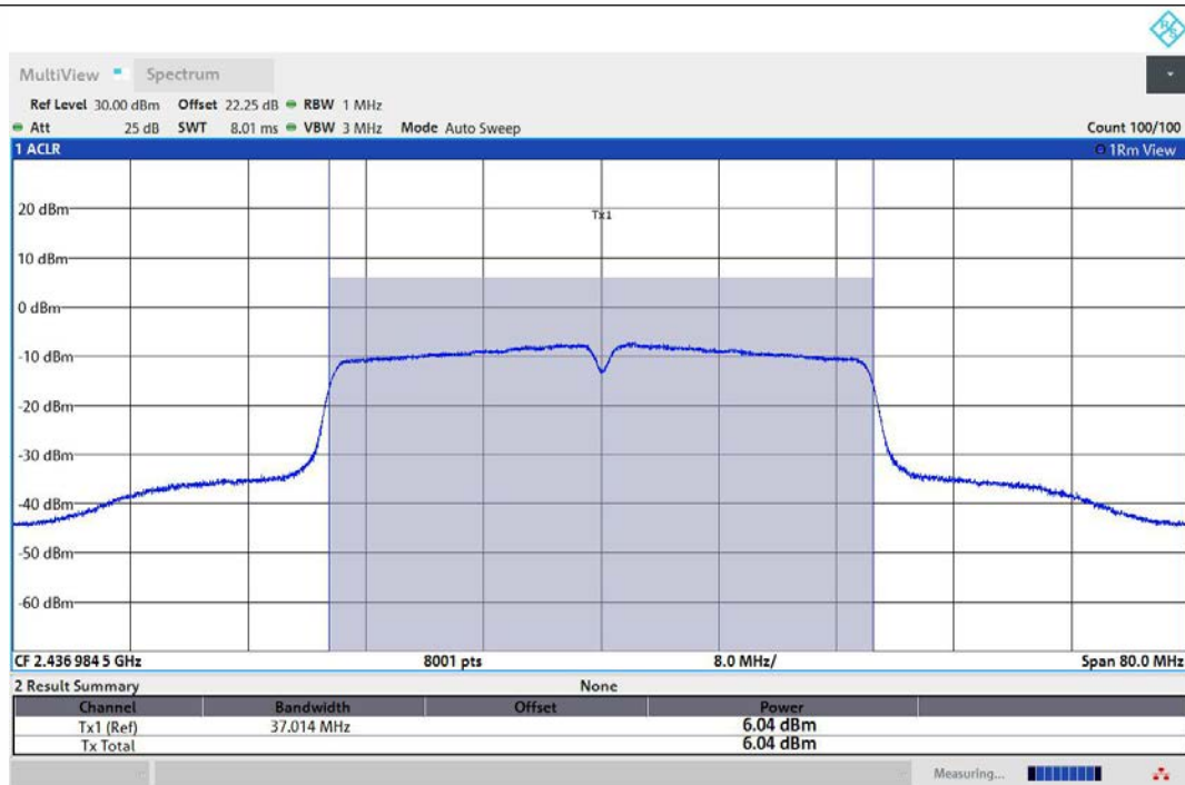
11N40MIMO-Ant1-2437-PASS
