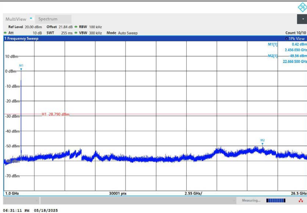
11B-Ant2-2437-1000~26500-PASS
