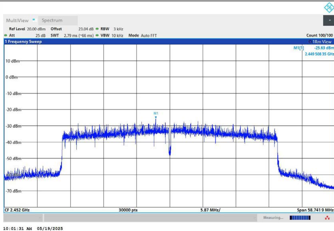
11AX40MIMO-Ant2-2452-PASS
