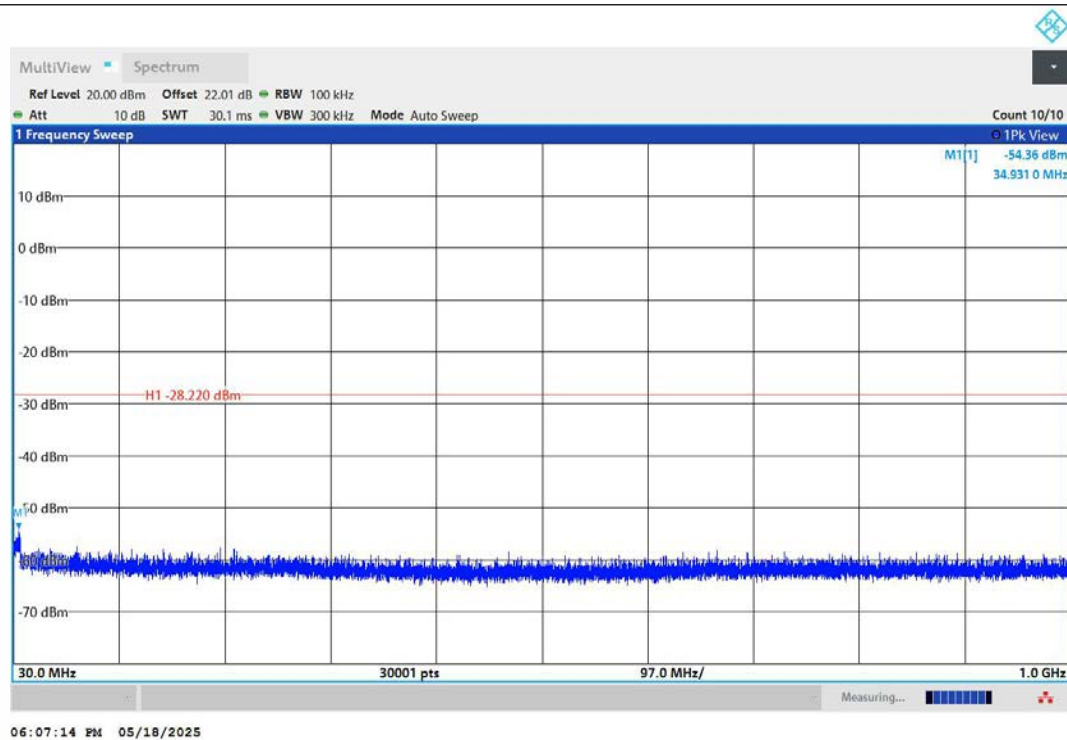
11B-Ant1-2412-30~1000-PASS
