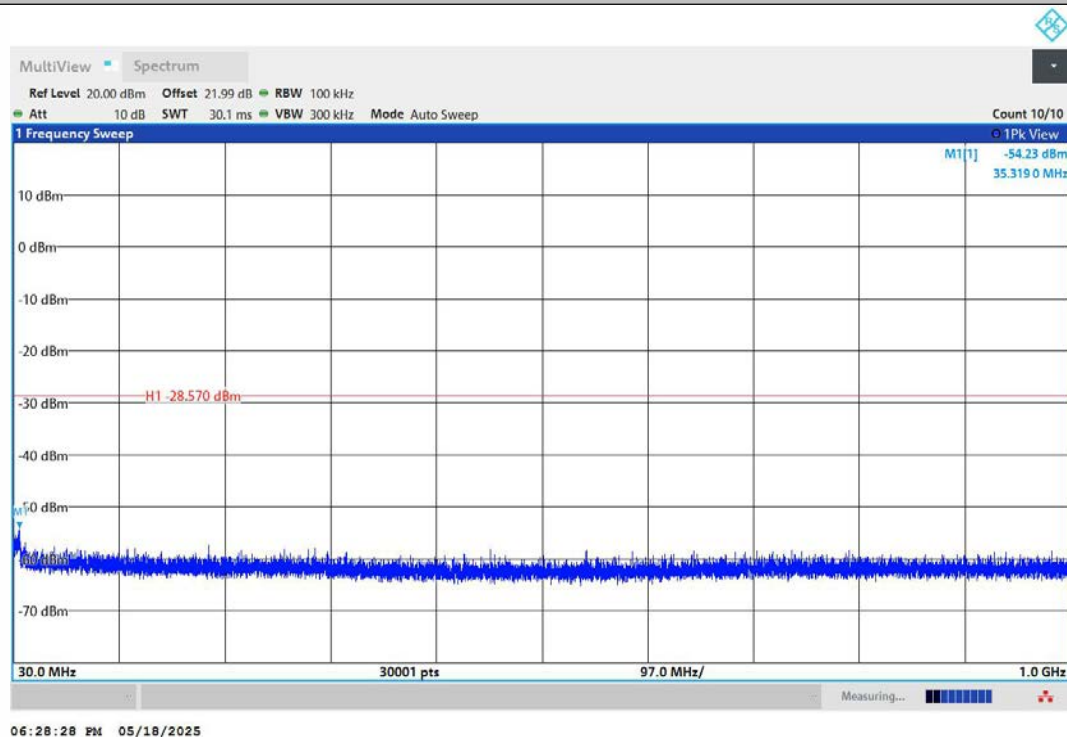
11B-Ant2-2412-30~1000-PASS
