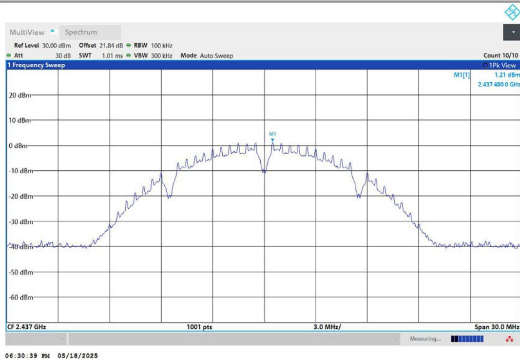
11B-Ant2-2437-0~Reference-PASS
