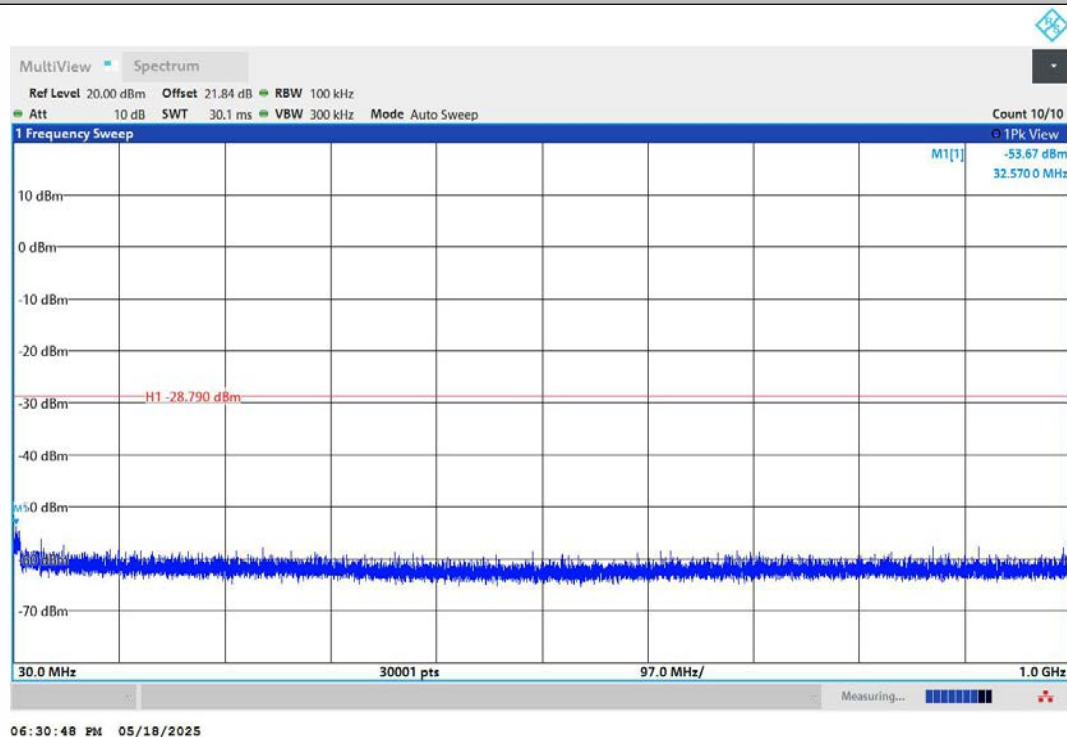
11B-Ant2-2437-30~1000-PASS
