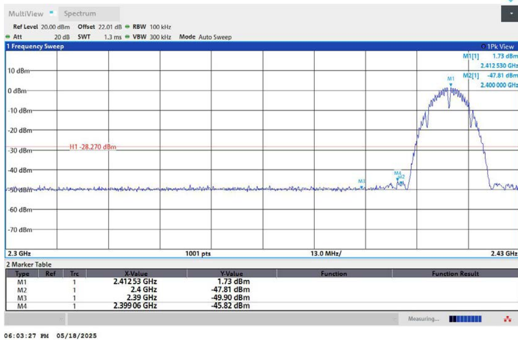
11B-Ant1-2412-PASS
