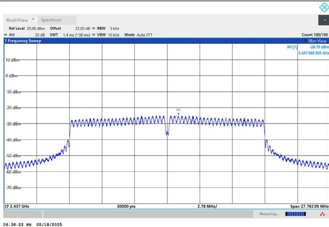
11G-Ant2-2437-PASS
