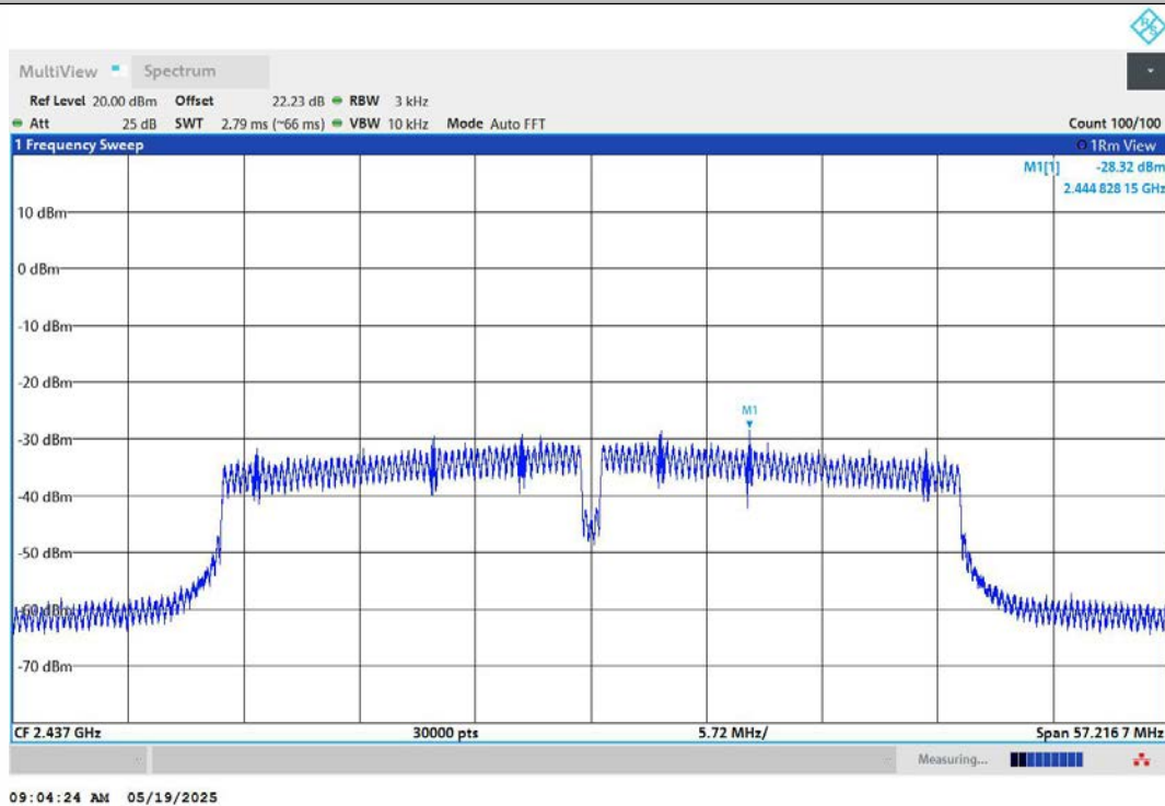
11N40MIMO-Ant2-2437-PASS
