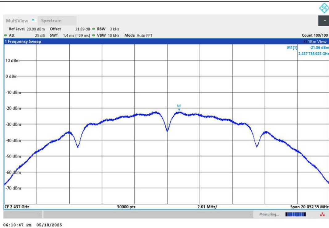
11B-Ant1-2437-PASS
