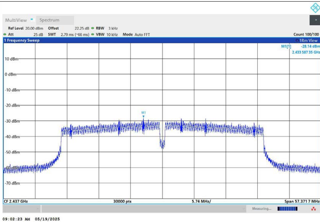
11N40MIMO-Ant1-2437-PASS
