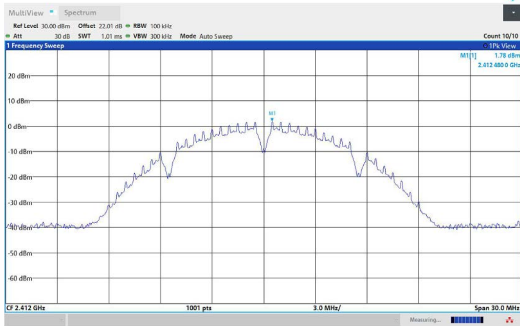
11B-Ant1-2412-0~Reference-PASS
