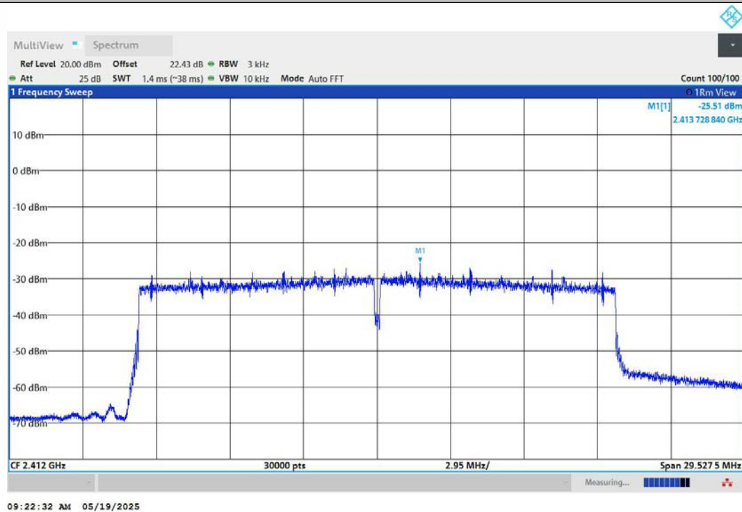
11AX20MIMO-Ant2-2412-PASS
