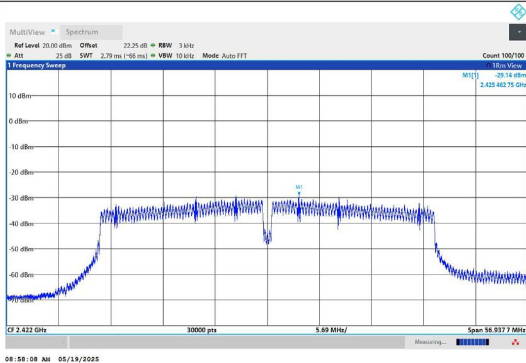
11N40MIMO-Ant2-2422-PASS
