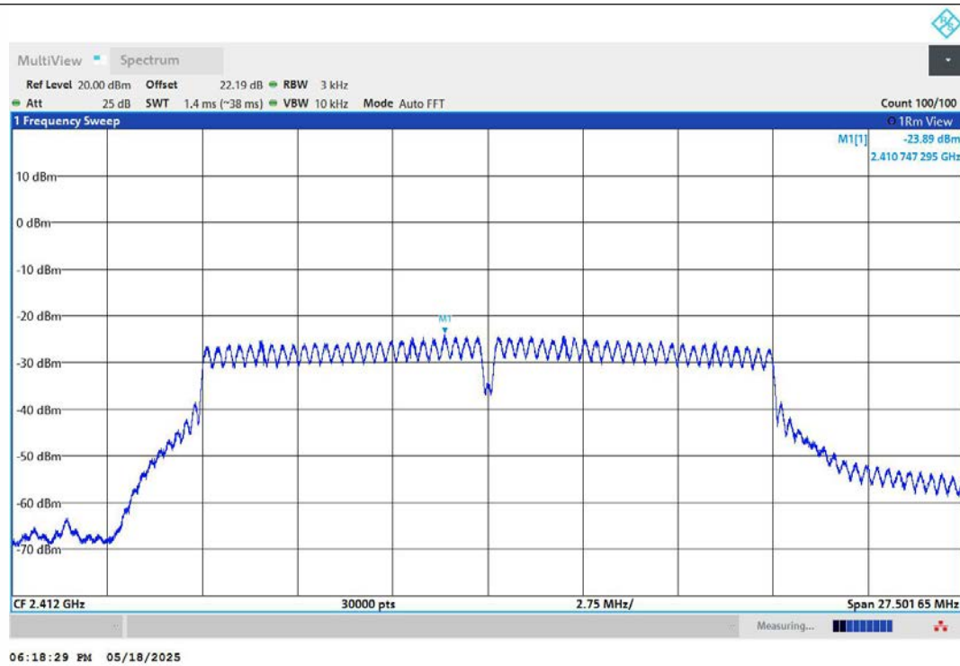
11G-Ant1-2412-PASS
