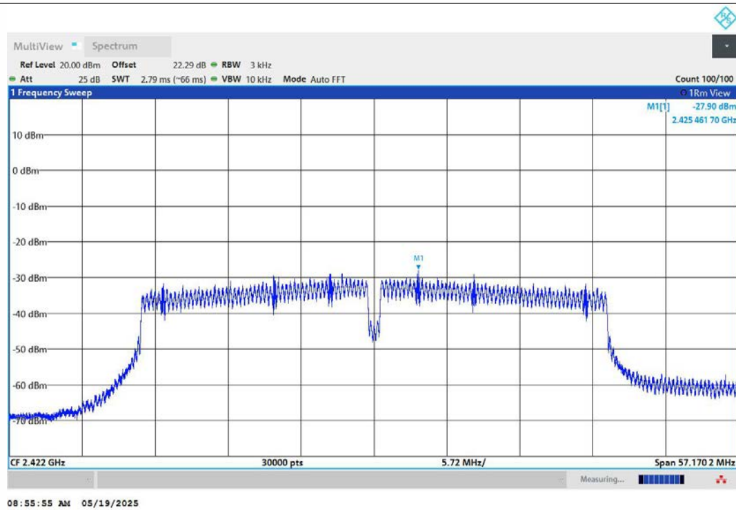
11N40MIMO-Ant1-2422-PASS
