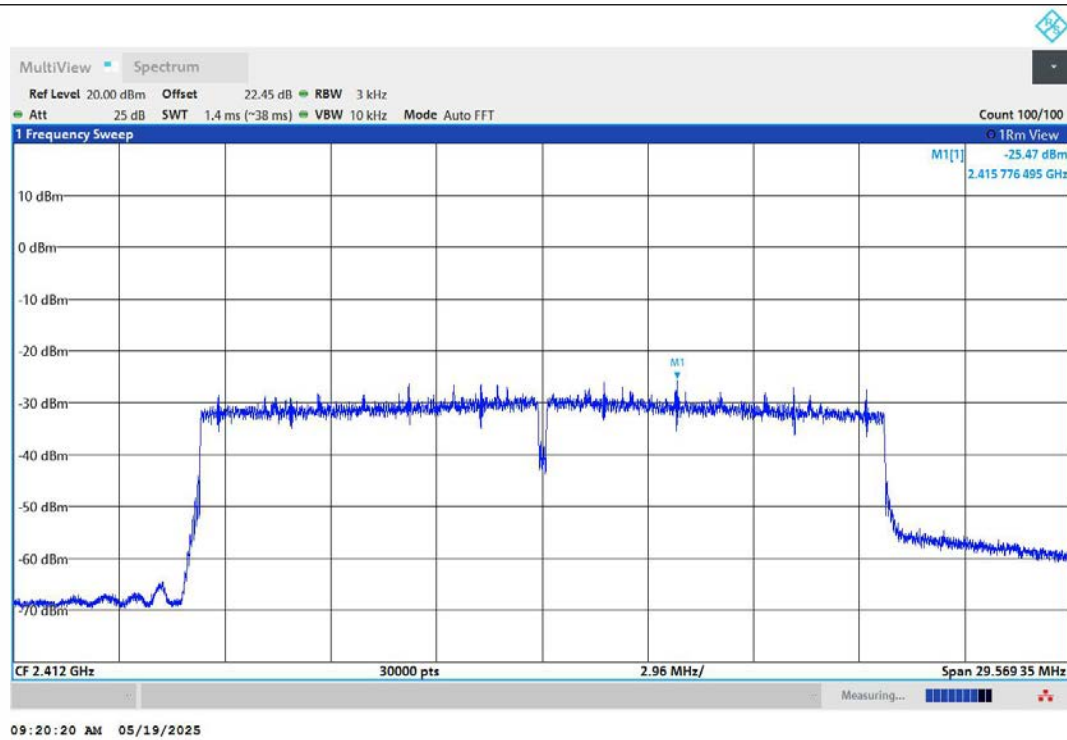
11AX20MIMO-Ant1-2412-PASS
