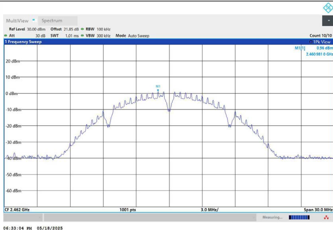
11B-Ant2-2462-0~Reference-PASS
