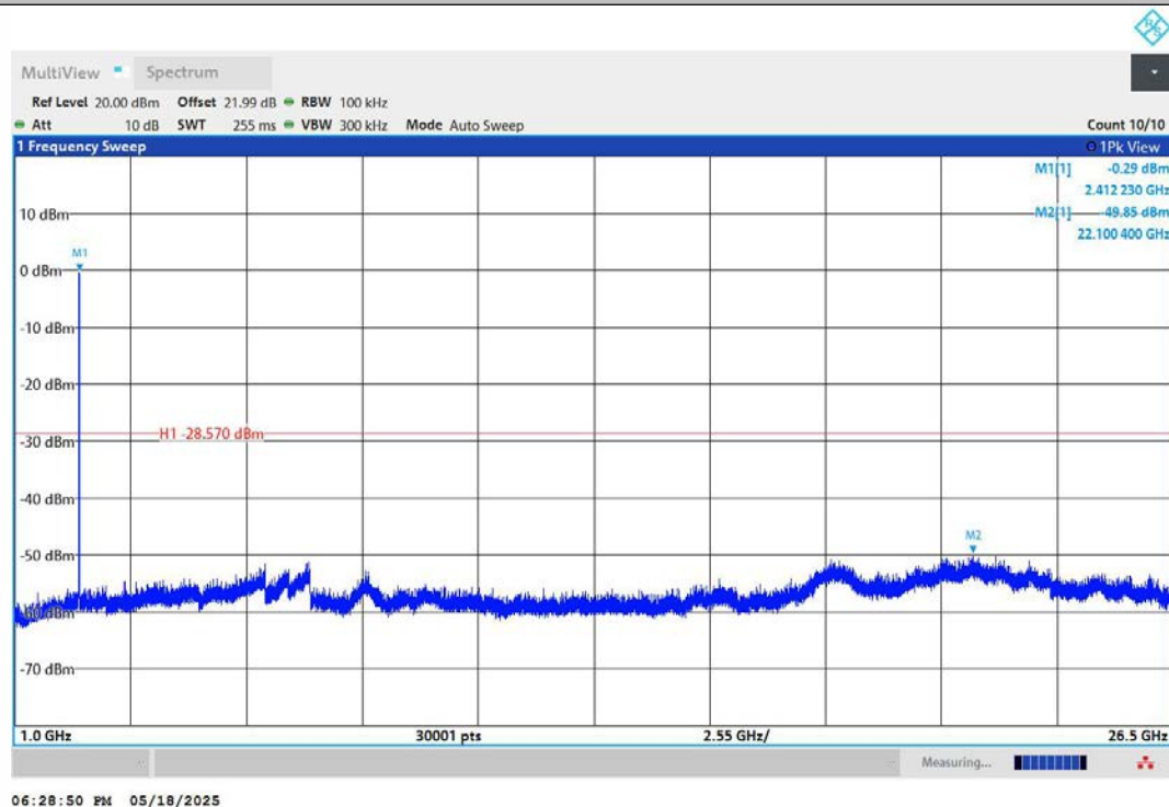
11B-Ant2-2412-1000~26500-PASS
