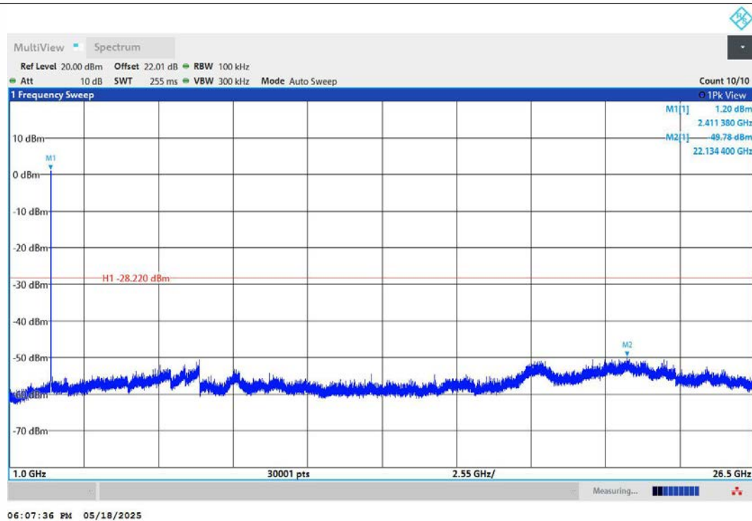
11B-Ant1-2412-1000~26500-PASS
