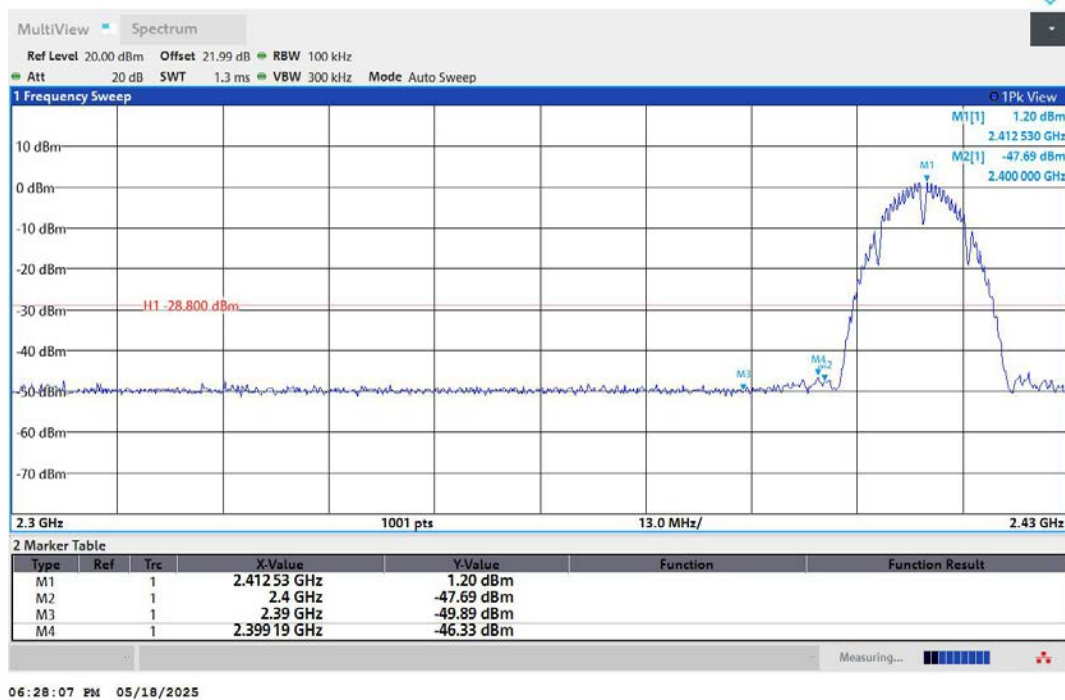
11B-Ant2-2412-PASS
