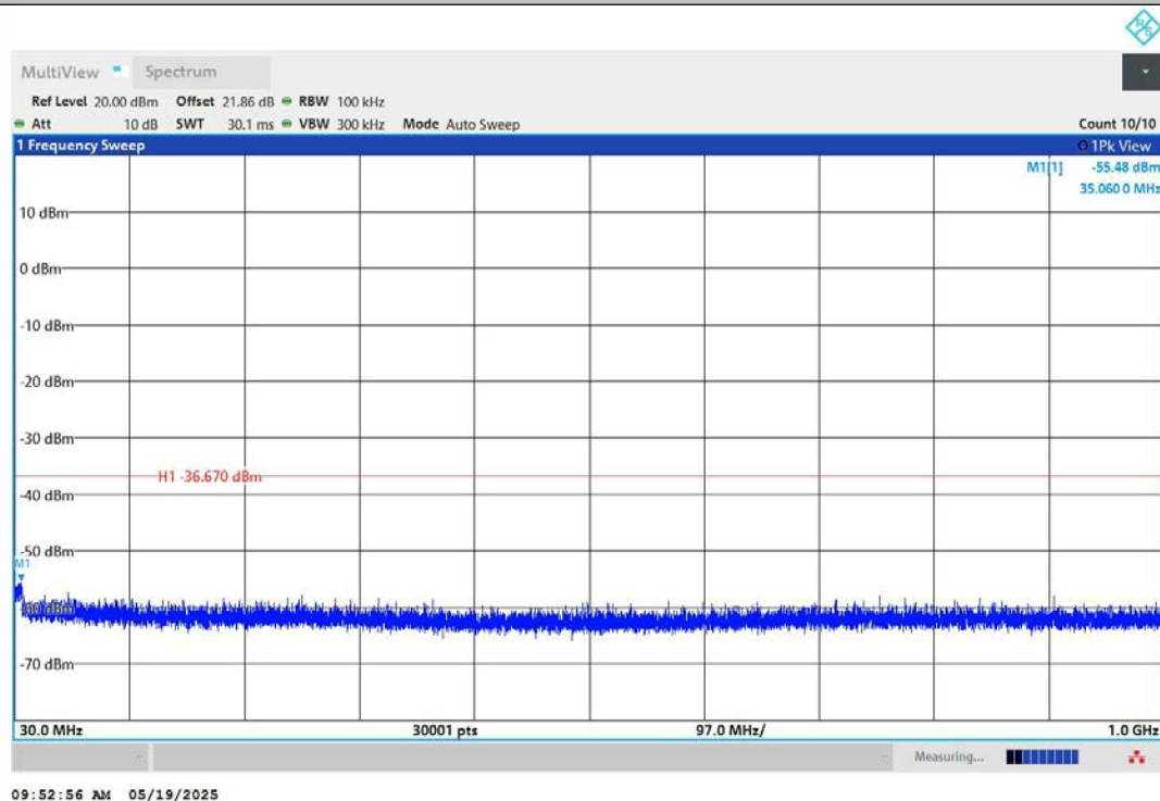
11AX40MIMO-Ant2-2422-30~1000-PASS
