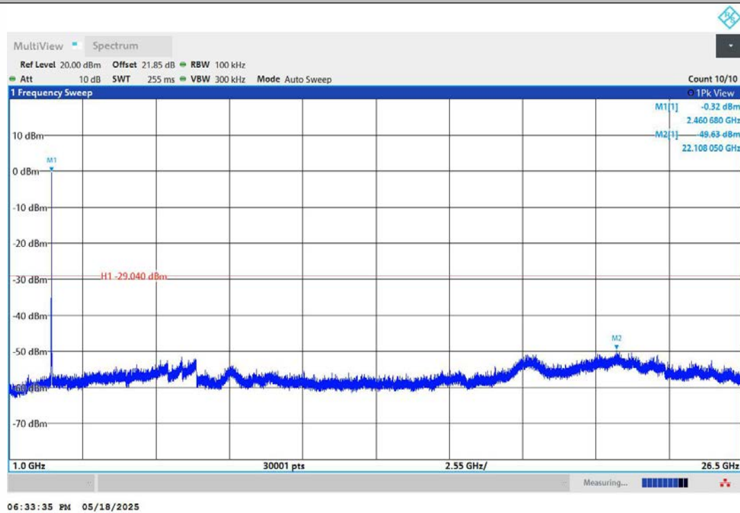
11B-Ant2-2462-1000~26500-PASS
