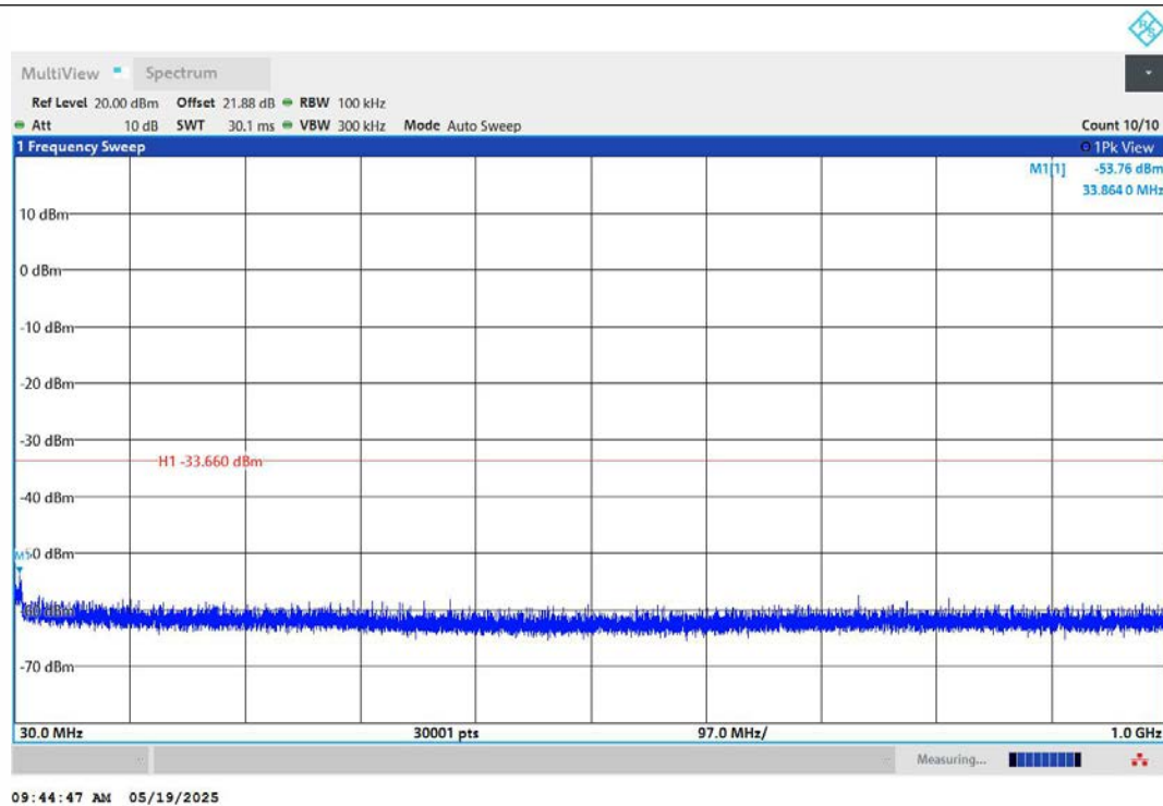
11AX20MIMO-Ant1-2462-30~1000-PASS
