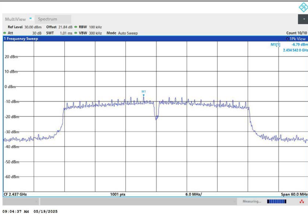
11N40MIMO-Ant2-2437-0~Reference-PASS
