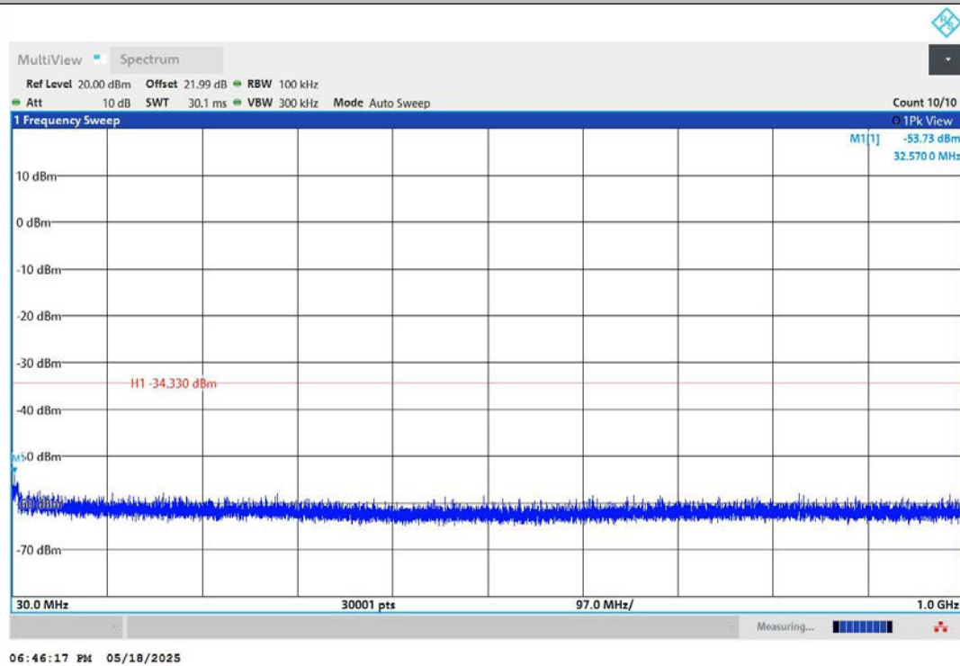
11N20MIMO-Ant2-2412-30~1000-PASS
