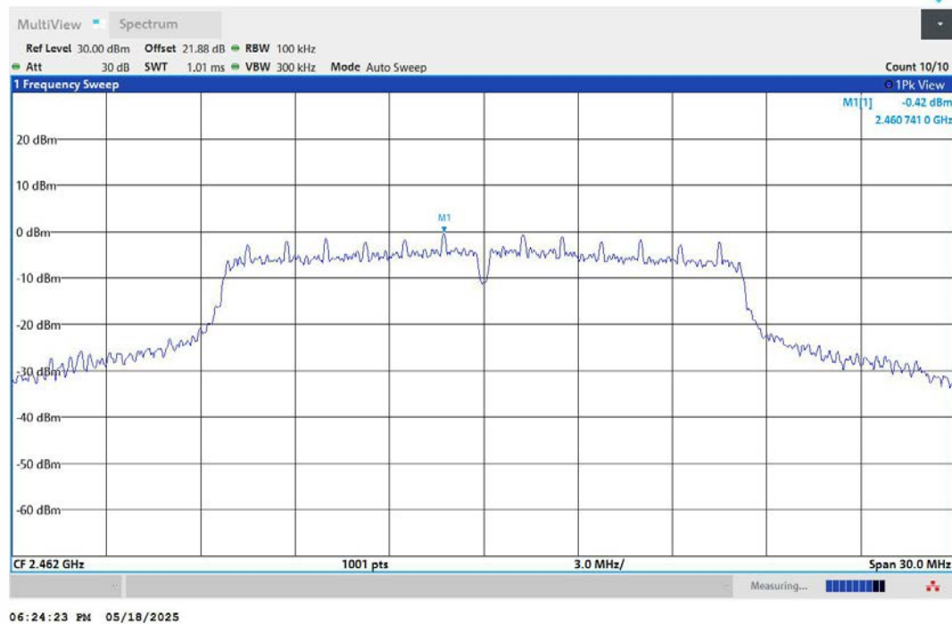
11G-Ant1-2462-0~Reference-PASS
