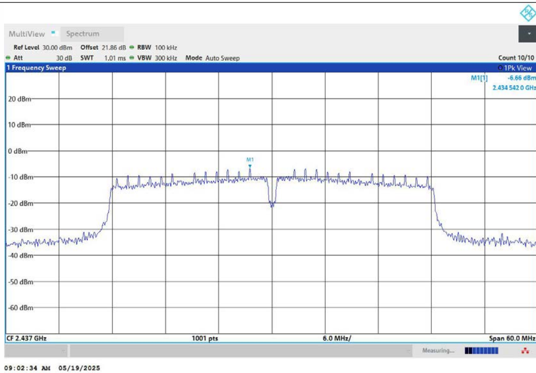
11N40MIMO-Ant1-2437-0~Reference-PASS
