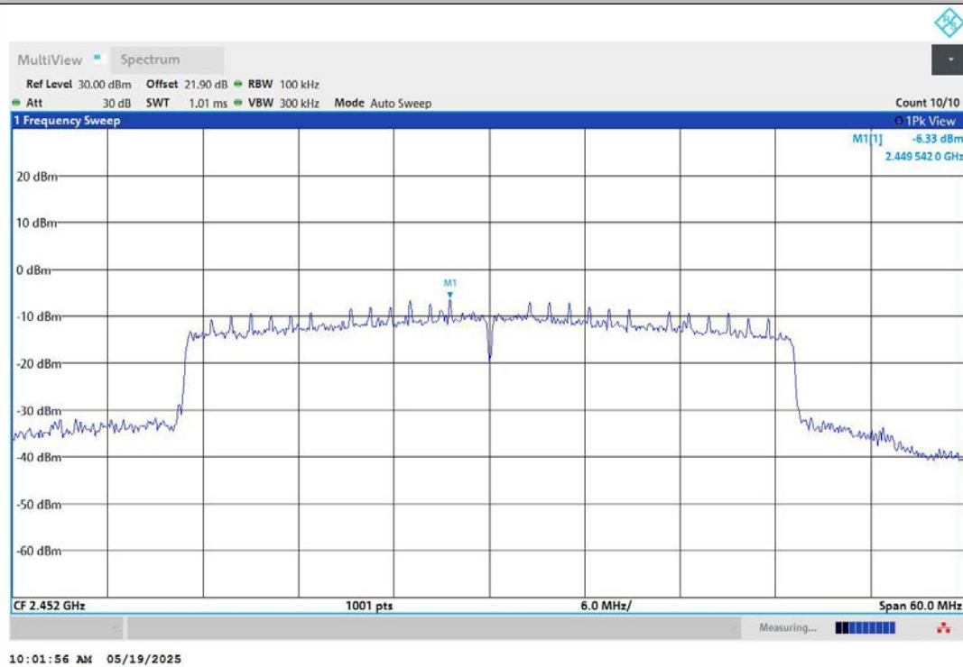
11AX40MIMO-Ant2-2452-0~Reference-PASS
