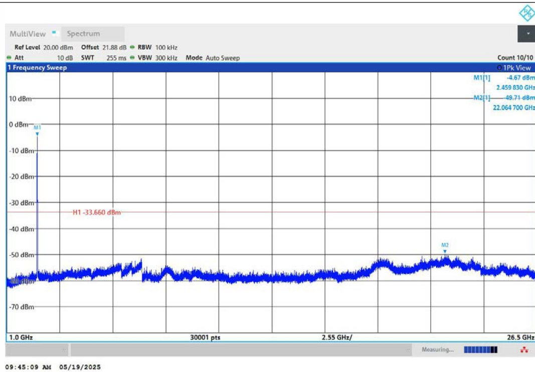
11AX20MIMO-Ant1-2462-1000~26500-PASS
