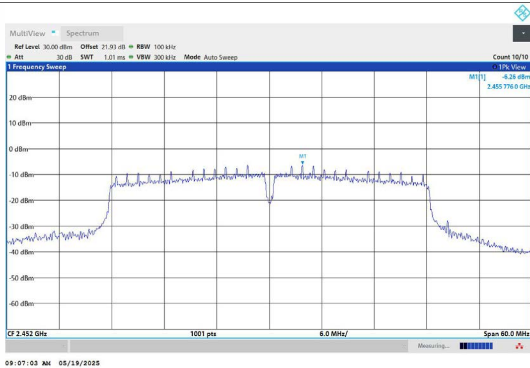
11N40MIMO-Ant1-2452-0~Reference-PASS
