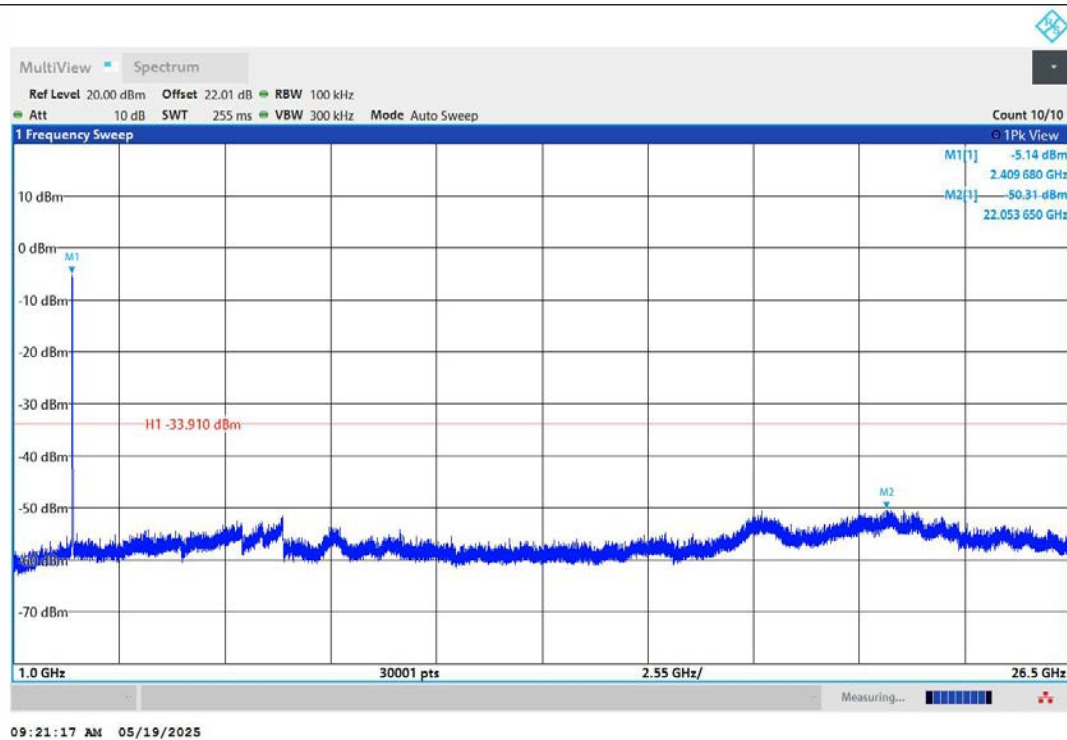
11AX20MIMO-Ant1-2412-1000~26500-PASS
