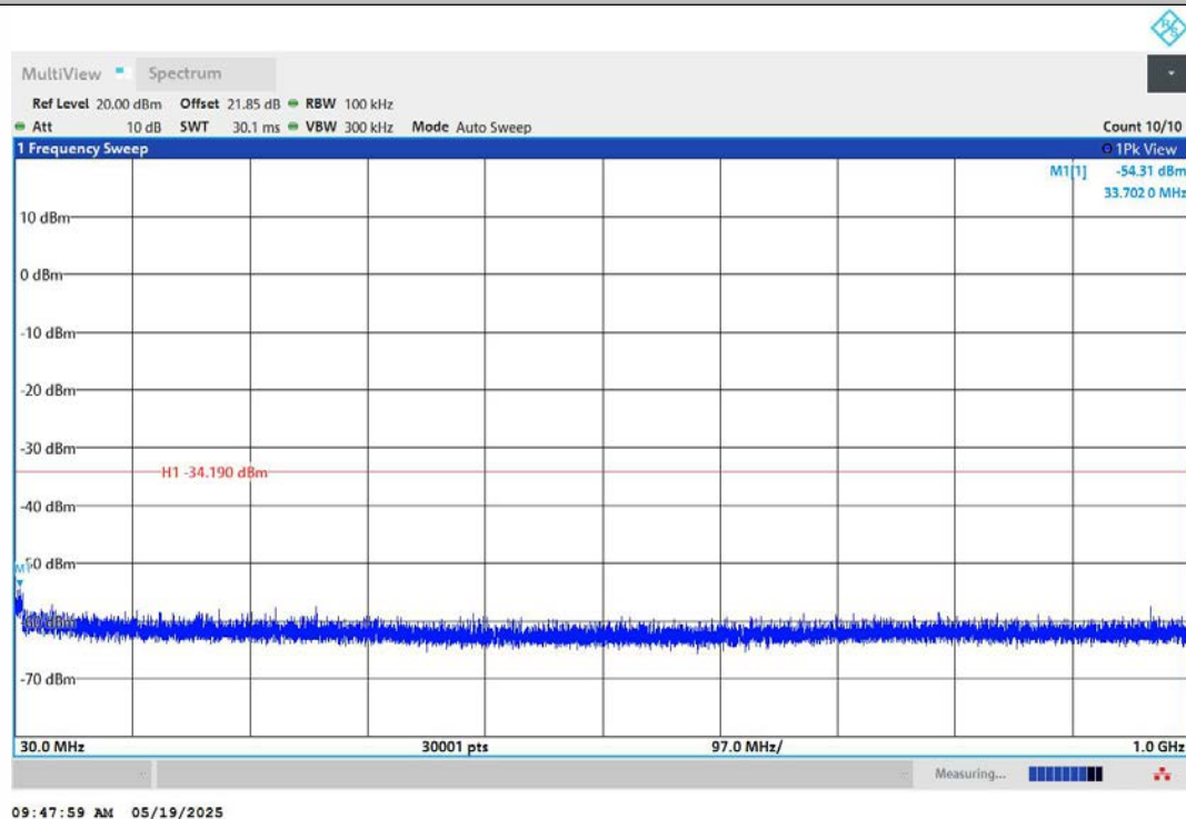
11AX20MIMO-Ant2-2462-30~1000-PASS
