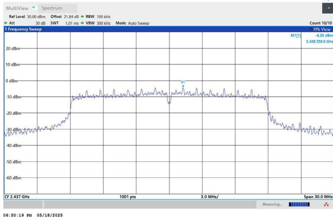
11N20MIMO-Ant2-2437-0~Reference-PASS
