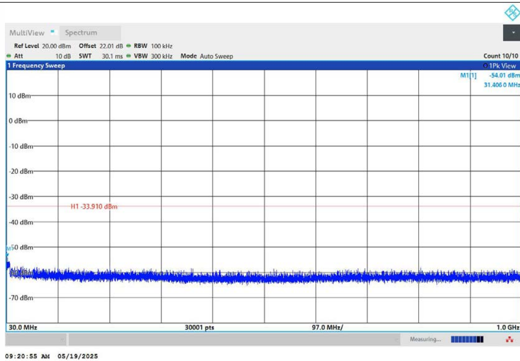
11AX20MIMO-Ant1-2412-30~1000-PASS
