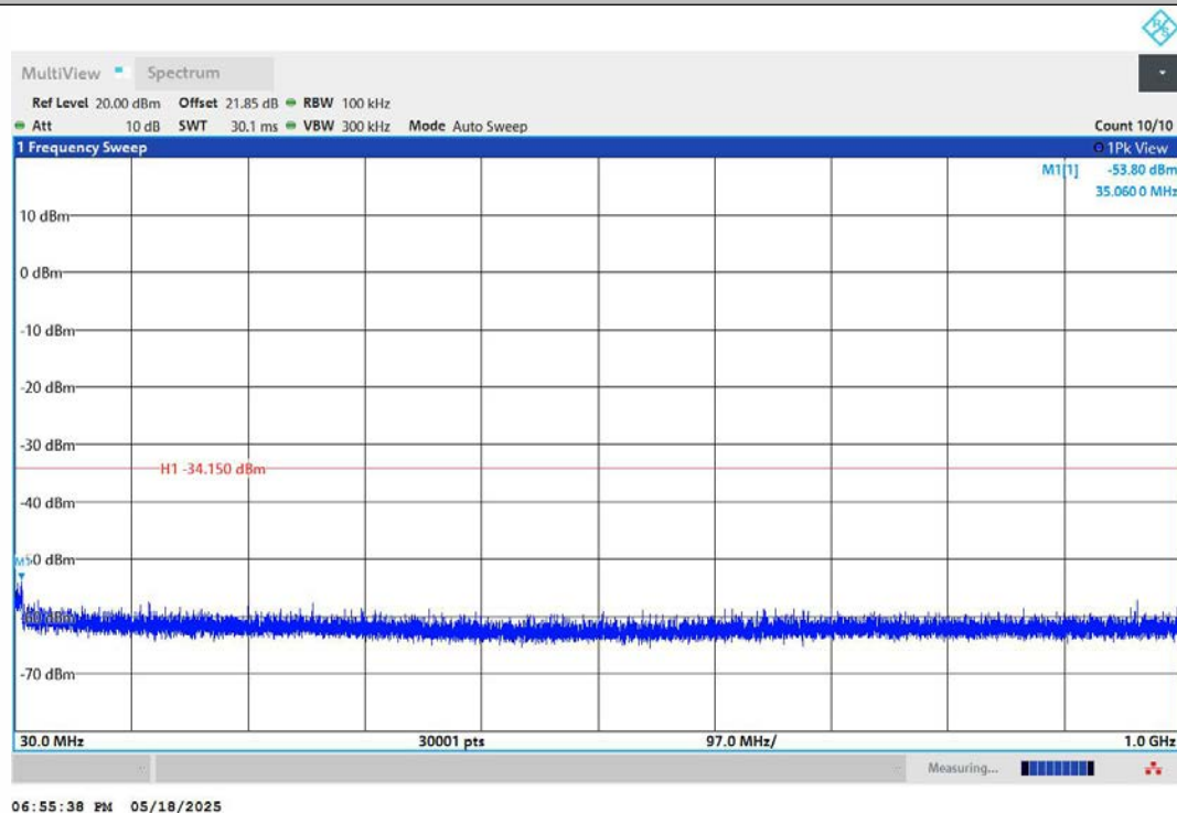
11N20MIMO-Ant2-2462-30~1000-PASS
