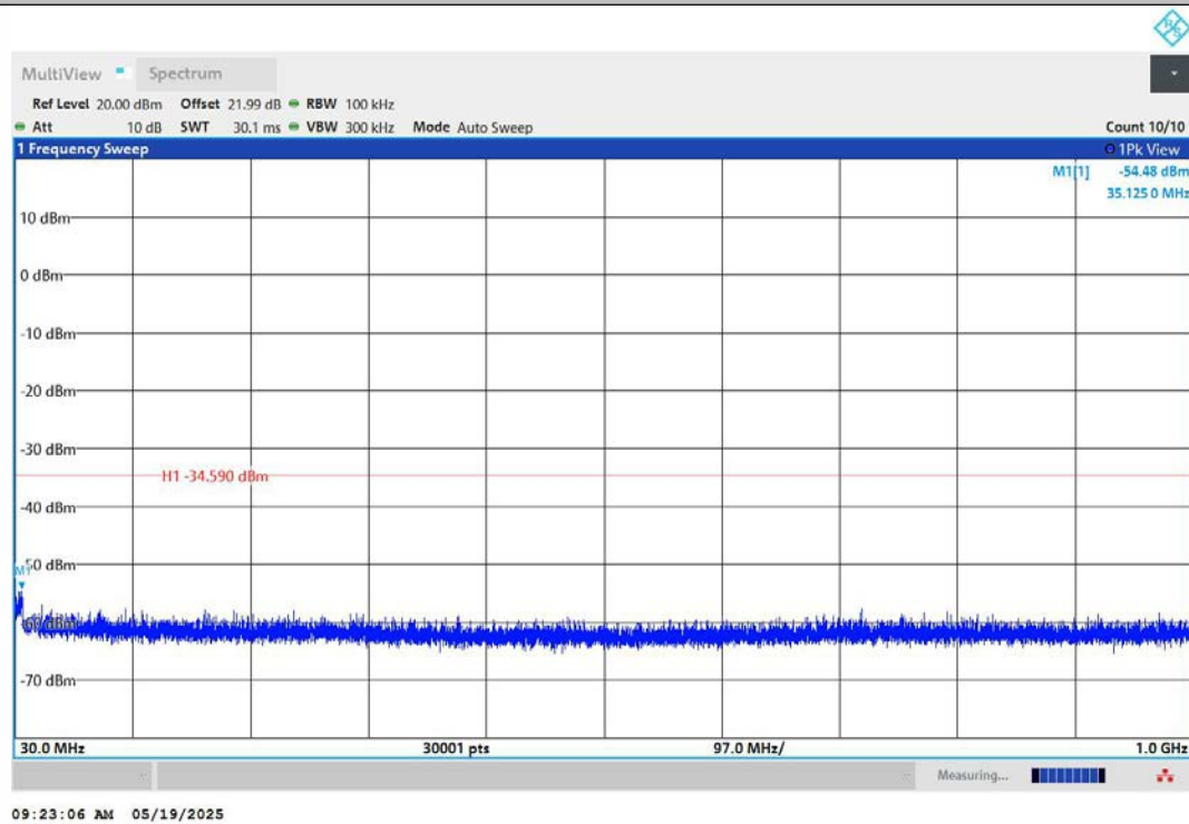
11AX20MIMO-Ant2-2412-30~1000-PASS
