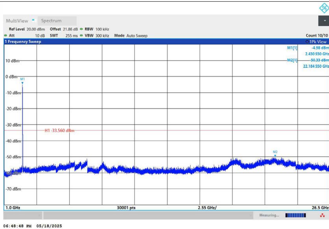
11N20MIMO-Ant1-2437-1000~26500-PASS
