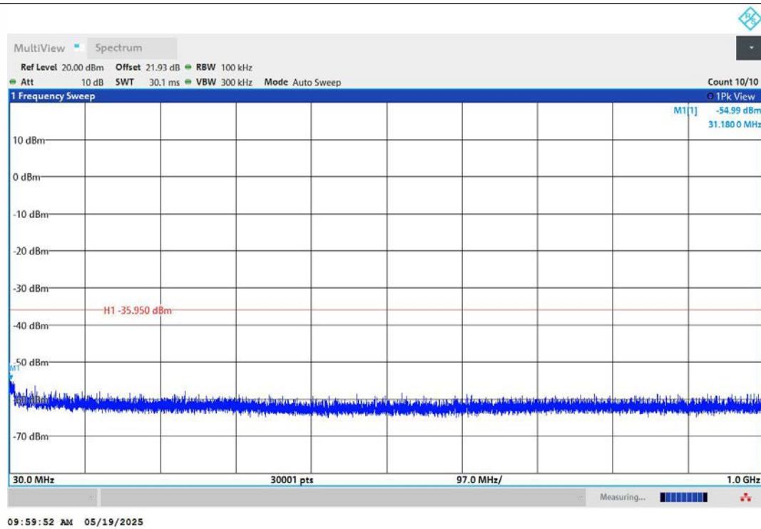
11AX40MIMO-Ant1-2452-30~1000-PASS
