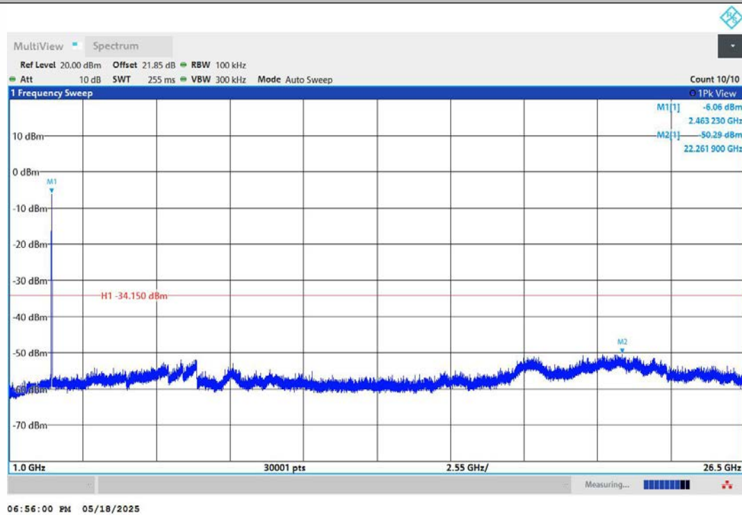
11N20MIMO-Ant2-2462-1000~26500-PASS
