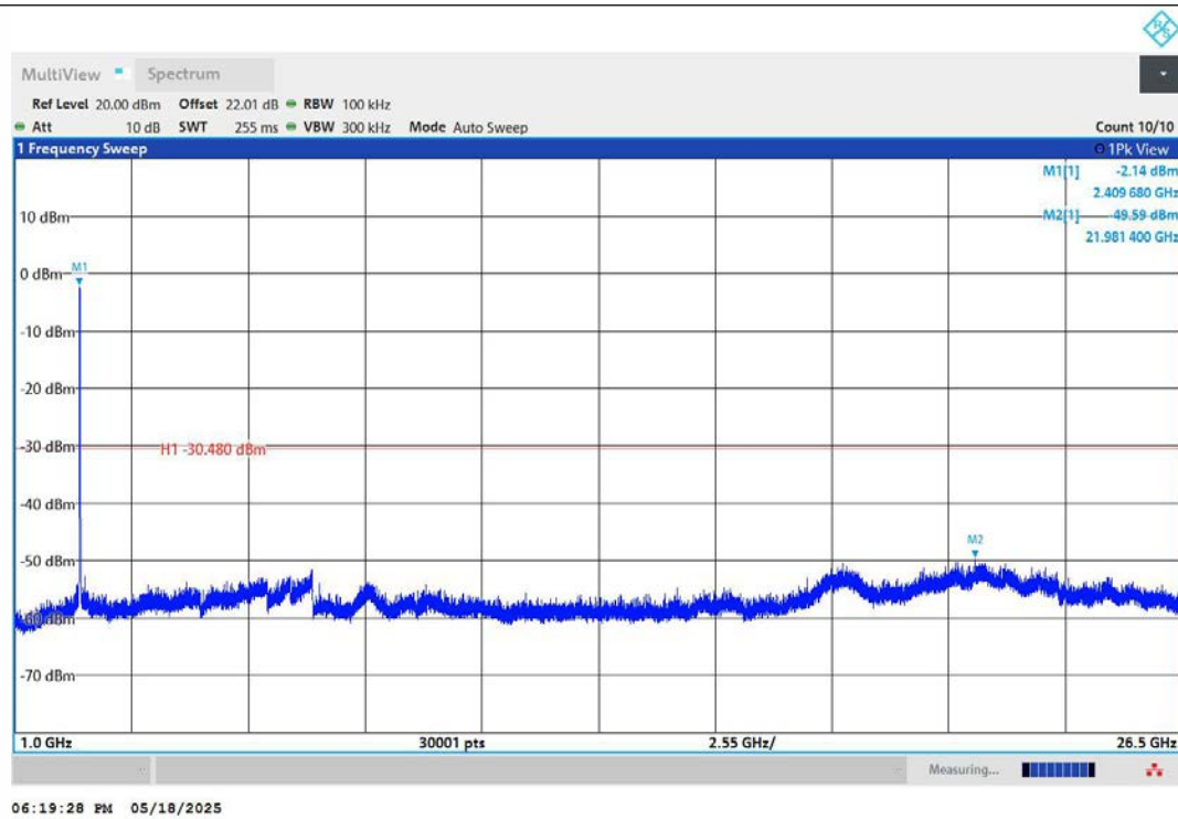
11G-Ant1-2412-1000~26500-PASS
