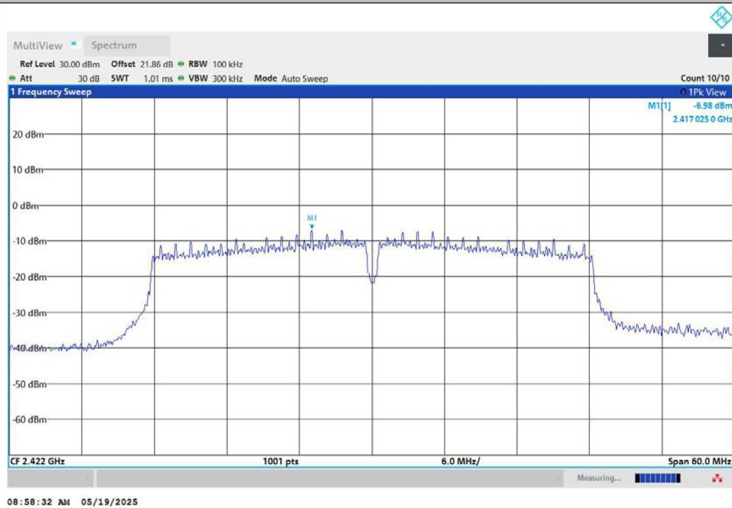
11N40MIMO-Ant2-2422-0~Reference-PASS
