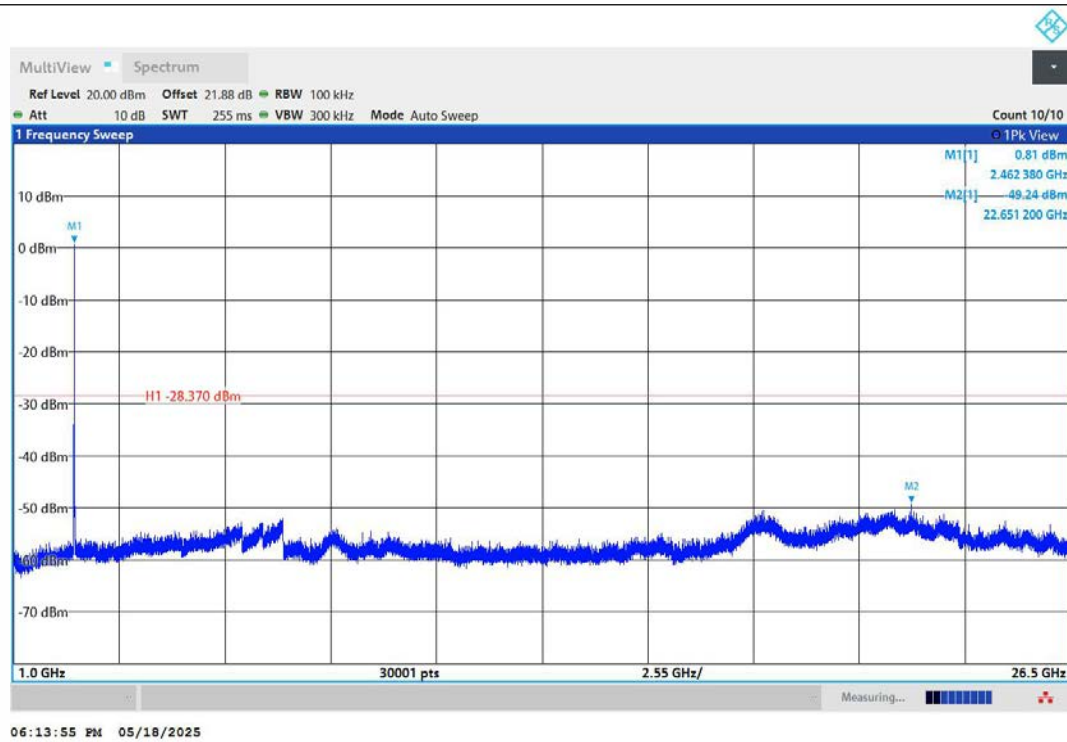
11B-Ant1-2462-1000~26500-PASS
