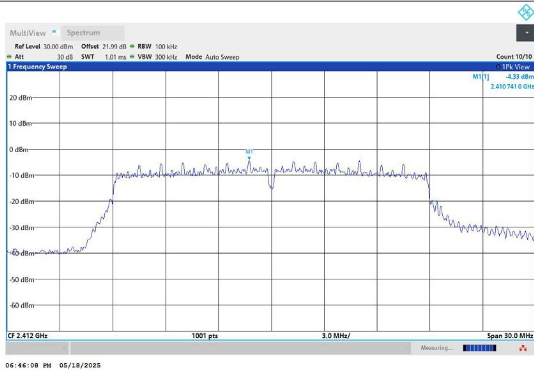
11N20MIMO-Ant2-2412-0~Reference-PASS
