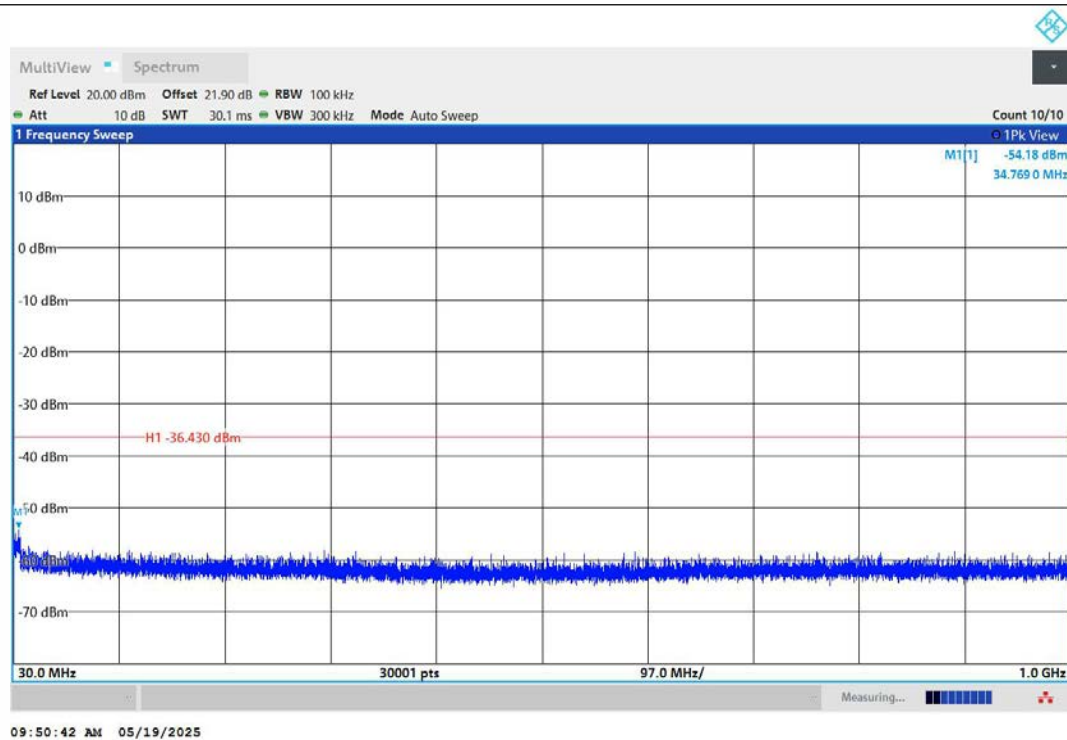
11AX40MIMO-Ant1-2422-30~1000-PASS
