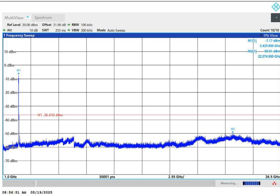
11N40MIMO-Ant1-2422-1000~26500-PASS
