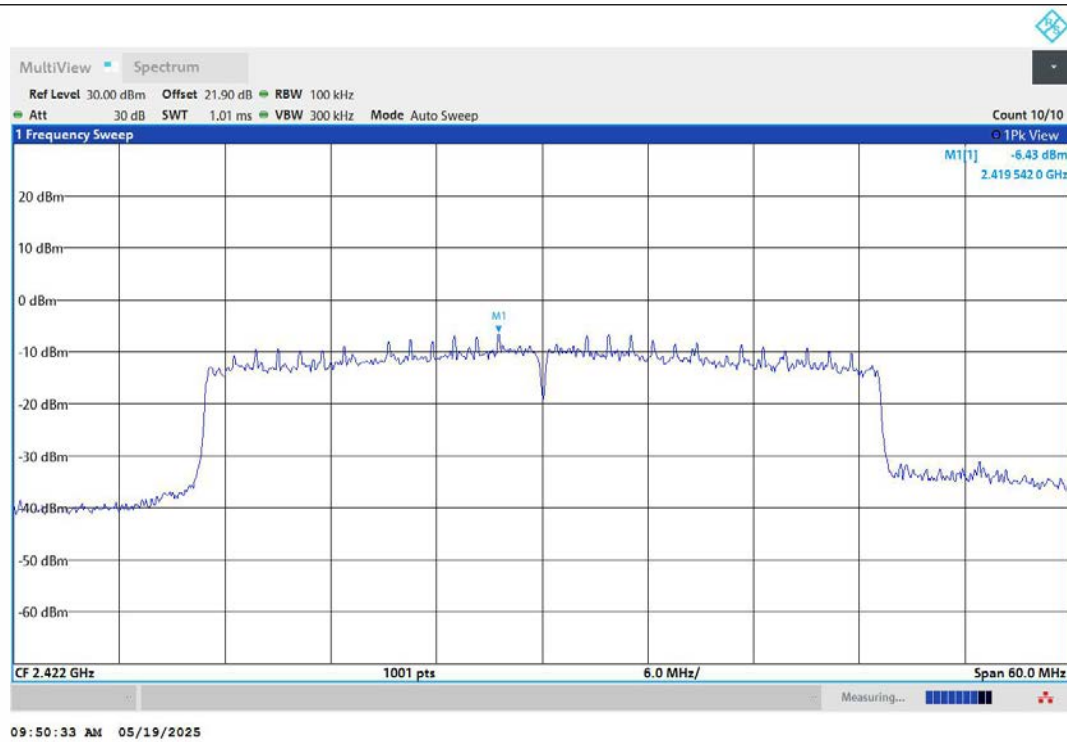
11AX40MIMO-Ant1-2422-0~Reference-PASS
