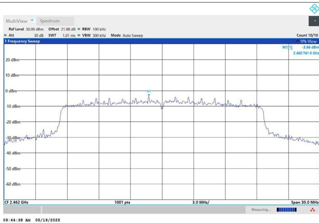
11AX20MIMO-Ant1-2462-0~Reference-PASS
