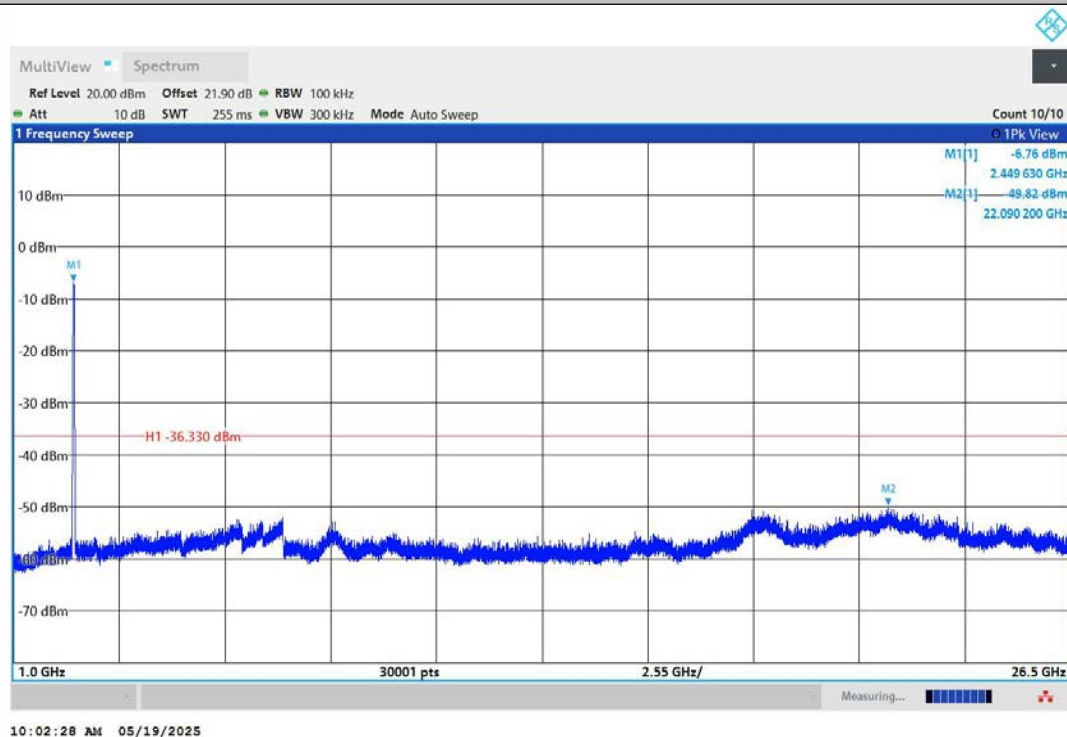
11AX40MIMO-Ant2-2452-1000~26500-PASS
