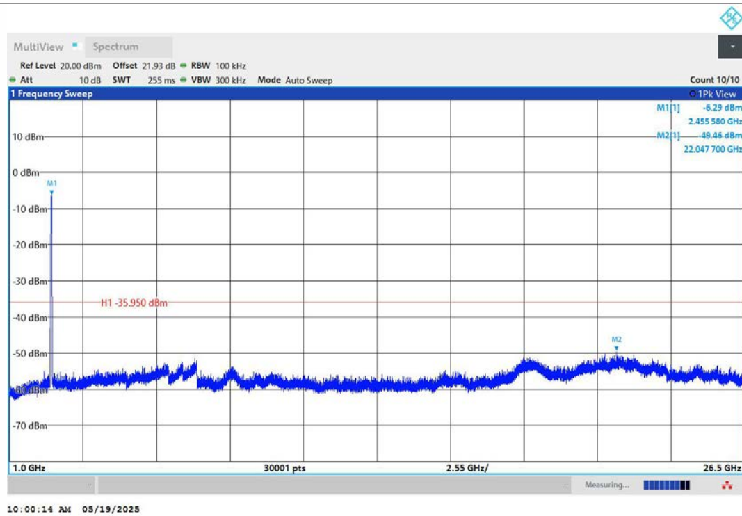
11AX40MIMO-Ant1-2452-1000~26500-PASS
