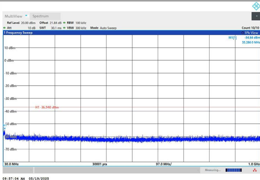
11AX40MIMO-Ant2-2437-30~1000-PASS
