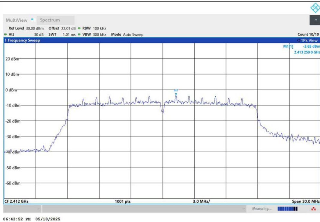
11N20MIMO-Ant1-2412-0~Reference-PASS
