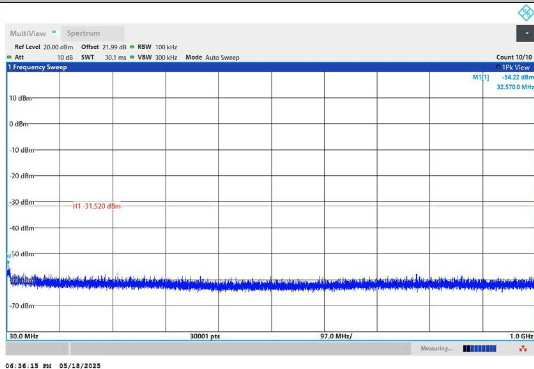
11G-Ant2-2412-30~1000-PASS
