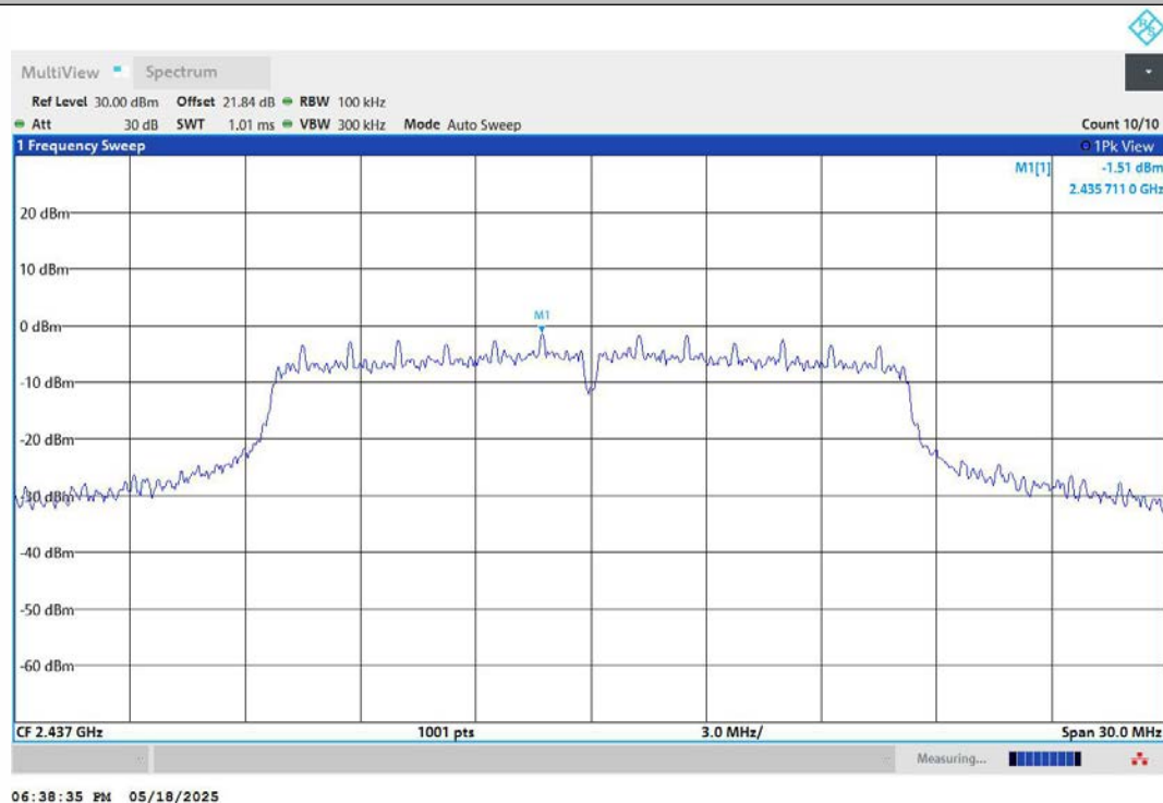
11G-Ant2-2437-0~Reference-PASS
