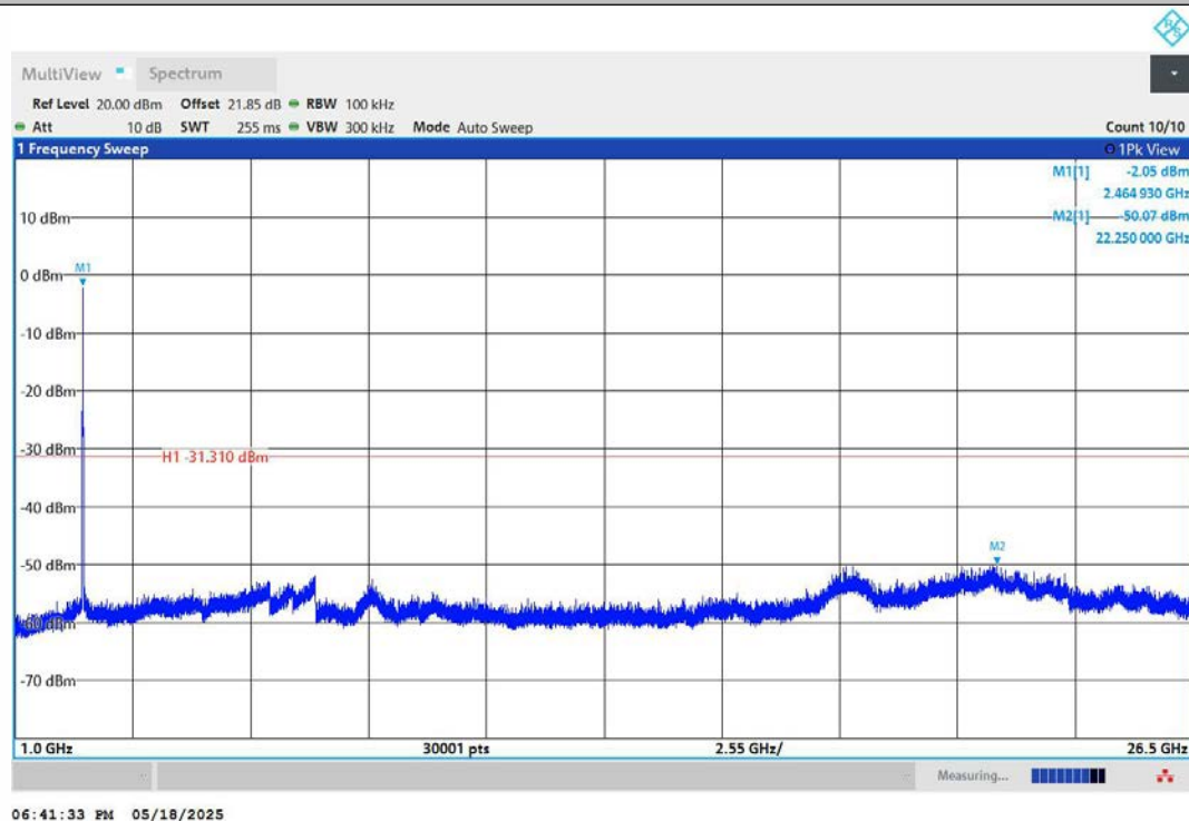
11G-Ant2-2462-1000~26500-PASS
