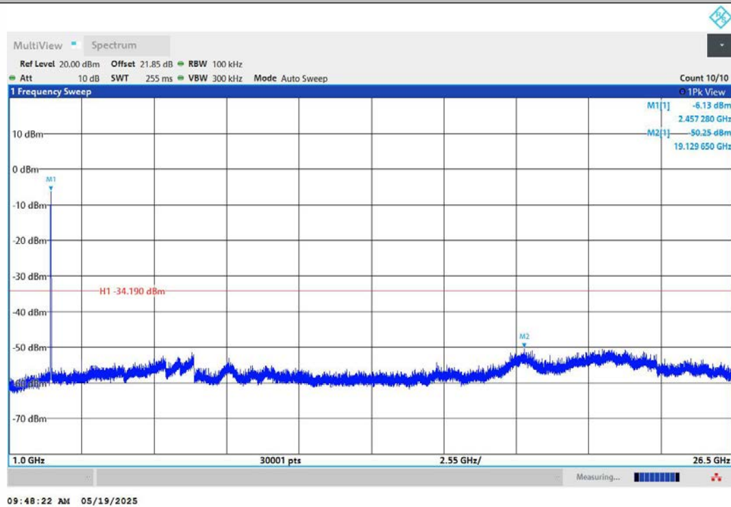
11AX20MIMO-Ant2-2462-1000~26500-PASS
