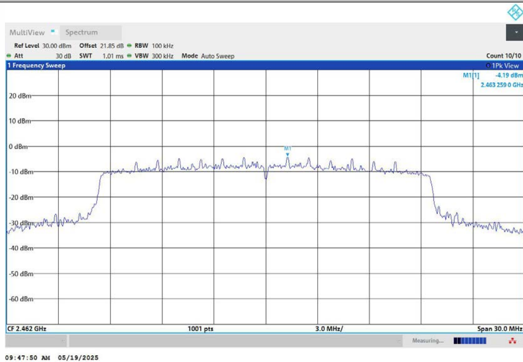
11AX20MIMO-Ant2-2462-0~Reference-PASS
