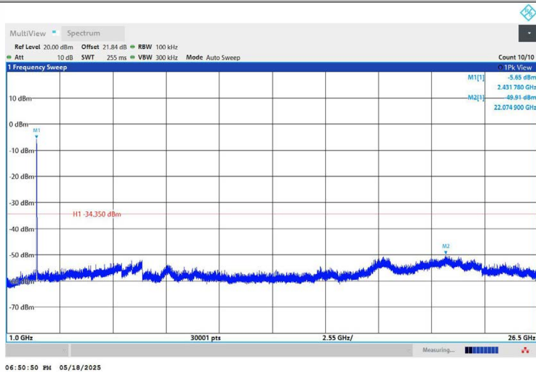
11N20MIMO-Ant2-2437-1000~26500-PASS
