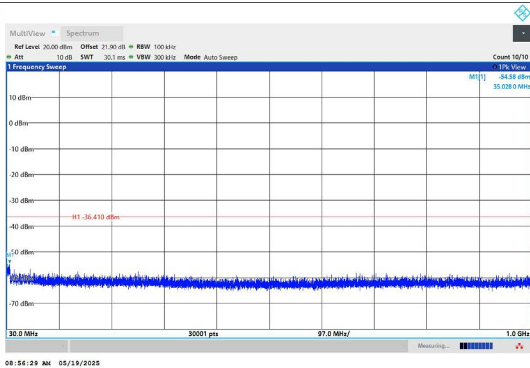
11N40MIMO-Ant1-2422-30~1000-PASS
