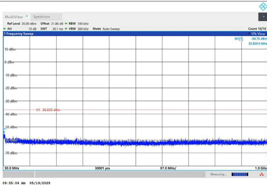
11AX40MIMO-Ant1-2437-30~1000-PASS
