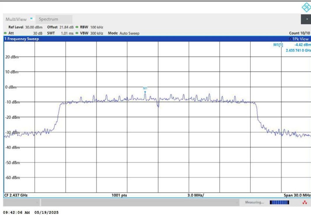
11AX20MIMO-Ant2-2437-0~Reference-PASS
