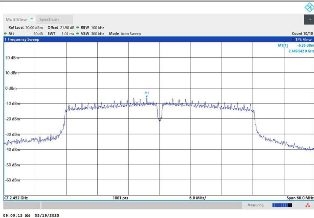
11N40MIMO-Ant2-2452-0~Reference-PASS
