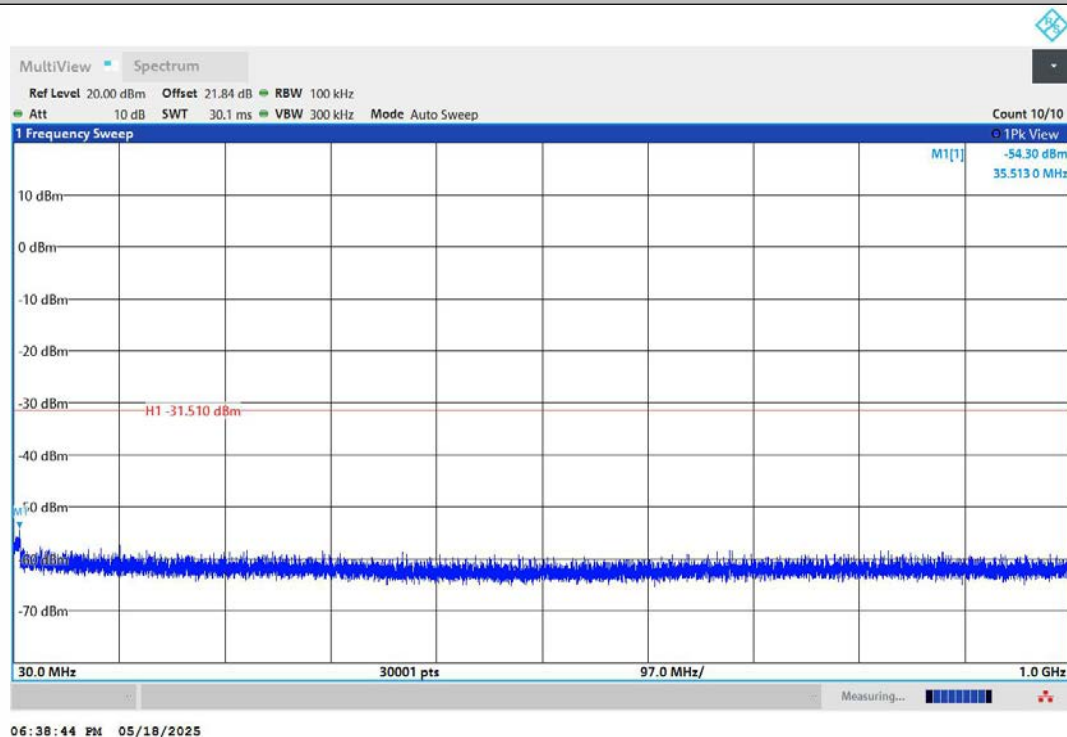
11G-Ant2-2437-30~1000-PASS
