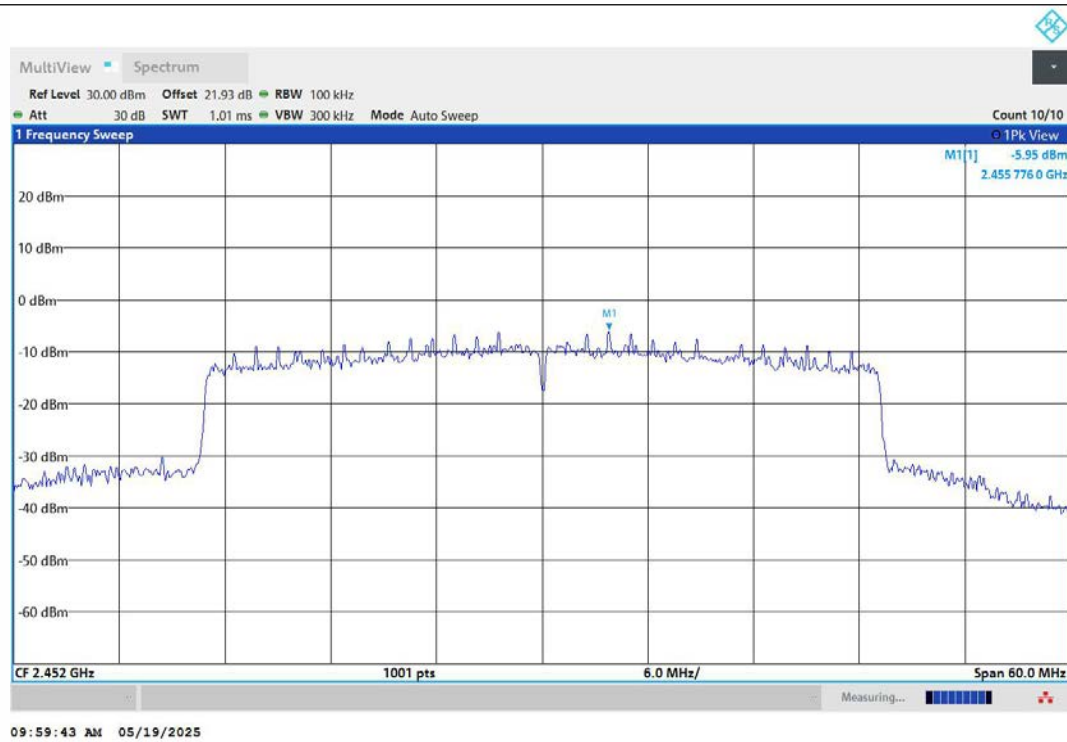
11AX40MIMO-Ant1-2452-0~Reference-PASS
