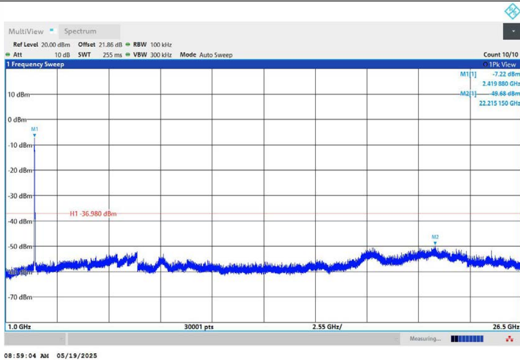
11N40MIMO-Ant2-2422-1000~26500-PASS
