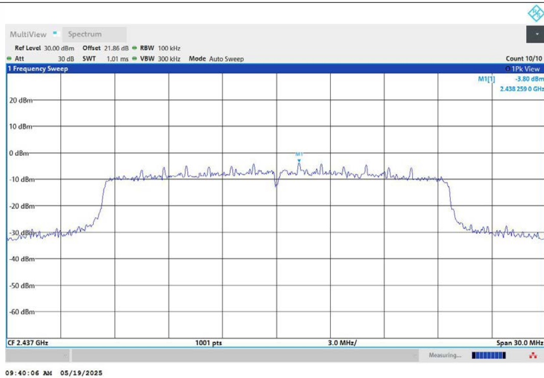
11AX20MIMO-Ant1-2437-0~Reference-PASS
