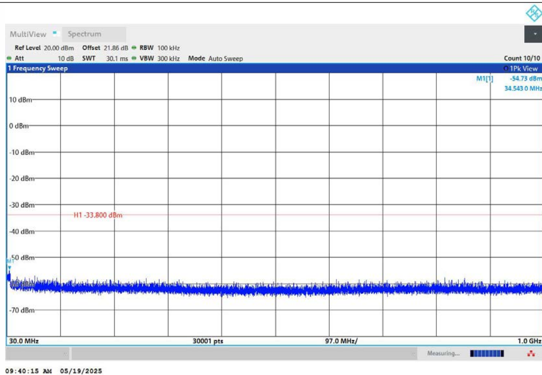
11AX20MIMO-Ant1-2437-30~1000-PASS
