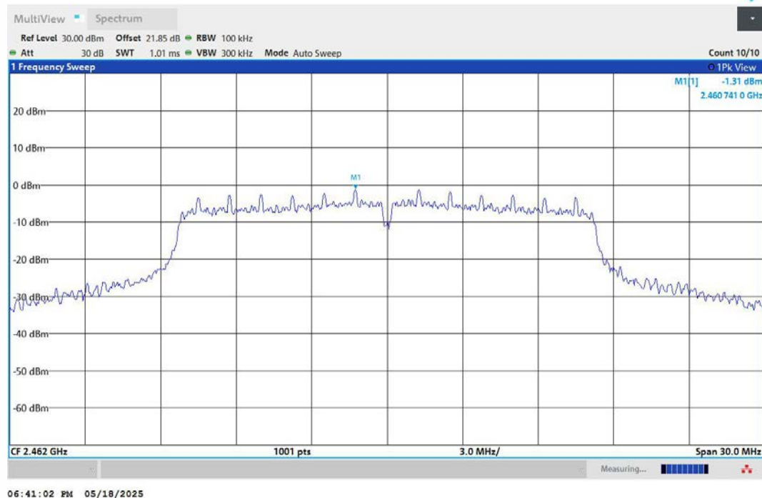
11G-Ant2-2462-0~Reference-PASS
