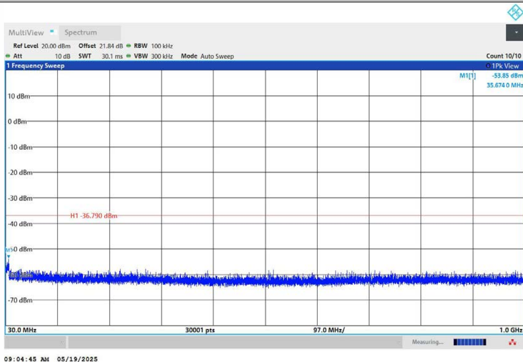
11N40MIMO-Ant2-2437-30~1000-PASS
