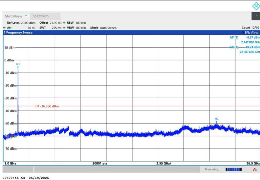
11N40MIMO-Ant2-2452-1000~26500-PASS
