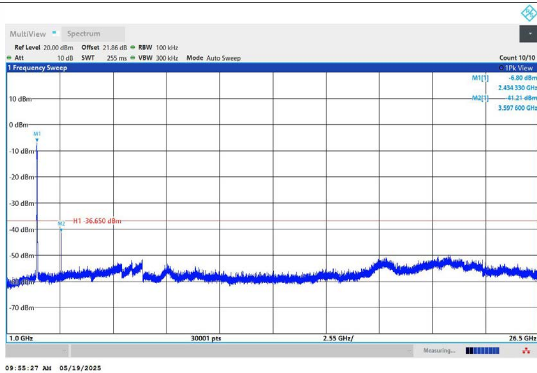
11AX40MIMO-Ant1-2437-1000~26500-PASS
