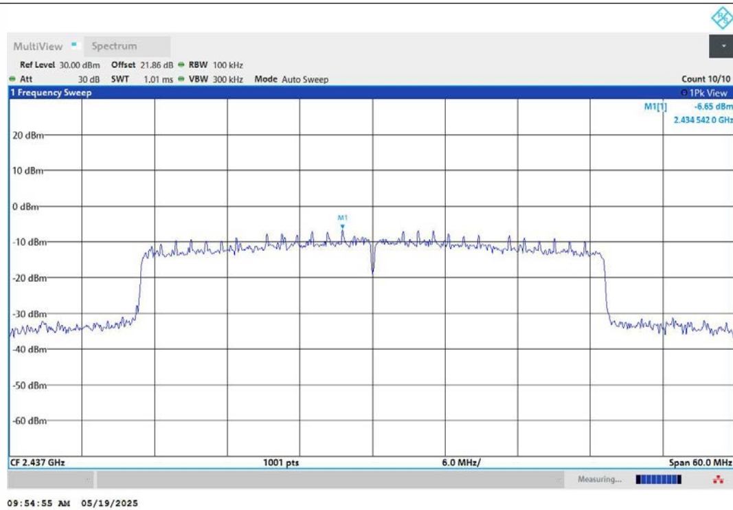
11AX40MIMO-Ant1-2437-0~Reference-PASS
