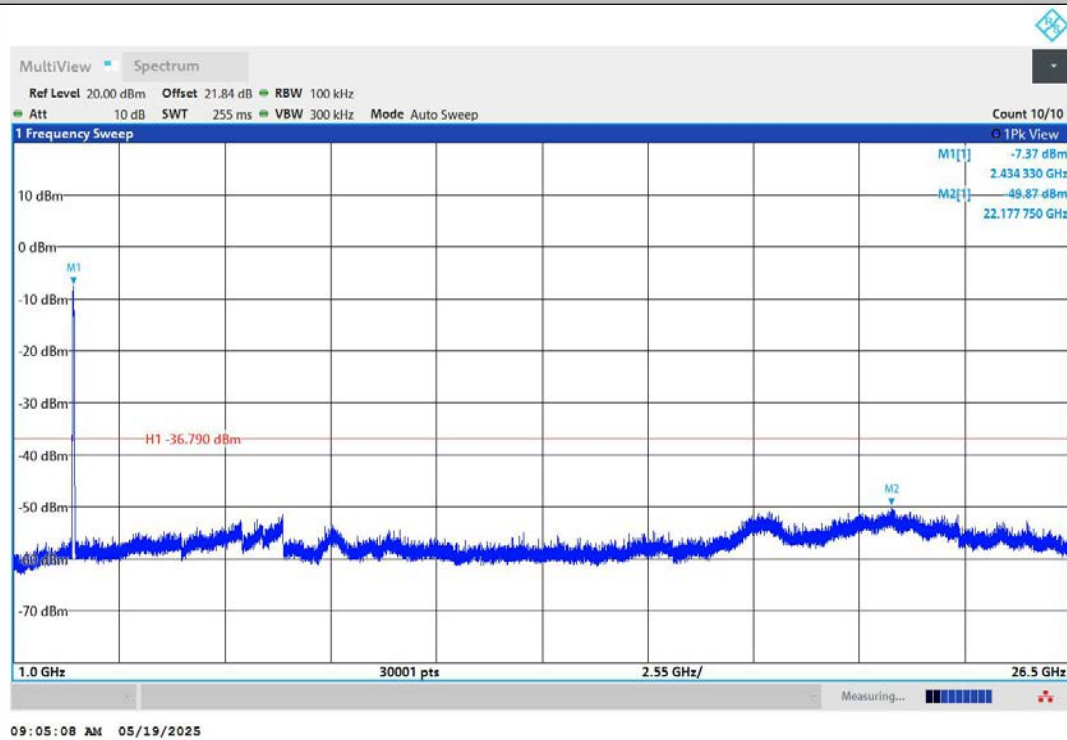
11N40MIMO-Ant2-2437-1000~26500-PASS
