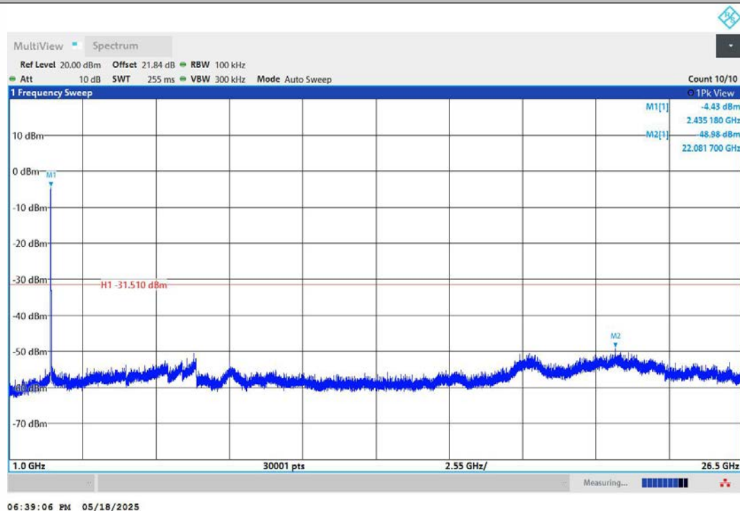
11G-Ant2-2437-1000~26500-PASS
