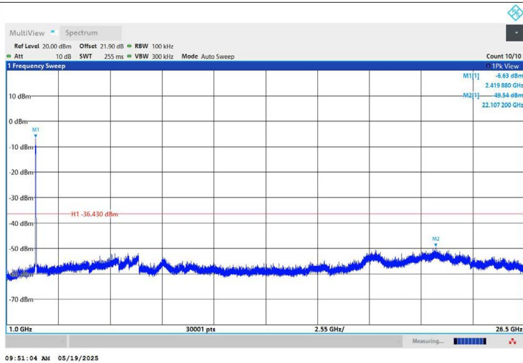
11AX40MIMO-Ant1-2422-1000~26500-PASS
