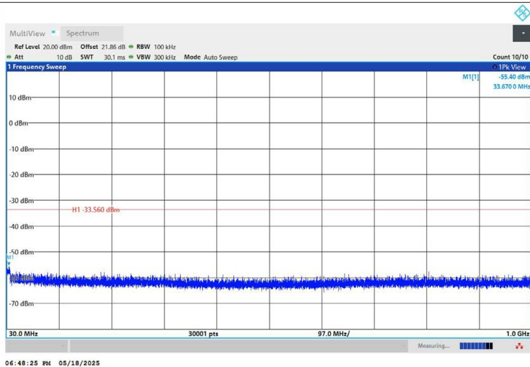
11N20MIMO-Ant1-2437-30~1000-PASS
