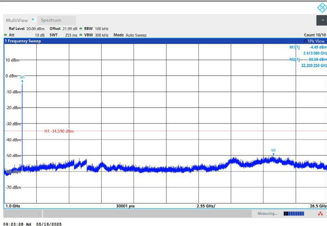
11AX20MIMO-Ant2-2412-1000~26500-PASS
