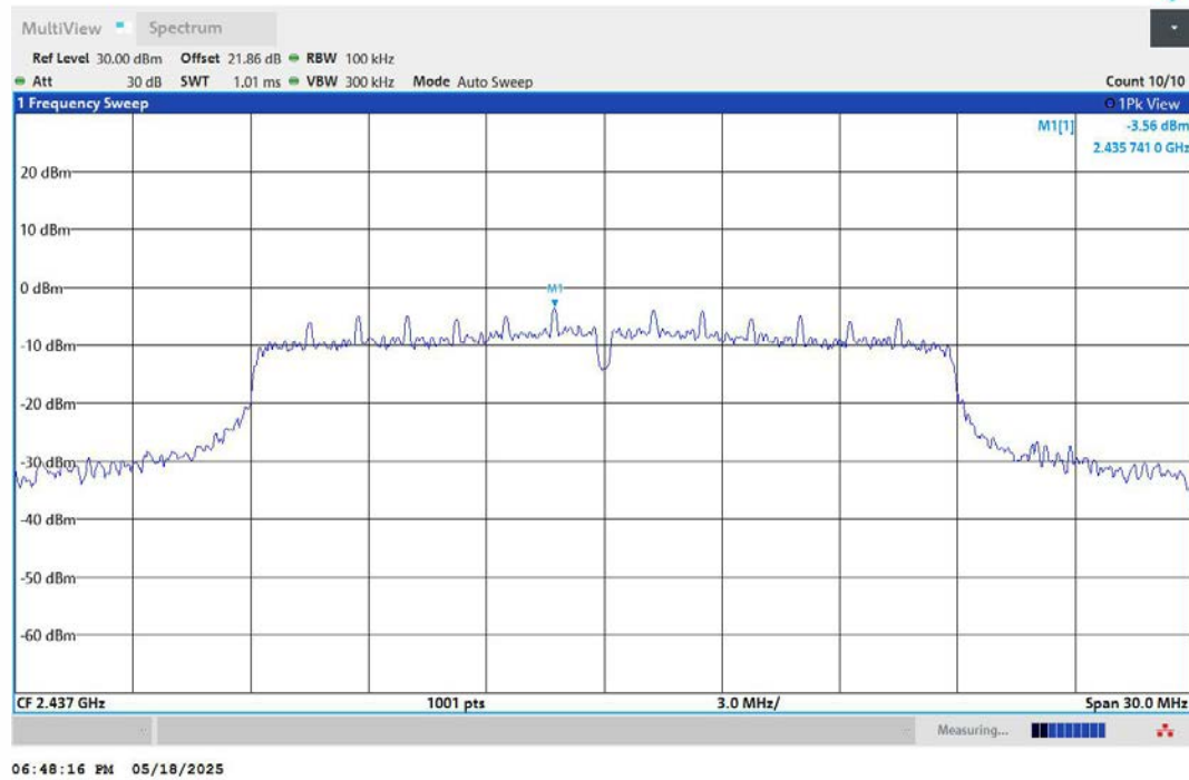
11N20MIMO-Ant1-2437-0~Reference-PASS
