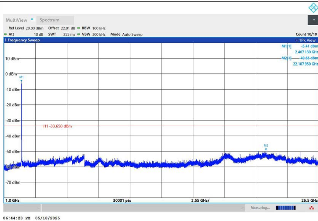
11N20MIMO-Ant1-2412-1000~26500-PASS
