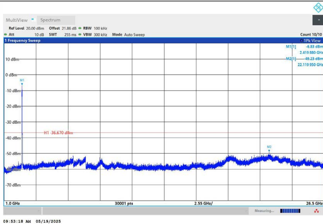
11AX40MIMO-Ant2-2422-1000~26500-PASS
