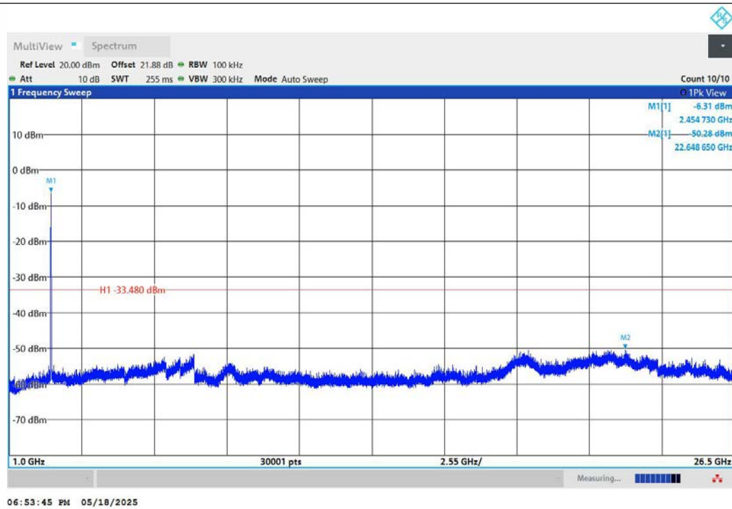
11N20MIMO-Ant1-2462-1000~26500-PASS
