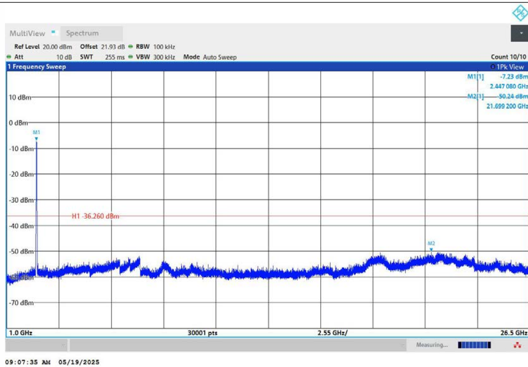
11N40MIMO-Ant1-2452-1000~26500-PASS
