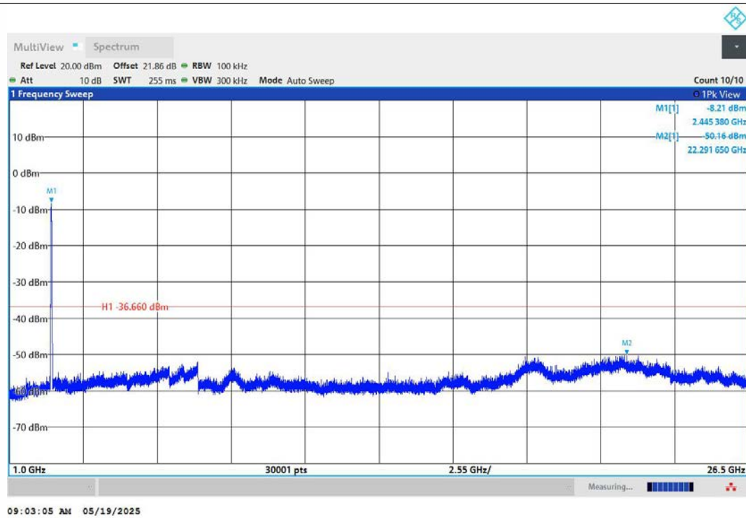
11N40MIMO-Ant1-2437-1000~26500-PASS
