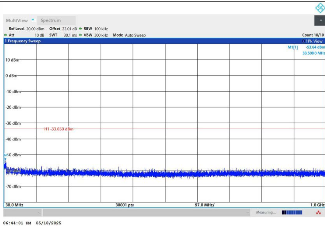
11N20MIMO-Ant1-2412-30~1000-PASS
