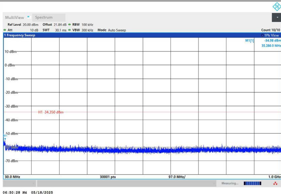
11N20MIMO-Ant2-2437-30~1000-PASS
