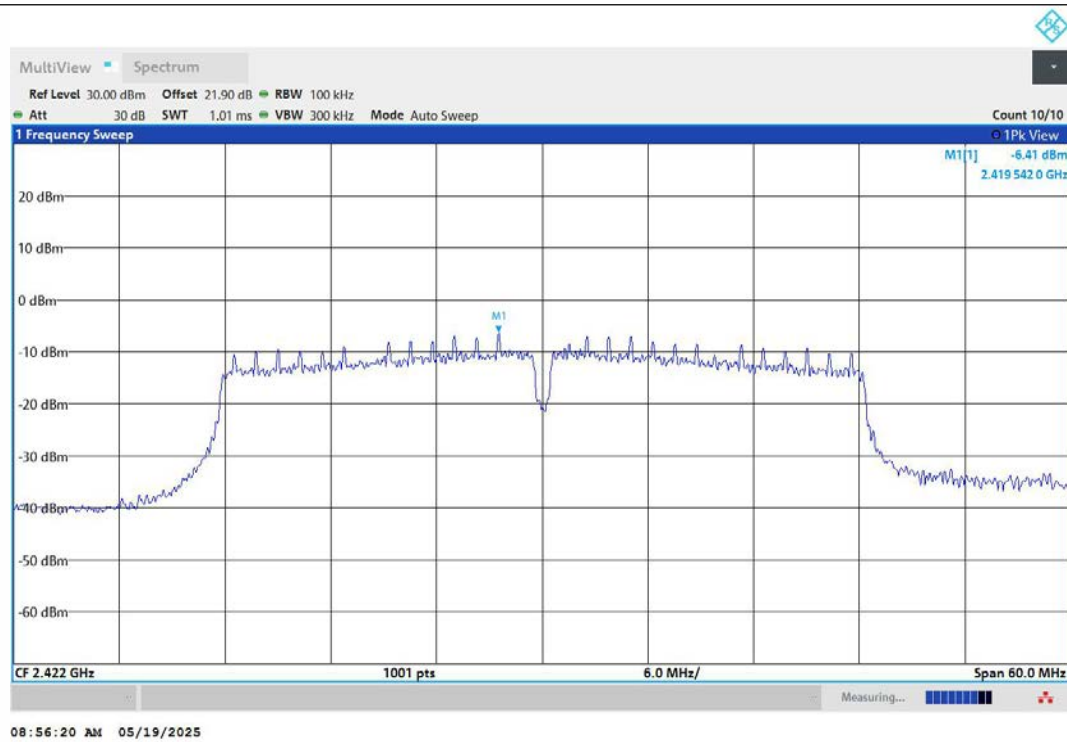
11N40MIMO-Ant1-2422-0~Reference-PASS
