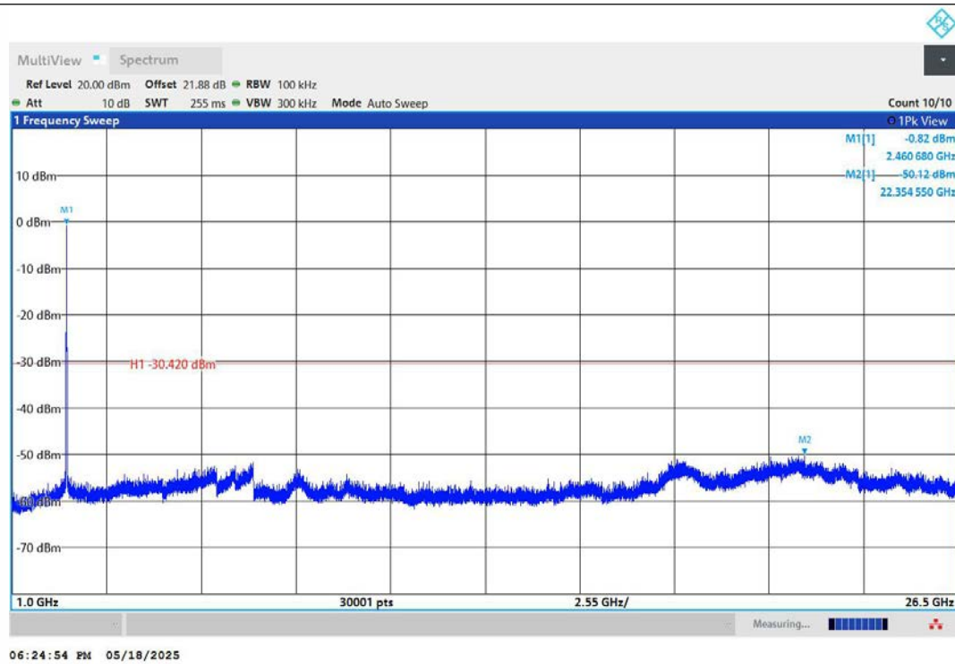
11G-Ant1-2462-1000~26500-PASS
