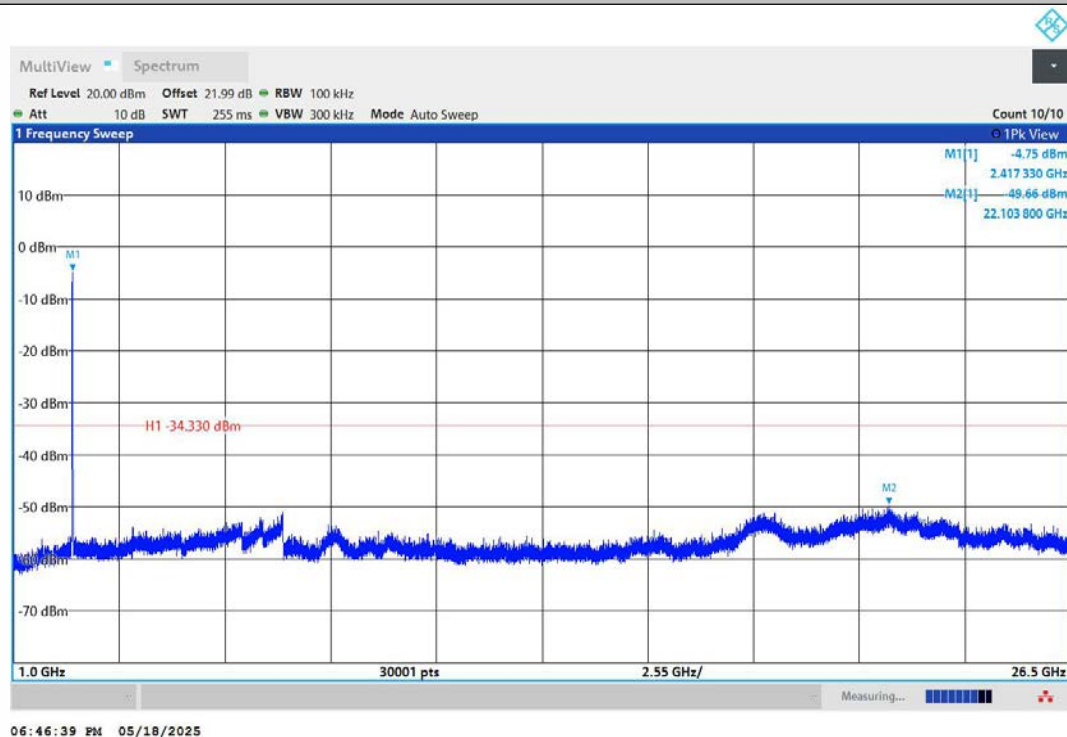
11N20MIMO-Ant2-2412-1000~26500-PASS
