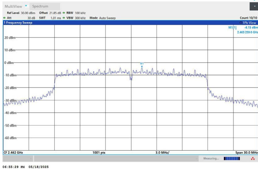
11N20MIMO-Ant2-2462-0~Reference-PASS
