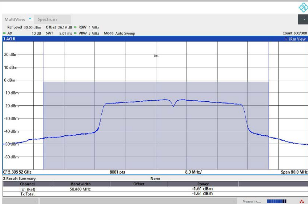
11AC40MIMO-Ant1-5310-TPC_L-PASS
