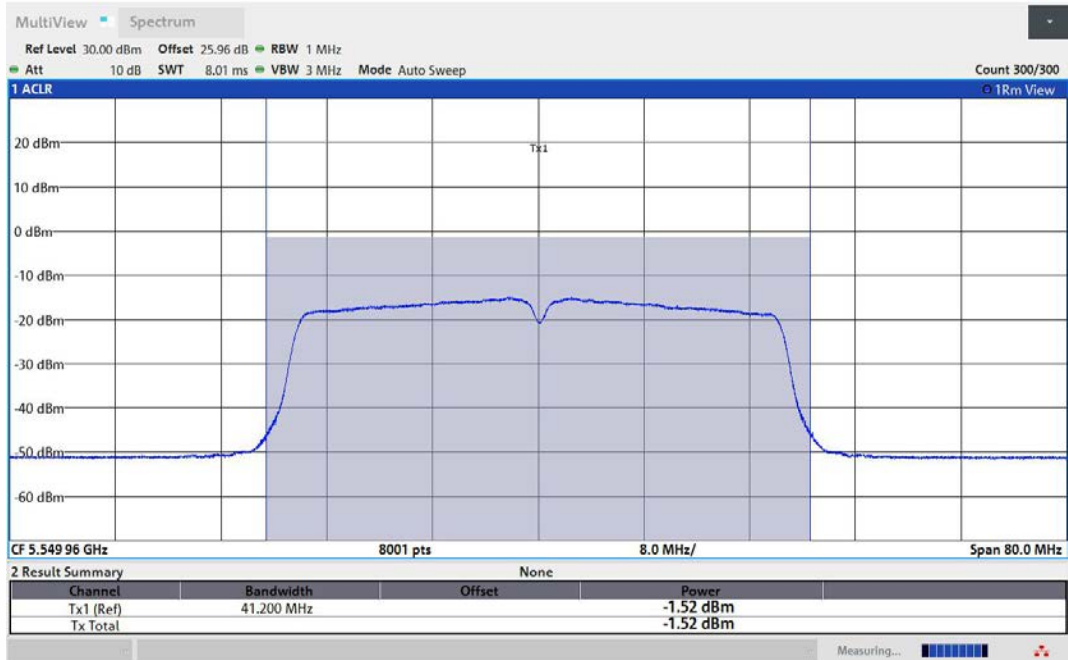
11AC40MIMO-Ant1-5550-TPC_L-PASS
