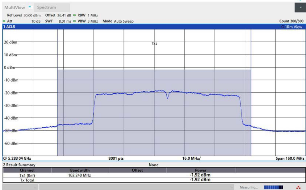
11AC80MIMO-Ant3-5290-TPC_L-PASS
