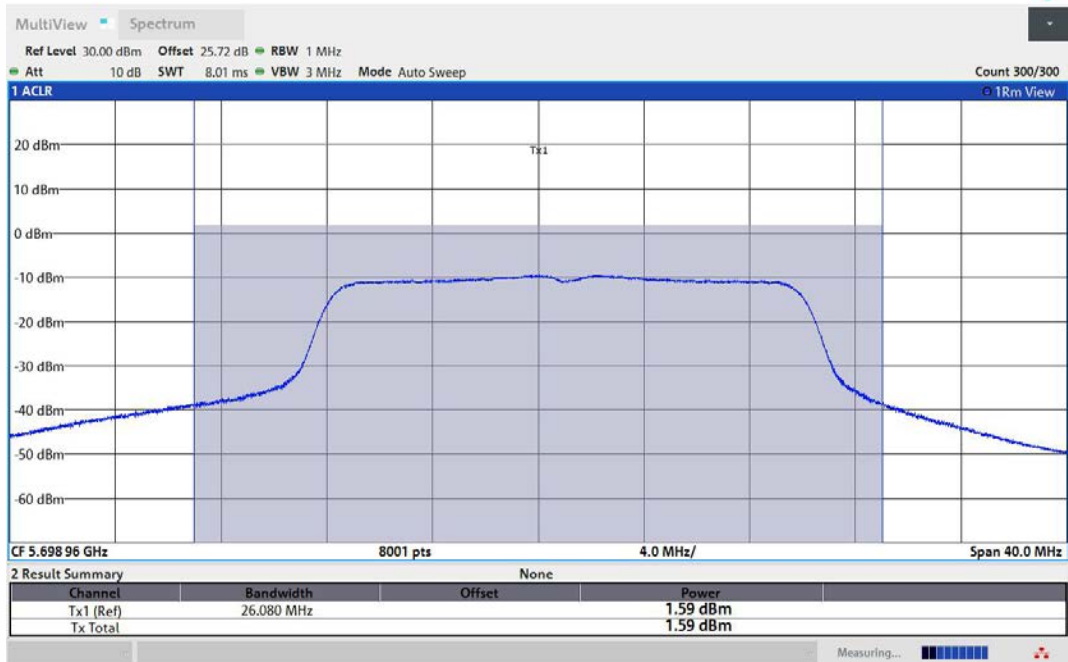
11AC20MIMO-Ant1-5700-TPC_H-PASS
