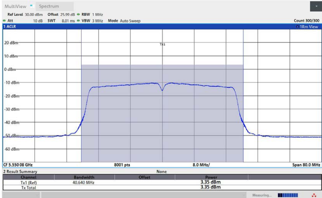
11AC40MIMO-Ant3-5550-TPC_H-PASS
