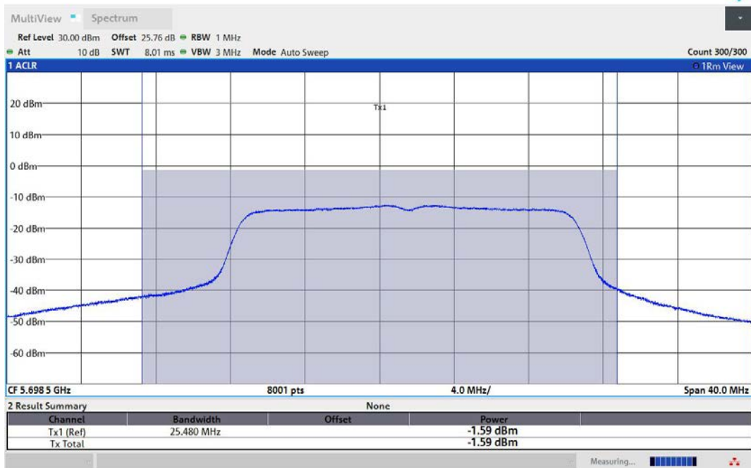
11AC20MIMO-Ant3-5700-TPC_L-PASS
