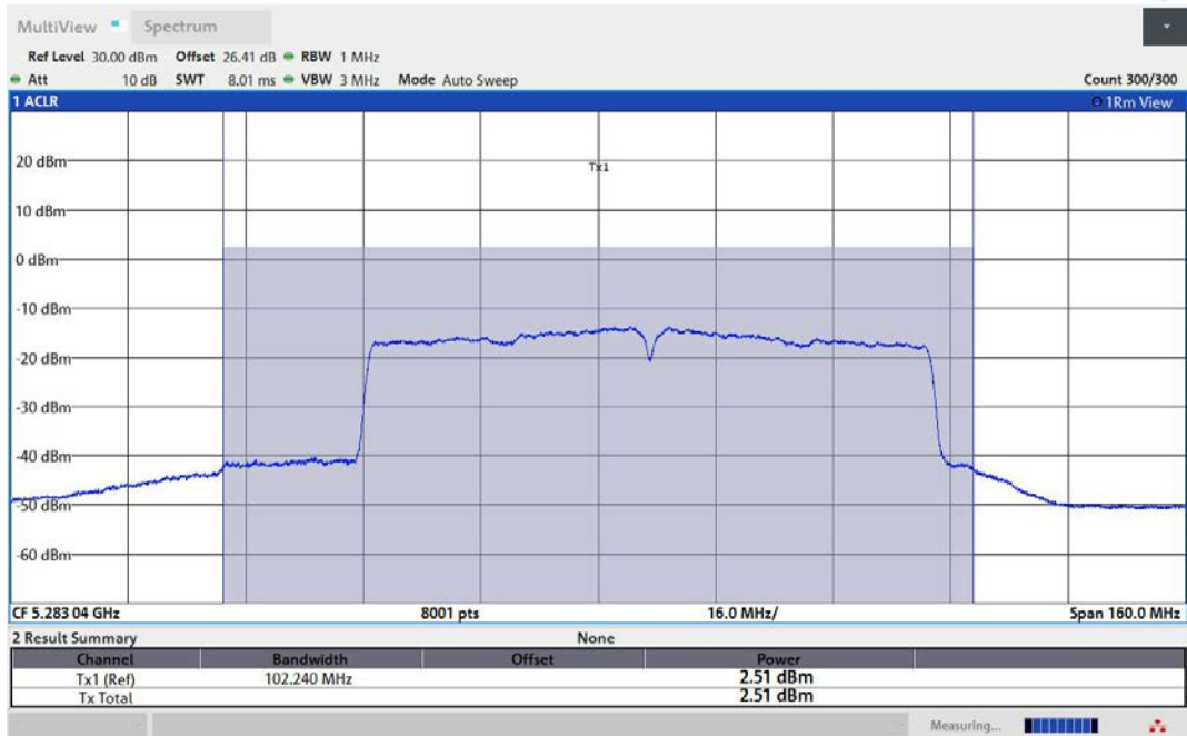
11AC80MIMO-Ant3-5290-TPC_H-PASS
