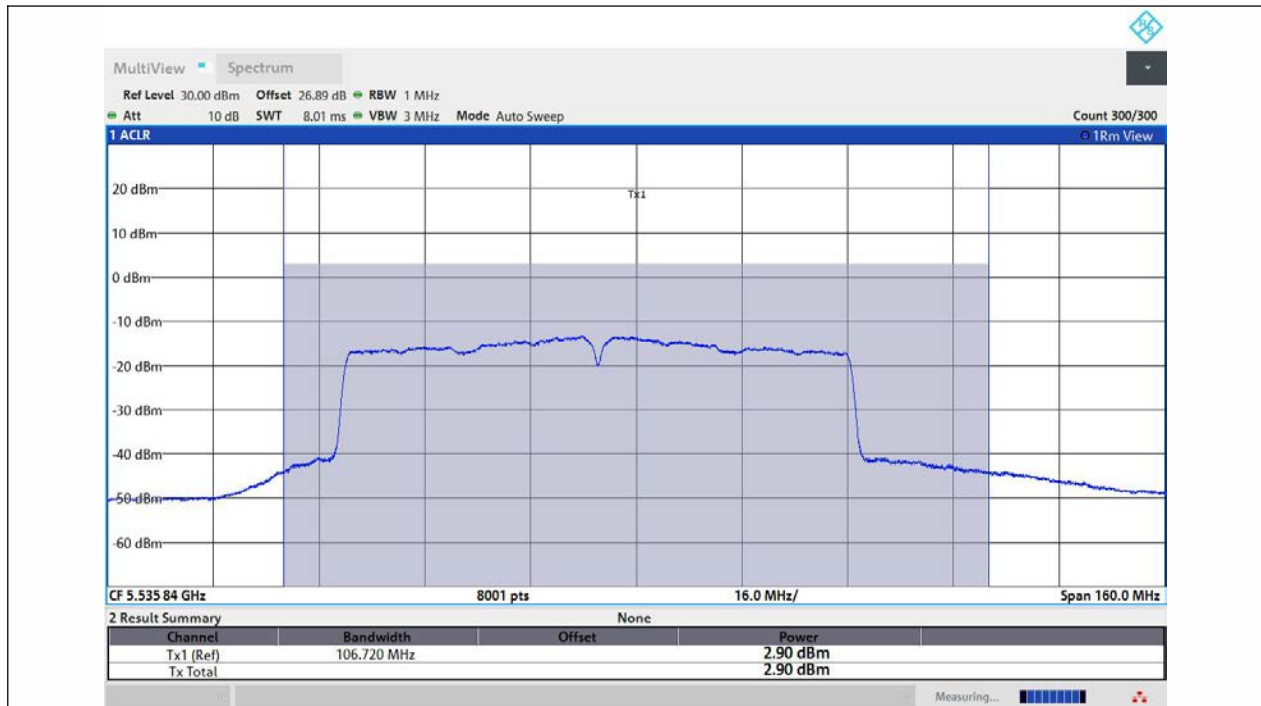
11AC80MIMO-Ant2-5530-TPC_H-PASS
