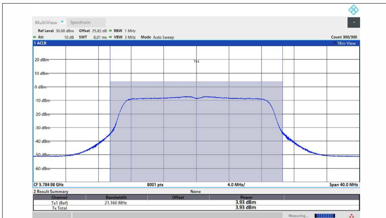
11AC20MIMO-Ant3-5785-PASS
