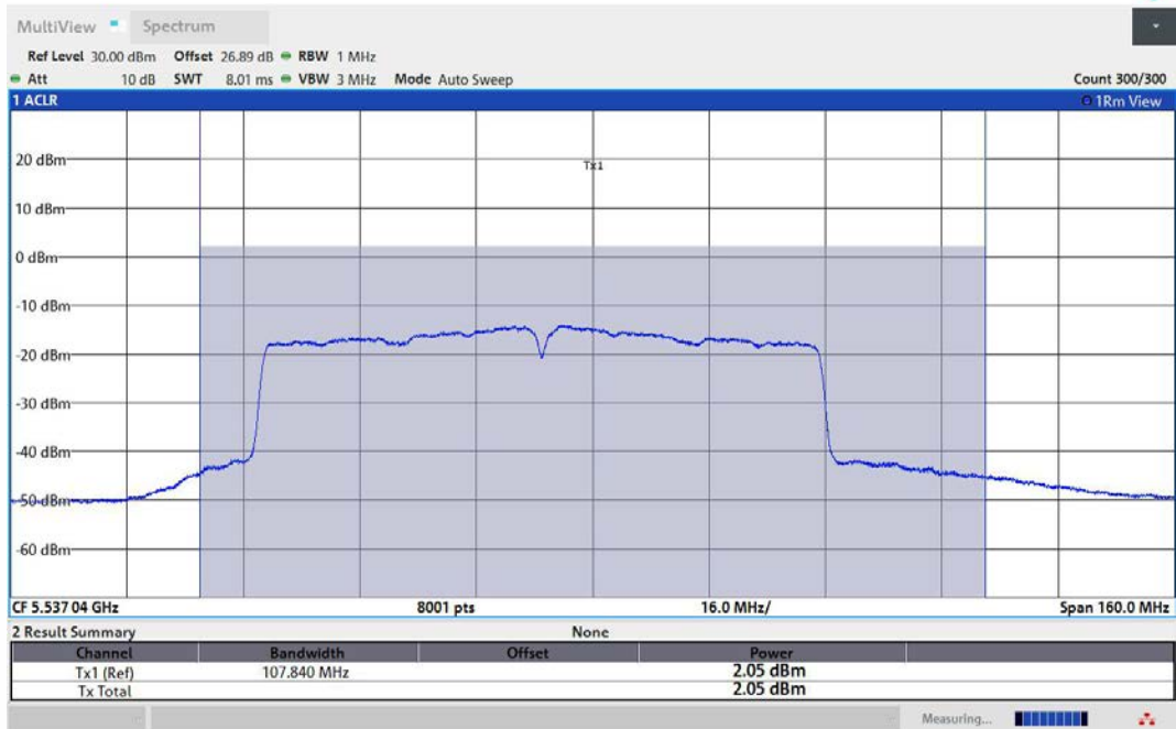
11AC80MIMO-Ant1-5530-TPC_H-PASS
