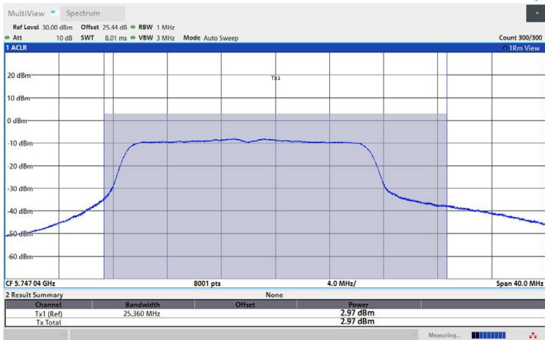
11AC20MIMO-Ant3-5745-PASS
