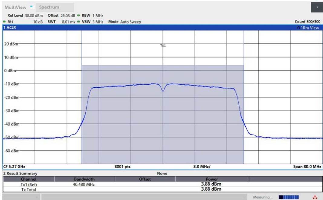
11AC40MIMO-Ant2-5270-TPC_H-PASS
