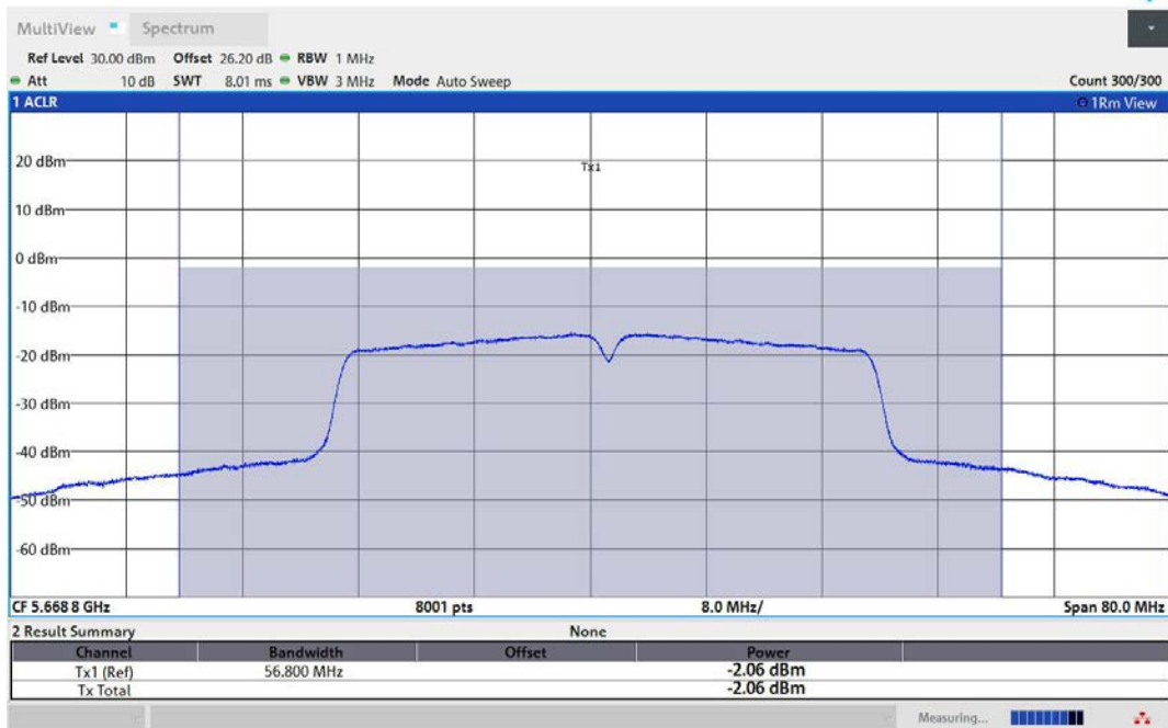
11AC40MIMO-Ant2-5670-TPC_L-PASS
