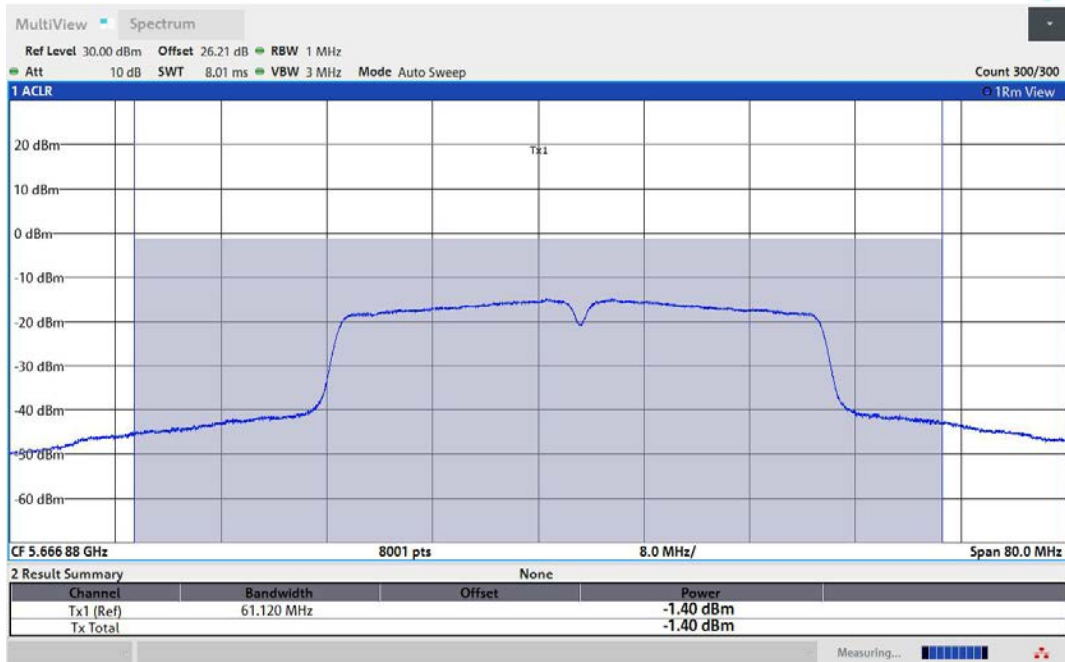
11AC40MIMO-Ant3-5670-TPC_L-PASS
