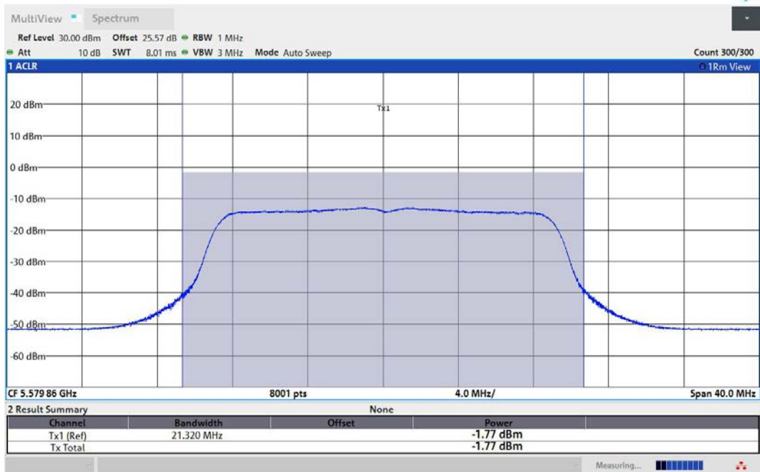
11AC20MIMO-Ant1-5580-TPC_L-PASS
