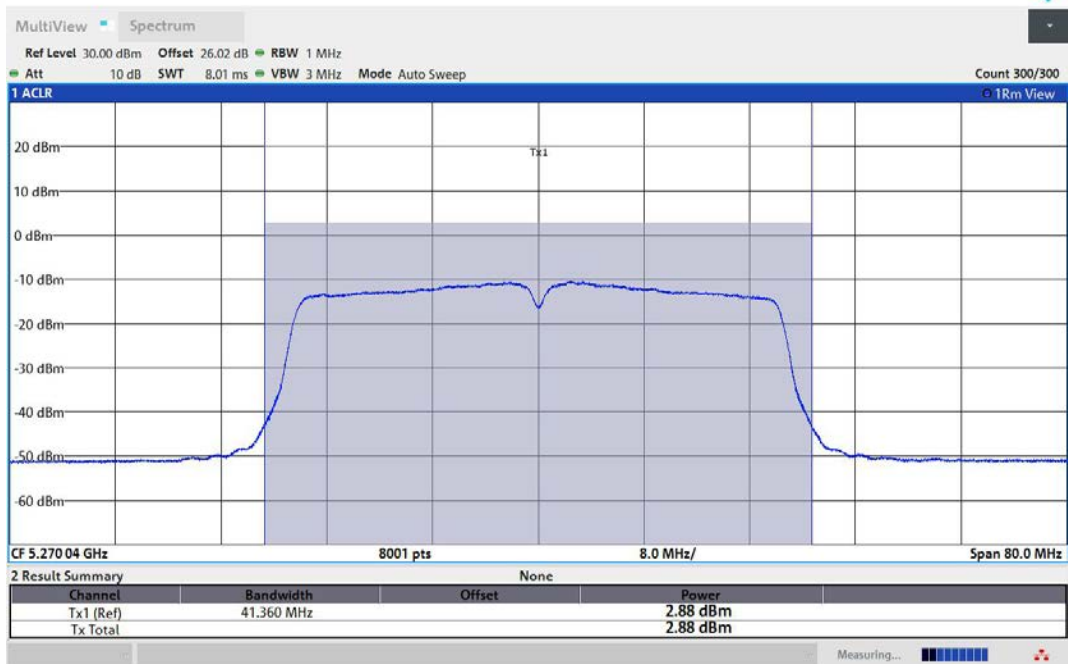
11AC40MIMO-Ant1-5270-TPC_H-PASS
