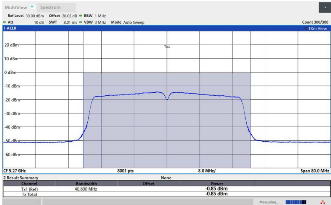
11AC40MIMO-Ant3-5270-TPC_L-PASS
