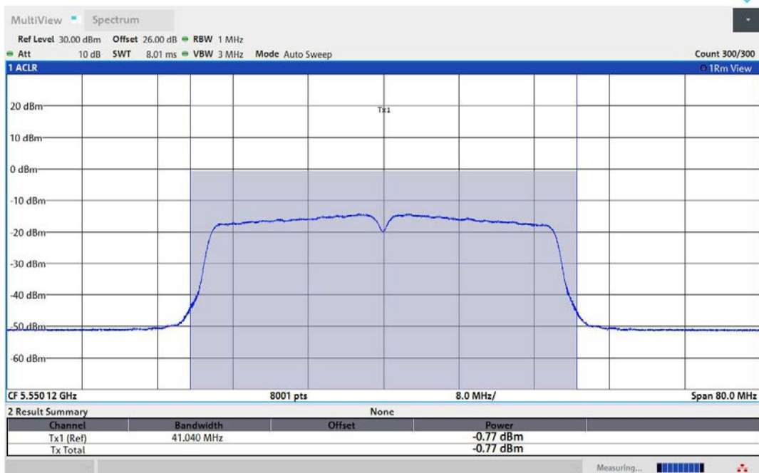
11AC40MIMO-Ant2-5550-TPC_L-PASS
