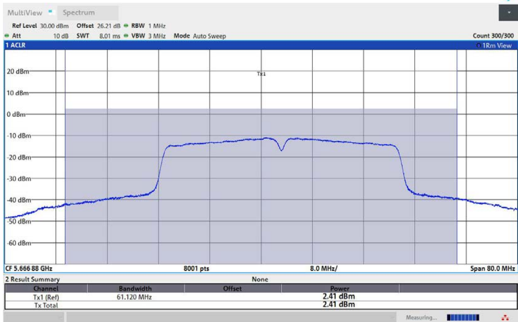
11AC40MIMO-Ant3-5670-TPC_H-PASS
