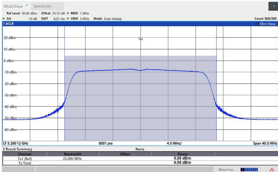
11AX20MIMO-Ant3-5260-TPC_H-PASS
