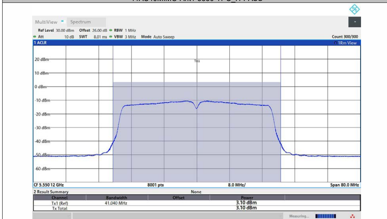
11AC40MIMO-Ant2-5550-TPC_H-PASS
