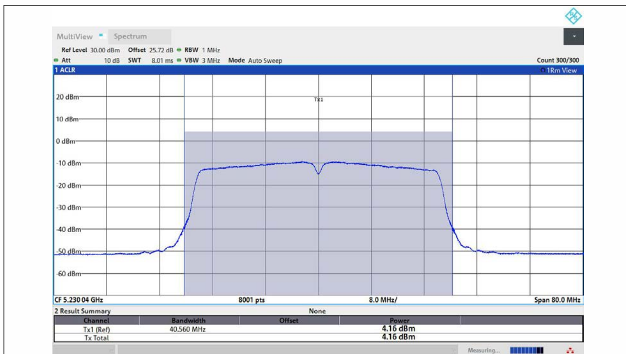
11AC40MIMO-Ant2-5230-PASS
