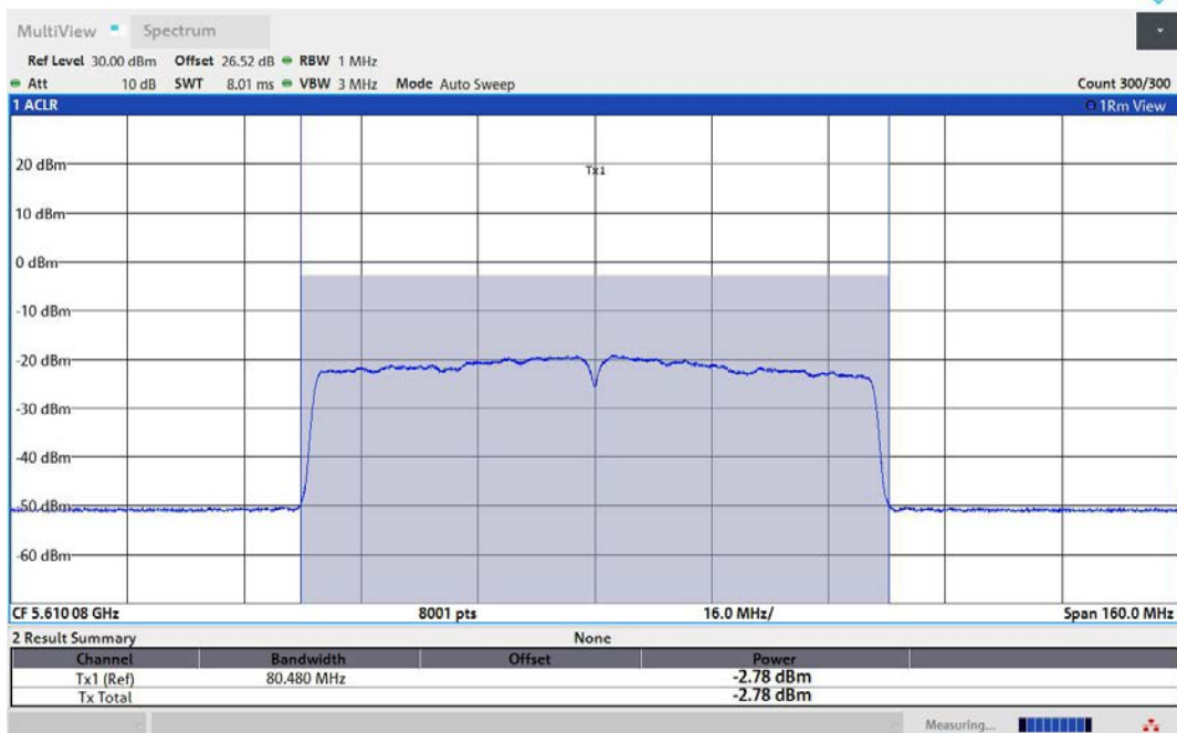
11AC80MIMO-Ant1-5610-TPC_L-PASS
