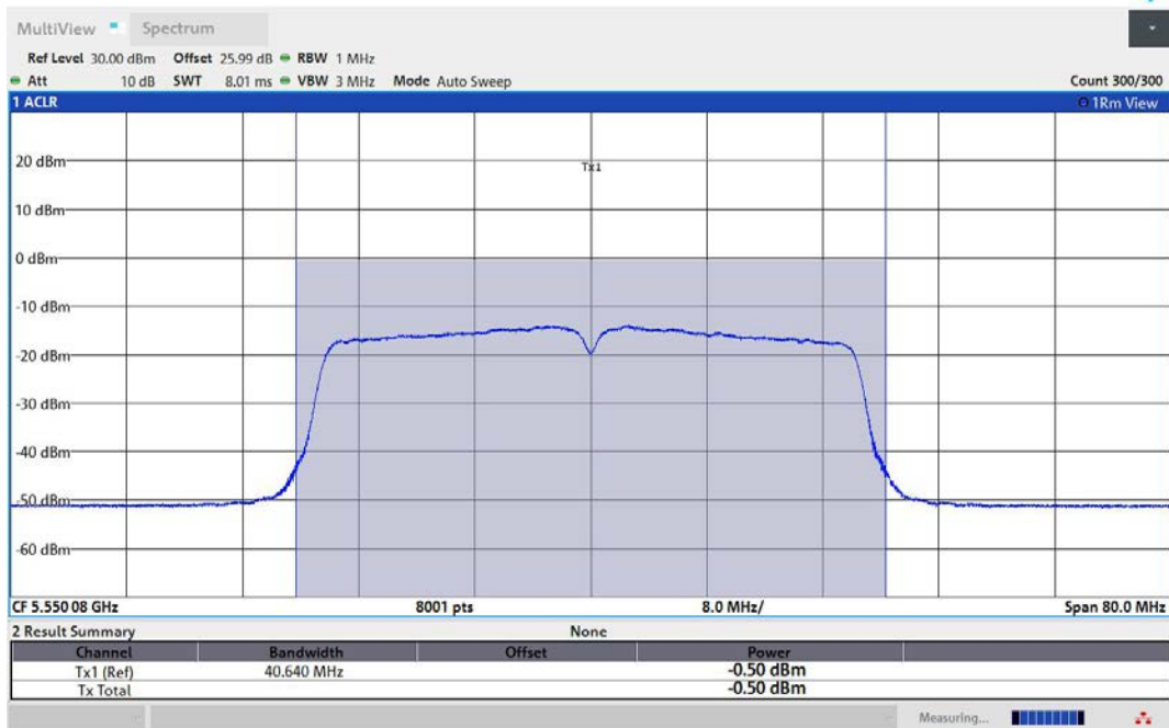
11AC40MIMO-Ant3-5550-TPC_L-PASS
