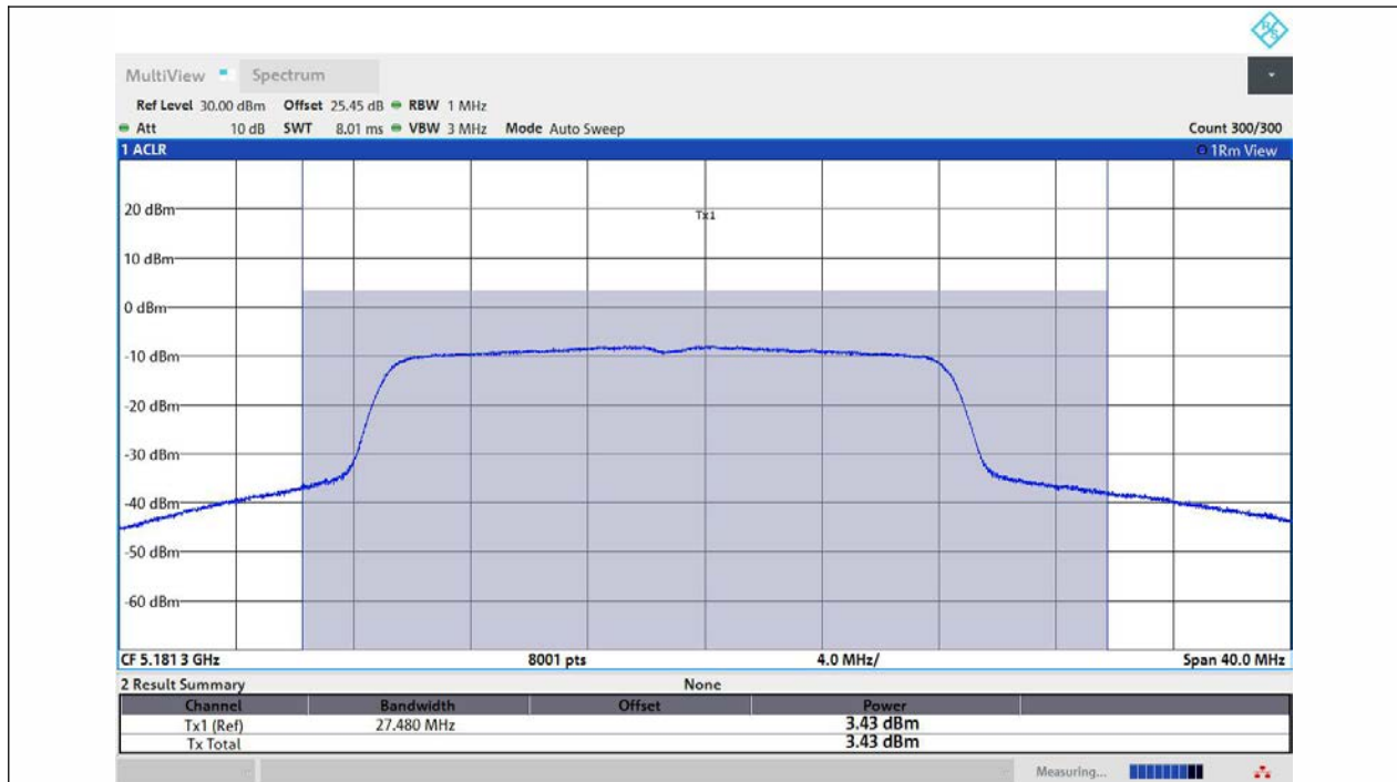
11AX20MIMO-Ant1-5180-PASS
