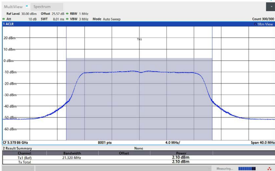
11AC20MIMO-Ant1-5580-TPC_H-PASS
