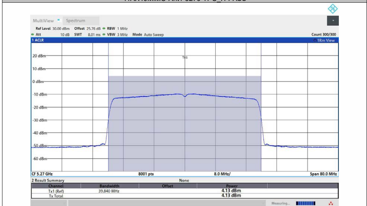
11AX40MIMO-Ant2-5270-TPC_H-PASS
