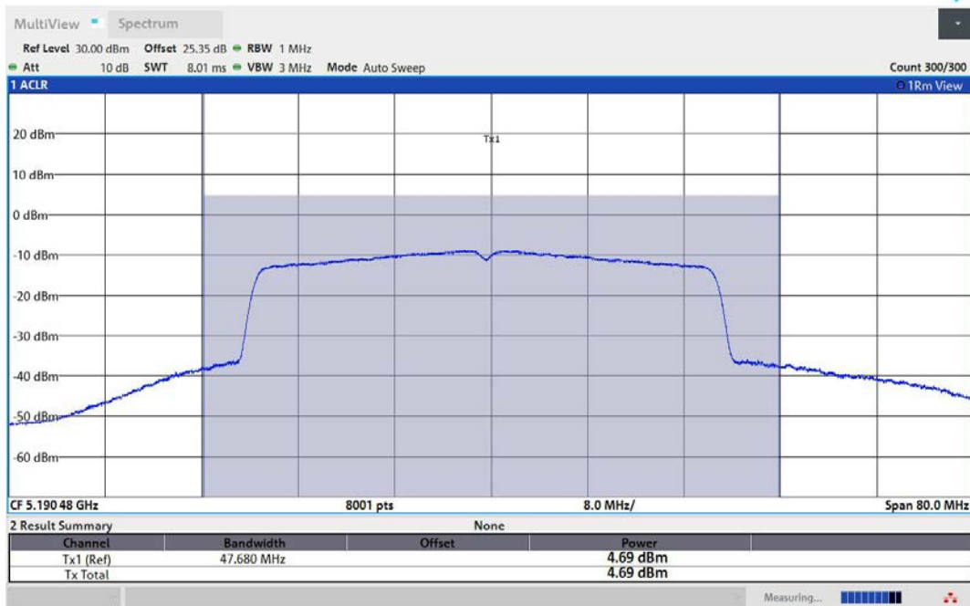
11AX40MIMO-Ant3-5190-PASS
