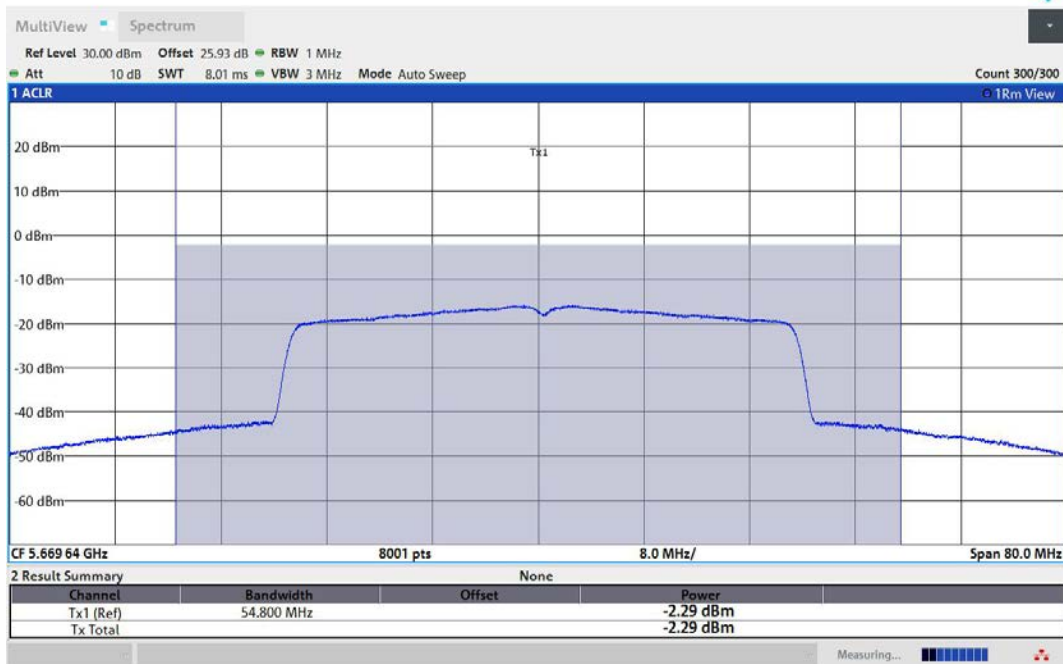
11AX40MIMO-Ant1-5670-TPC_L-PASS
