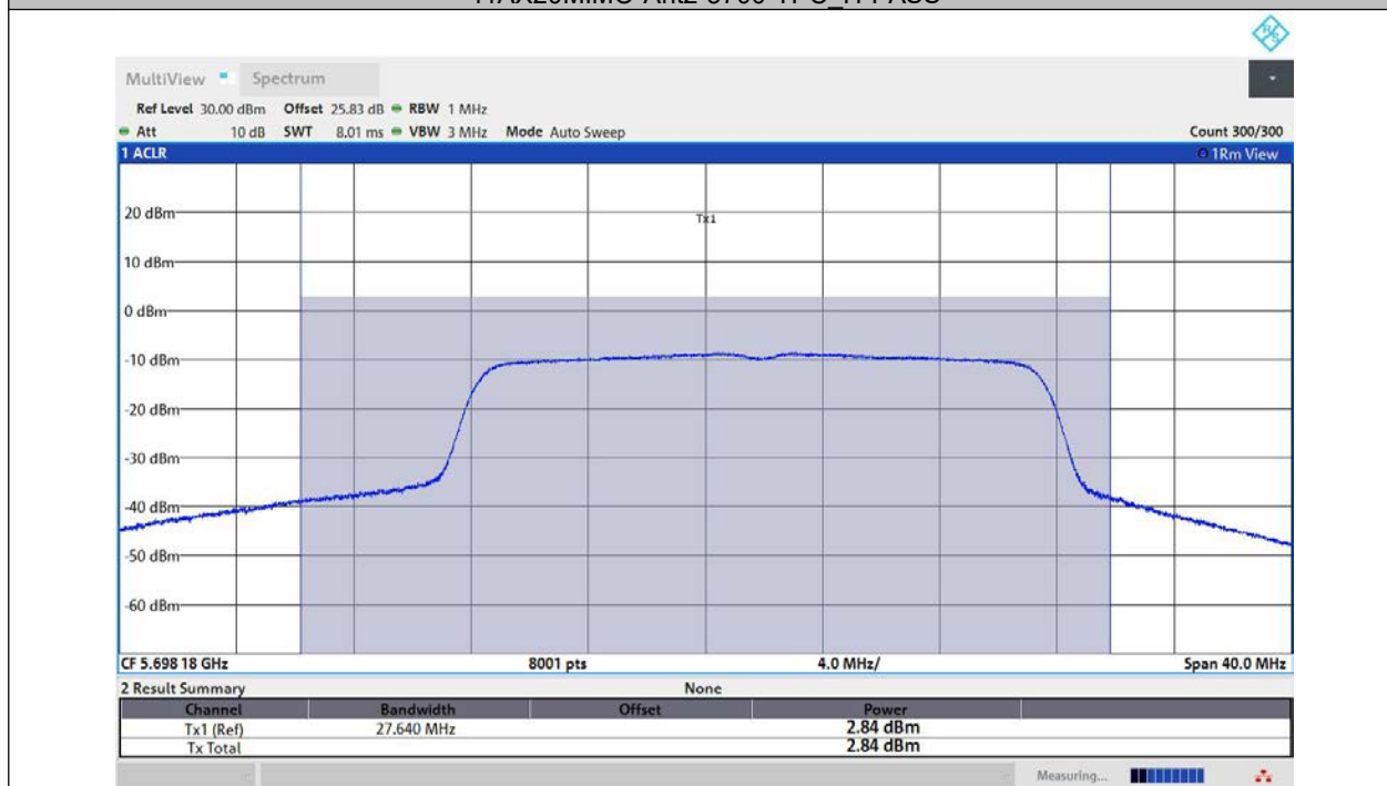
11AX20MIMO-Ant3-5700-TPC_H-PASS
