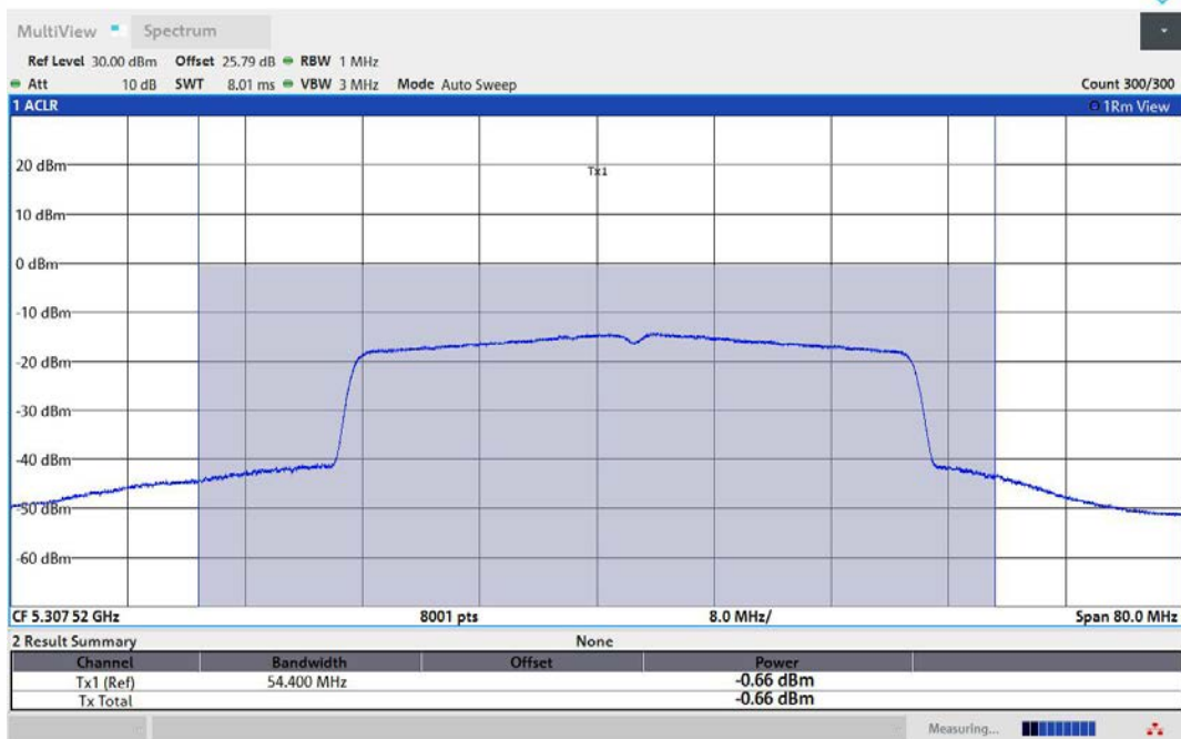
11AX40MIMO-Ant2-5310-TPC_L-PASS
