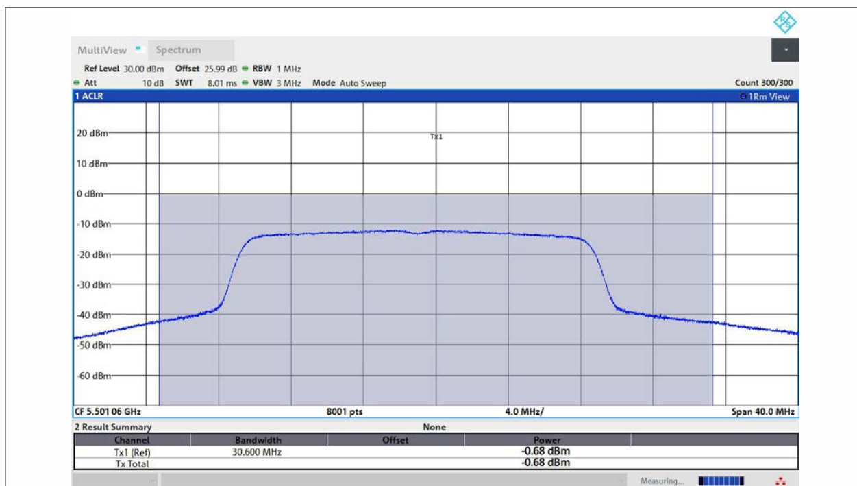
11AX20MIMO-Ant2-5500-TPC_L-PASS
