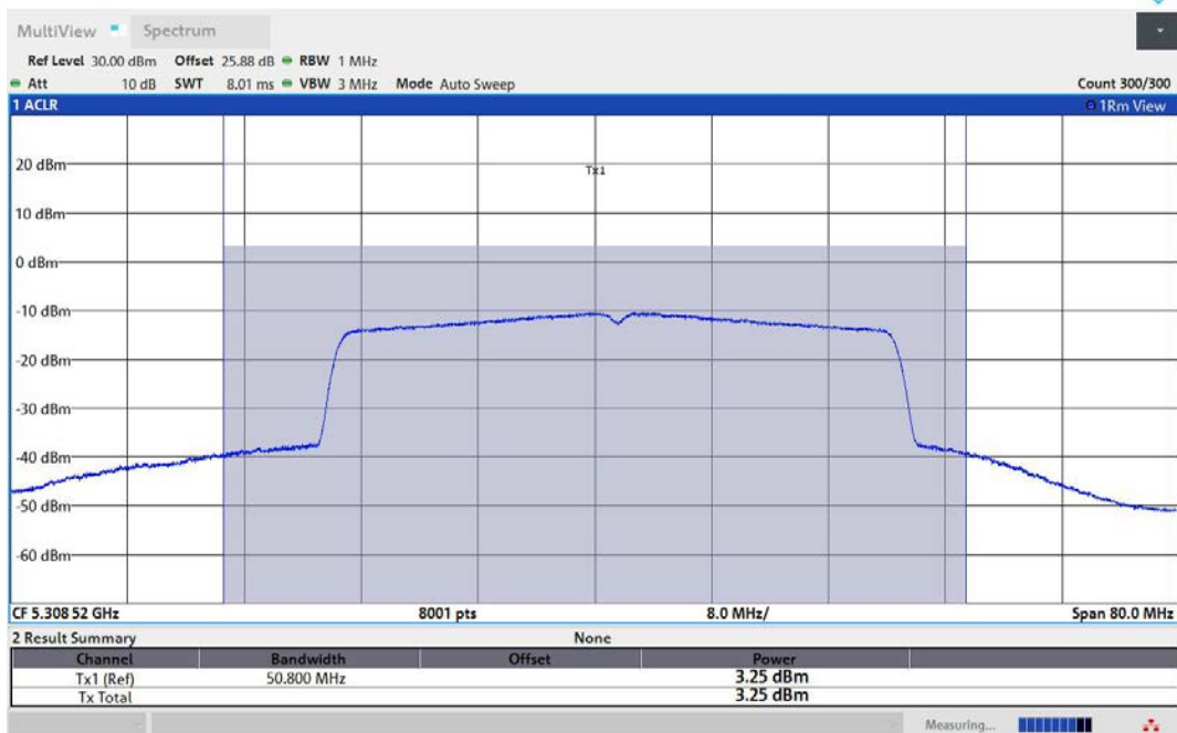
11AX40MIMO-Ant3-5310-TPC_H-PASS
