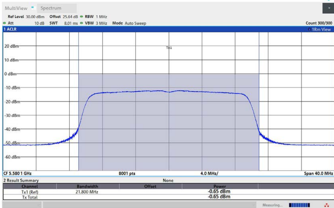
11AX20MIMO-Ant3-5580-TPC_L-PASS
