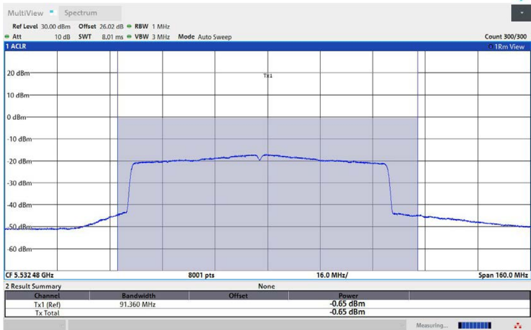
11AX80MIMO-Ant2-5530-TPC_L-PASS
