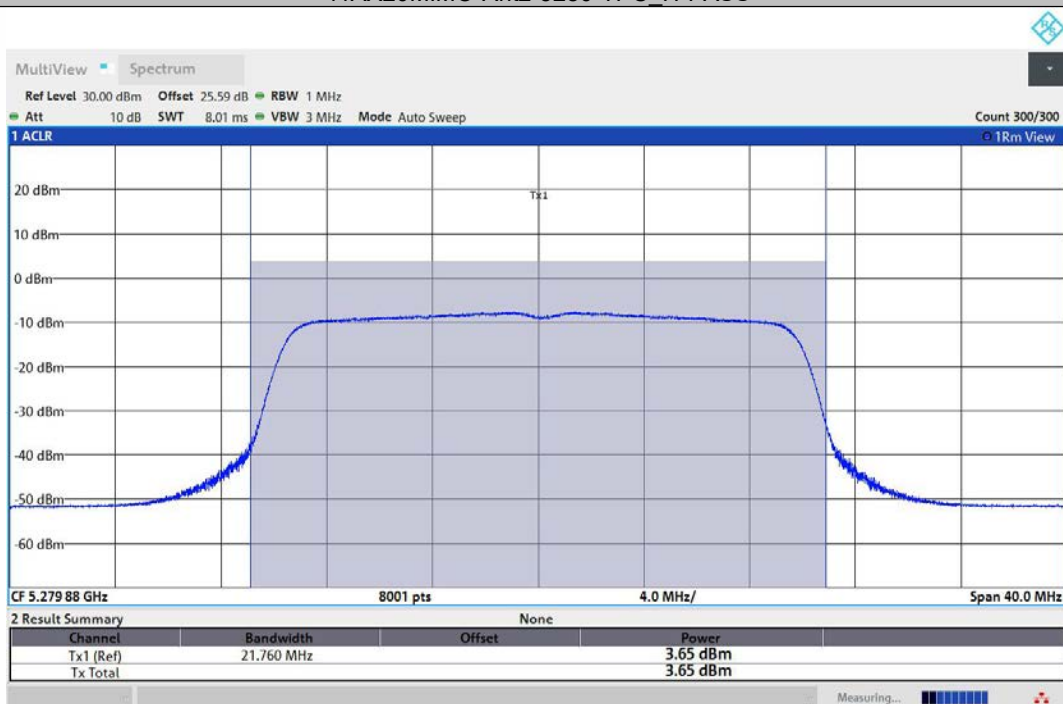
11AX20MIMO-Ant3-5280-TPC_H-PASS
