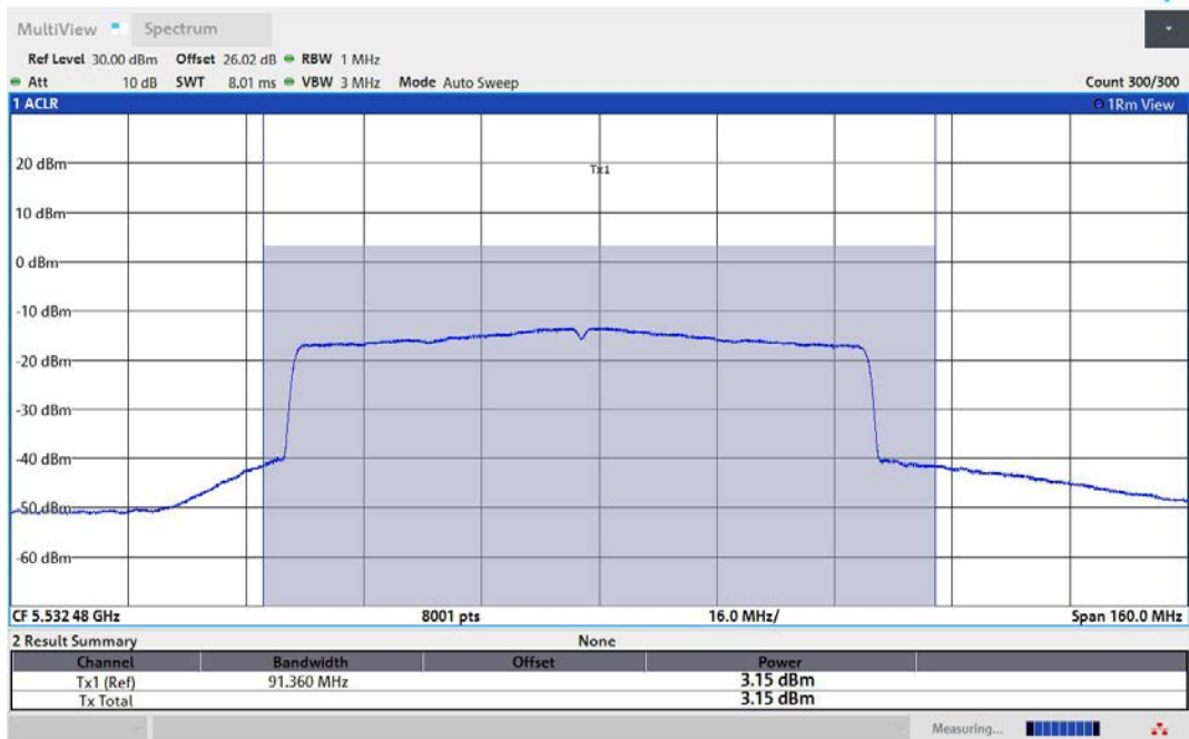
11AX80MIMO-Ant2-5530-TPC_H-PASS
