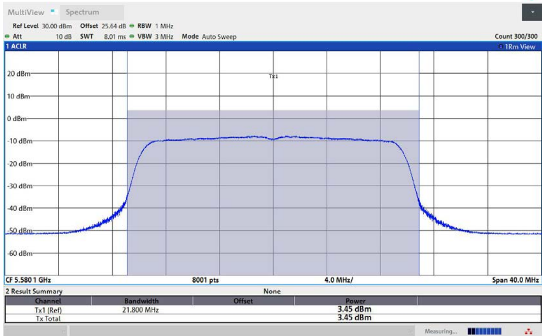
11AX20MIMO-Ant3-5580-TPC_H-PASS
