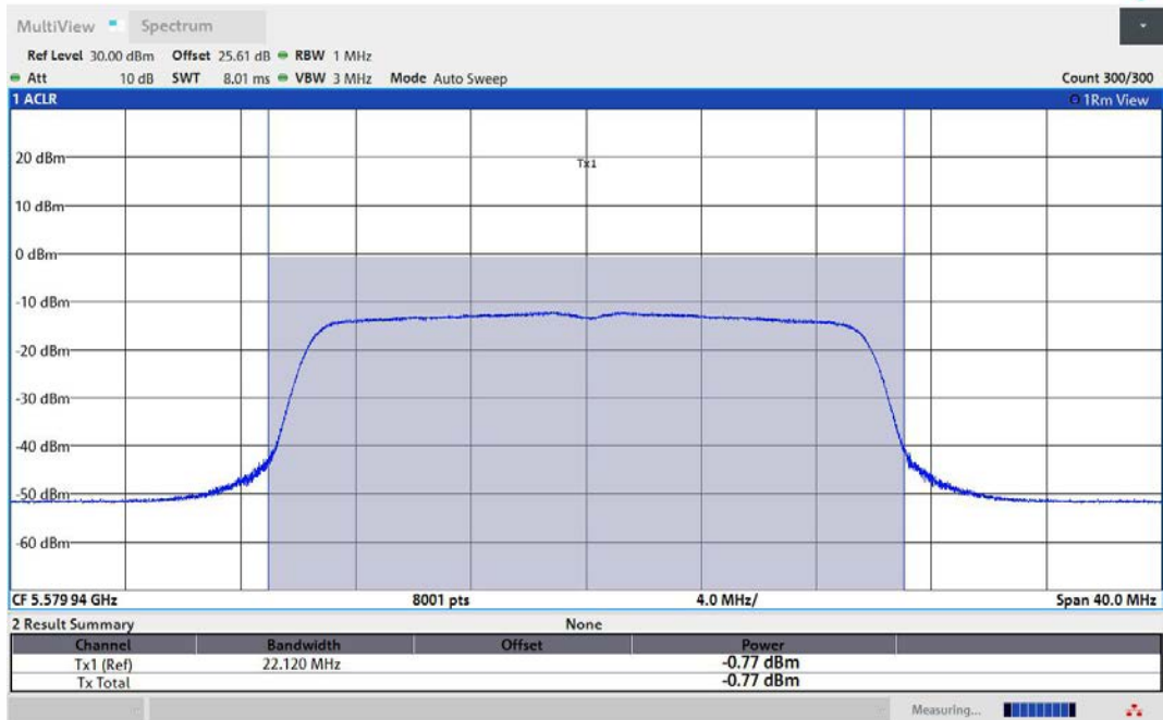
11AX20MIMO-Ant2-5580-TPC_L-PASS
