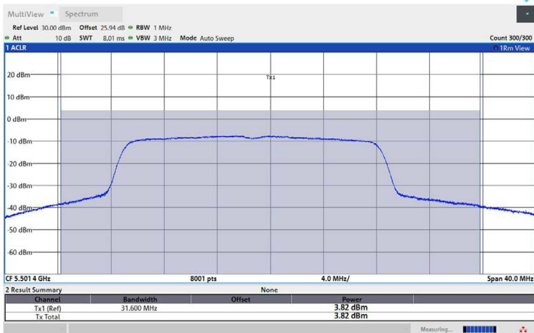
11AX20MIMO-Ant3-5500-TPC_H-PASS
