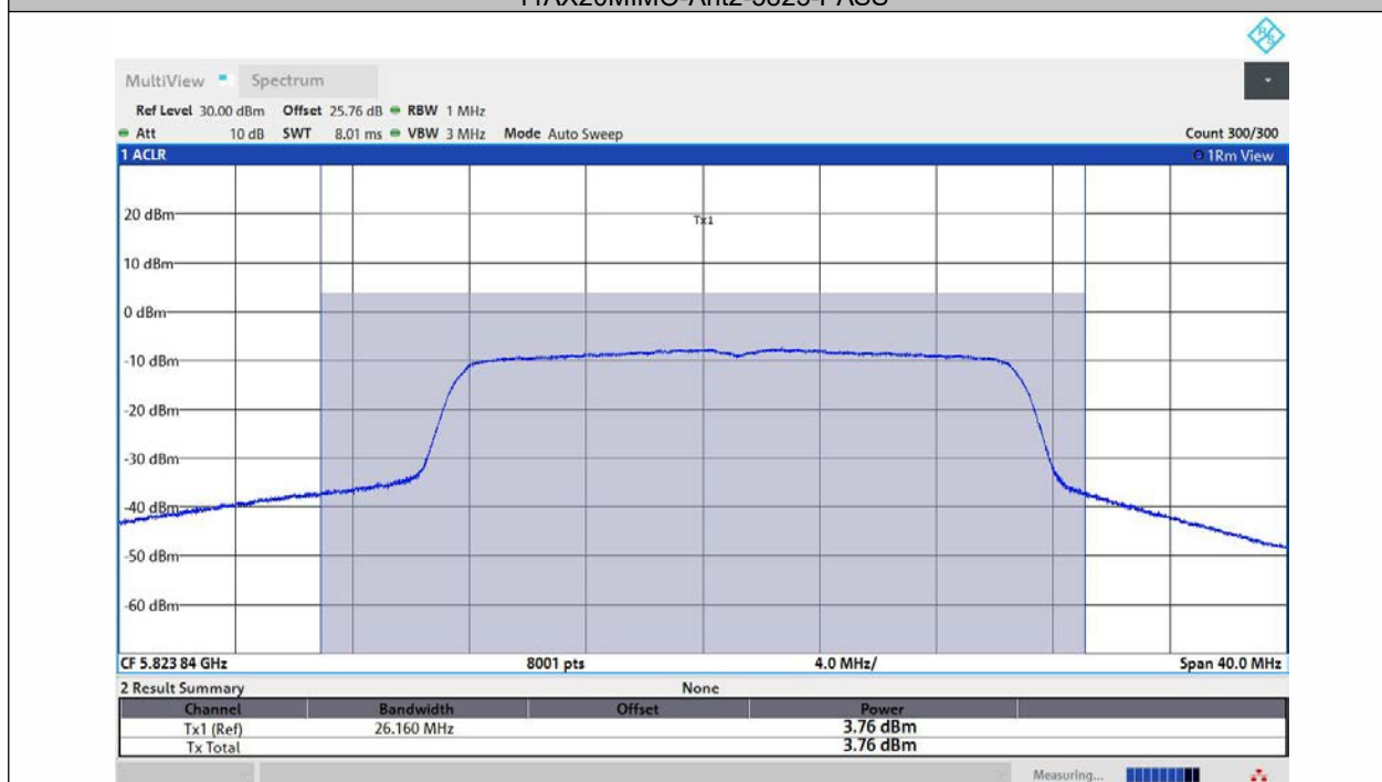
11AX20MIMO-Ant3-5825-PASS
