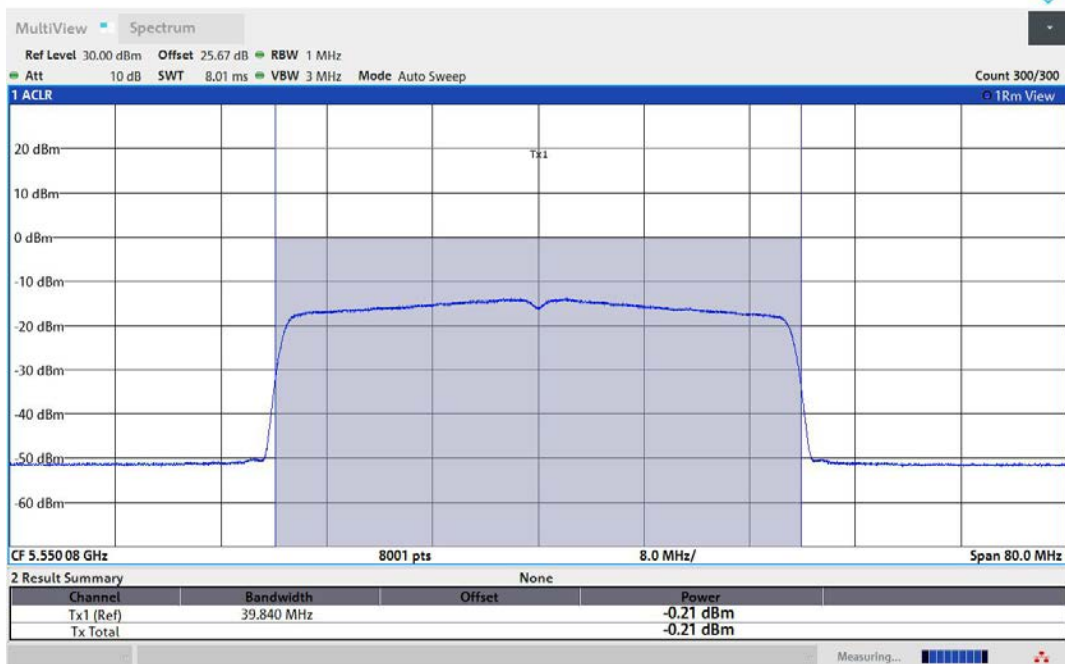
11AX40MIMO-Ant3-5550-TPC_L-PASS
