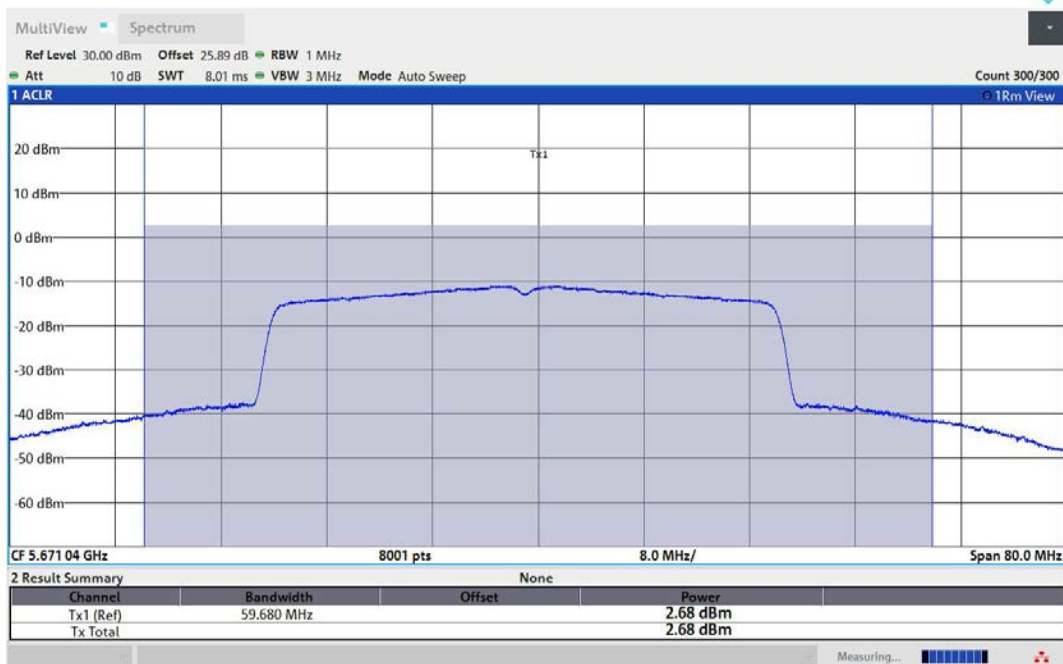
11AX40MIMO-Ant3-5670-TPC_H-PASS
