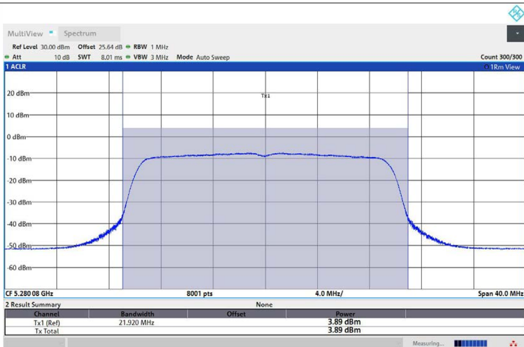
11AX20MIMO-Ant2-5280-TPC_H-PASS
