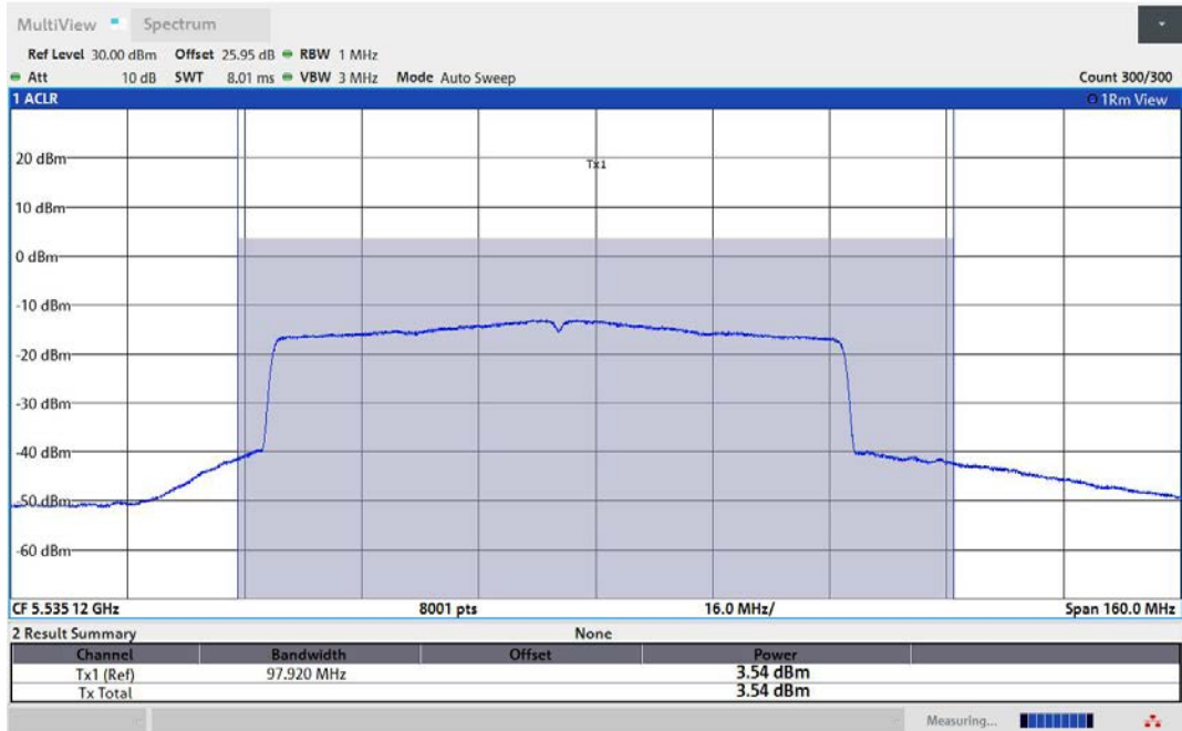
11AX80MIMO-Ant3-5530-TPC_H-PASS
