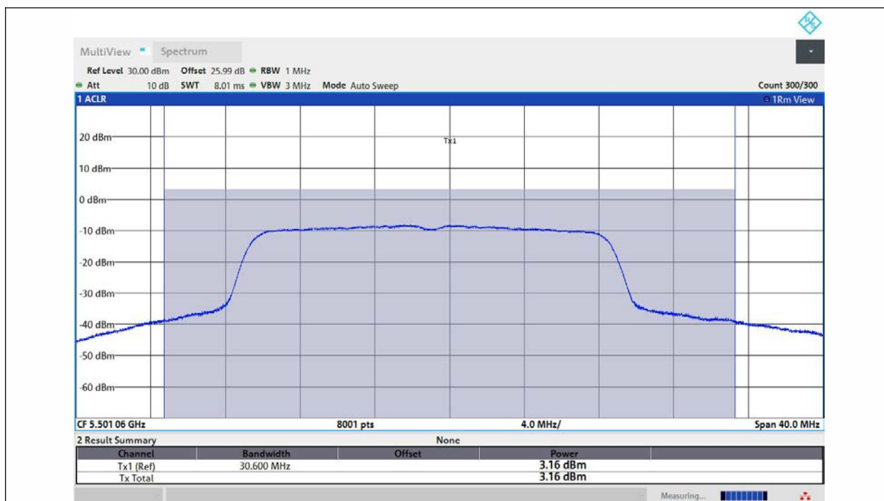
11AX20MIMO-Ant2-5500-TPC_H-PASS
