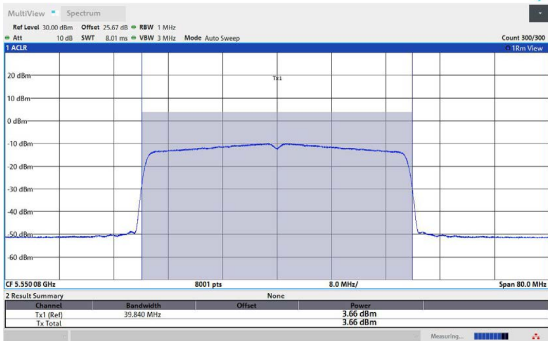
11AX40MIMO-Ant3-5550-TPC_H-PASS
