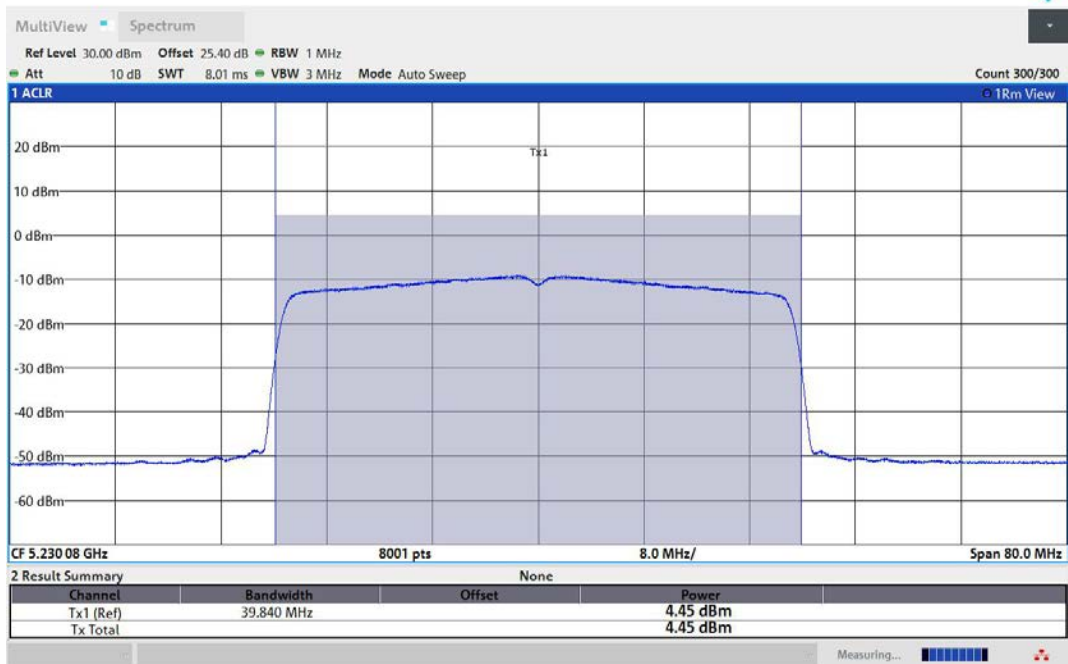
11AX40MIMO-Ant2-5230-PASS
