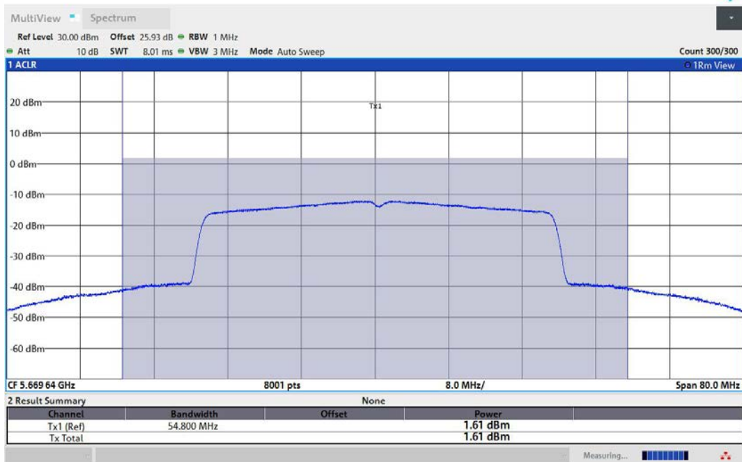
11AX40MIMO-Ant1-5670-TPC_H-PASS
