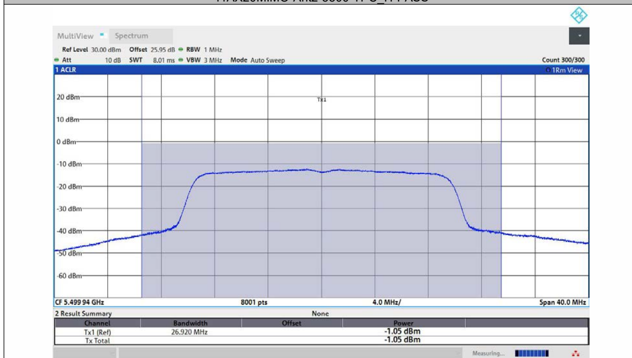
11AX20MIMO-Ant1-5500-TPC_L-PASS
