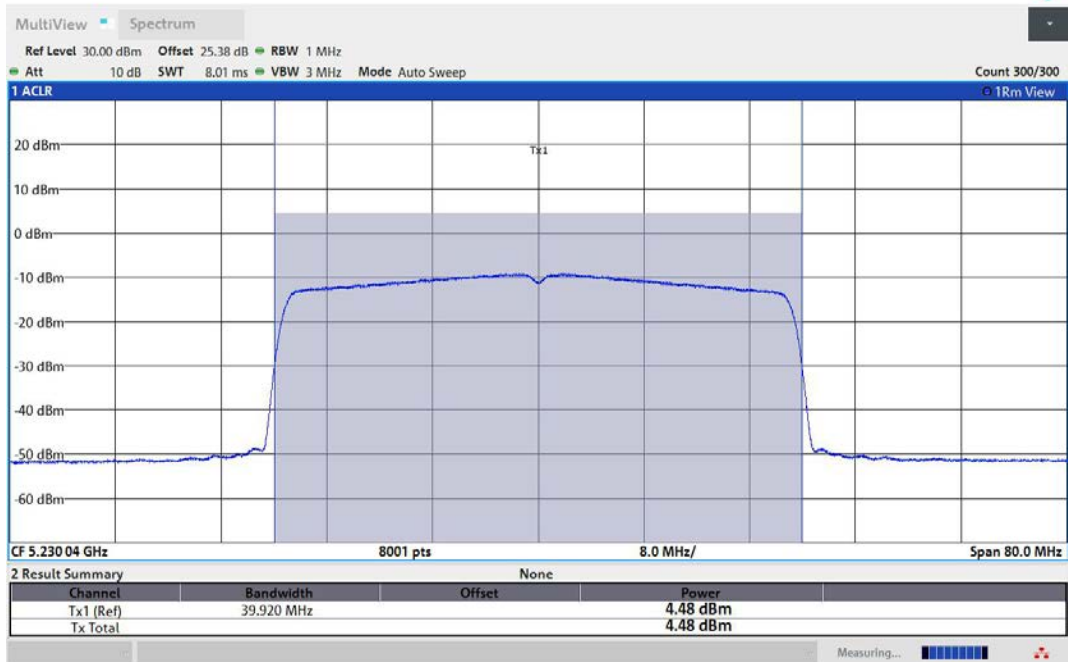
11AX40MIMO-Ant3-5230-PASS
