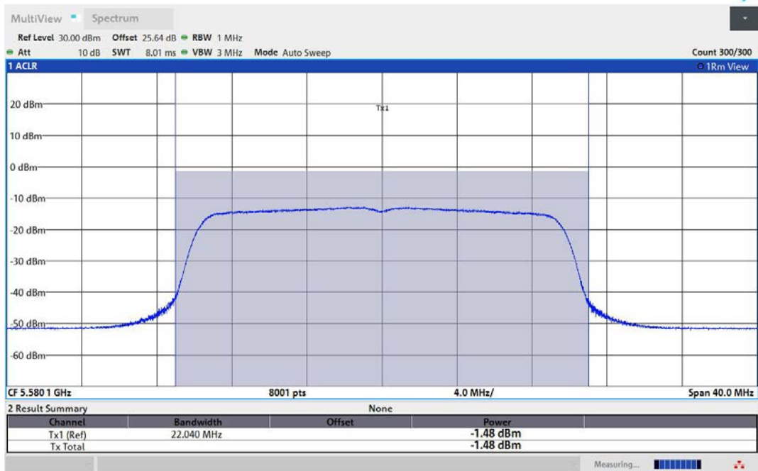
11AX20MIMO-Ant1-5580-TPC_L-PASS
