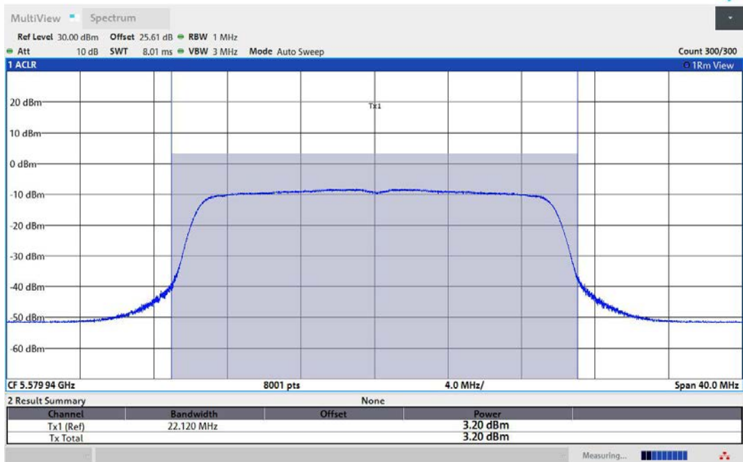
11AX20MIMO-Ant2-5580-TPC_H-PASS
