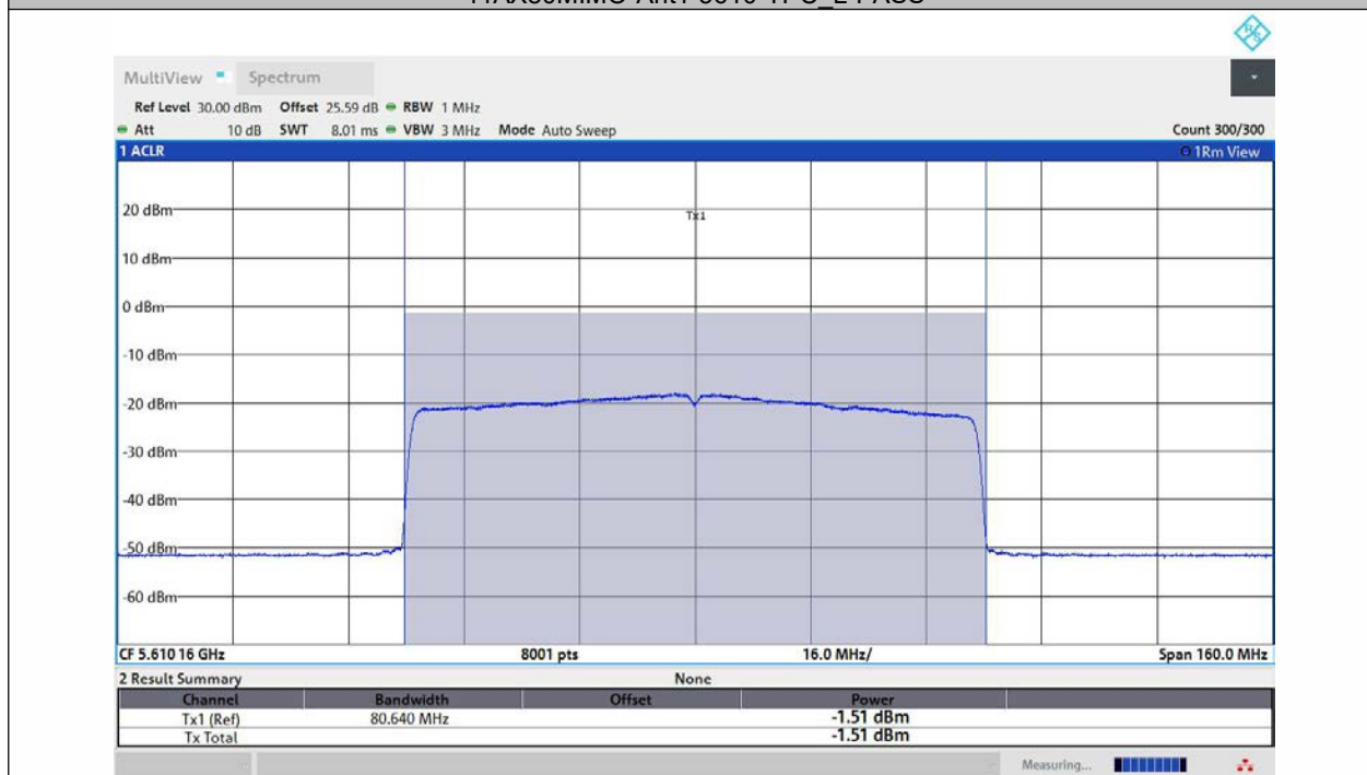
11AX80MIMO-Ant2-5610-TPC_L-PASS
