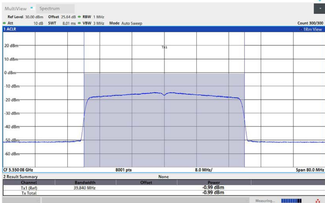
11AX40MIMO-Ant1-5550-TPC_L-PASS
