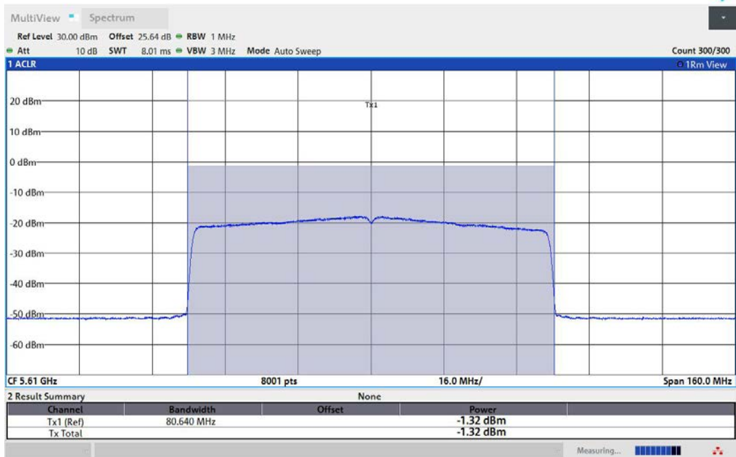
11AX80MIMO-Ant3-5610-TPC_L-PASS
