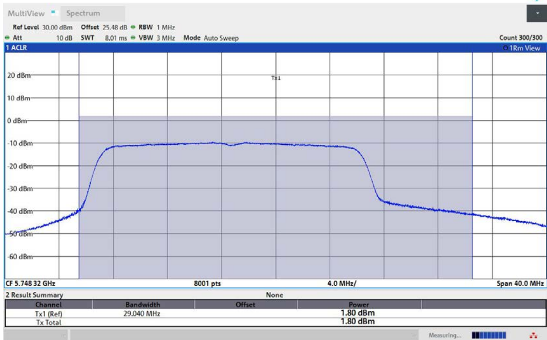
11AX20MIMO-Ant2-5745-PASS
