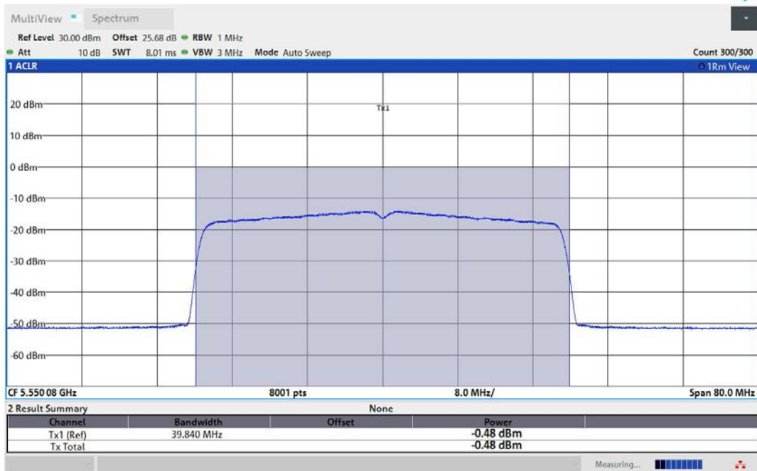
11AX40MIMO-Ant2-5550-TPC_L-PASS
