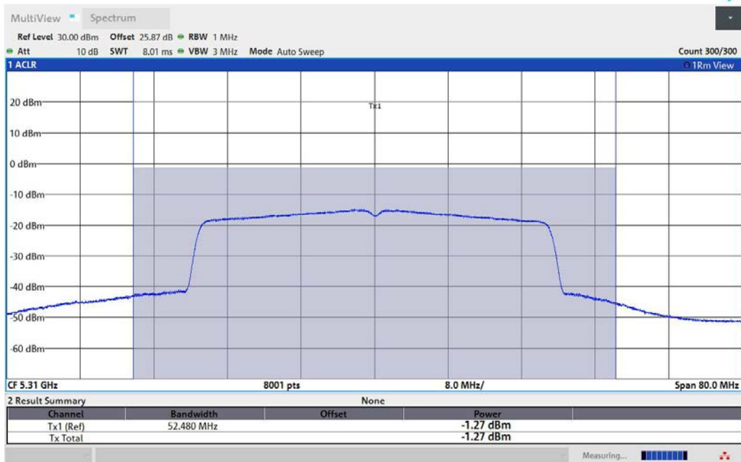
11AX40MIMO-Ant1-5310-TPC_L-PASS
