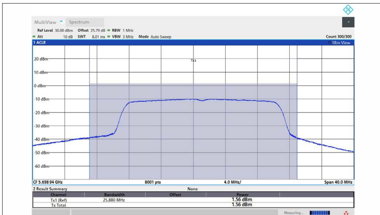
11AX20MIMO-Ant2-5700-TPC_H-PASS
