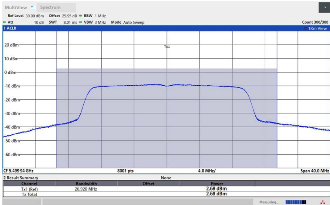
11AX20MIMO-Ant1-5500-TPC_H-PASS
