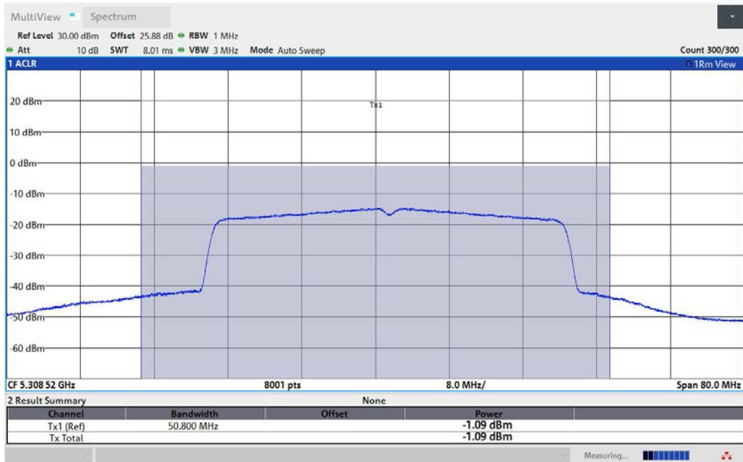
11AX40MIMO-Ant3-5310-TPC_L-PASS
