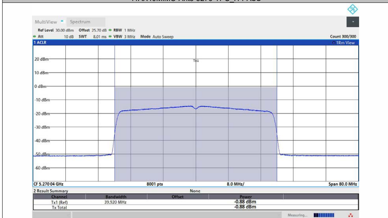
11AX40MIMO-Ant1-5270-TPC_L-PASS
