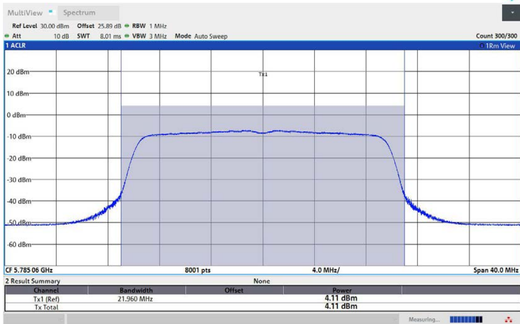
11AX20MIMO-Ant3-5785-PASS
