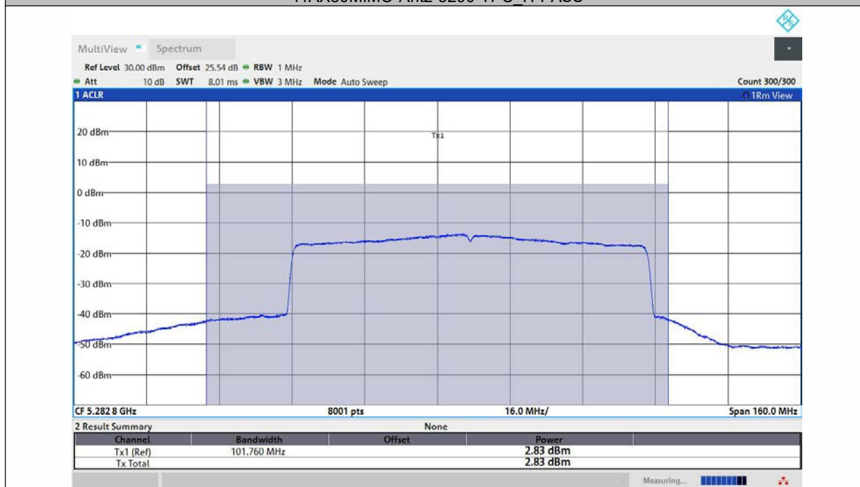
11AX80MIMO-Ant3-5290-TPC_H-PASS
