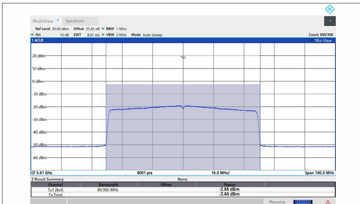
11AX80MIMO-Ant1-5610-TPC_L-PASS
