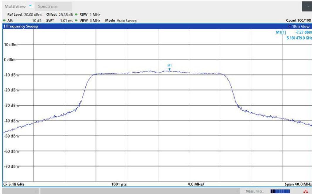
11AC20MIMO-Ant1-5180-PASS
