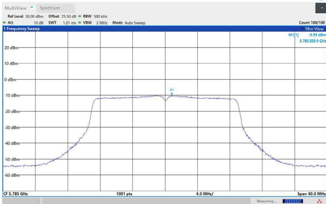
11N20MIMO-Ant3-5785-PASS
