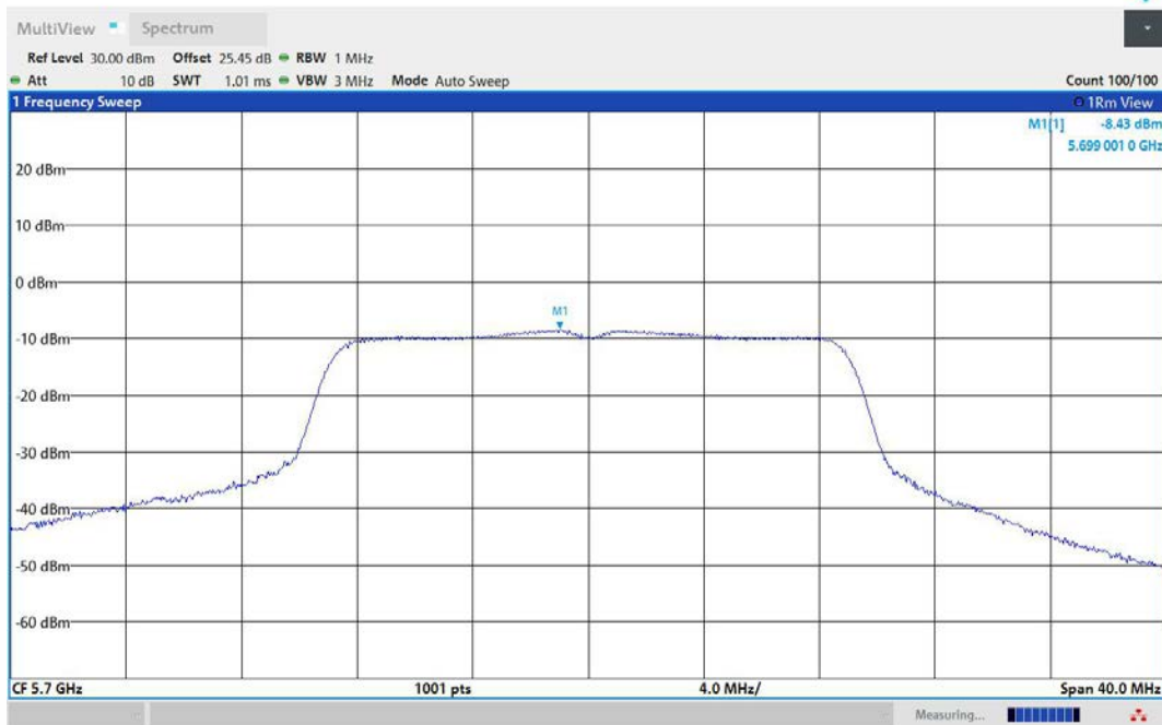
11N20MIMO-Ant3-5700-PASS
