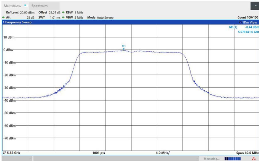
11A-Ant3-5580-PASS
