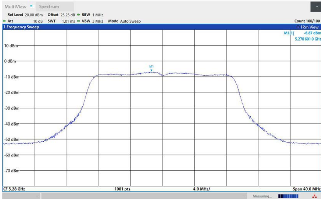
11N20MIMO-Ant2-5280-PASS
