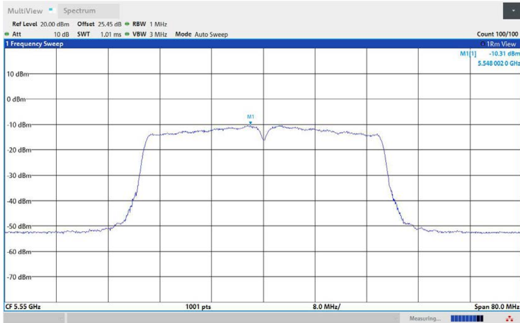
11N40MIMO-Ant1-5550-PASS
