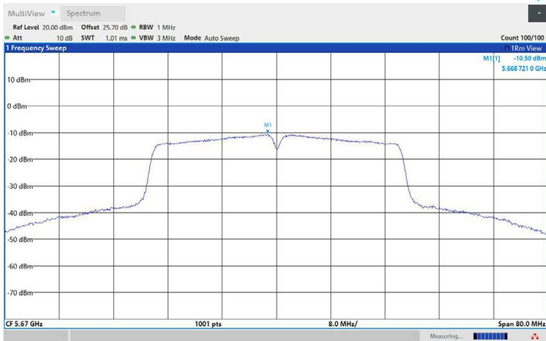
11N40MIMO-Ant3-5670-PASS
