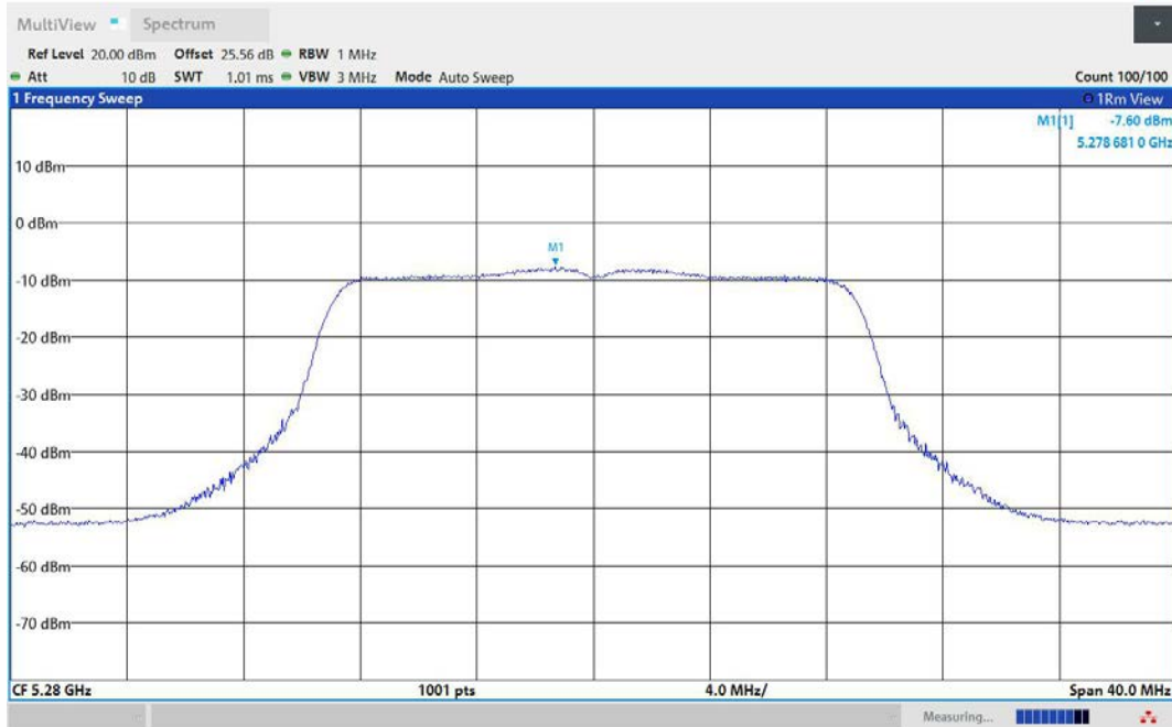
11AC20MIMO-Ant1-5280-PASS
