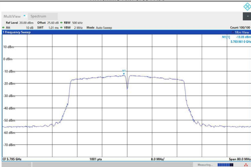
11N40MIMO-Ant2-5795-PASS
