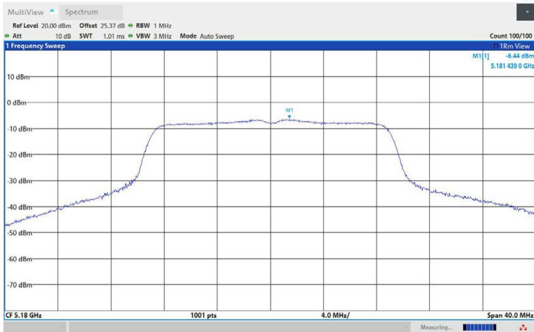
11AC20MIMO-Ant3-5180-PASS
