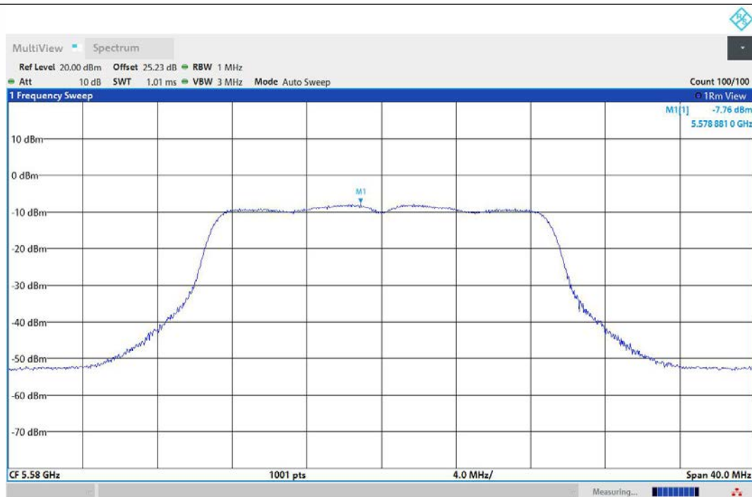
11N20MIMO-Ant2-5580-PASS
