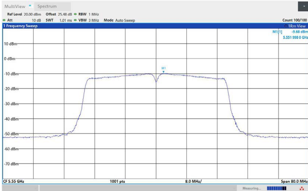
11N40MIMO-Ant3-5550-PASS
