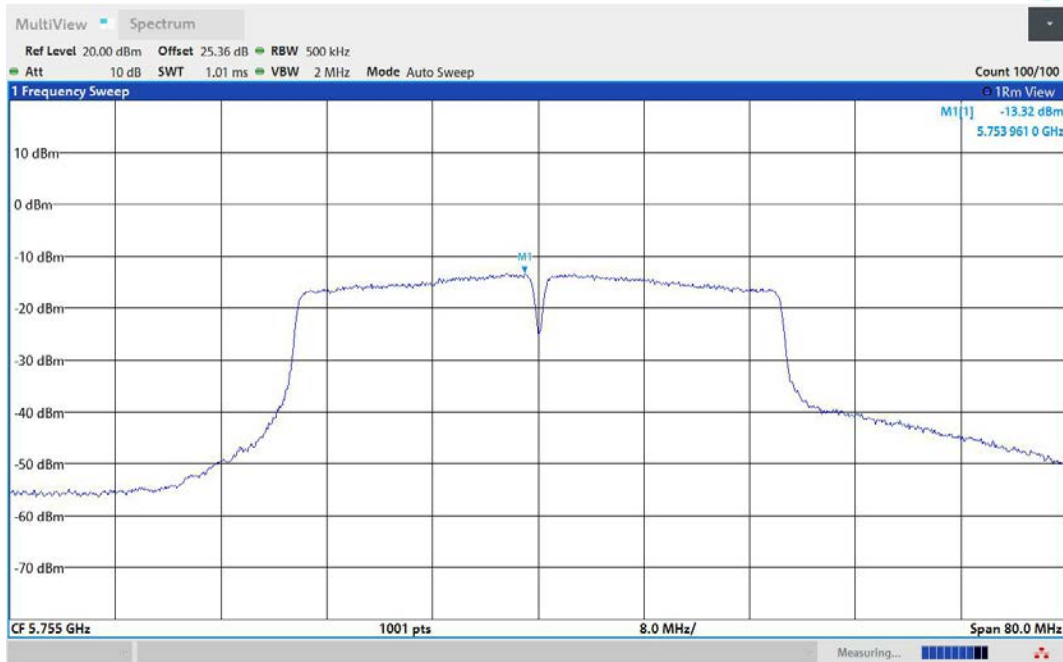
11N40MIMO-Ant3-5755-PASS
