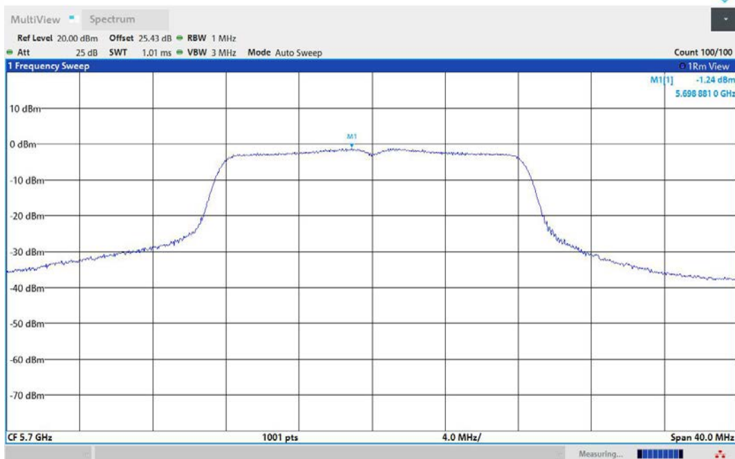
11A-Ant3-5700-PASS
