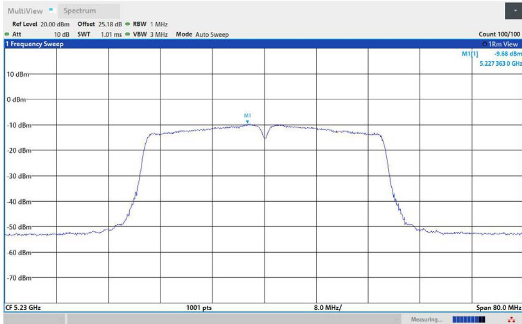
11N40MIMO-Ant1-5230-PASS
