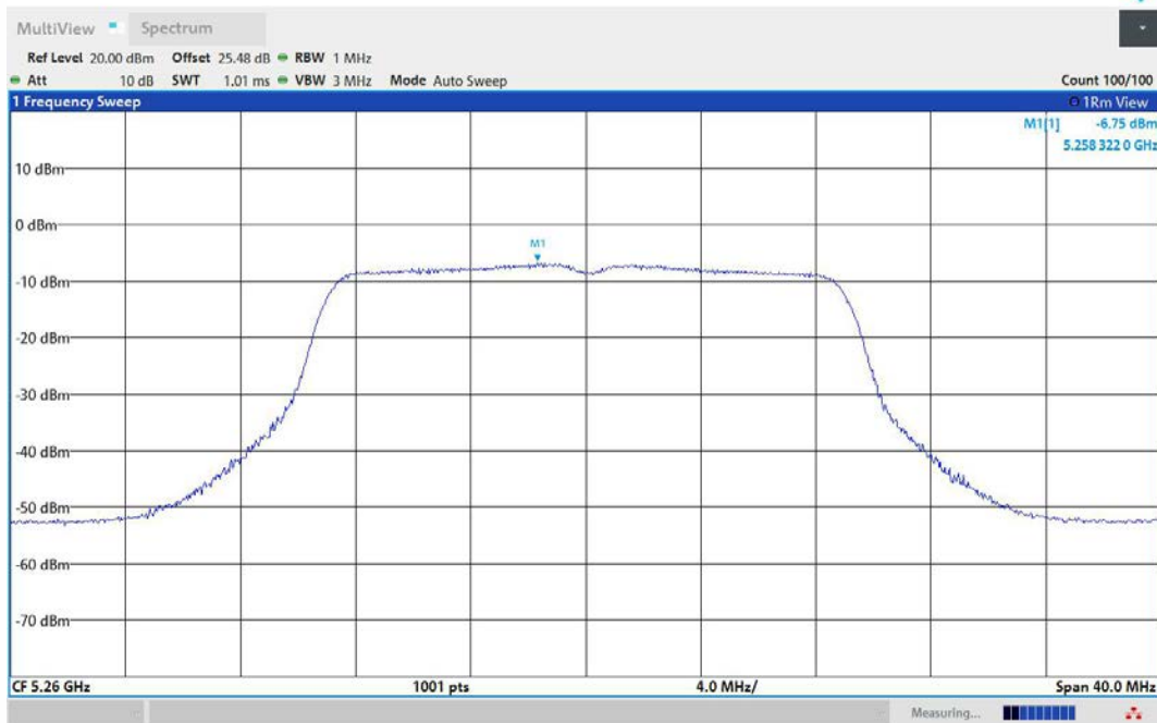
11AC20MIMO-Ant3-5260-PASS
