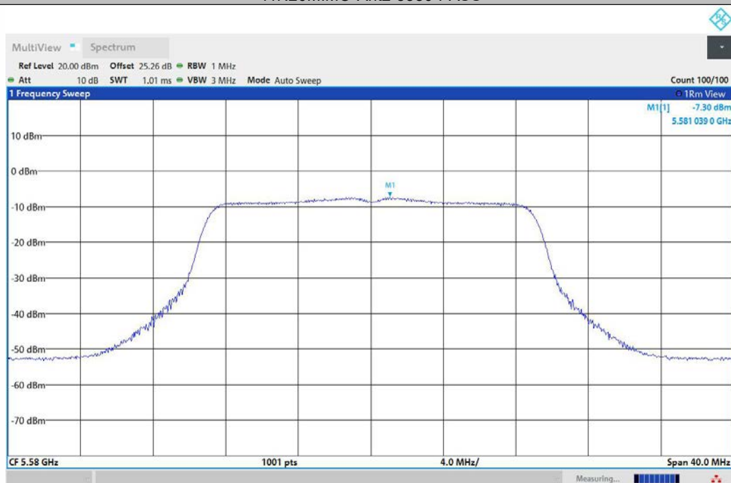
11N20MIMO-Ant3-5580-PASS
