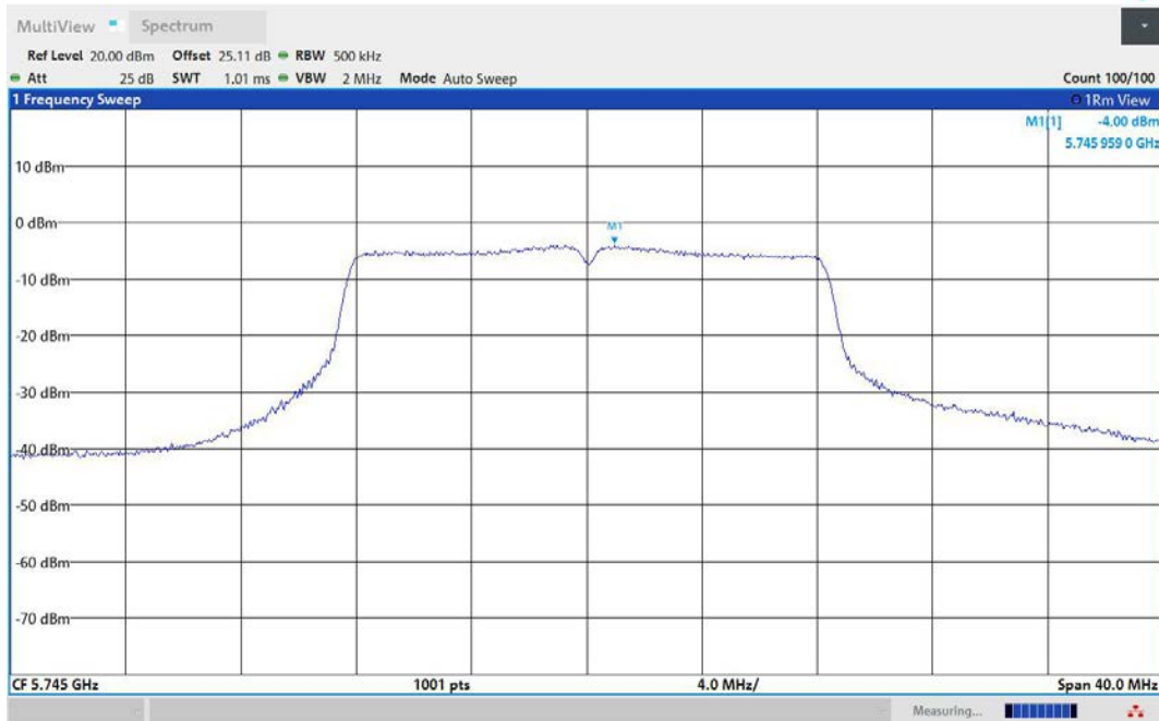
11A-Ant3-5745-PASS
