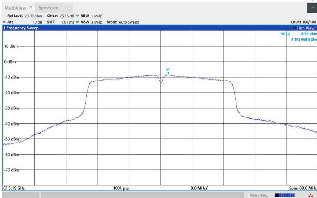
11N40MIMO-Ant3-5190-PASS
