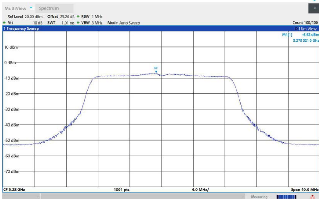
11N20MIMO-Ant3-5280-PASS
