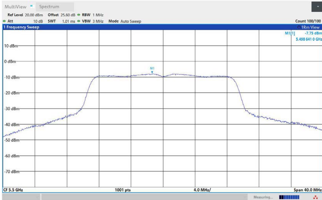
11N20MIMO-Ant2-5500-PASS
