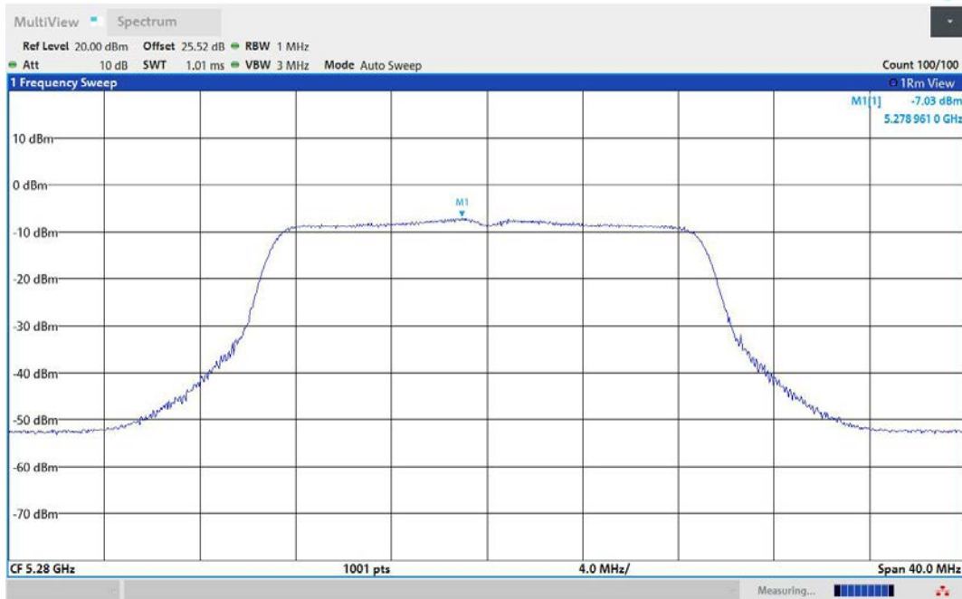
11AC20MIMO-Ant3-5280-PASS
