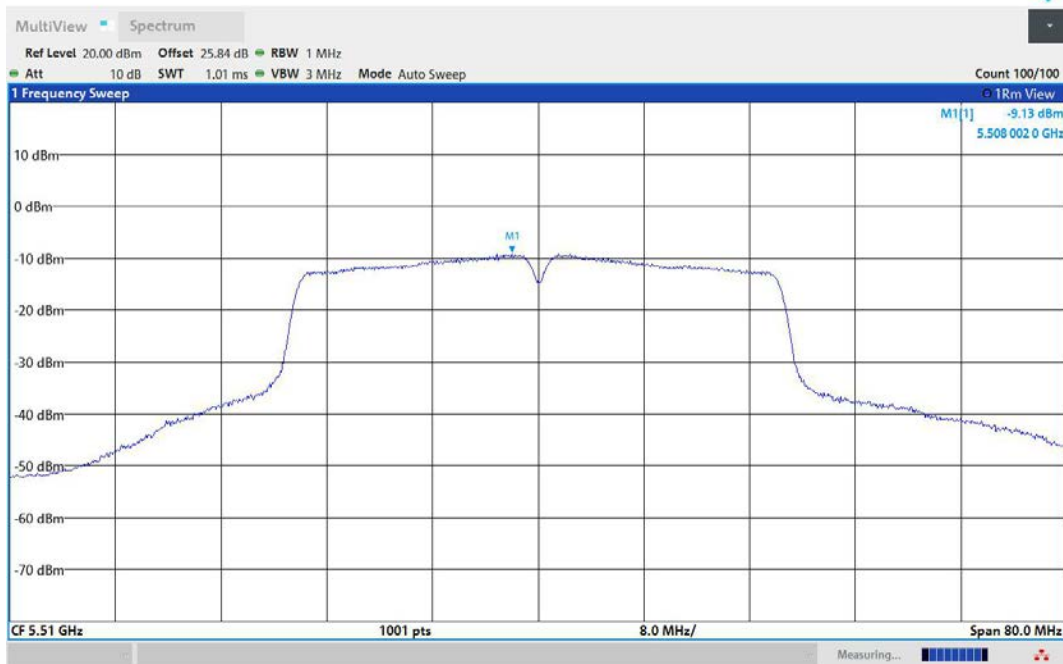
11N40MIMO-Ant3-5510-PASS
