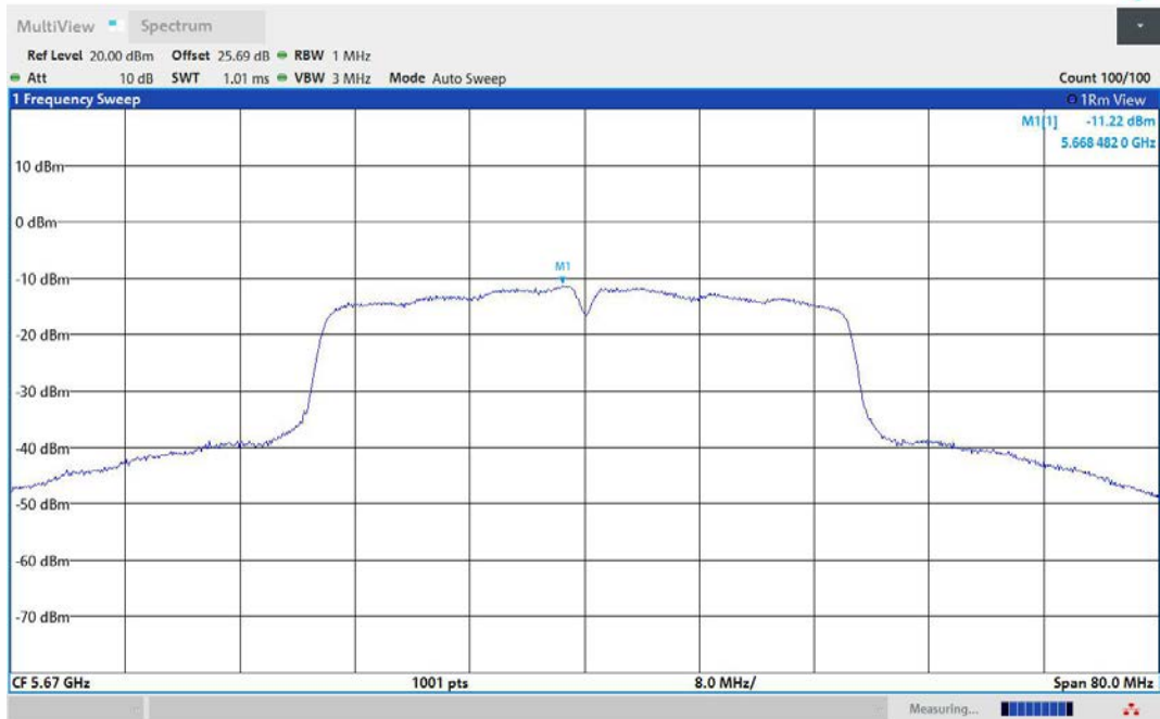
11N40MIMO-Ant2-5670-PASS
