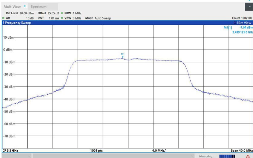
11N20MIMO-Ant3-5500-PASS
