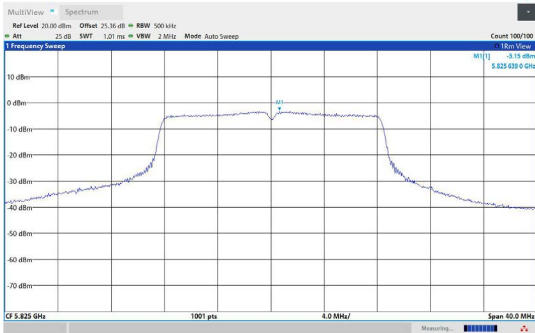
11A-Ant3-5825-PASS
