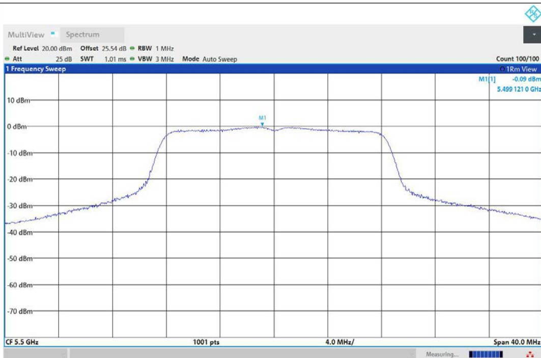
11A-Ant3-5500-PASS
