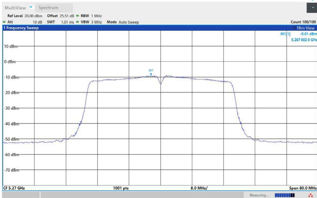
11N40MIMO-Ant3-5270-PASS
