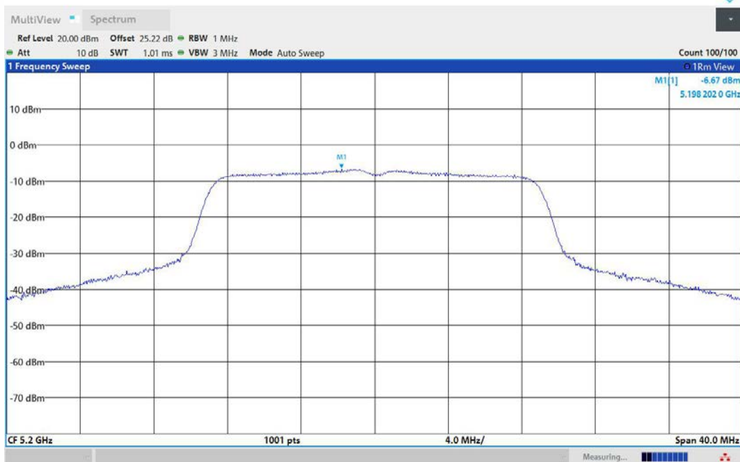
11AC20MIMO-Ant3-5200-PASS
