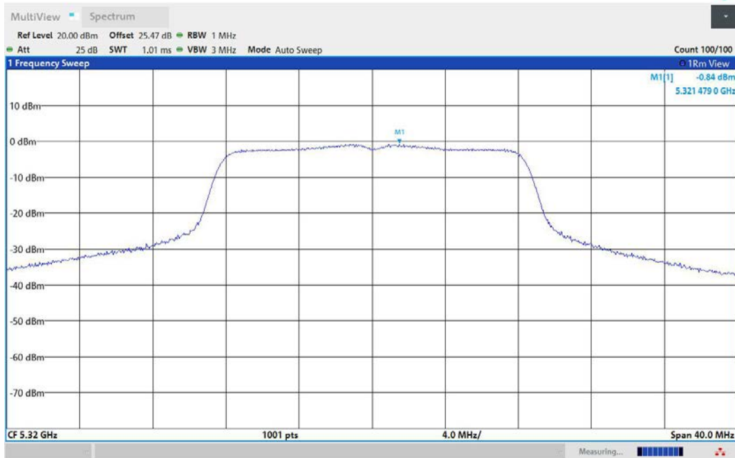
11A-Ant3-5320-PASS
