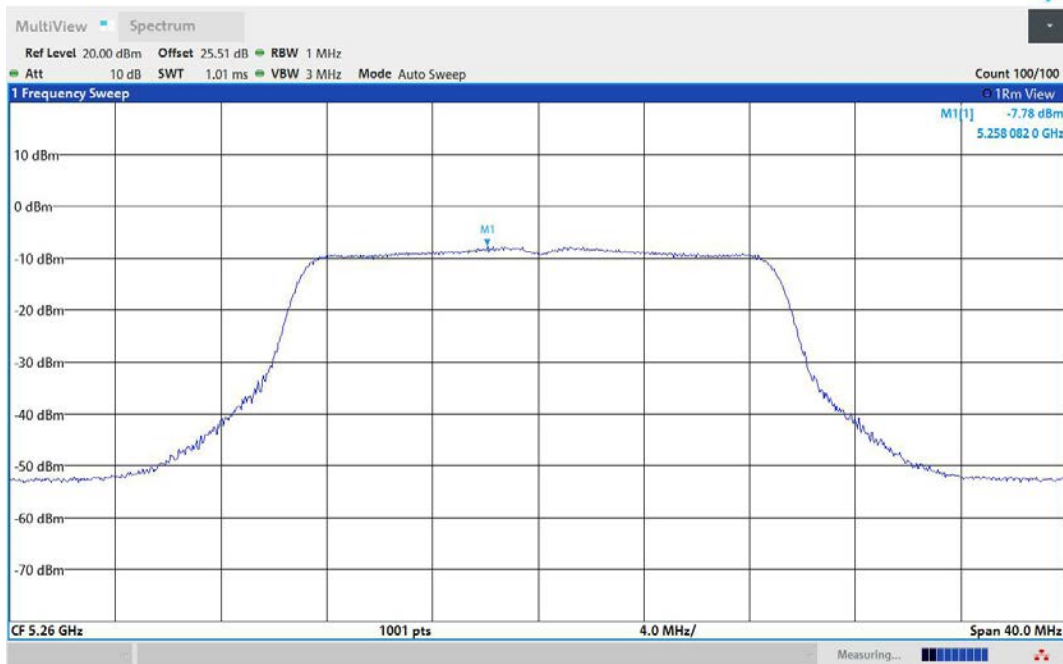
11AC20MIMO-Ant1-5260-PASS
