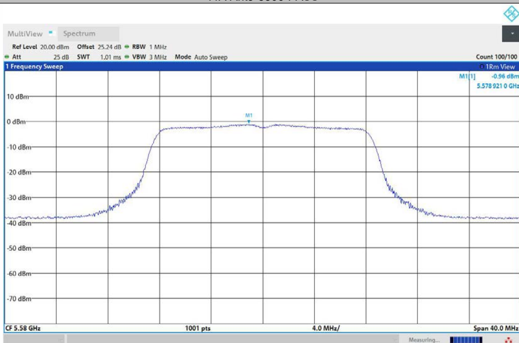
11A-Ant1-5580-PASS
