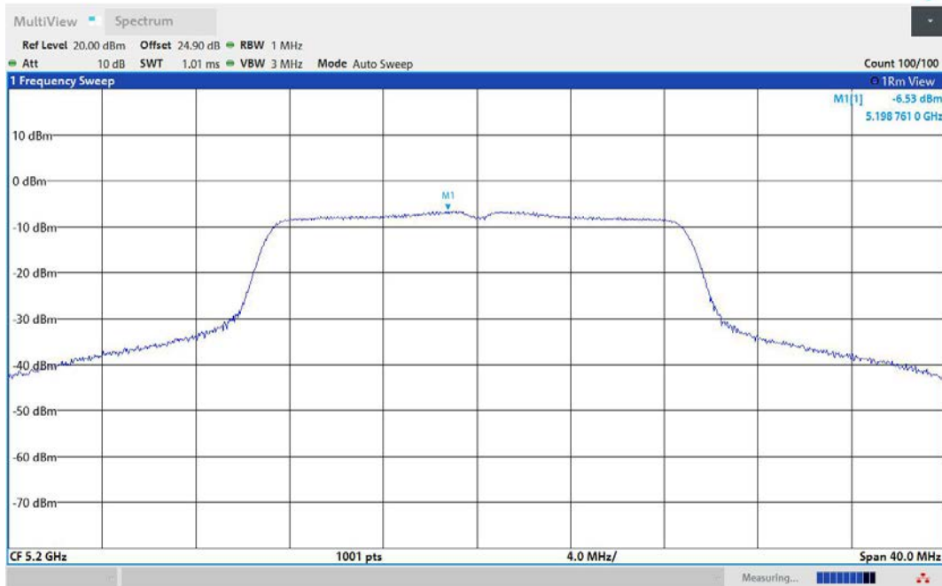
11N20MIMO-Ant3-5200-PASS
