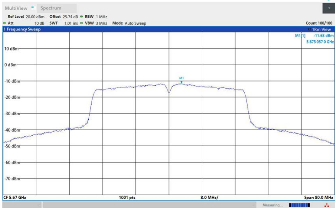
11N40MIMO-Ant1-5670-PASS
