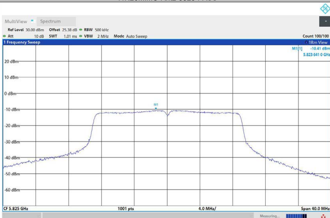
11N20MIMO-Ant3-5825-PASS
