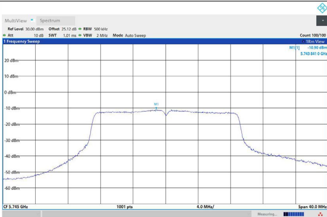
11N20MIMO-Ant3-5745-PASS
