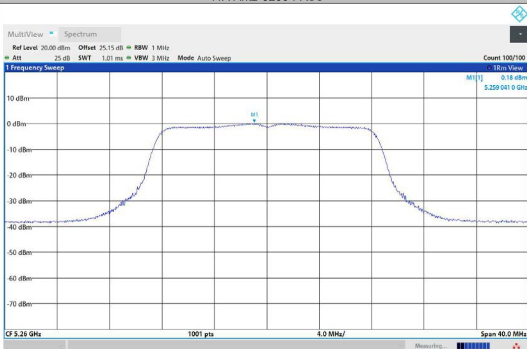
11A-Ant3-5260-PASS
