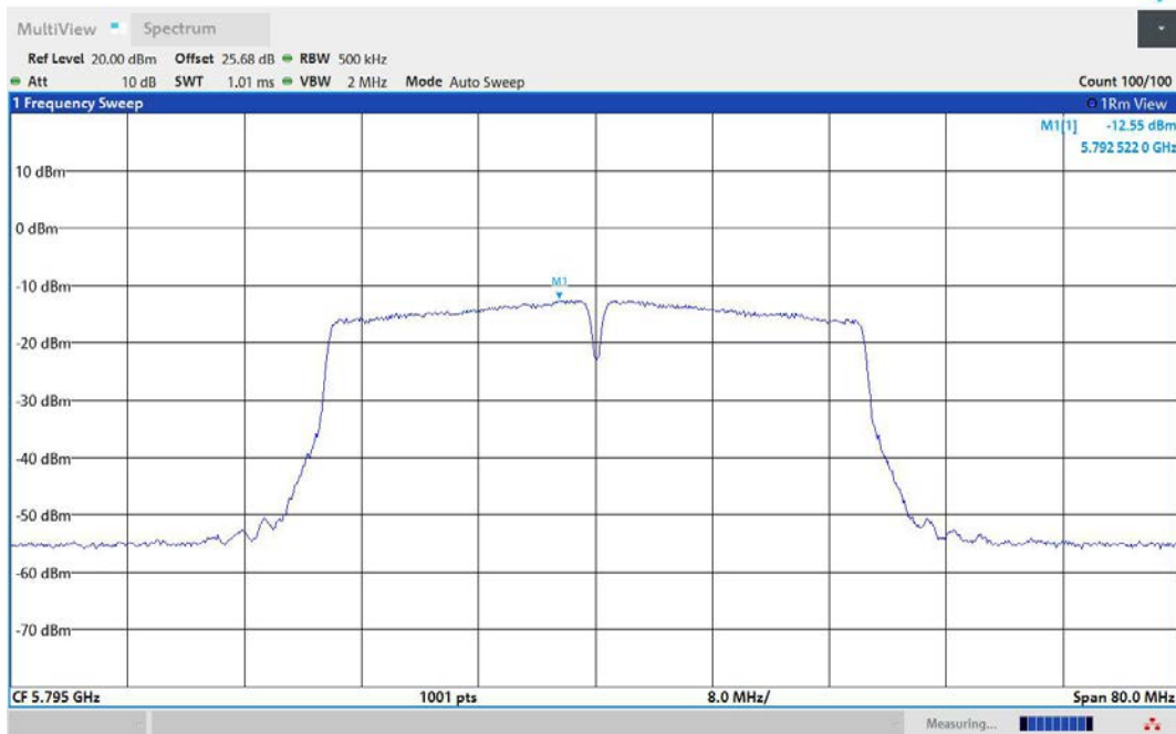
11N40MIMO-Ant3-5795-PASS
