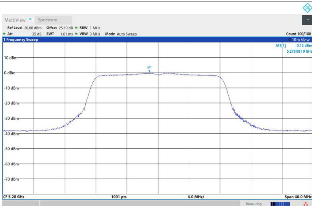
11A-Ant3-5280-PASS
