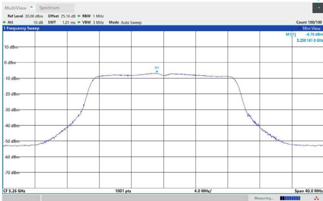
11N20MIMO-Ant3-5260-PASS
