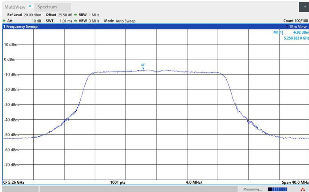
11AC20MIMO-Ant2-5260-PASS
