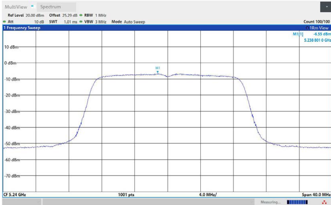
11AC20MIMO-Ant3-5240-PASS
