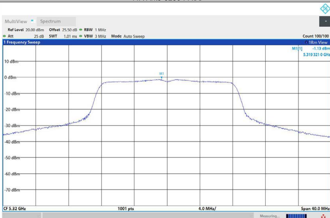
11A-Ant1-5320-PASS
