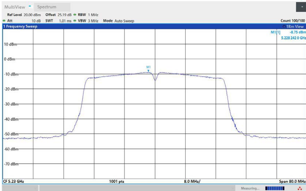
11N40MIMO-Ant3-5230-PASS
