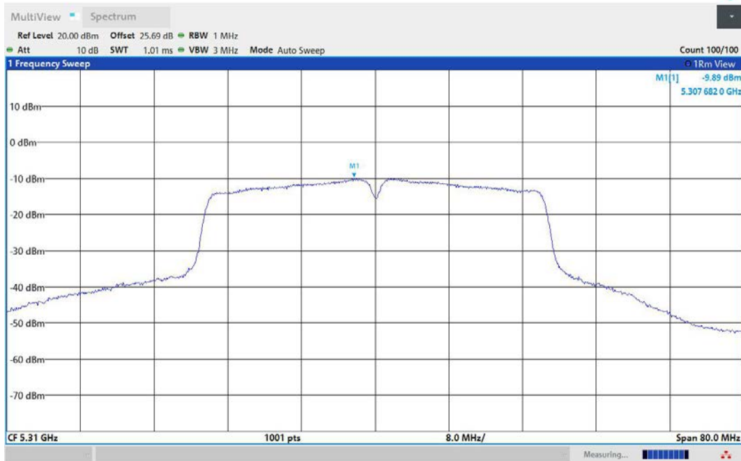
11N40MIMO-Ant3-5310-PASS
