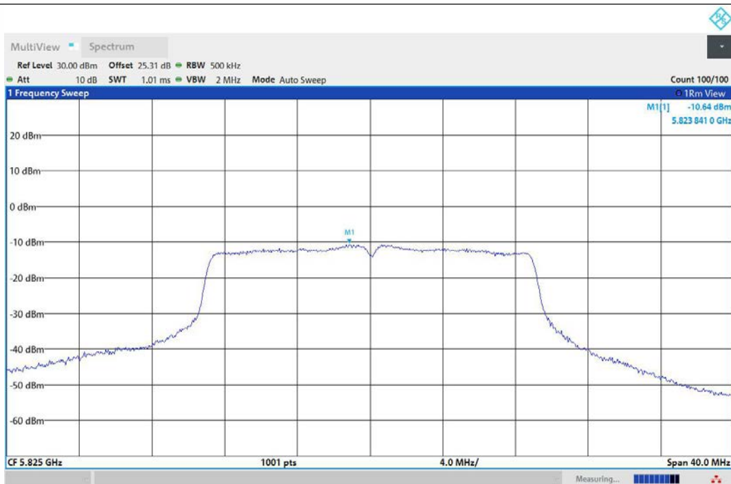
11N20MIMO-Ant2-5825-PASS
