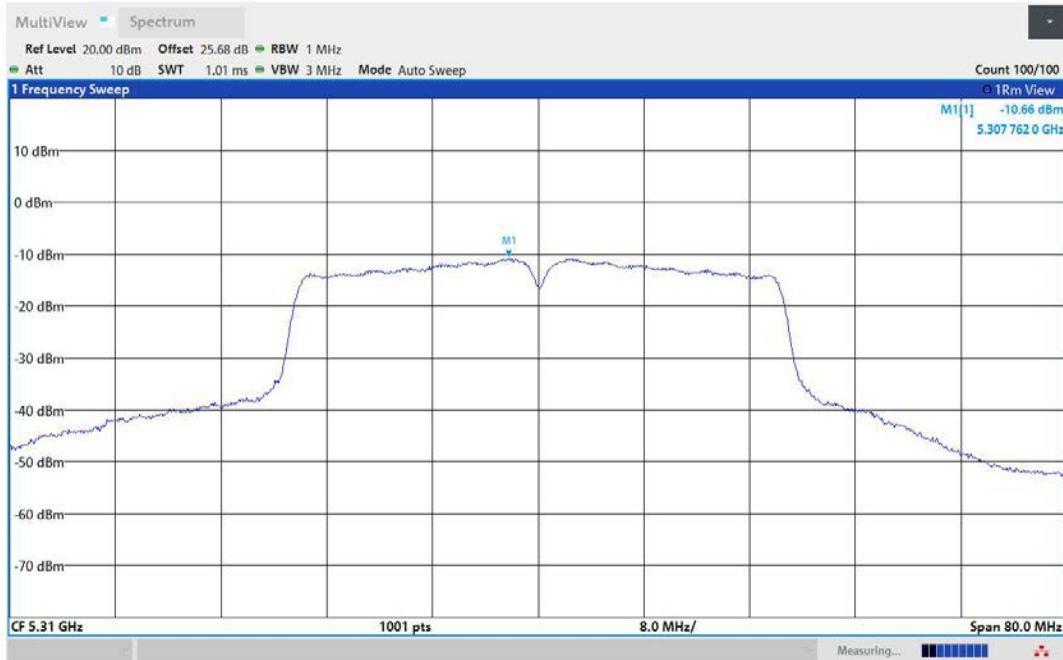
11N40MIMO-Ant1-5310-PASS
